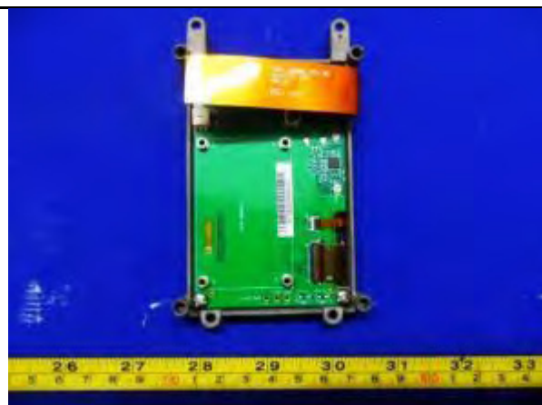
LCD Display - Rear View
