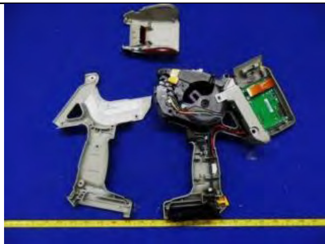
Host – Without Cover
