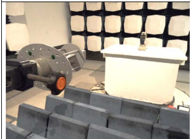
Radiated Emissions (>18GHz) – Front View
