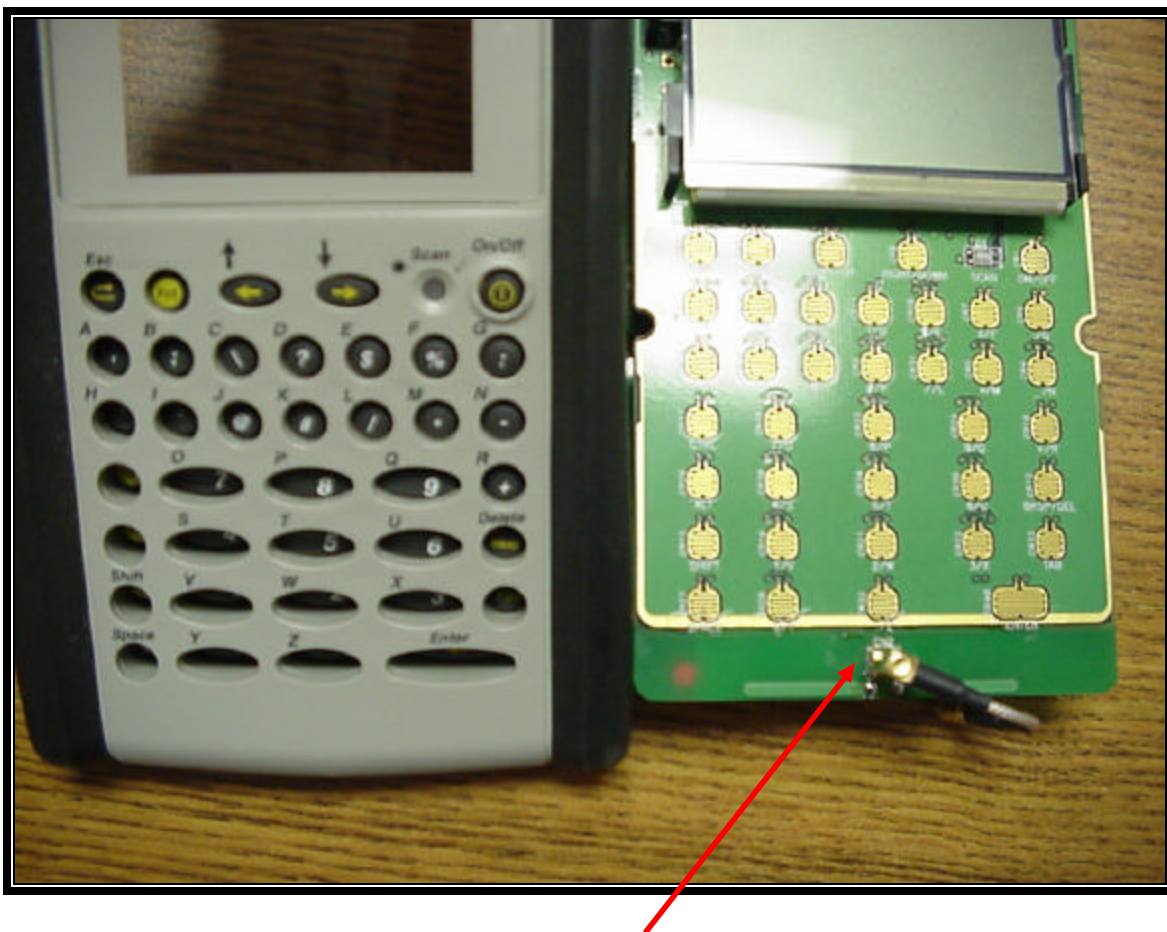
PHOTOGRAPH 13: LOCATION OF ANTENNA RELATIVE TO THE KEYPAD, ON EDGE OF THE PCB
