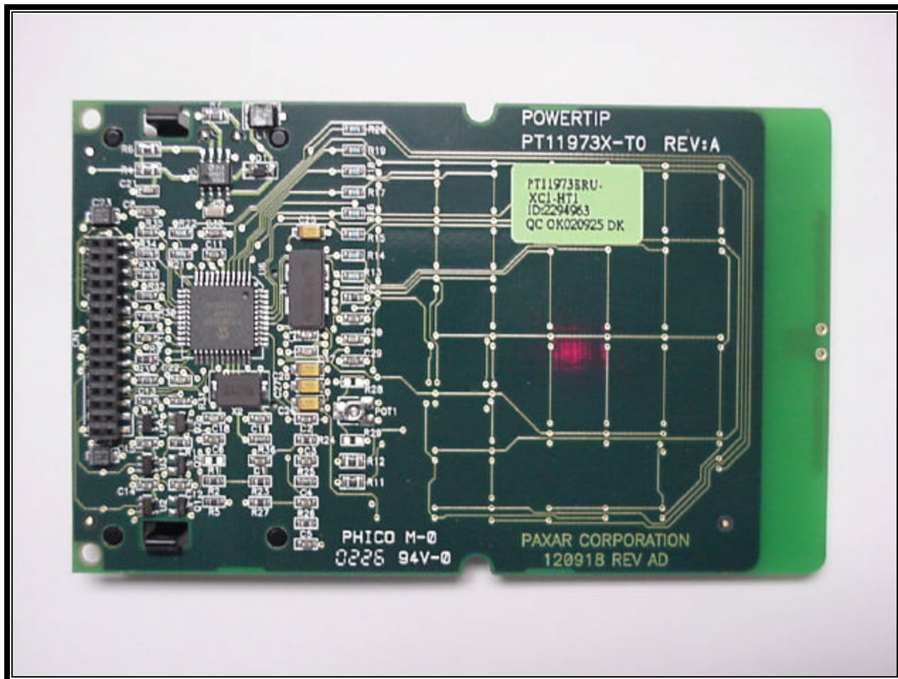
PHOTOGRAPH 19: BOTTOM OF UPPER PCB
