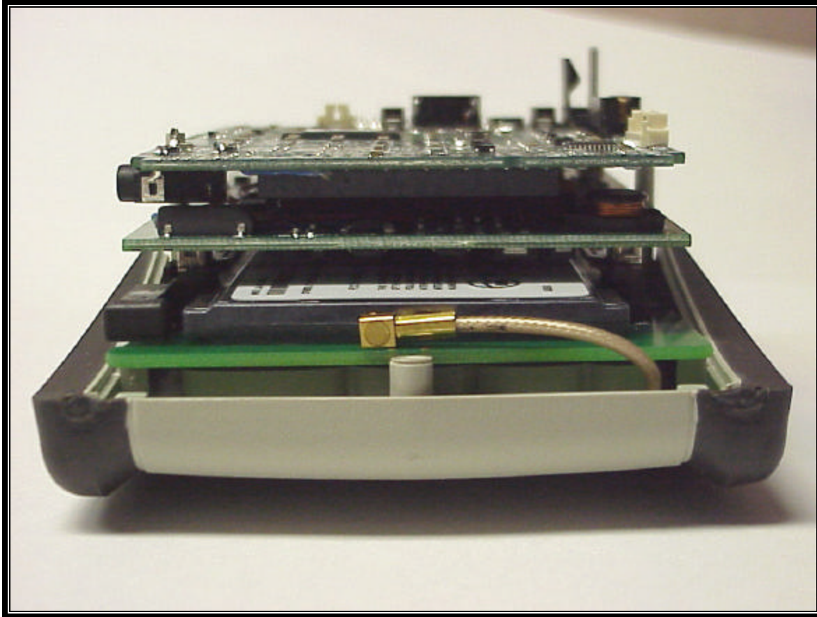
PHOTOGRAPH 15: PCMCIA CARD SLOT; COAX ROUTED BETWEEN CARD AND ANTENNA
