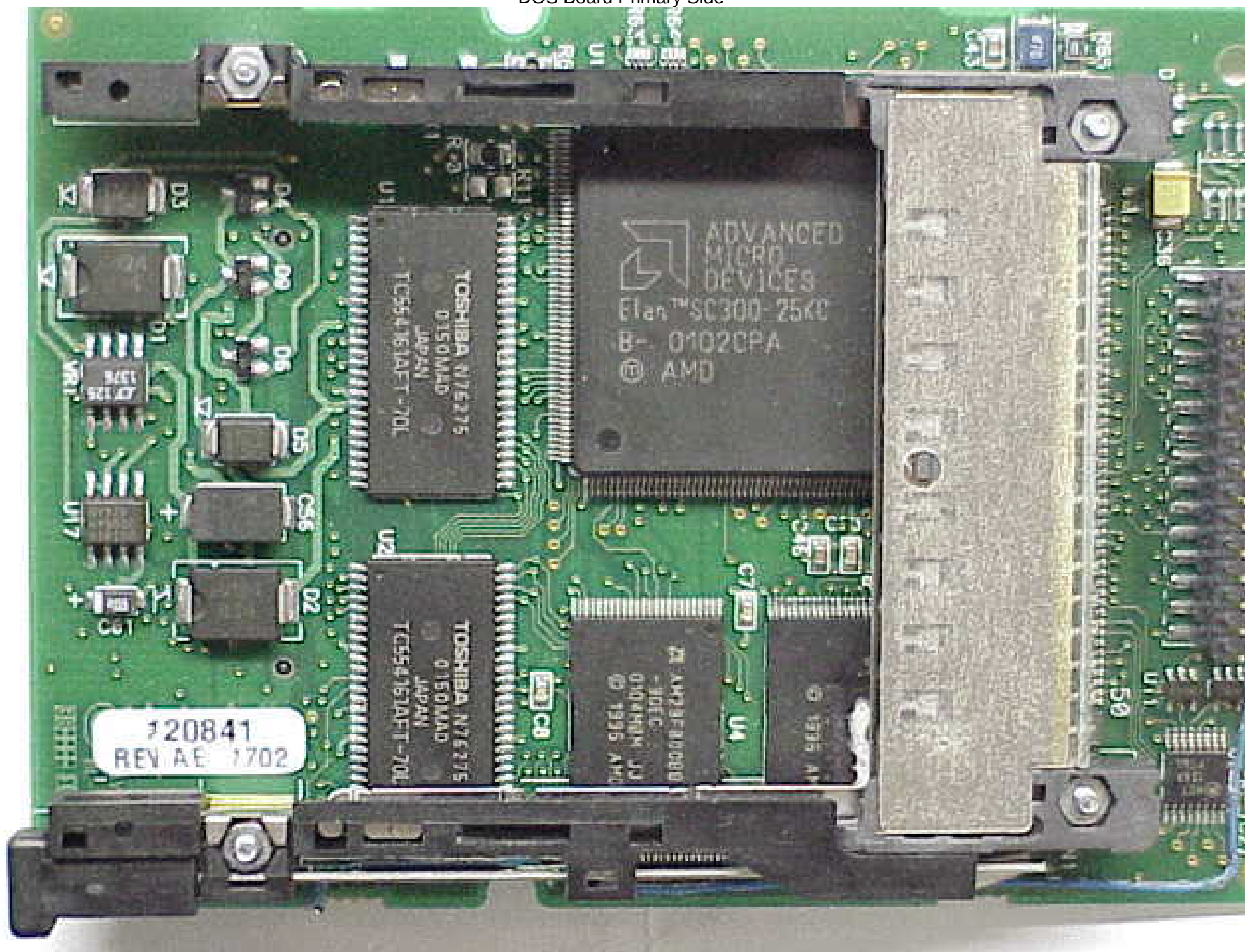
DOS Board Primary Side
