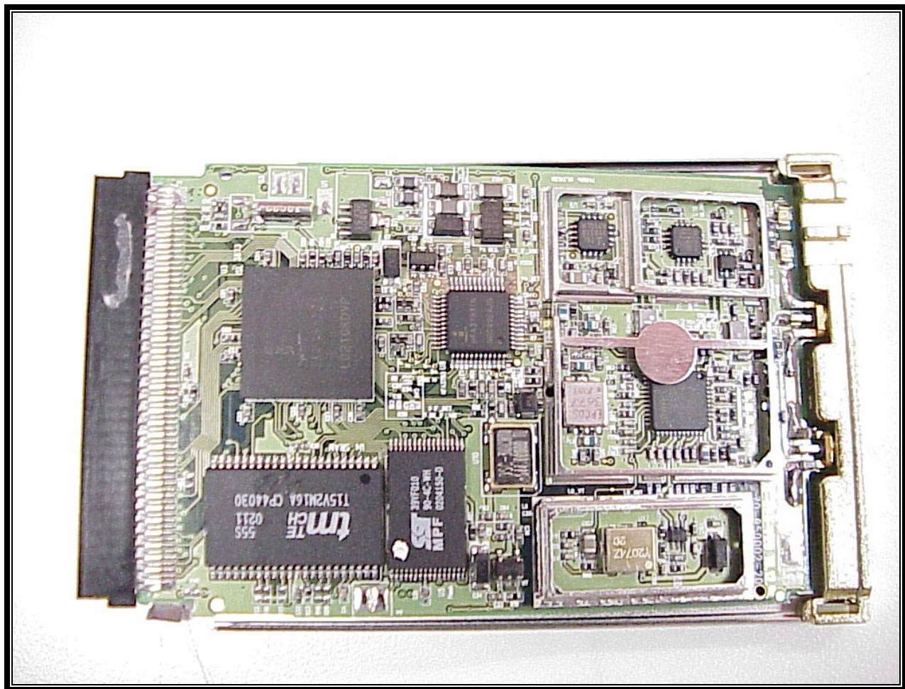
Top View PCMCIA Card Without Shields
