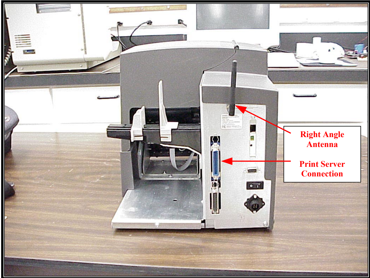
PHOTOGRAPH 15: 98XX SERIES PRINTER WITH PLASTIC HOUSING REAR VIEW
