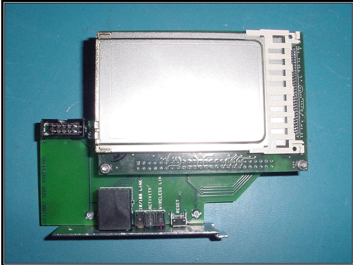
PHOTOGRAPH 18: PRINT SERVER TOP VIEW
