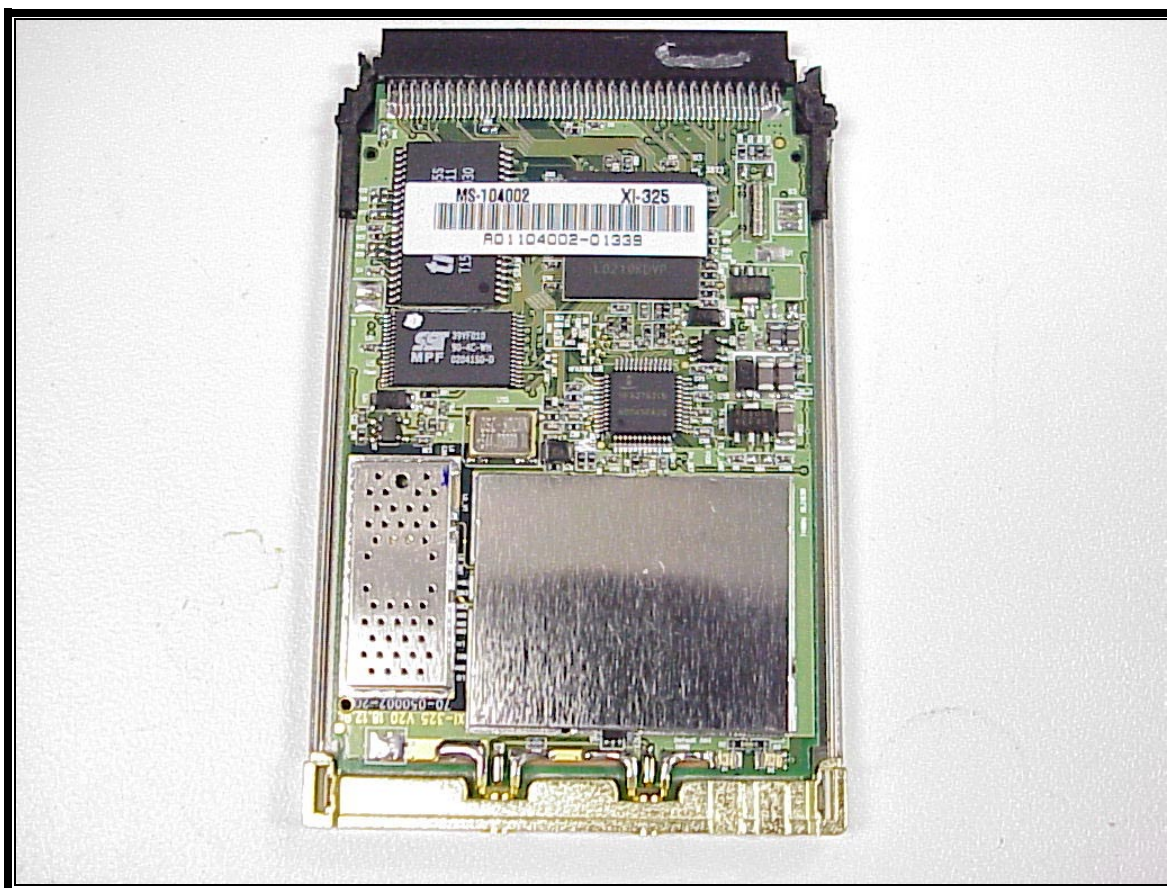
PHOTOGRAPH 26: WLAN CARD PCB FRONT WITH SHIELDS
