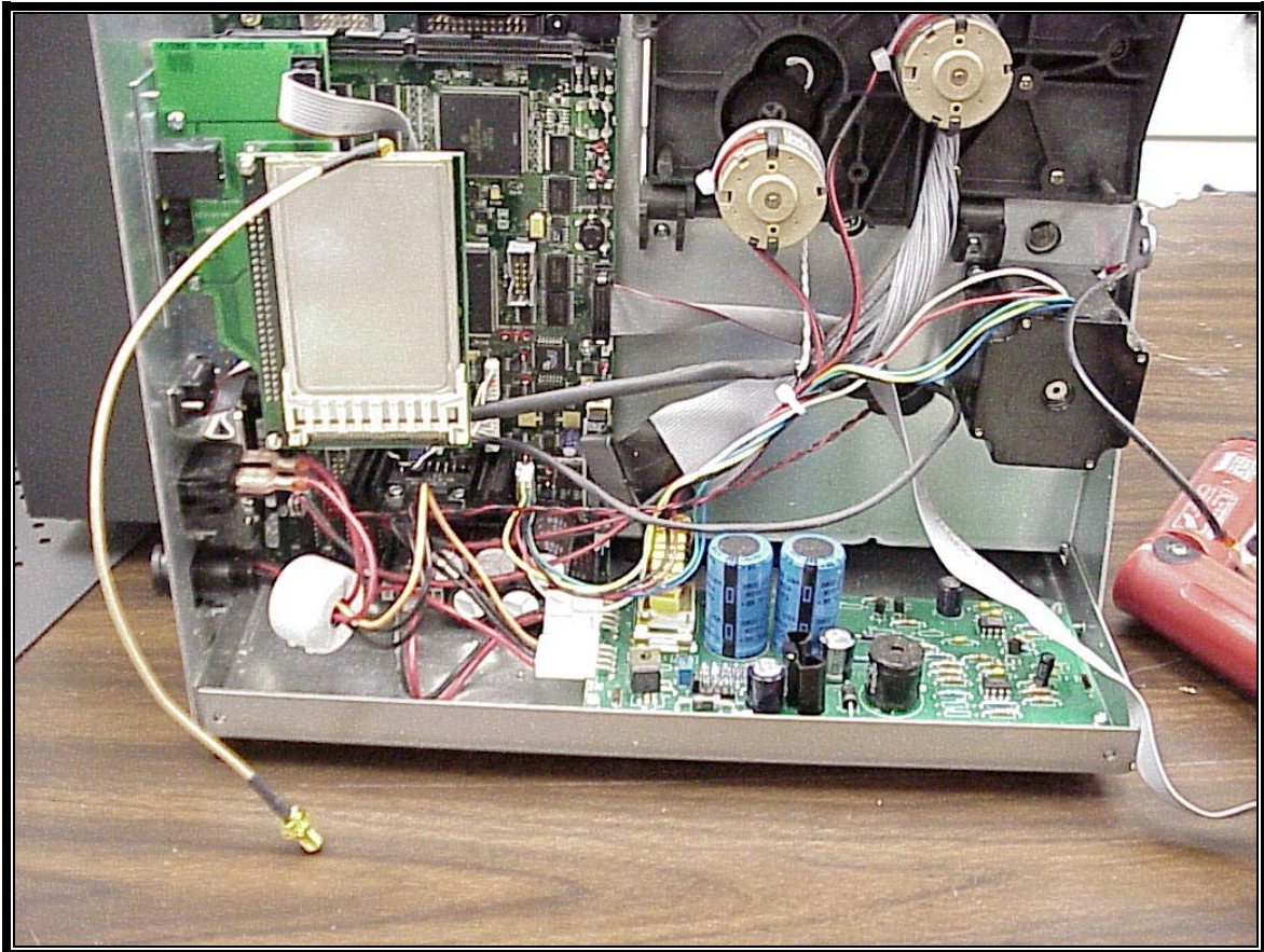
PHOTOGRAPH 30: PRINT SERVER AND WLAN CARD MOUNTED IN PLACE IN HOST
