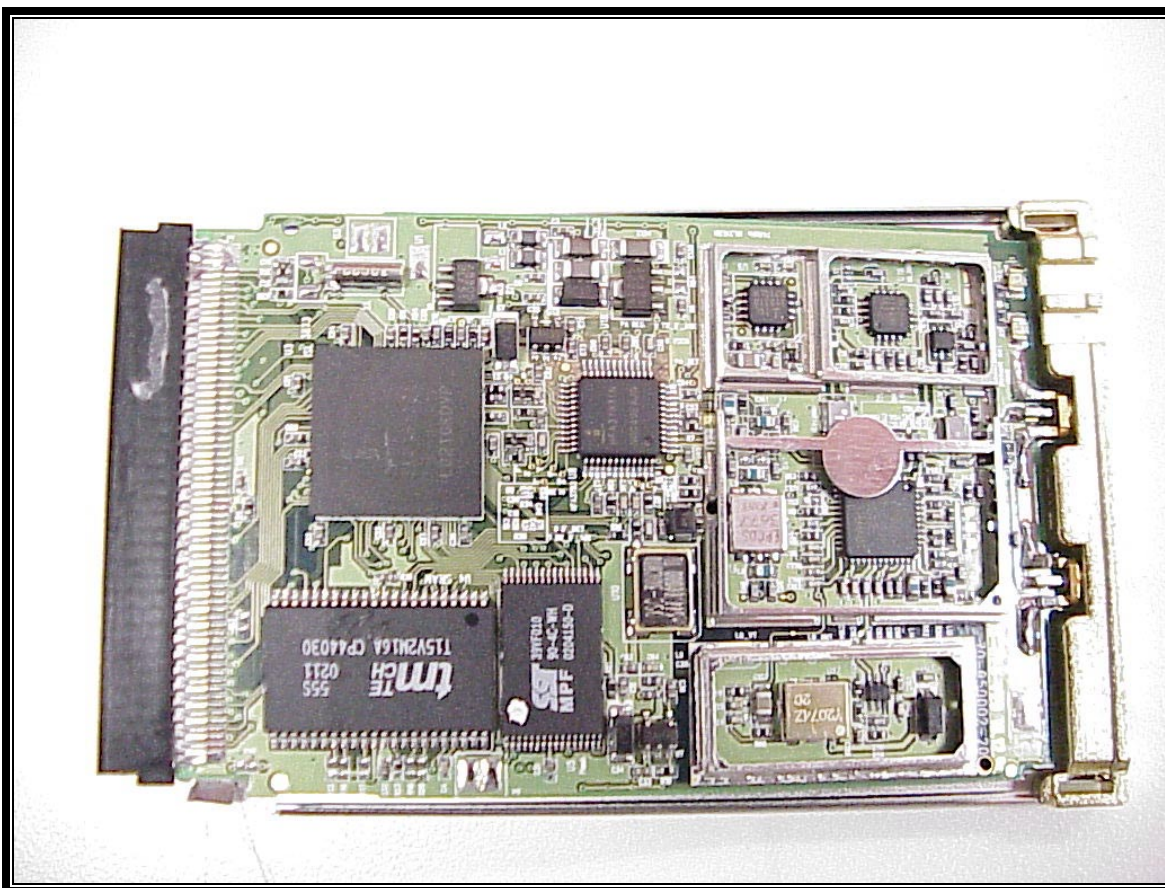
PHOTOGRAPH 28: WLAN CARD PCB FRONT WITHOUT SHIELDS
