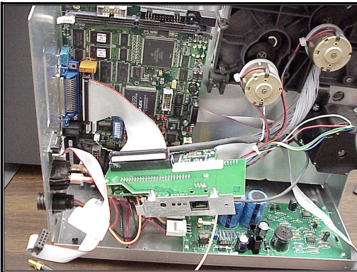
PHOTOGRAPH 29: PRINT SERVER PLUGGED INTO MOUNTED MAIN PCB IN HOST
