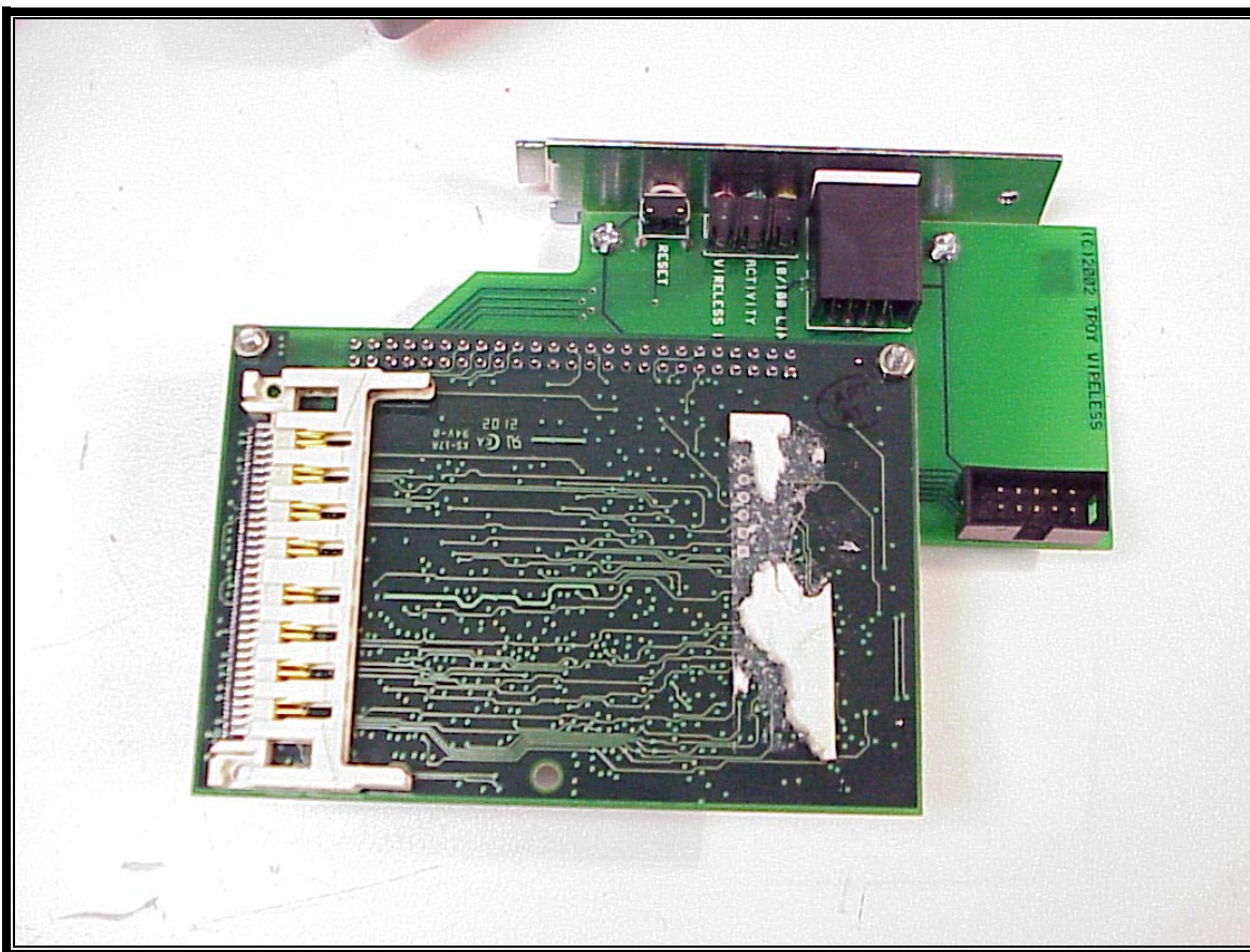
PHOTOGRAPH 25: COMPLETE PRINT SERVER REAR VIEW WITH WLAN CARD REMOVED
