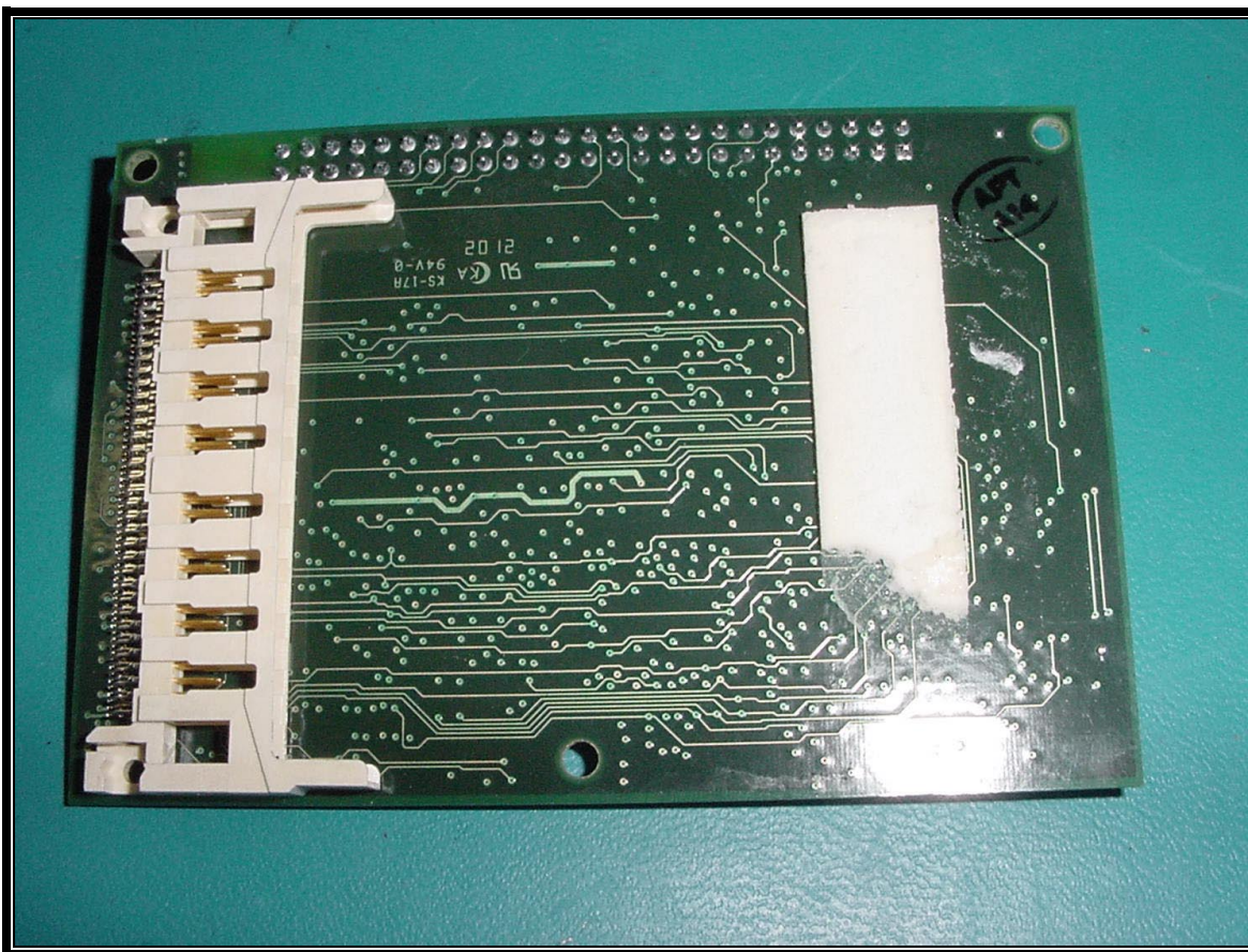
PHOTOGRAPH 24: PRINT SERVER PCB BACK VIEW WITH WLAN PCMCIA CARD AND PCB MOUNTING ADAPTER REMOVED
