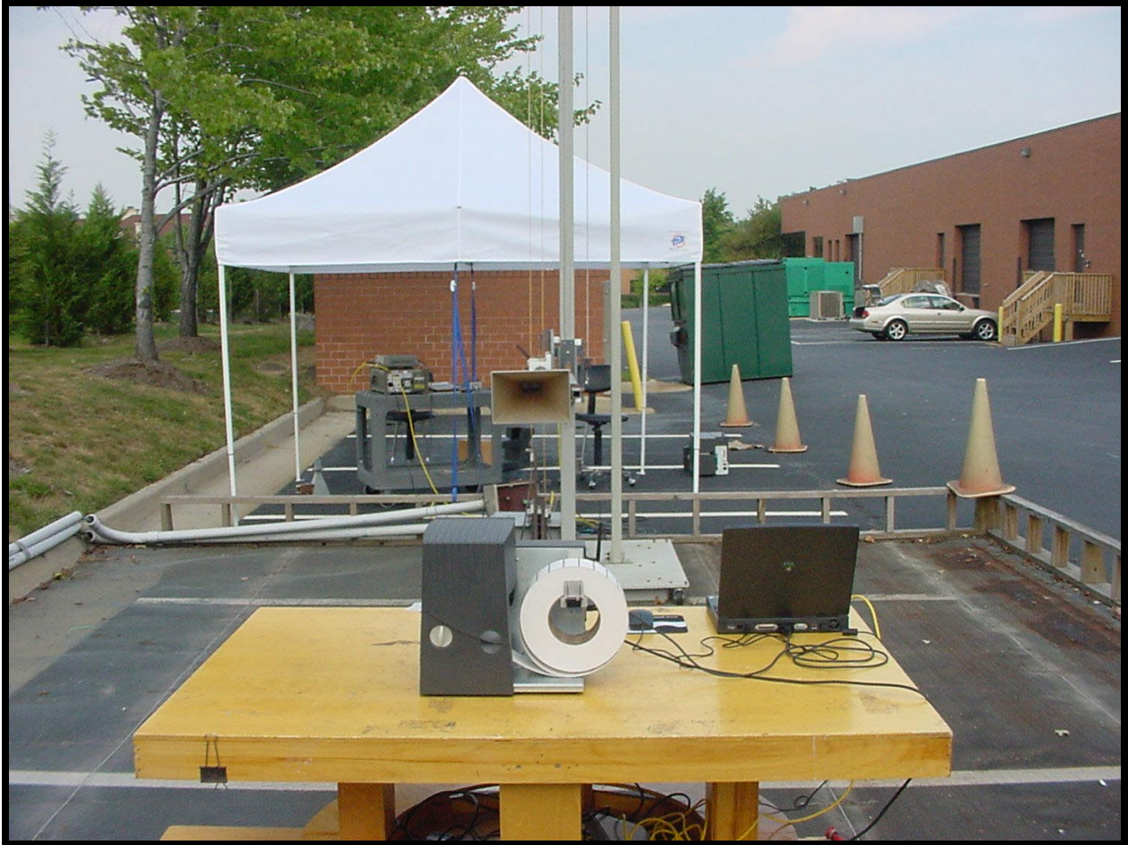
PHOTOGRAPH 7: RADIATED EMISSIONS REAR VIEW; WORST CASE CONFIGURATION
