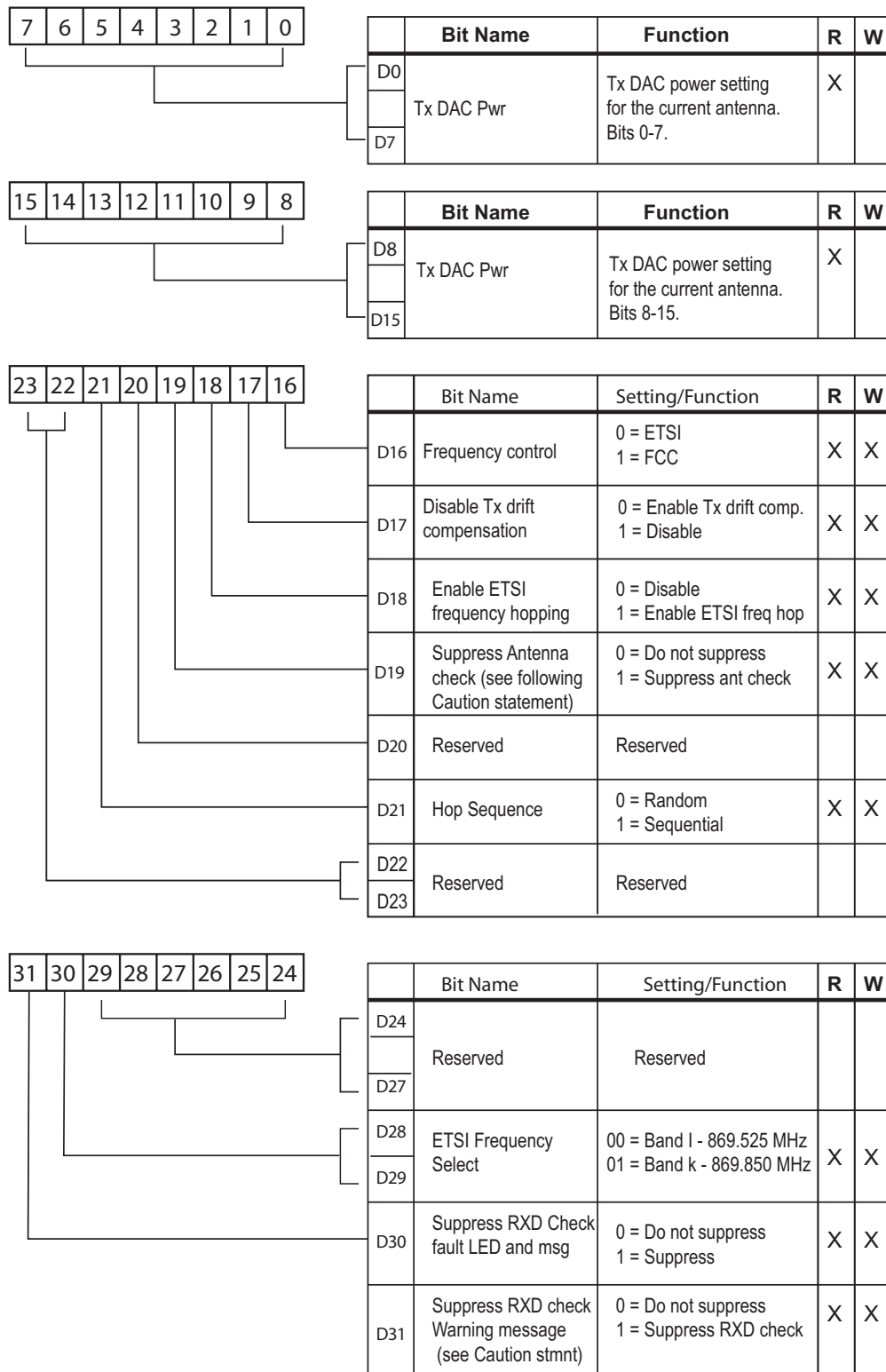
Figure 11–TPC Bit Configuration
