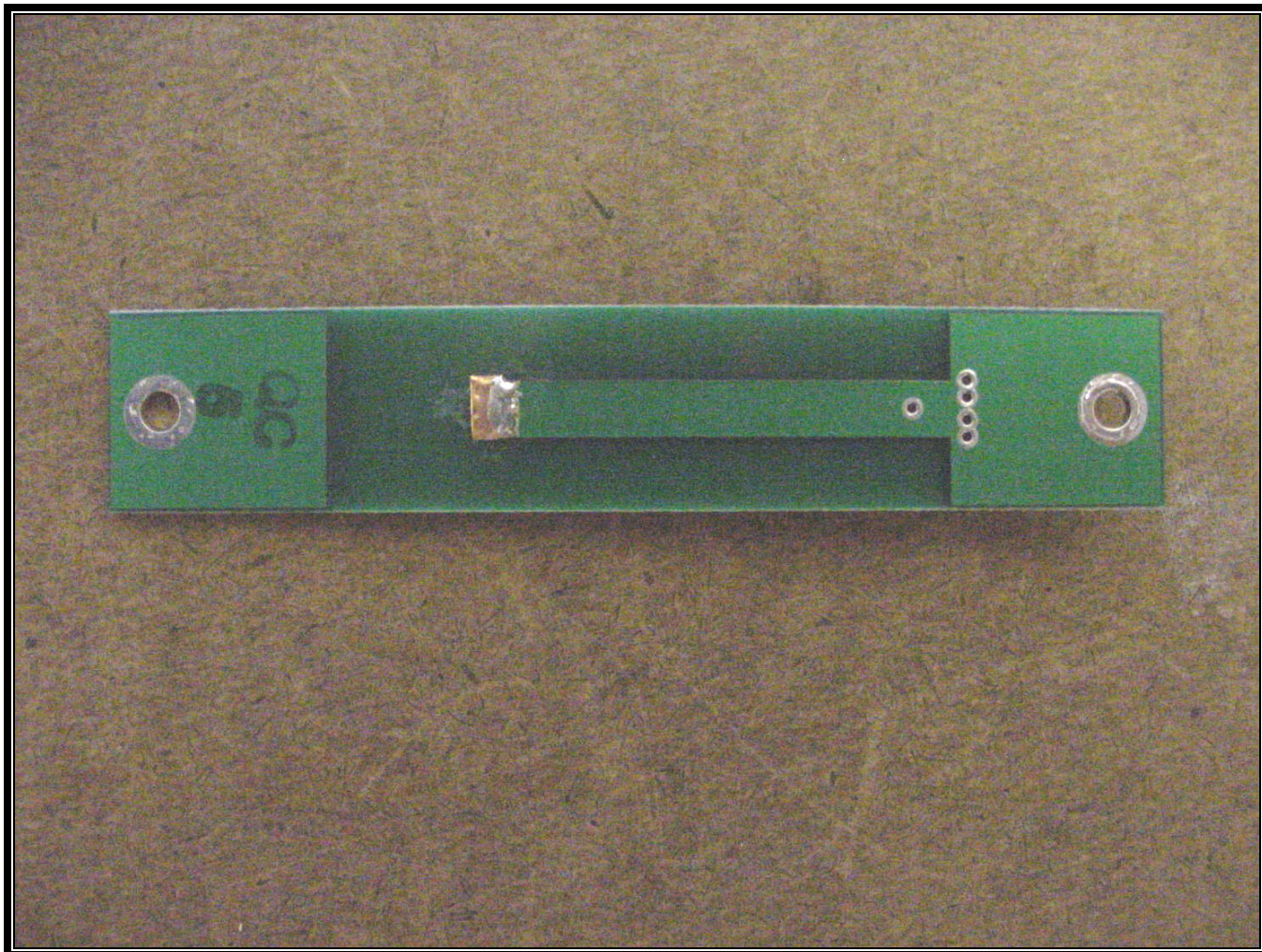
PHOTOGRAPH 10: ANTENNA FRONT
