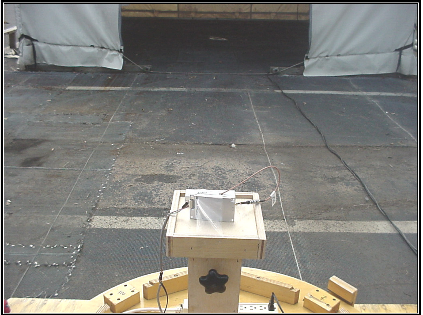
PHOTOGRAPH 3: RADIATED EMISSIONS REAR VIEW (3M)
