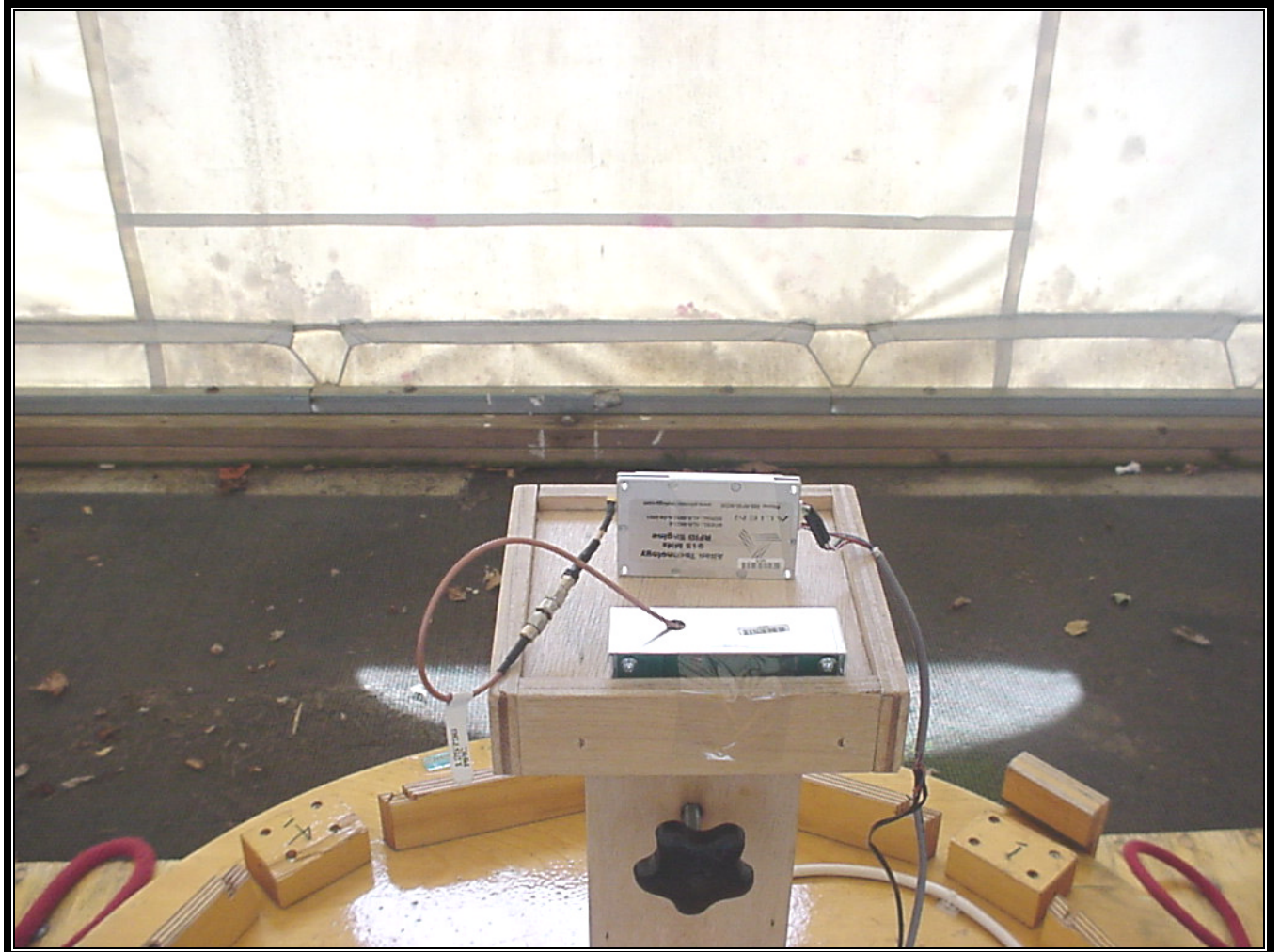
PHOTOGRAPH 4: RADIATED EMISSIONS FRONT VIEW (10M)
