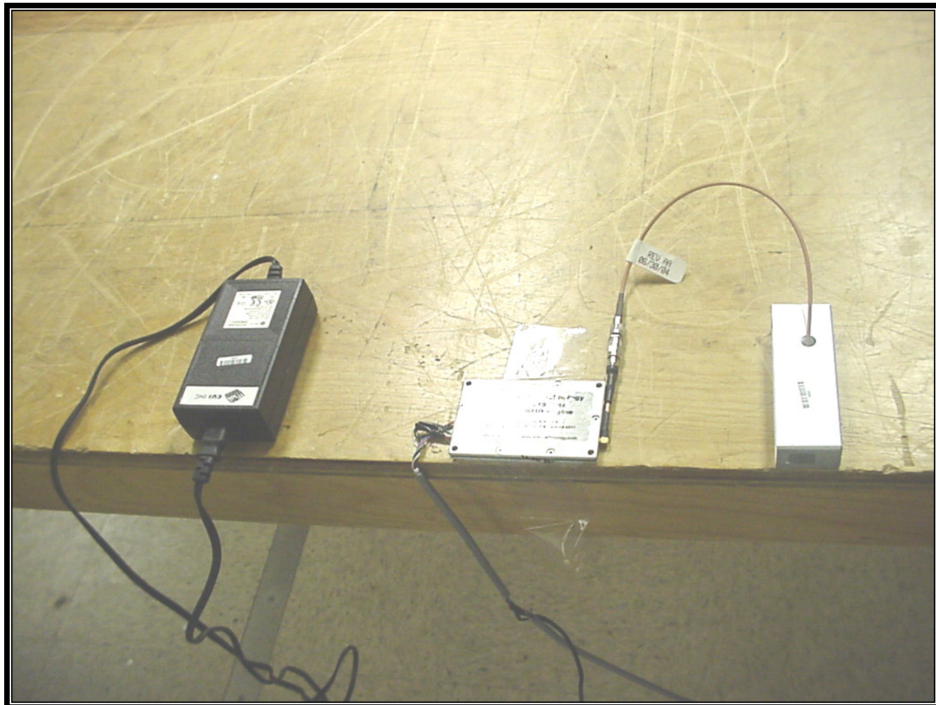
PHOTOGRAPH 7: CONDUCTED EMISSIONS REAR VIEW
