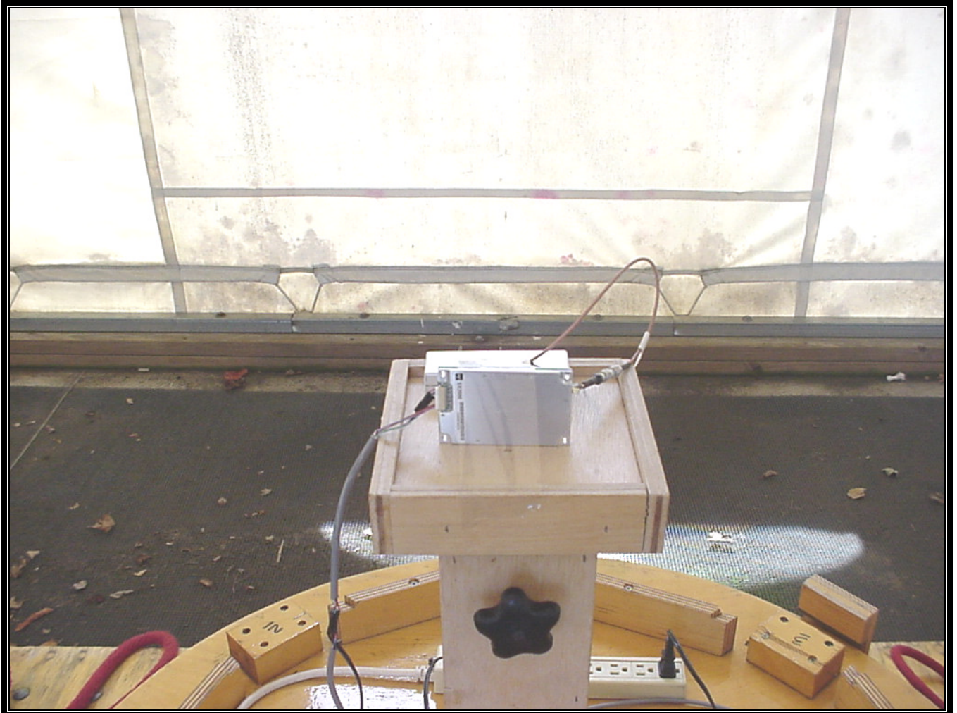
PHOTOGRAPH 5: RADIATED EMISSIONS REAR VIEW (10M)
