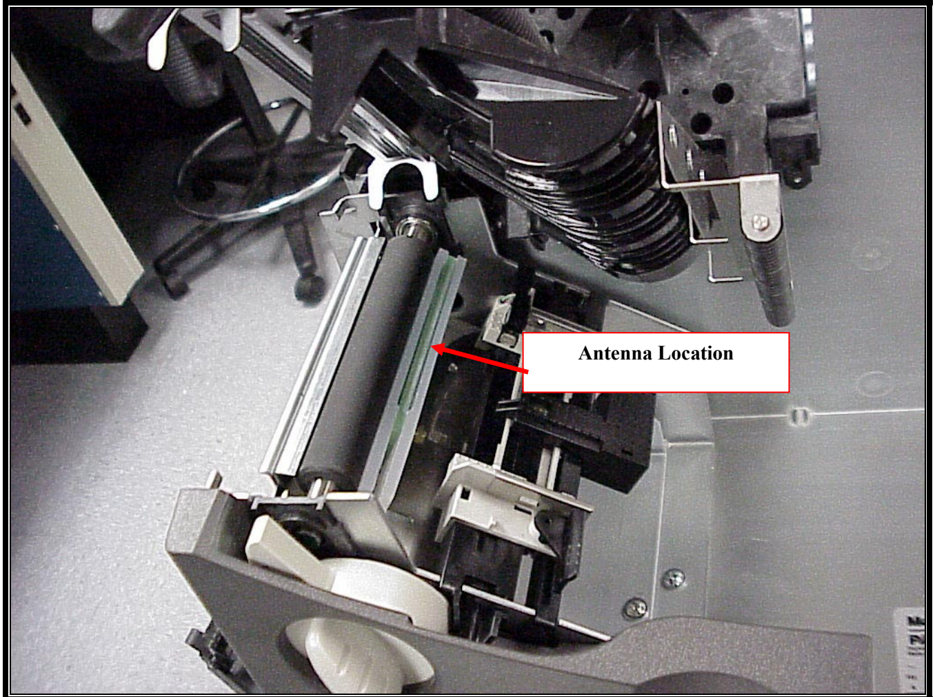
PHOTOGRAPH 15: ANTENNA LOCATION
