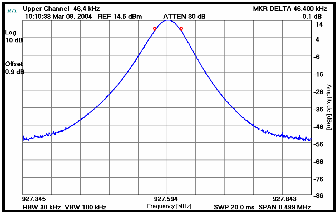
PLOT 9-3: MODULATED BANDWIDTH HIGH CHANNEL
