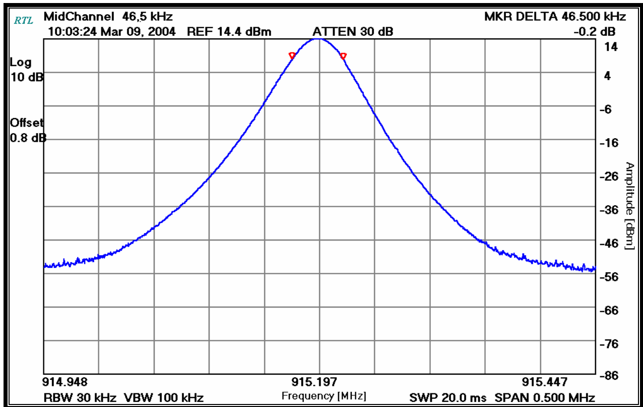
PLOT 9-2: MODULATED BANDWIDTH MID CHANNEL
