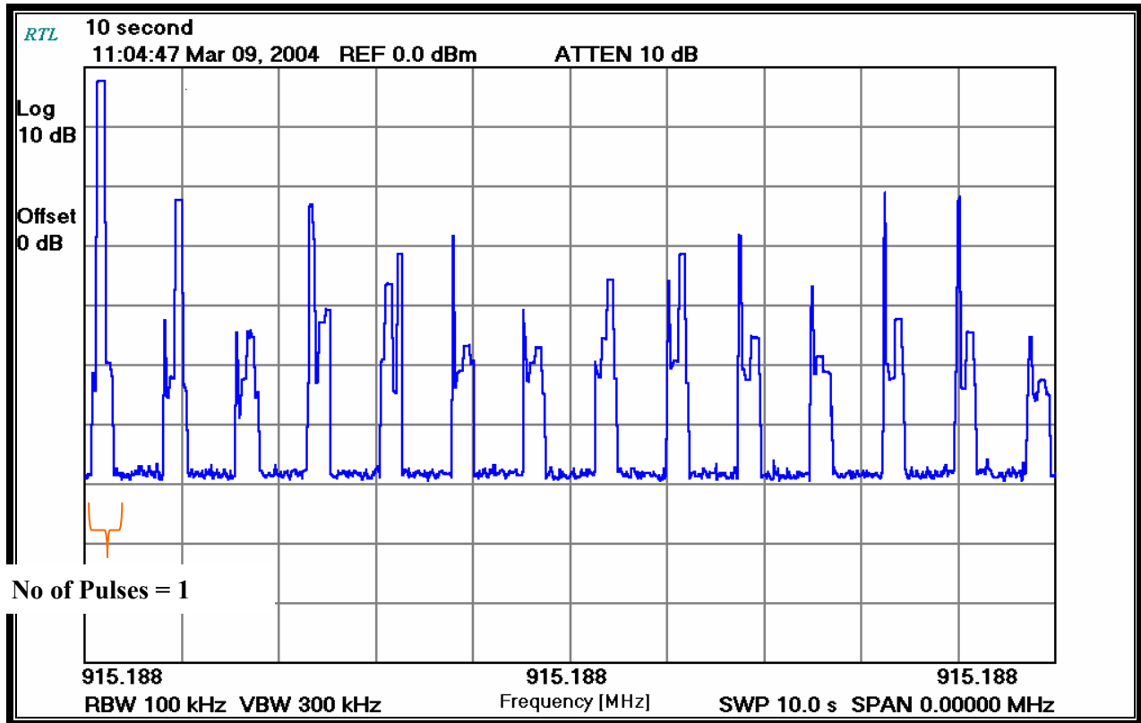
PLOT 8-6: TIME OF OCCUPANCY (DWELL TIME 10 SECOND SWEEP)
