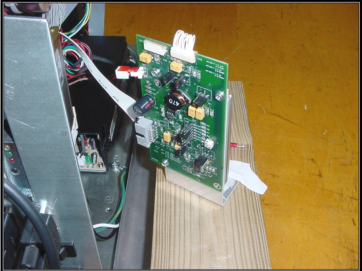
PHOTOGRAPH 2: MODULE SHOWN SEPARATED FROM PRINTER FOR TESTING
