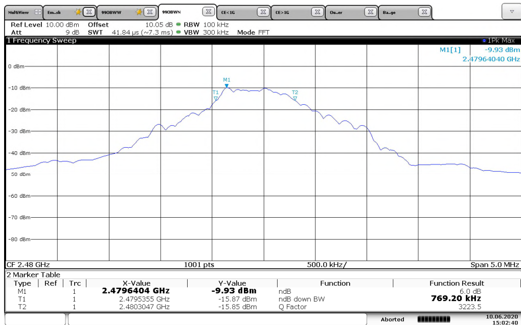
Figure 7.3.2-5: 6dB Bandwidth High Channel
