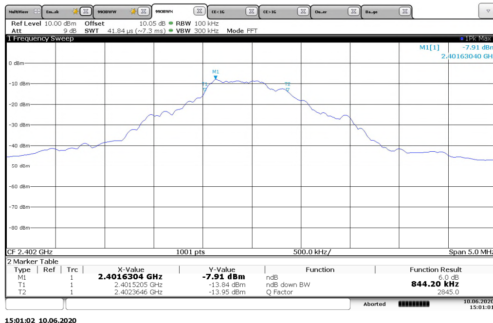
Figure 7.3.2-1: 6dB Bandwidth Low Channel
