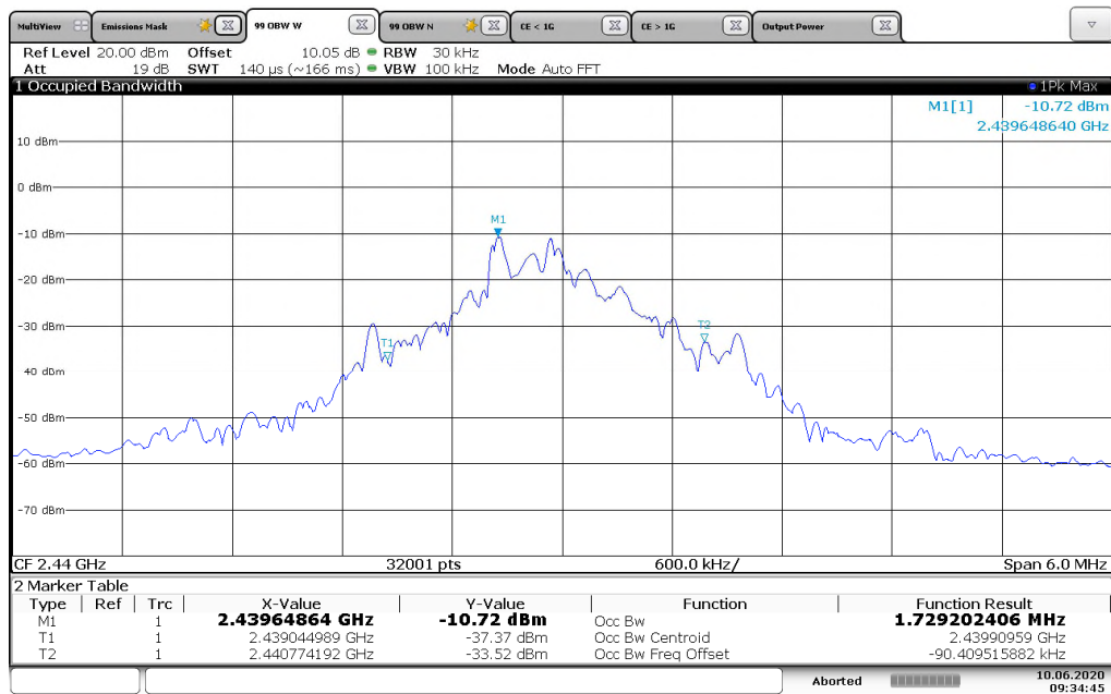
Figure 7.3.2-4: 99% Bandwidth Mid Channel
