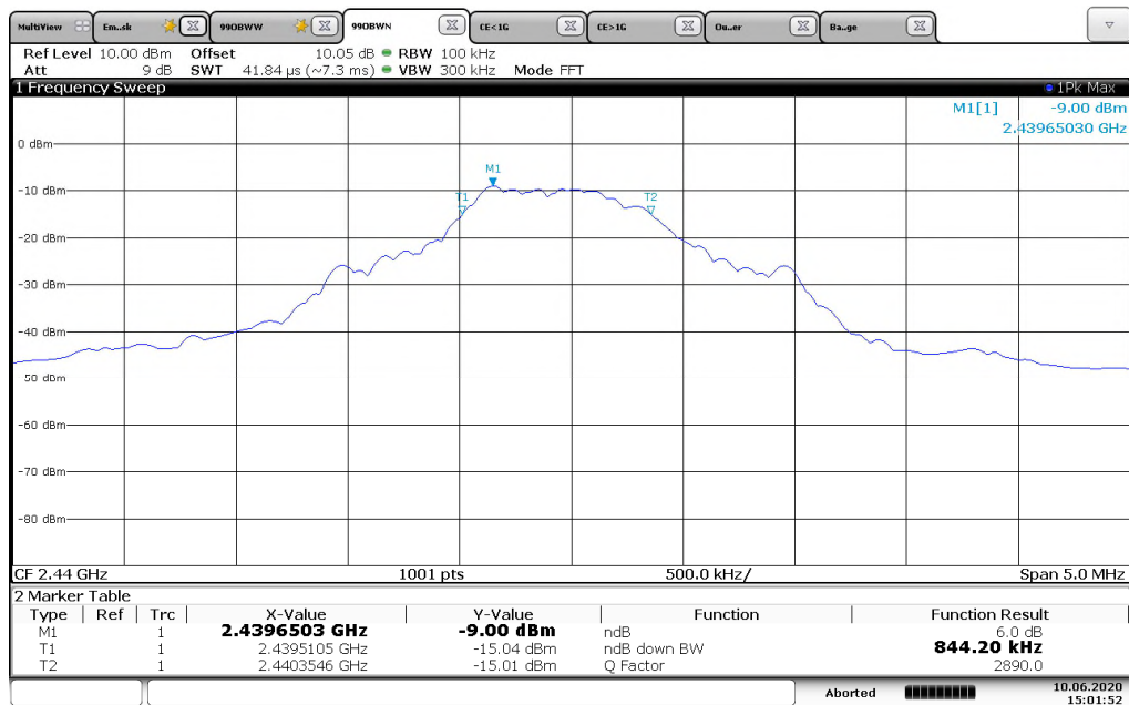
Figure 7.3.2-3: 6dB Bandwidth Mid Channel
