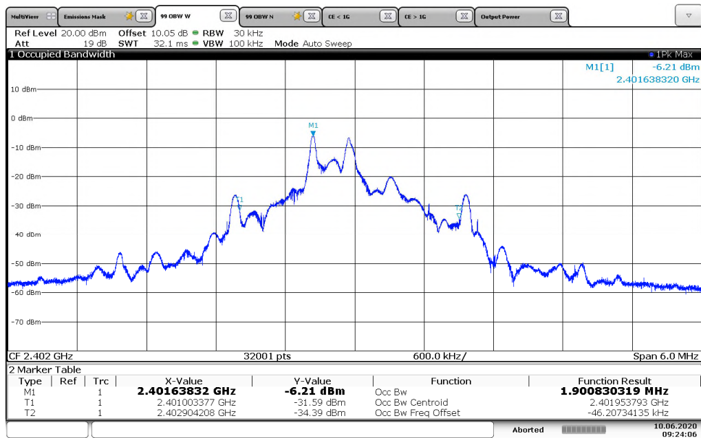
Figure 7.3.2-2: 99% Bandwidth Low Channel
