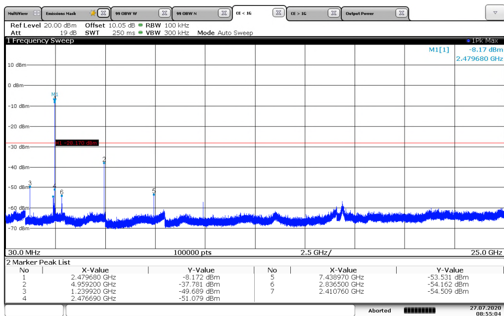
Figure 7.5.1.2-3: 30 MHz - 25 GHz – HCH
