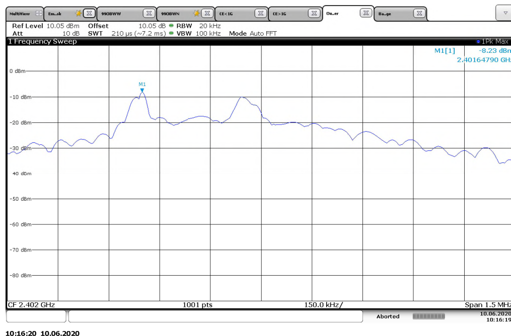
Figure 7.6.2-1: PSD Plot –LCH
