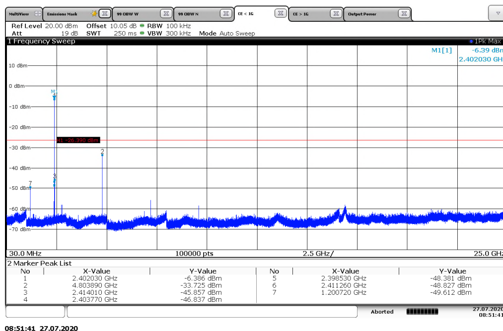
Figure 7.5.1.2-1: 30 MHz - 25 GHz – LCH
