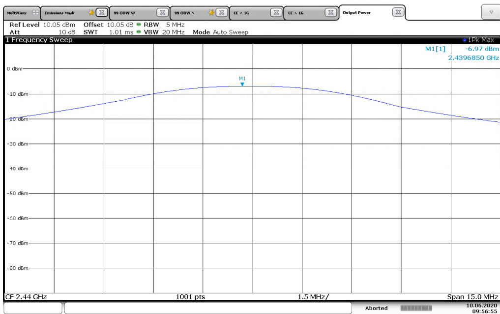
Figure 7.4.2-2: Mid Channel
