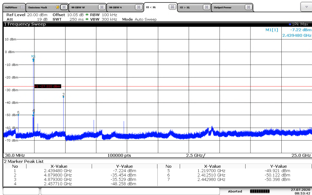
Figure 7.5.1.2-2: 30 MHz – 25 GHz – MCH
