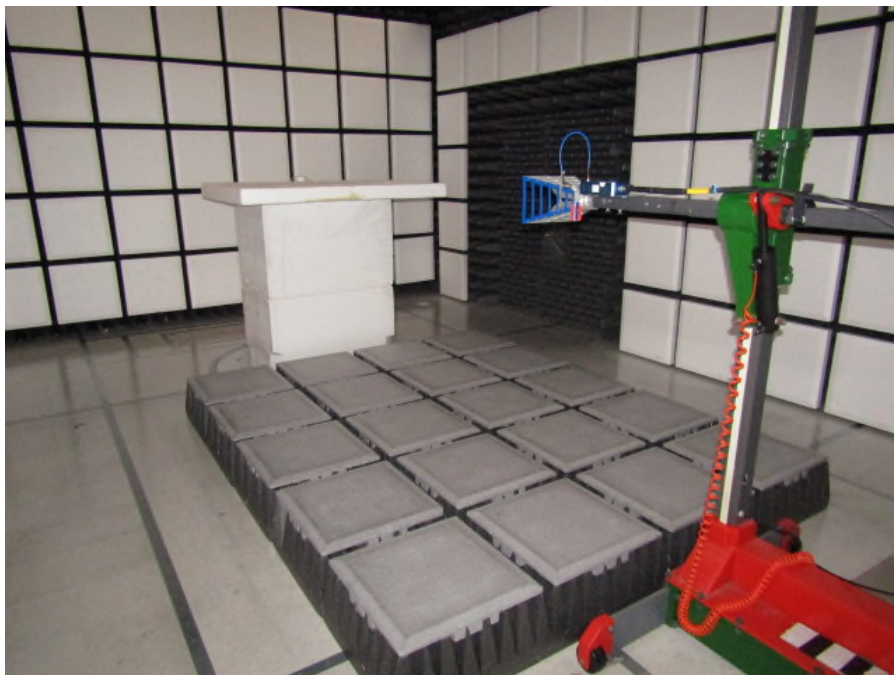
Figure 3: Radiated Emissions – Front – Above 1GHz
