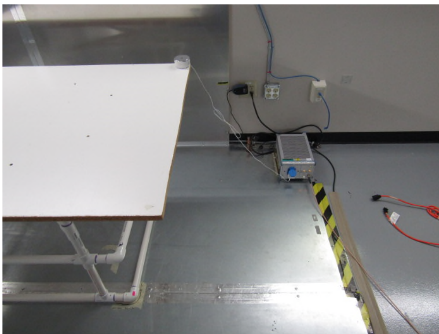
Figure 6: Conducted Emissions
