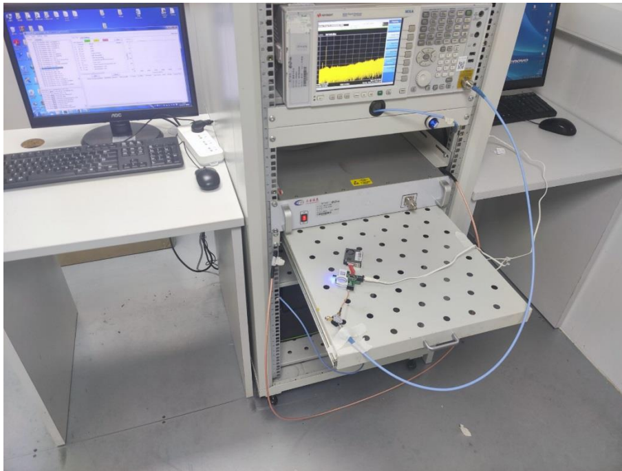
Conducted Test-2.4G
