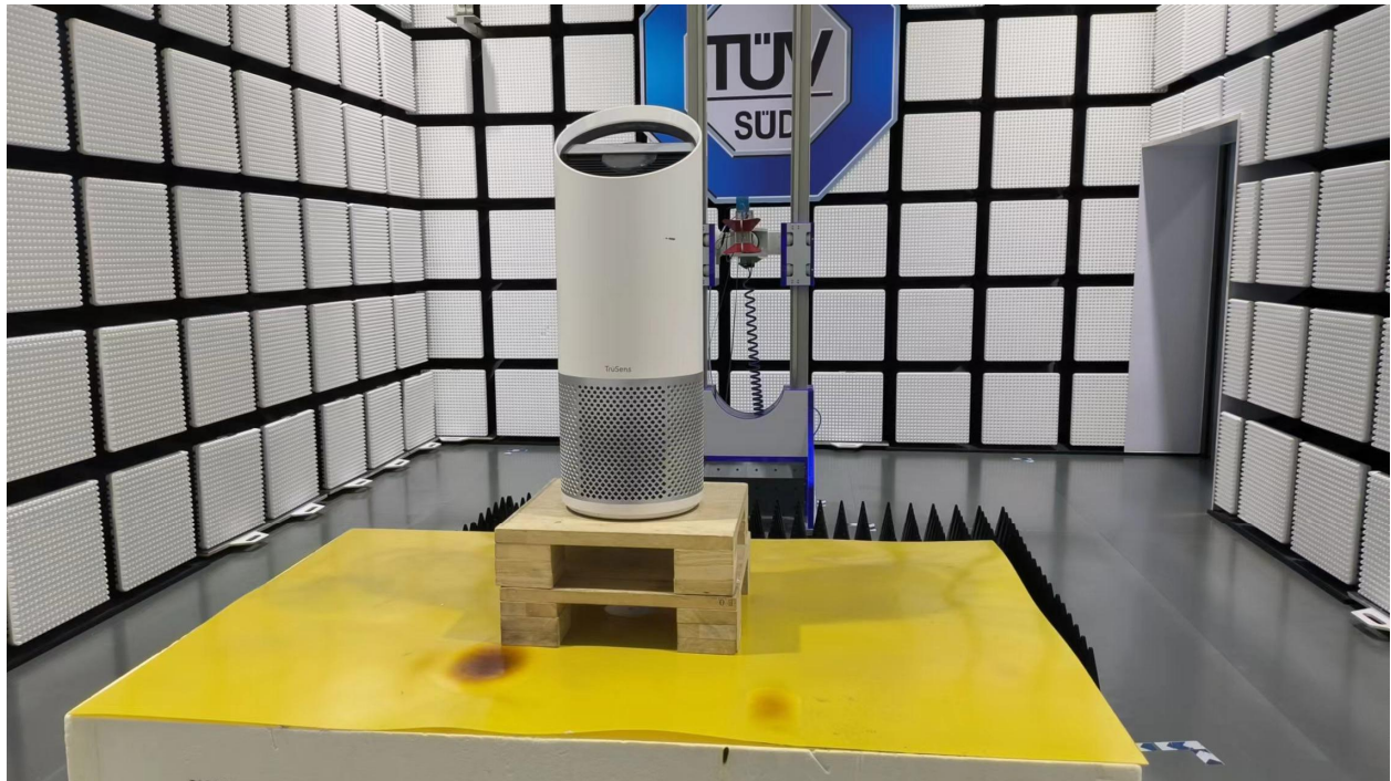
Radiated Emission Test 18GHz-40GHz
