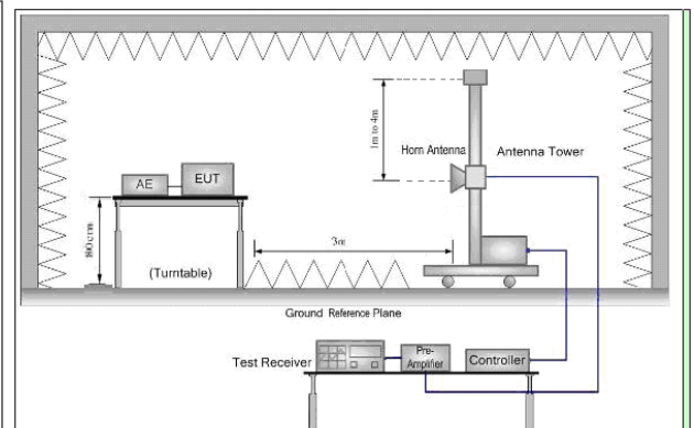
Figure 2. Above 1 GHz
