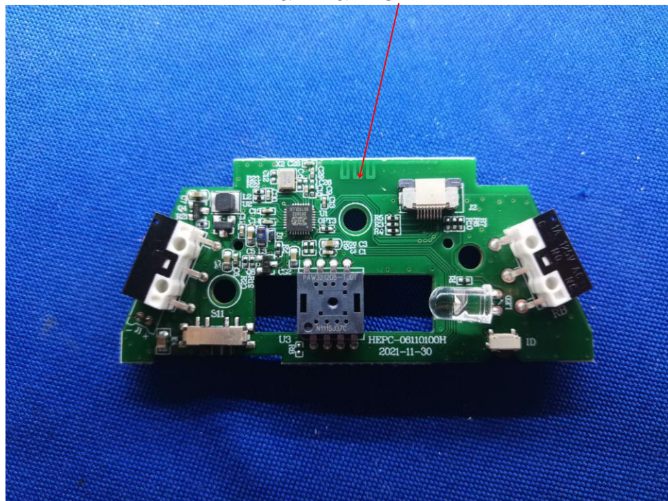
BDR&BLE&2.4G ANT
