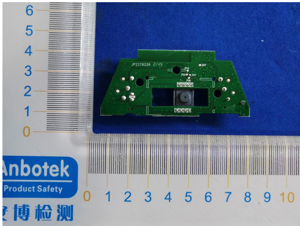
BDR&BLE&2.4G ANT
