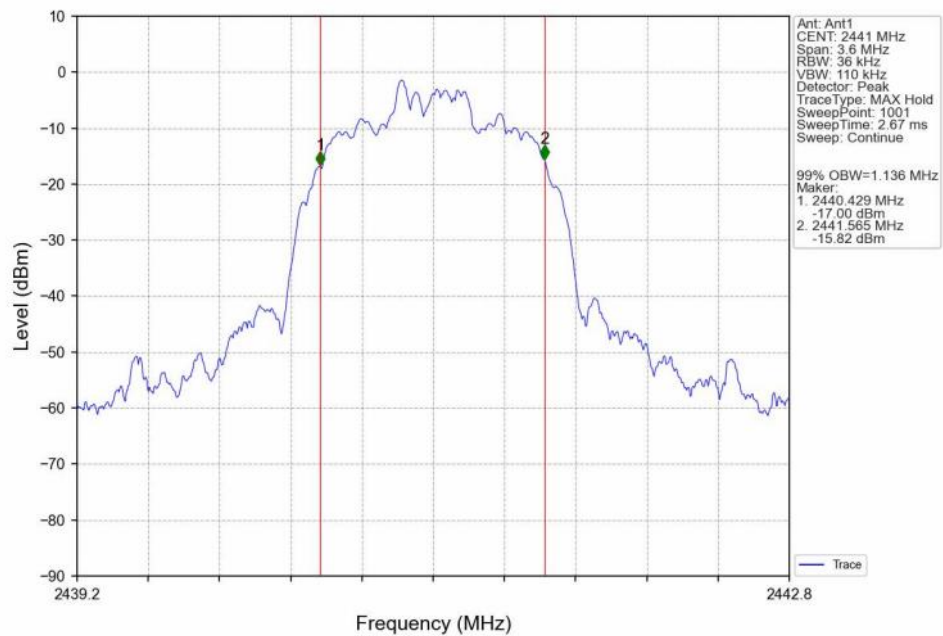
99%_Occupied_Bandwidth_NVNT_ANT1_2-DH5_2441
