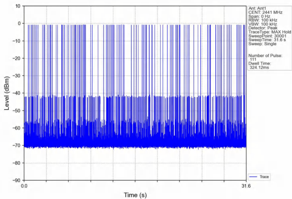
Dwell_Time_(Hopping)_NVNT_ANT1_3-DH5_2441_Accumulated
