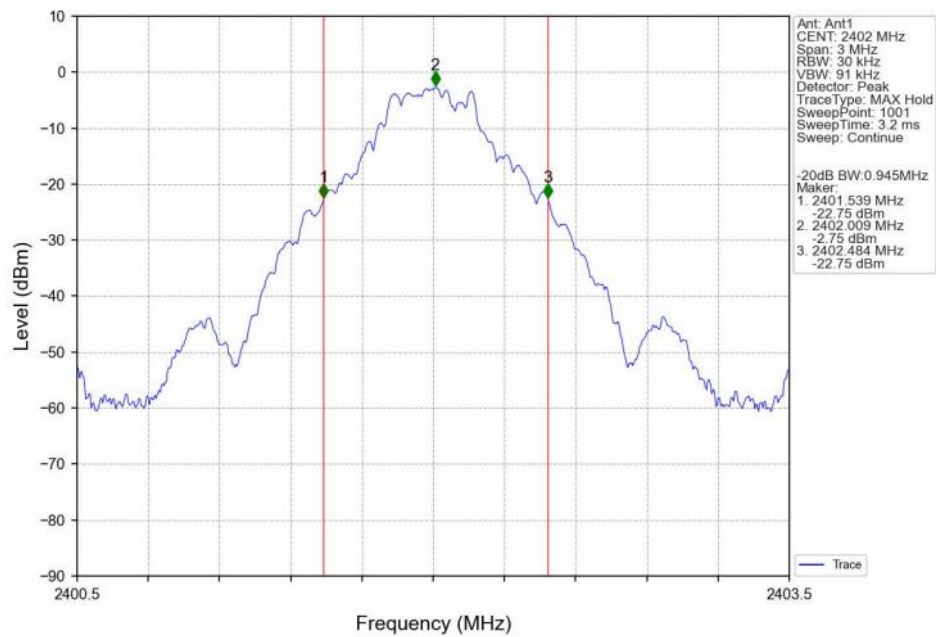
-20dB_Bandwidth_NVNT_ANT1_DH5_2402
