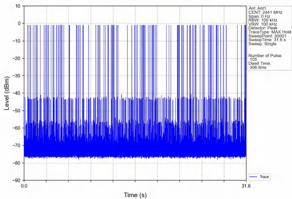
Dwell_Time_(Hopping)_NVNT_ANT1_2-DH5_2441_Accumulated
