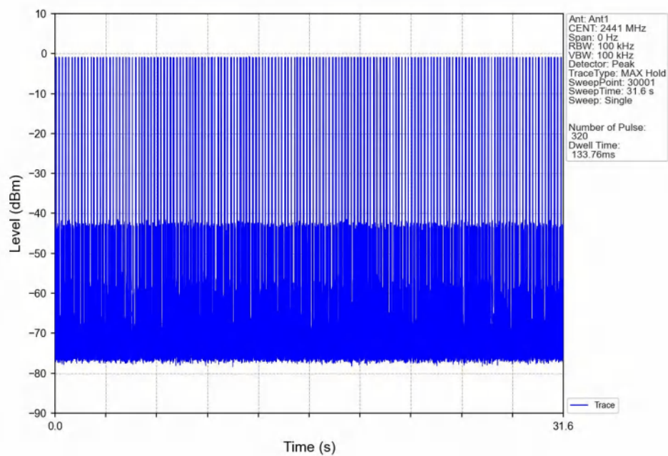
Dwell_Time_(Hopping)_NVNT_ANT1_2-DH1_2441_Accumulated
