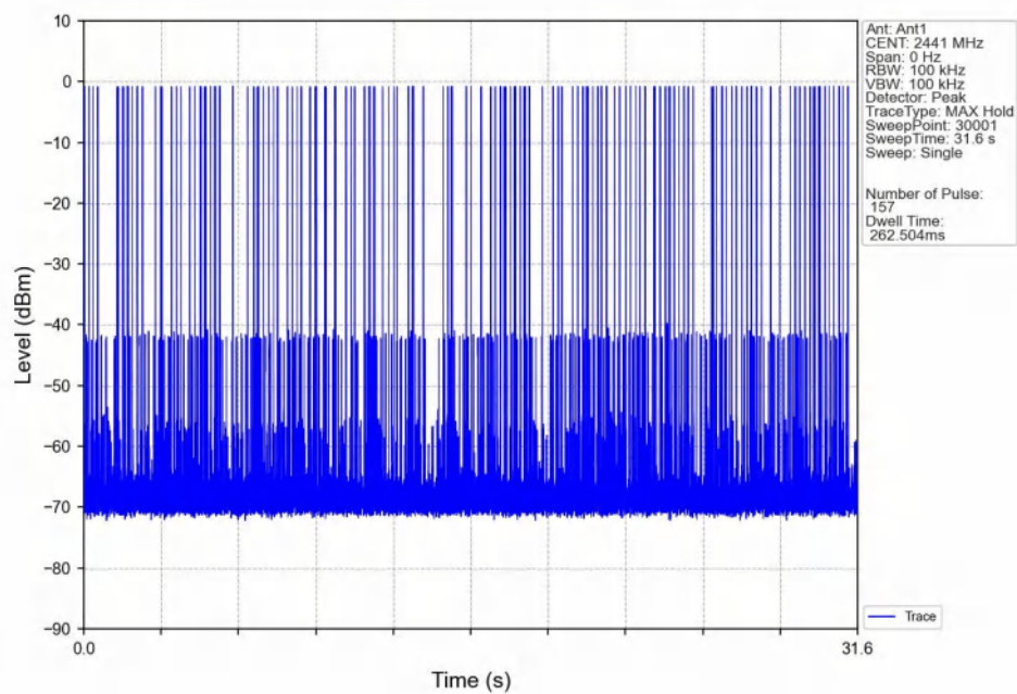
Dwell_Time_(Hopping)_NVNT_ANT1_3-DH3_2441_Accumulated
