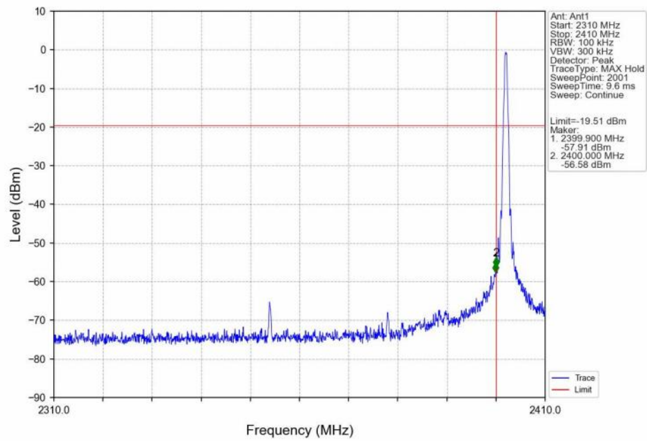
GFSK_DH5_LCH_2402MHz_Ant1_NTNV
