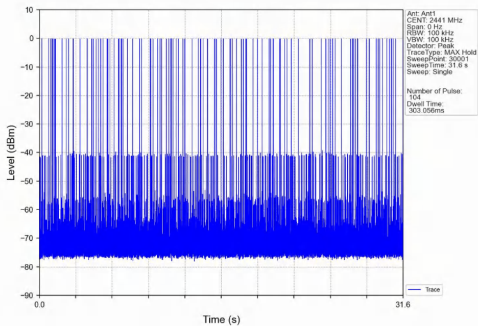
Dwell_Time_(Hopping)_NVNT_ANT1_DH5_2441_Accumulated
