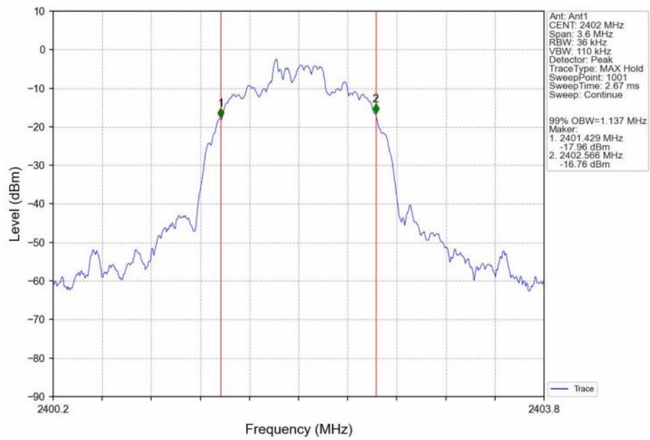
99%_Occupied_Bandwidth_NVNT_ANT1_2-DH5_2402
