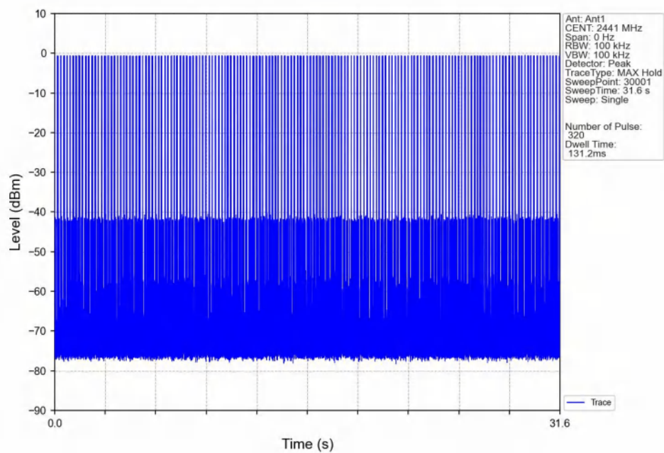
Dwell_Time_(Hopping)_NVNT_ANT1_1-DH1_2441_Accumulated
