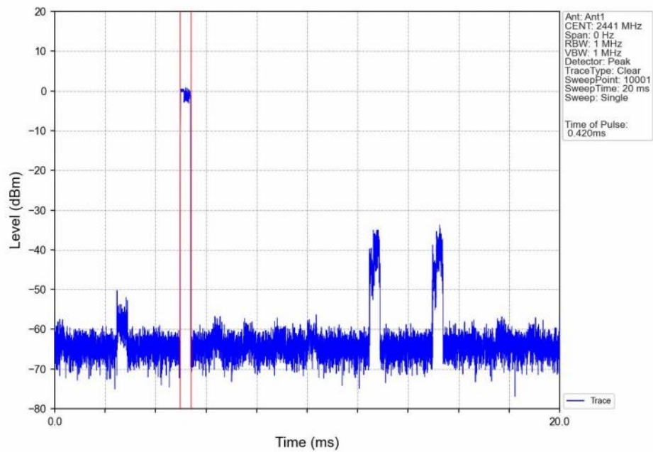
Dwell_Time_(Hopping)_NVNT_ANT1_3-DH1_2441_Accumulated
