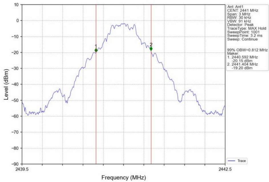
99%_Occupied_Bandwidth_NVNT_ANT1_DH5_2441
