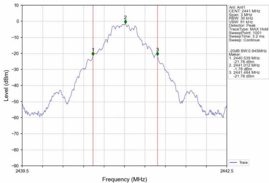
-20dB_Bandwidth_NVNT_ANT1_DH5_2441
