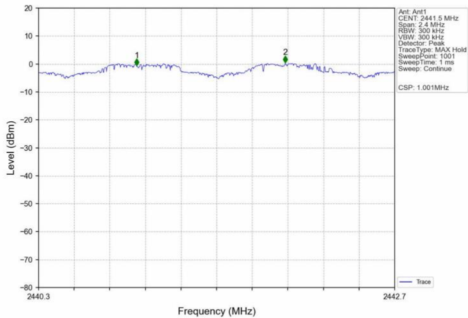
Carrier_Frequencies_Separation_(Hopping)_NVNT_ANT1_2DH5_Hopping
