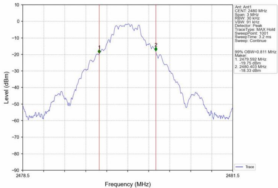
99%_Occupied_Bandwidth_NVNT_ANT1_DH5_2480
