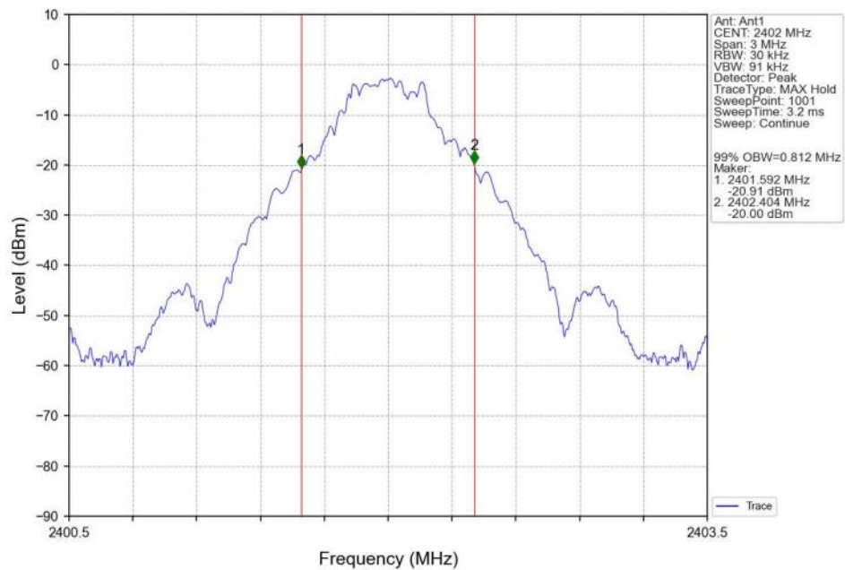
99%_Occupied_Bandwidth_NVNT_ANT1_DH5_2402
