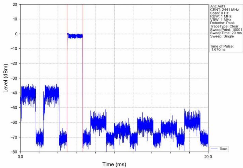
Dwell_Time_(Hopping)_NVNT_ANT1_2-DH3_2441_Accumulated
