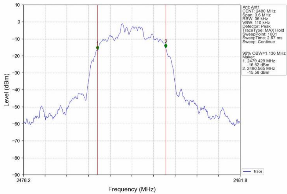
99%_Occupied_Bandwidth_NVNT_ANT1_2-DH5_2480
