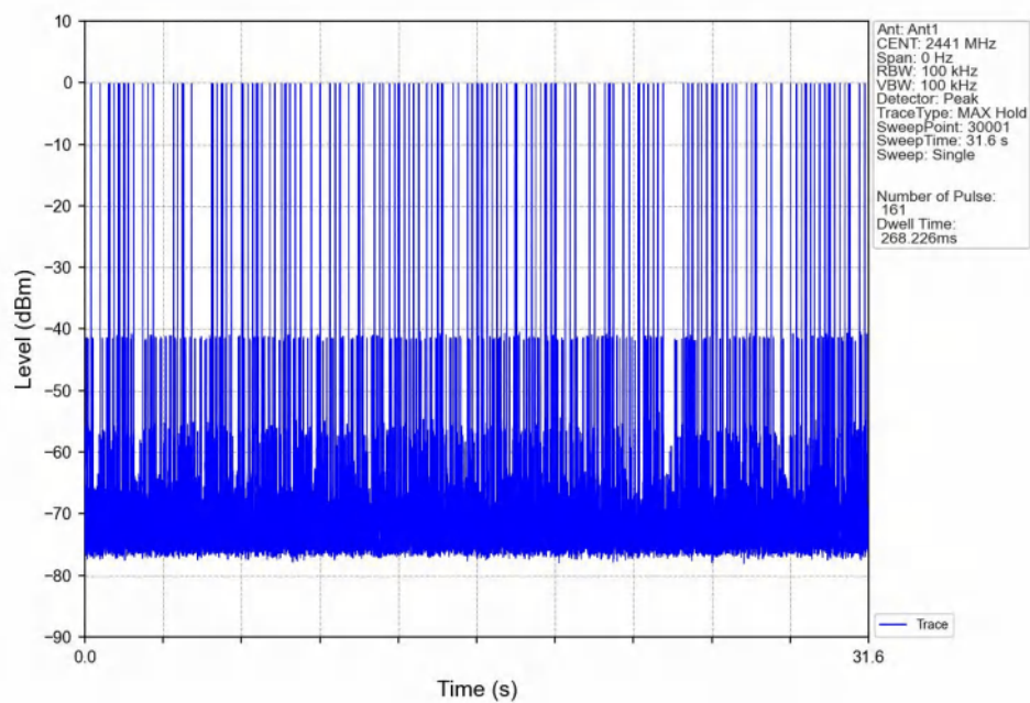
Dwell_Time_(Hopping)_NVNT_ANT1_DH3_2441_Accumulated
