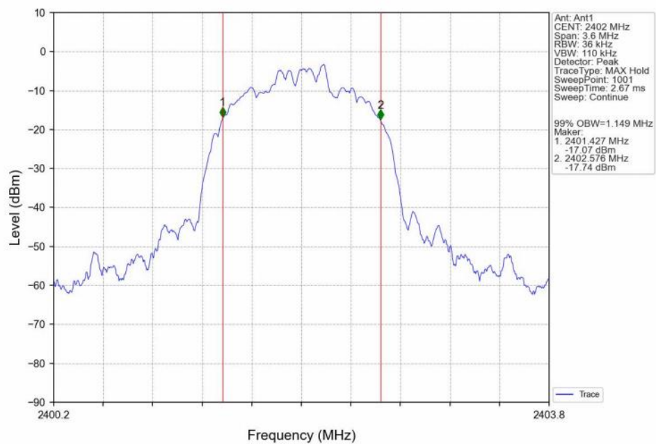
99%_Occupied_Bandwidth_NVNT_ANT1_3-DH5_2402
