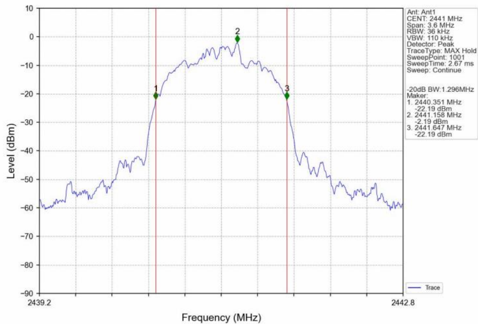
-20dB_Bandwidth_NVNT_ANT1_3-DH5_2441
