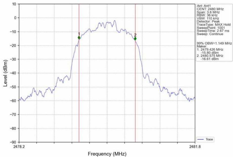
99%_Occupied_Bandwidth_NVNT_ANT1_3-DH5_2480
