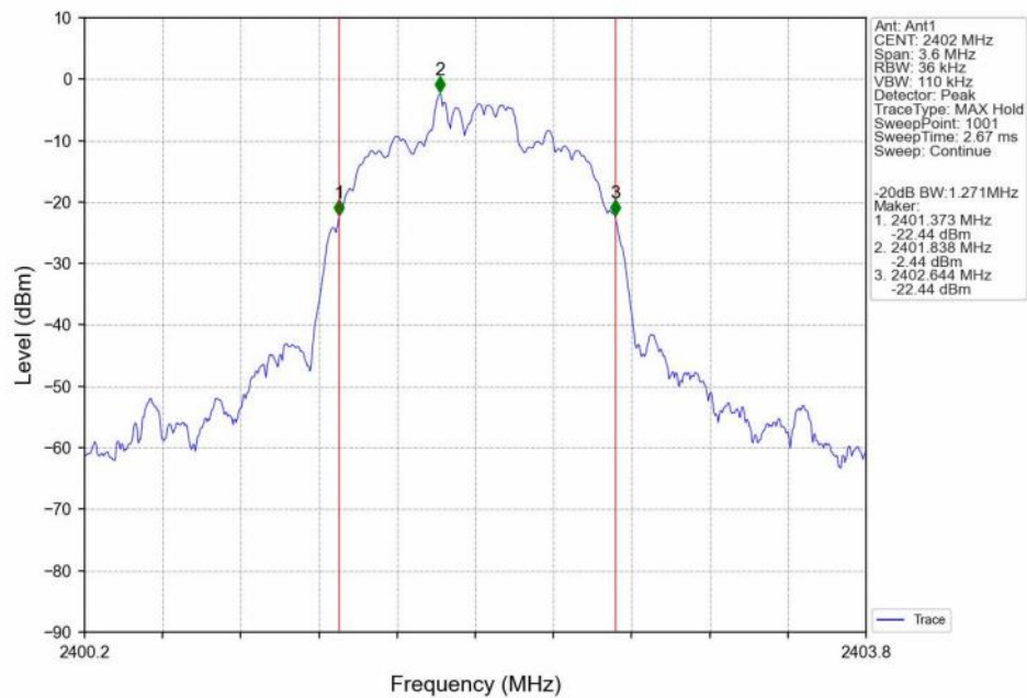
-20dB_Bandwidth_NVNT_ANT1_2-DH5_2402
