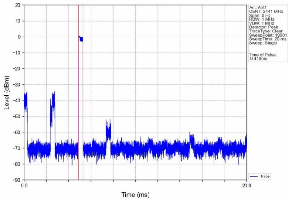
Dwell_Time_(Hopping)_NVNT_ANT1_2-DH1_2441_Accumulated
