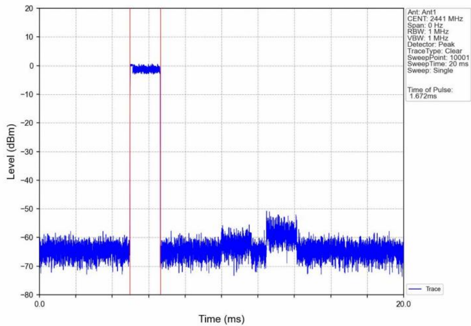
Dwell_Time_(Hopping)_NVNT_ANT1_3-DH3_2441_Accumulated
