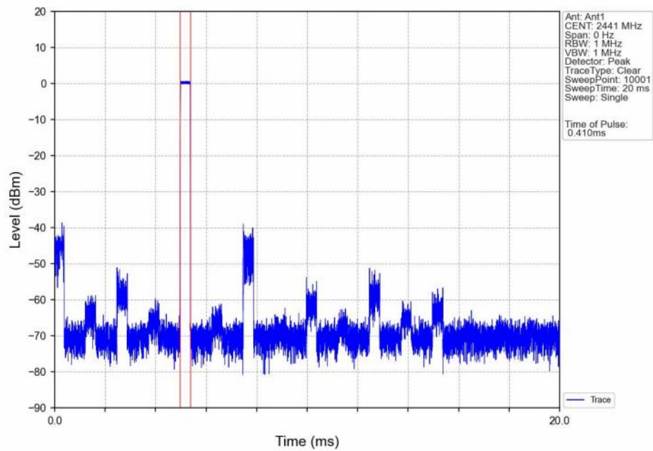
Dwell_Time_(Hopping)_NVNT_ANT1_1-DH1_2441_Accumulated
