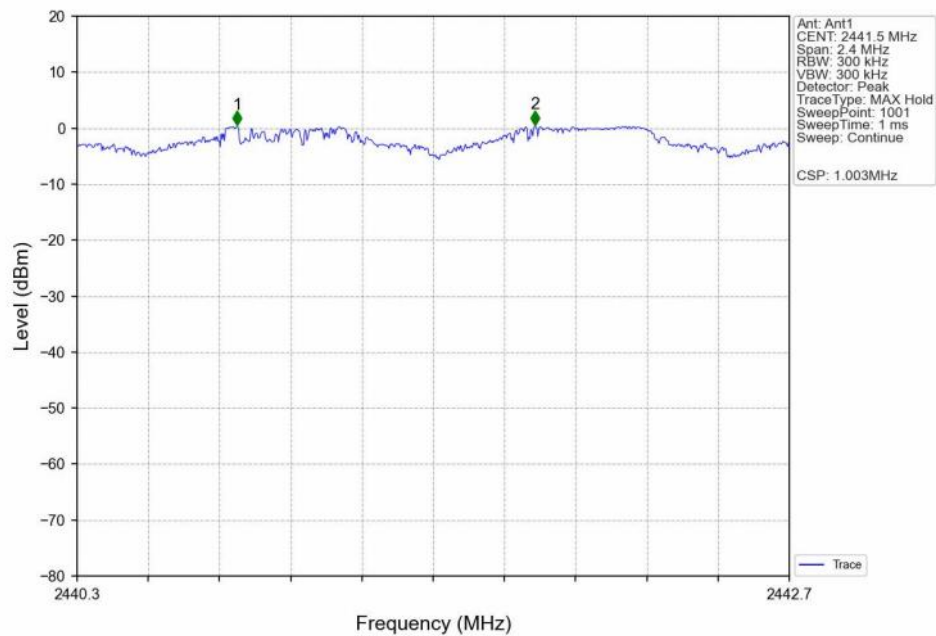
Carrier_Frequencies_Separation_(Hopping)_NVNT_ANT1_3DH5_Hopping
