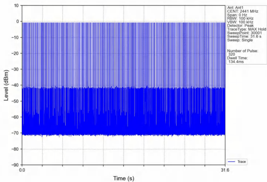
Dwell_Time_(Hopping)_NVNT_ANT1_3-DH1_2441_Accumulated
