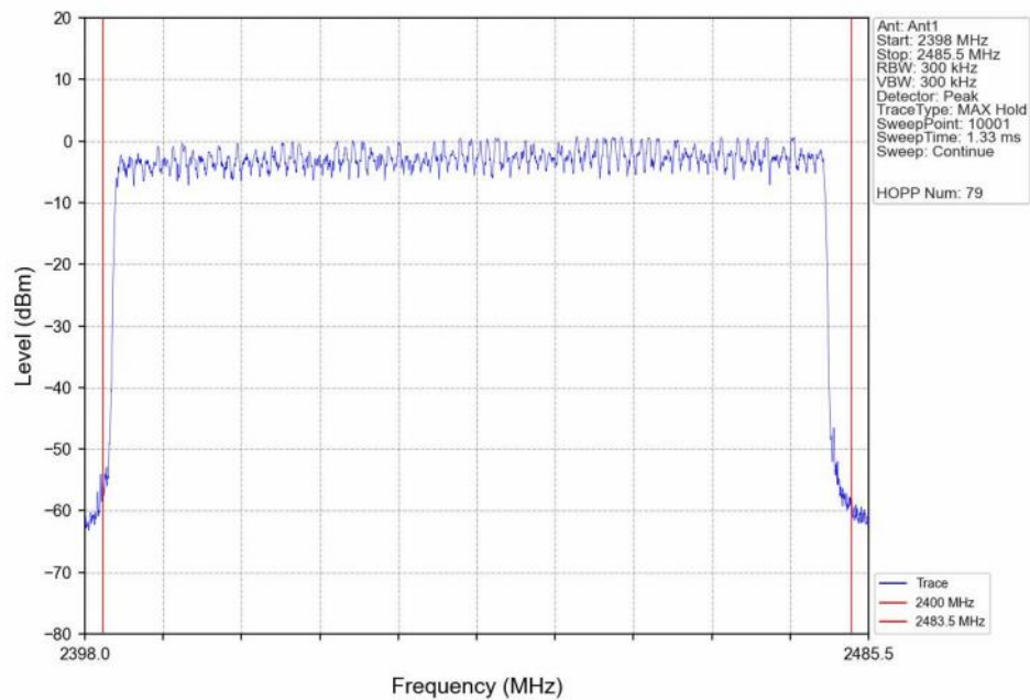
Number_of_Hopping_Channel_(Hopping)_NVNT_ANT1_3DH5_Hopping
