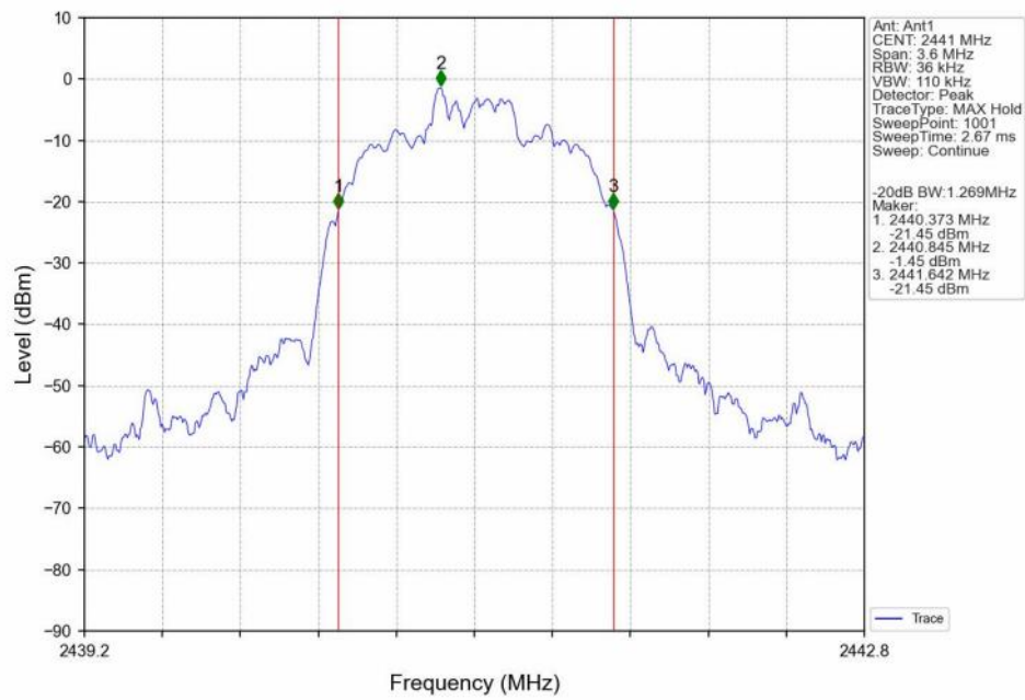
-20dB_Bandwidth_NVNT_ANT1_2-DH5_2441
