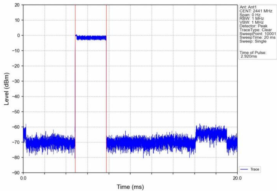
Dwell_Time_(Hopping)_NVNT_ANT1_2-DH5_2441_Accumulated
