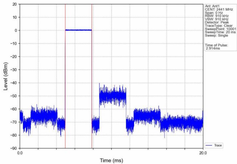
Dwell_Time_(Hopping)_NVNT_ANT1_DH5_2441_Accumulated
