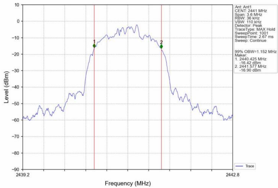
99%_Occupied_Bandwidth_NVNT_ANT1_3-DH5_2441
