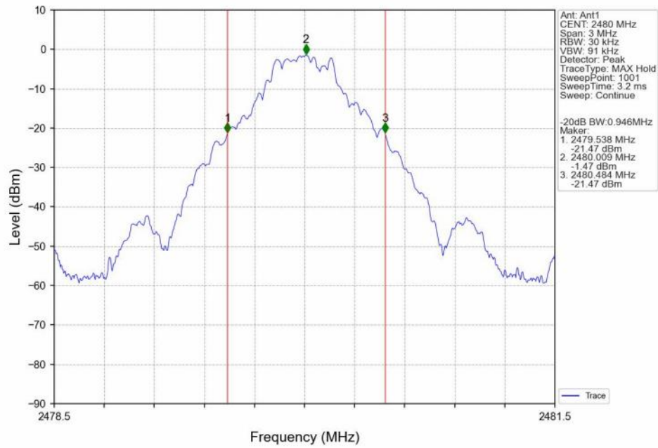
-20dB_Bandwidth_NVNT_ANT1_DH5_2480
