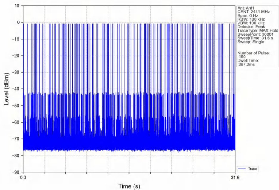
Dwell_Time_(Hopping)_NVNT_ANT1_2-DH3_2441_Accumulated
