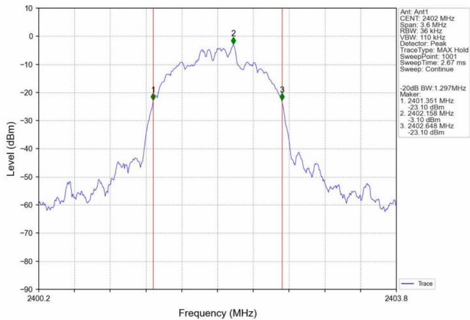
-20dB_Bandwidth_NVNT_ANT1_3-DH5_2402
