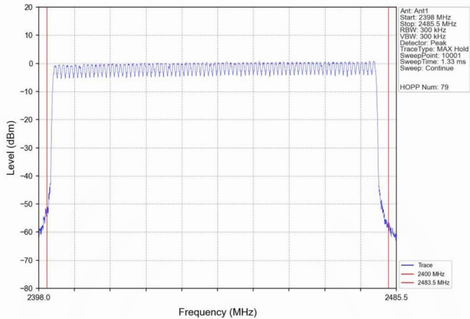
Number_of_Hopping_Channel_(Hopping)_NVNT_ANT1_2DH5_Hopping
