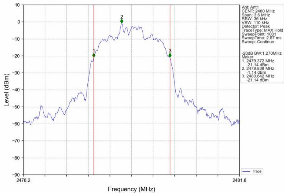
-20dB_Bandwidth_NVNT_ANT1_2-DH5_2480
