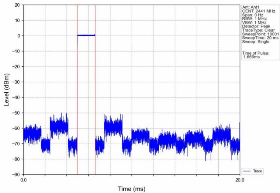
Dwell_Time_(Hopping)_NVNT_ANT1_DH3_2441_Accumulated
