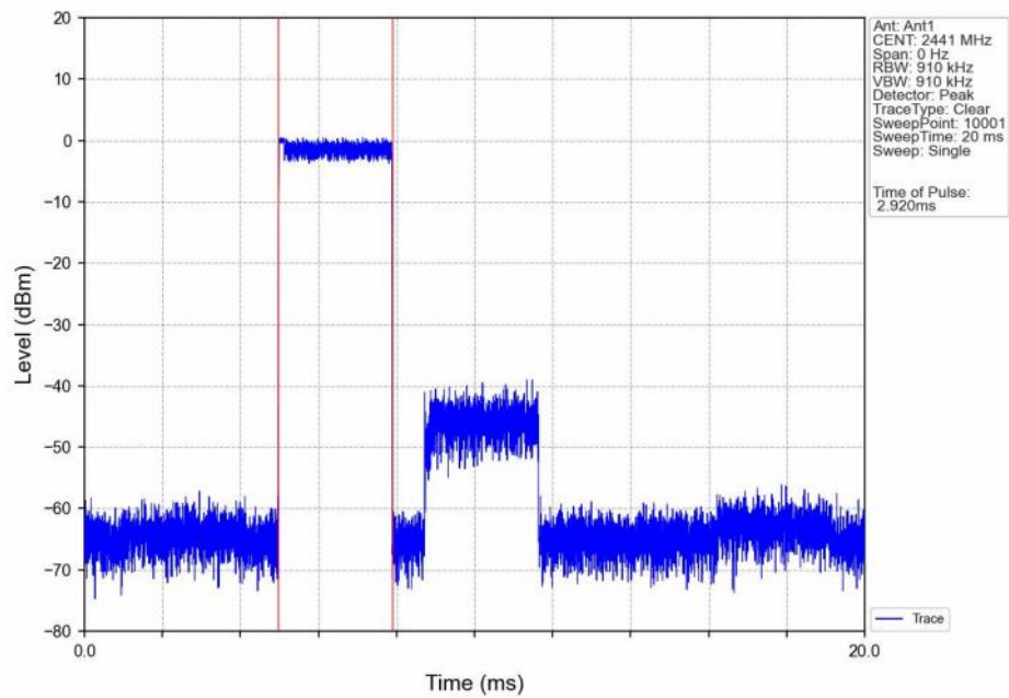
Dwell_Time_(Hopping)_NVNT_ANT1_3-DH5_2441_Accumulated
