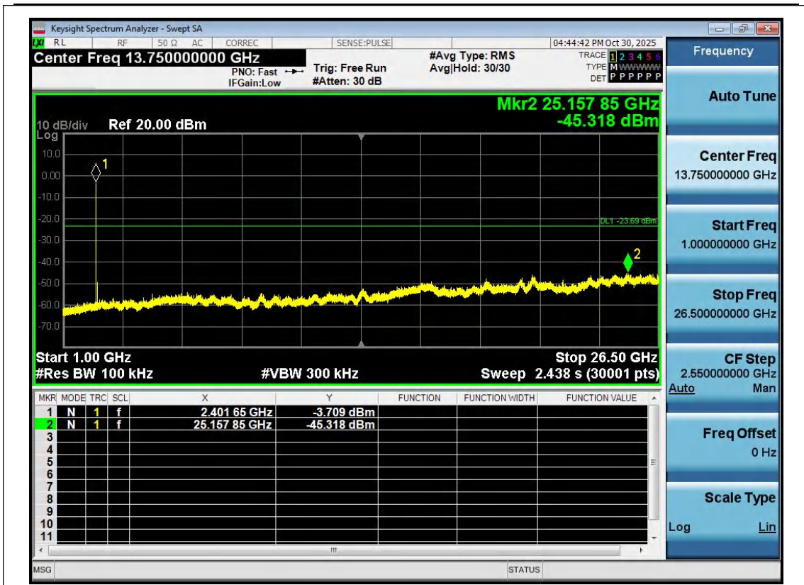
BLE_1M-Ant1-2402-1000~26500-PASS
