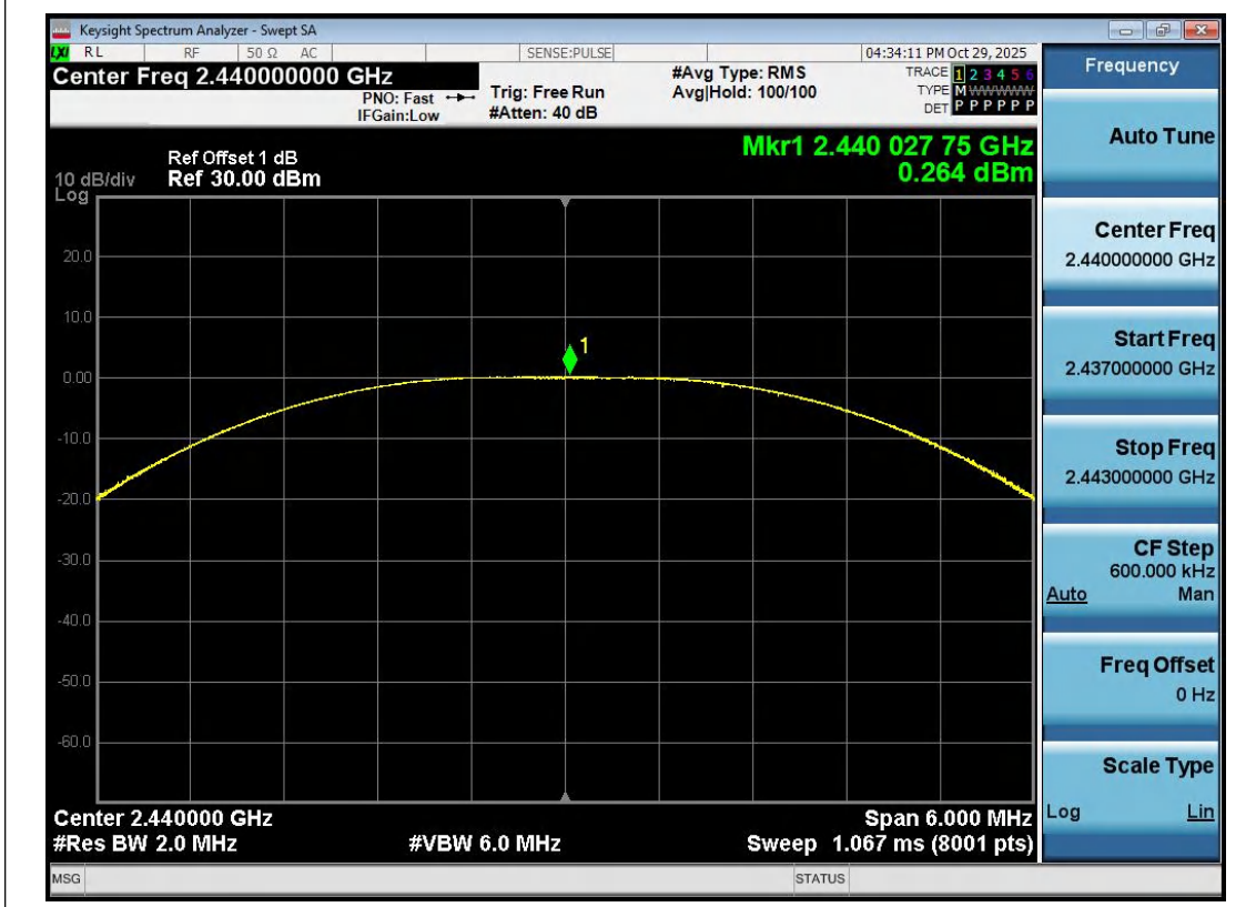
BLE_2M-Ant1-2440-PASS
