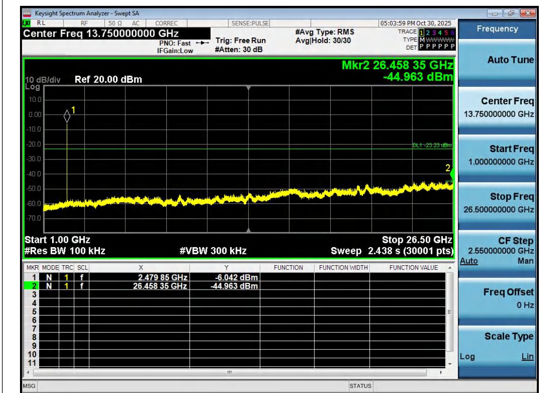
BLE_2M-Ant1-2480-1000~26500-PASS
