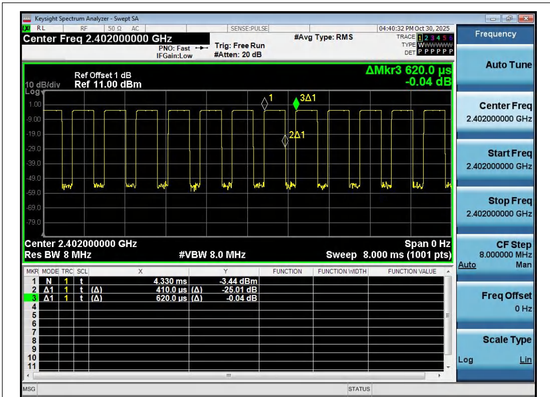
NTNV-BLE_1M-Ant1-2402
