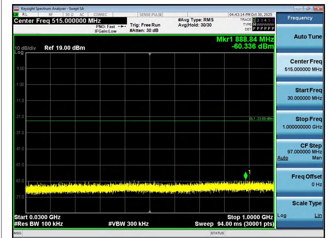
BLE_1M-Ant1-2402-30~1000-PASS
