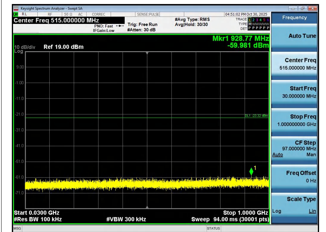
BLE_1M-Ant1-2480-30~1000-PASS
