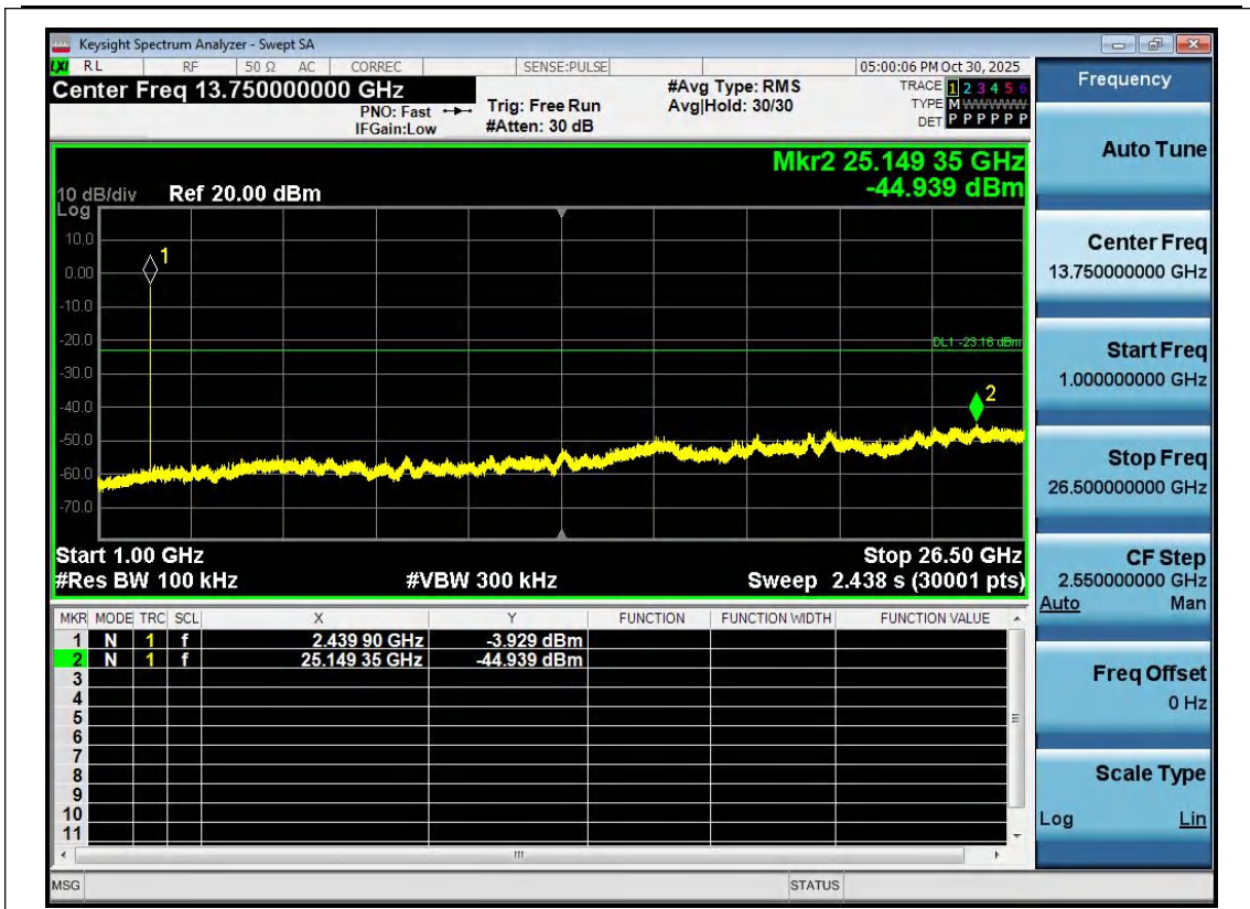
BLE_2M-Ant1-2440-1000~26500-PASS
