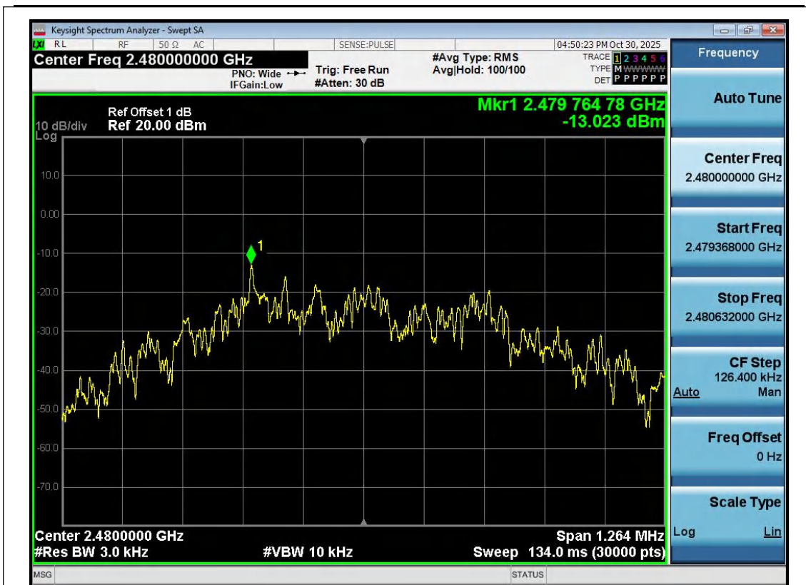
BLE_1M-Ant1-2480-PASS
