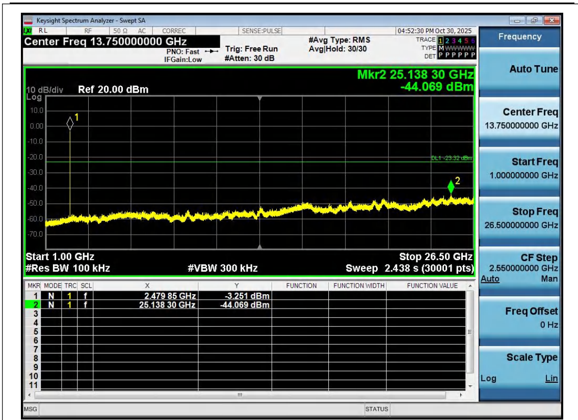
BLE_1M-Ant1-2480-1000~26500-PASS
