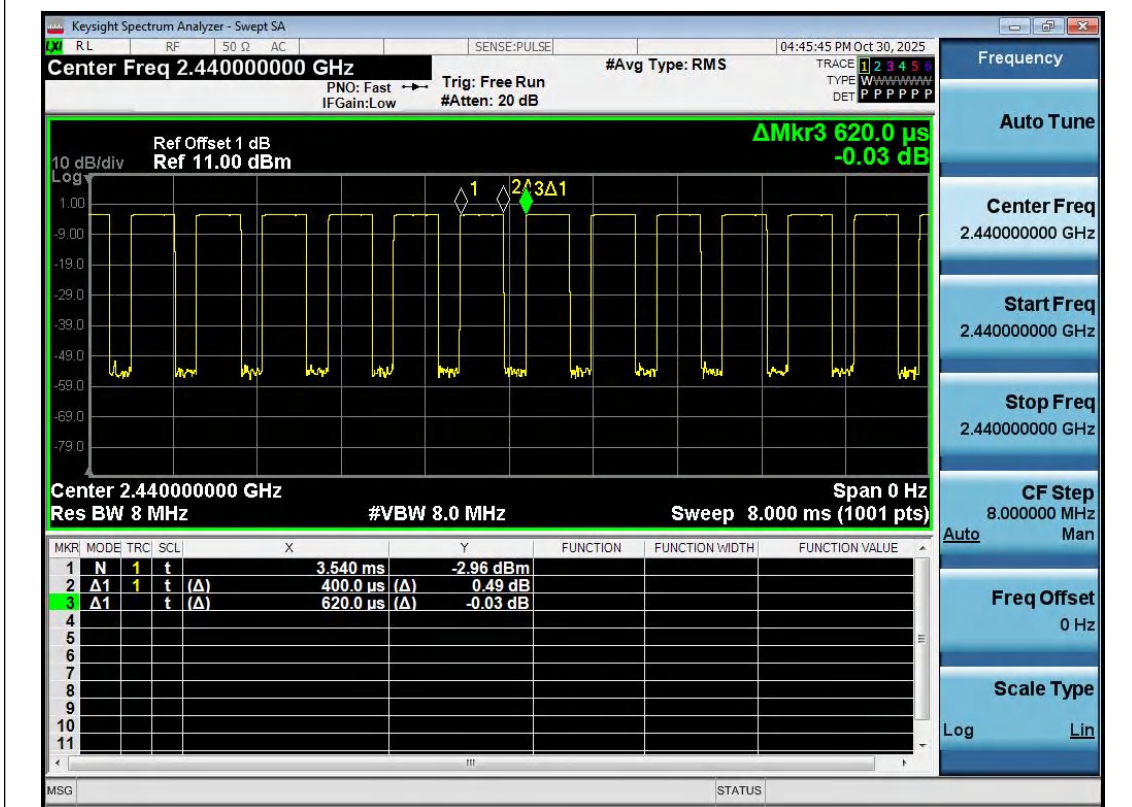
NTNV-BLE_1M-Ant1-2440
