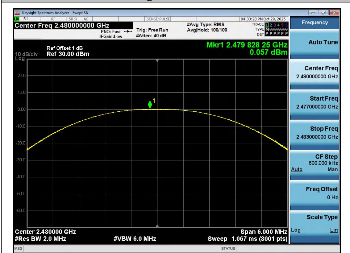
BLE_1M-Ant1-2480-PASS
