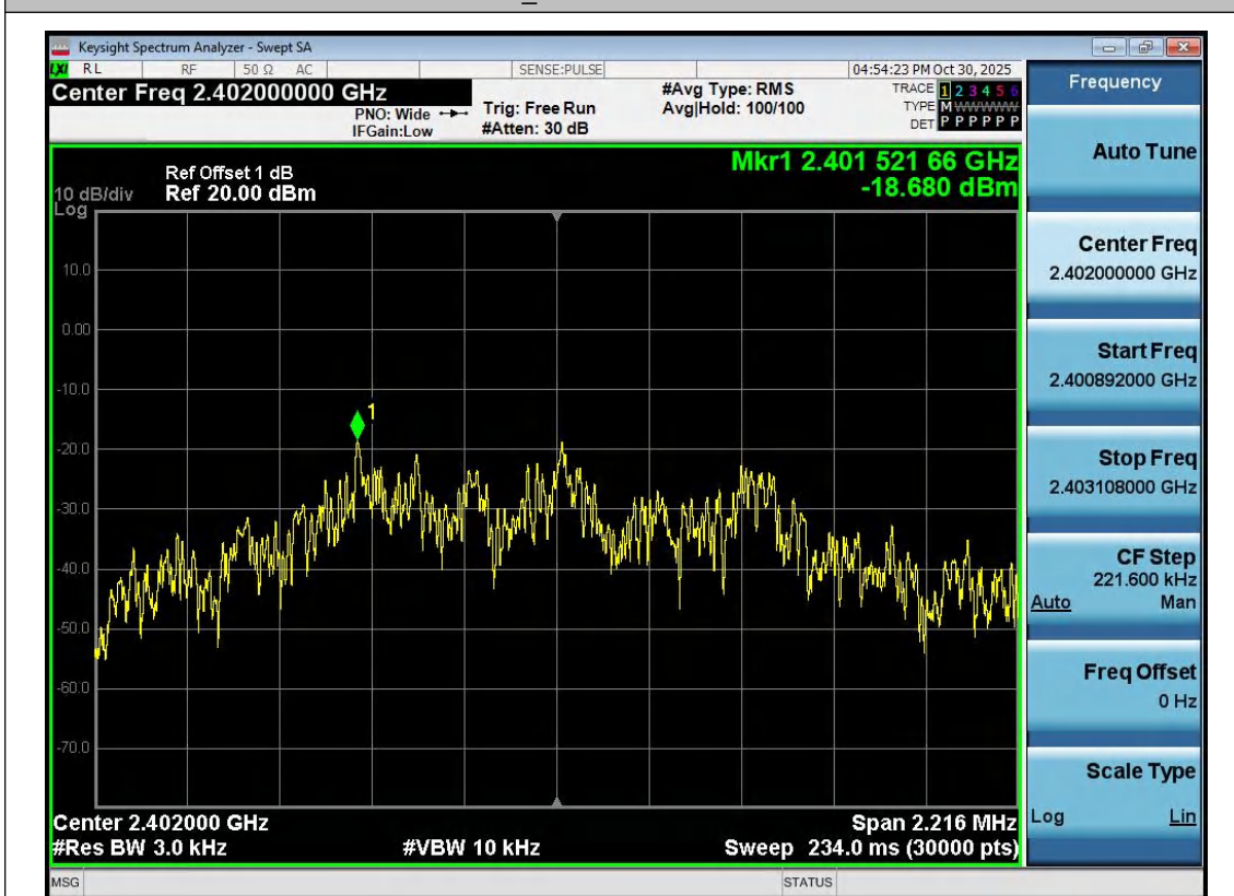
BLE_2M-Ant1-2402-PASS
