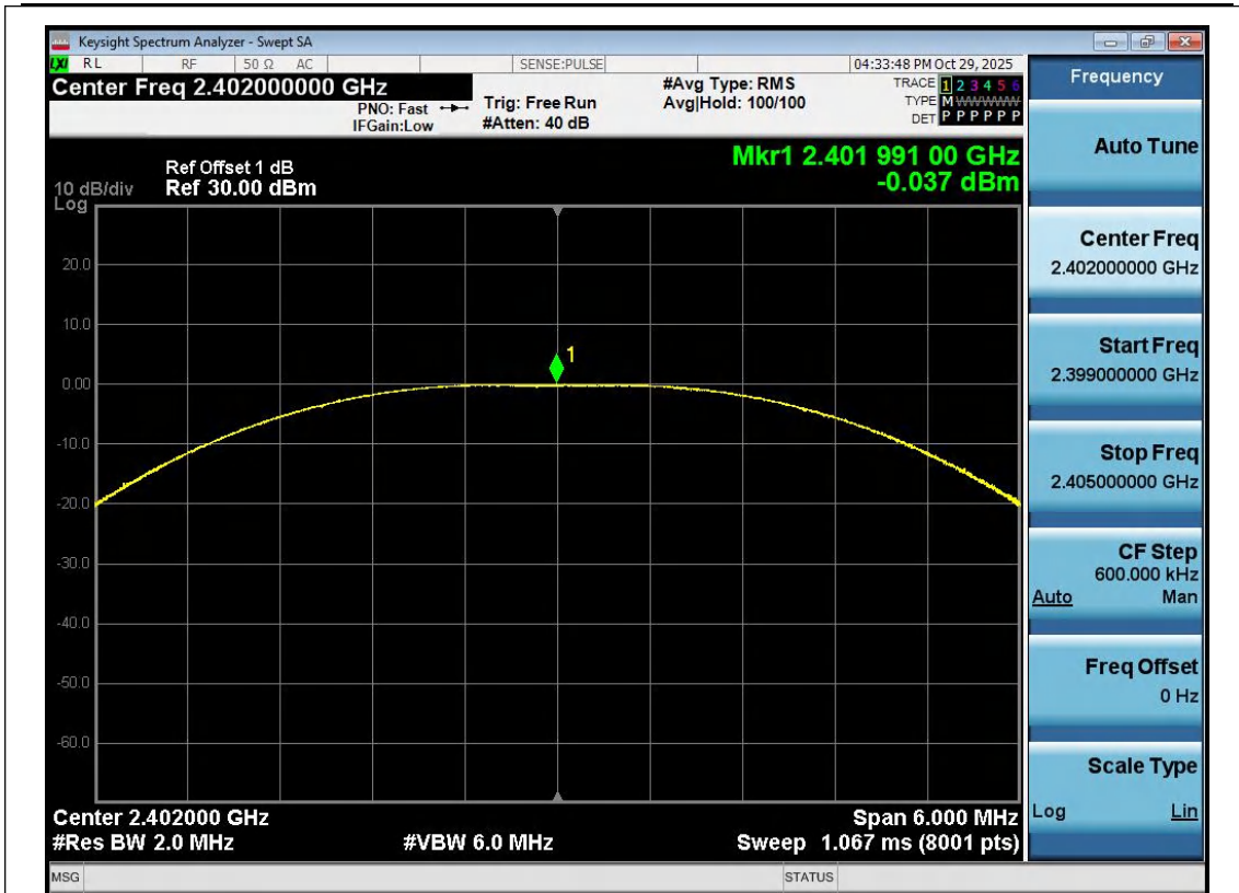
BLE_2M-Ant1-2402-PASS
