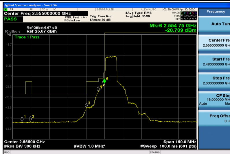
Band41-15MHz-QPSK-40315-1RB#0
