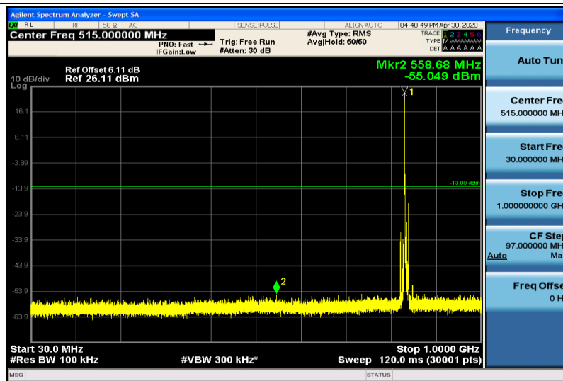
Band5-5MHz-16QAM-20525-1RB#0-30~1000MHz
