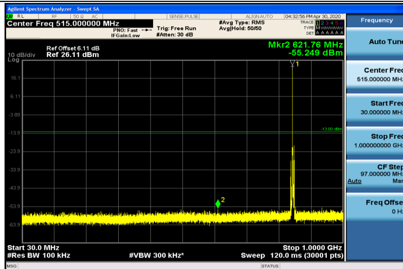
Band5-3MHz-16QAM-20635-1RB#0-30~1000MHz
