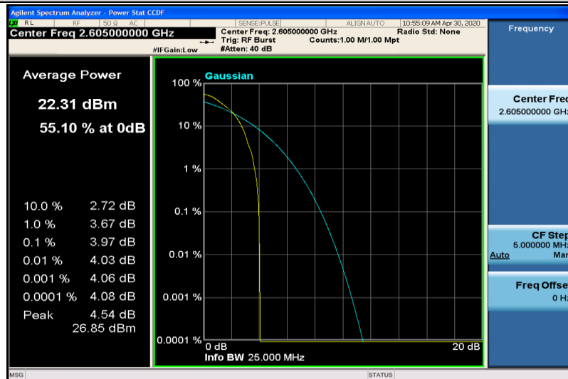
Band41-10MHz-QPSK-40740-1RB#0
