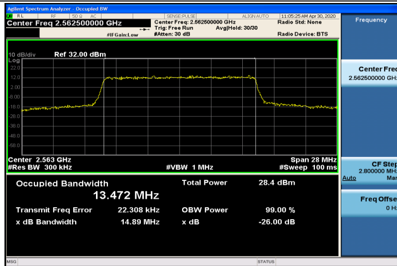
Band41-15MHz-QPSK-40315-75RB#0-13.472
