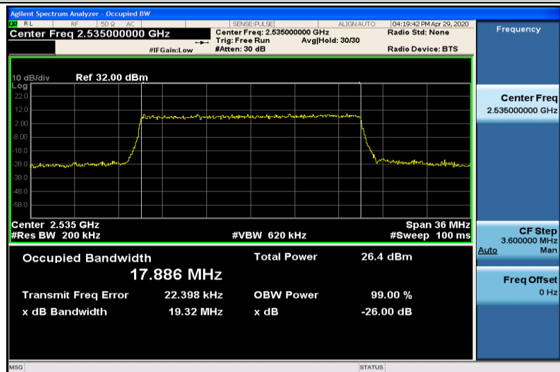
Band7-20MHz-16QAM-21100-100RB#0-17.886
