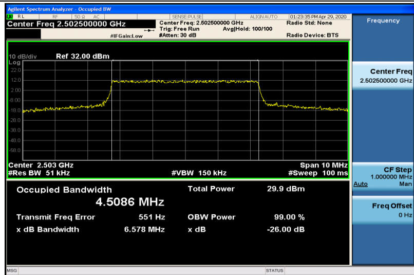
Band7-5MHz-QPSK-20775-25RB#0-4.5086
