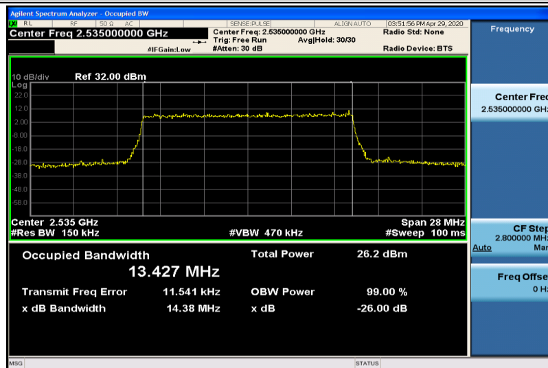
Band7-15MHz-16QAM-21100-75RB#0-13.427
