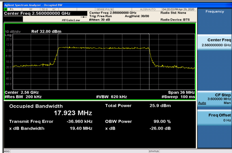
Band7-20MHz-16QAM-21350-100RB#0-17.923
