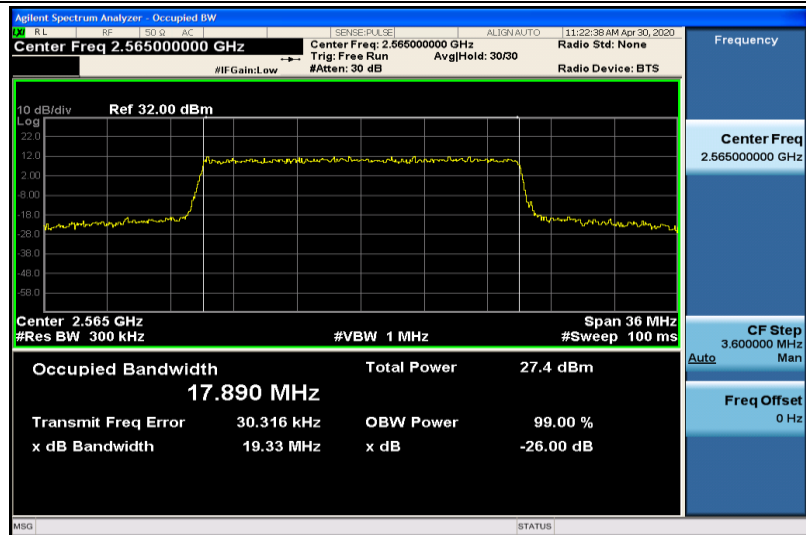
Band41-20MHz-16QAM-40340-100RB#0-17.890
