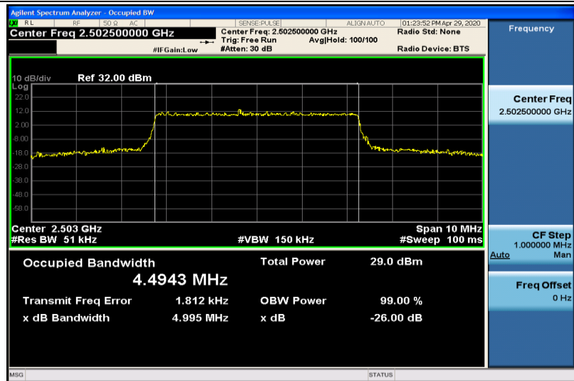
Band7-5MHz-16QAM-20775-25RB#0-4.4943
