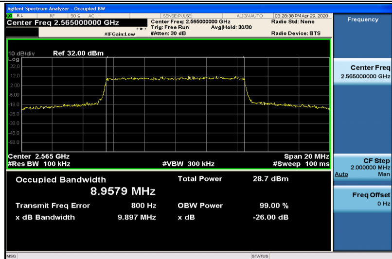
Band7-10MHz-QPSK-21400-50RB#0-8.9579
