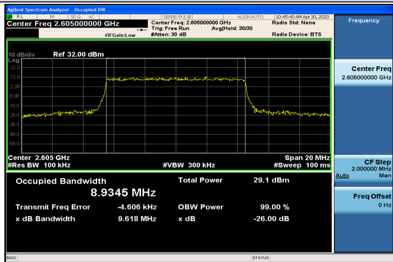
Band41-10MHz-16QAM-40740-50RB#0-8.9345
