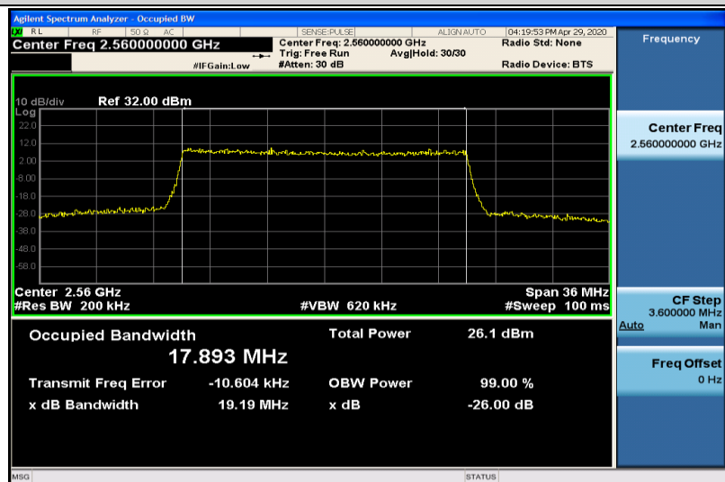
Band7-20MHz-QPSK-21350-100RB#0-17.893
