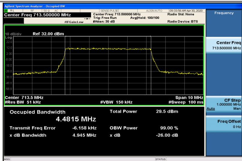
Band17-5MHz-QPSK-23825-25RB#0-4.4815
