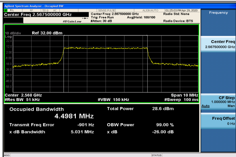
Band7-5MHz-16QAM-21425-25RB#0-4.4981
