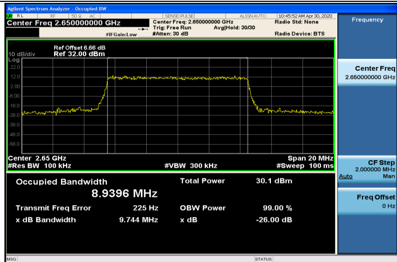
Band41-10MHz-QPSK-41190-50RB#0-8.9396
