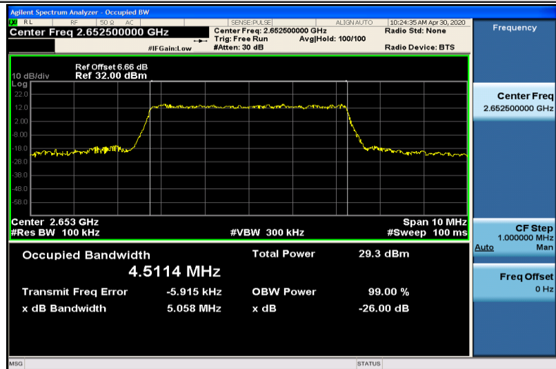
Band41-5MHz-16QAM-41215-25RB#0-4.5114
