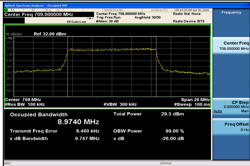
Band17-10MHz-QPSK-23780-50RB#0-8.9740
