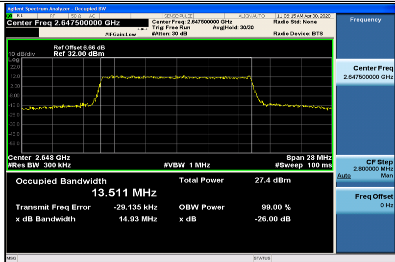
Band41-15MHz-16QAM-41165-75RB#0-13.511
