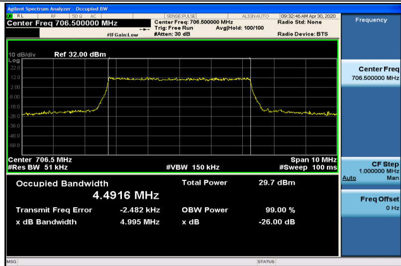
Band17-5MHz-QPSK-23755-25RB#0-4.4916
