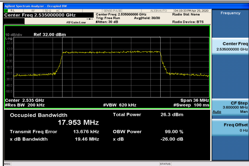
Band7-20MHz-QPSK-21100-100RB#0-17.953
