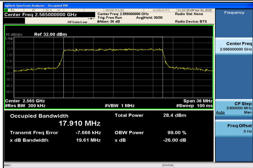
Band41-20MHz-QPSK-40340-100RB#0-17.910
