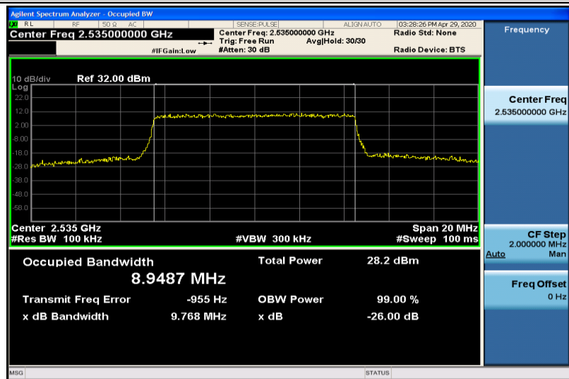
Band7-10MHz-16QAM-21100-50RB#0-8.9487
