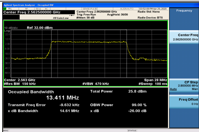
Band7-15MHz-QPSK-21375-75RB#0-13.411
