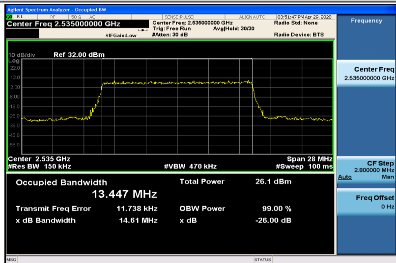
Band7-15MHz-QPSK-21100-75RB#0-13.447
