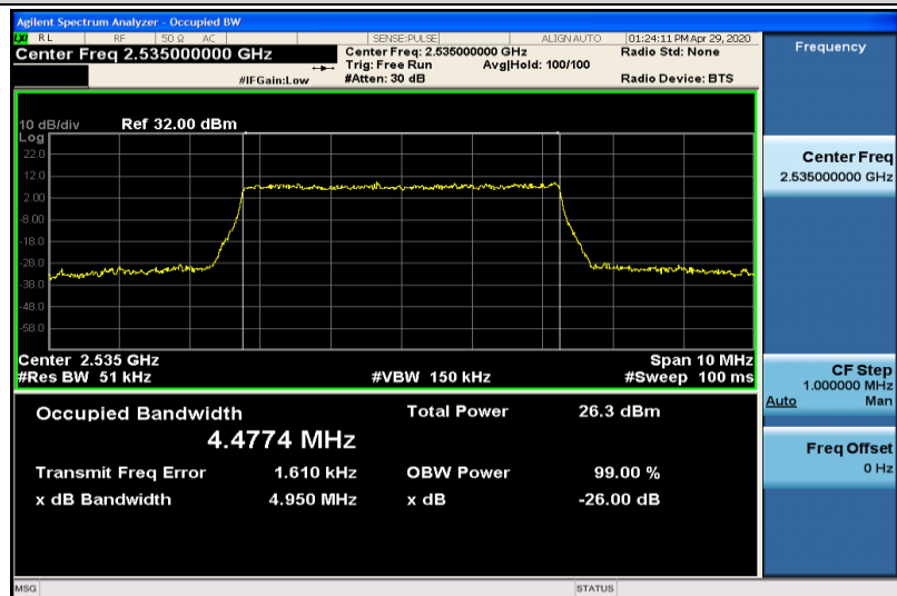
Band7-5MHz-QPSK-21100-25RB#0-4.4774
