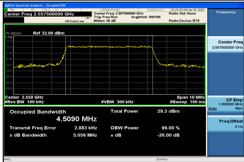
Band41-5MHz-16QAM-40265-25RB#0-4.5090
