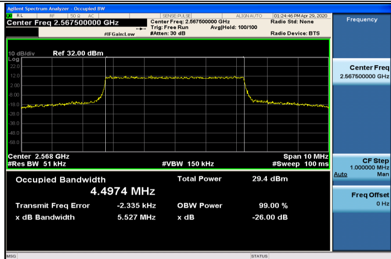
Band7-5MHz-QPSK-21425-25RB#0-4.4974
