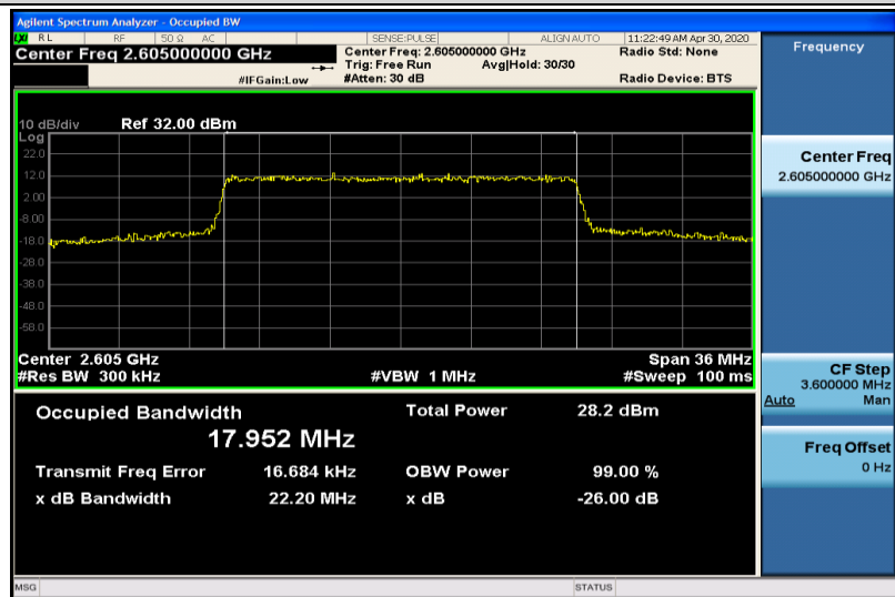
Band41-20MHz-QPSK-40740-100RB#0-17.952
