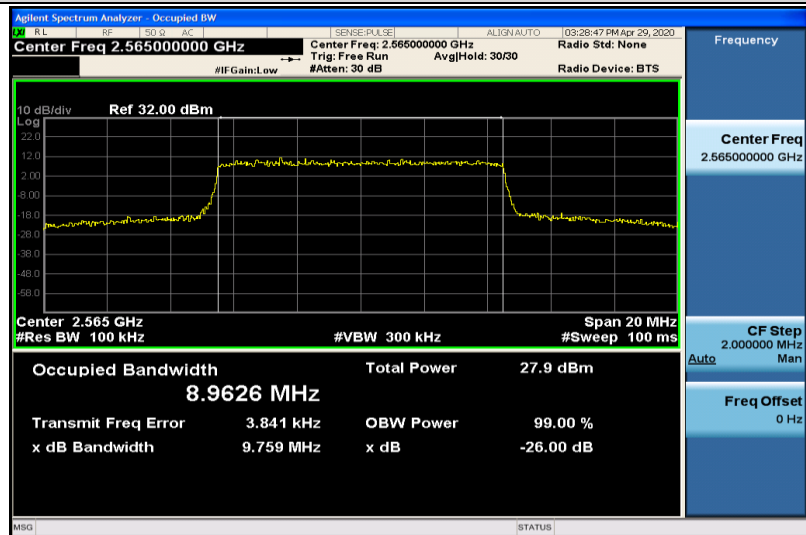
Band7-10MHz-16QAM-21400-50RB#0-8.9626
