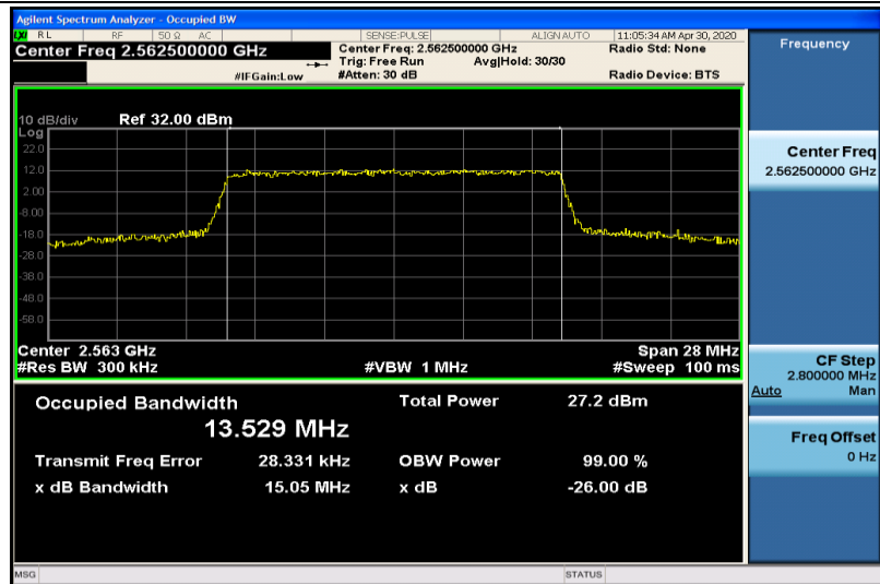
Band41-15MHz-16QAM-40315-75RB#0-13.529
