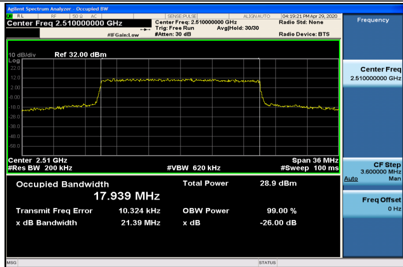
Band7-20MHz-16QAM-20850-100RB#0-17.939
