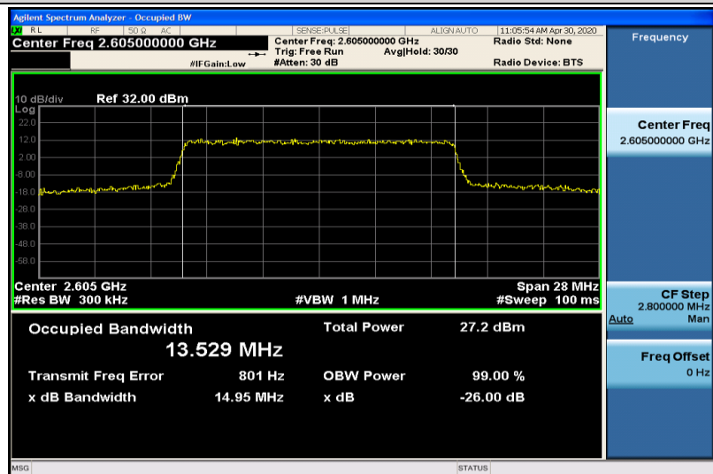
Band41-15MHz-16QAM-40740-75RB#0-13.529
