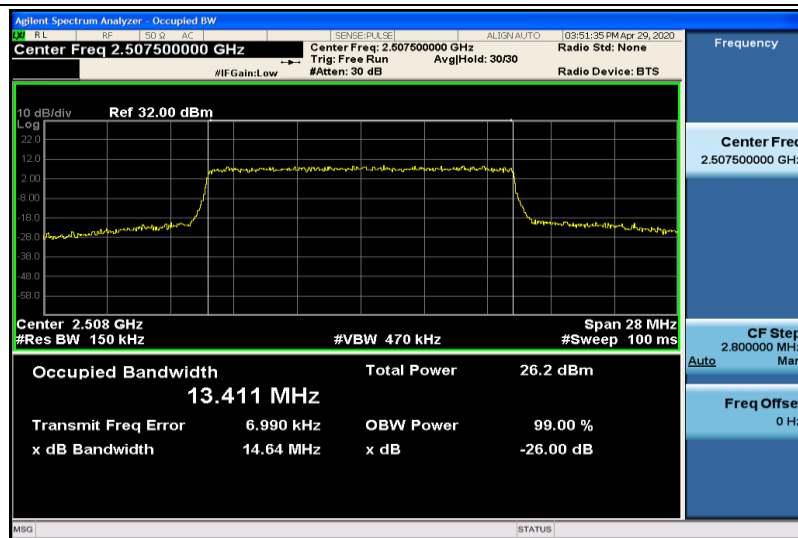
Band7-15MHz-16QAM-20825-75RB#0-13.411
