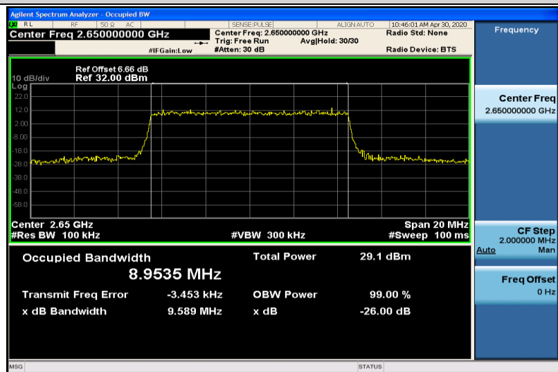
Band41-10MHz-16QAM-41190-50RB#0-8.9535
