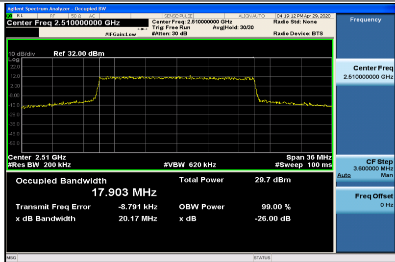
Band7-20MHz-QPSK-20850-100RB#0-17.903
