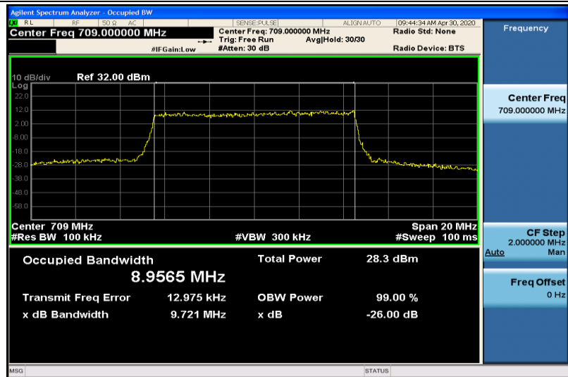
Band17-10MHz-16QAM-23780-50RB#0-8.9565
