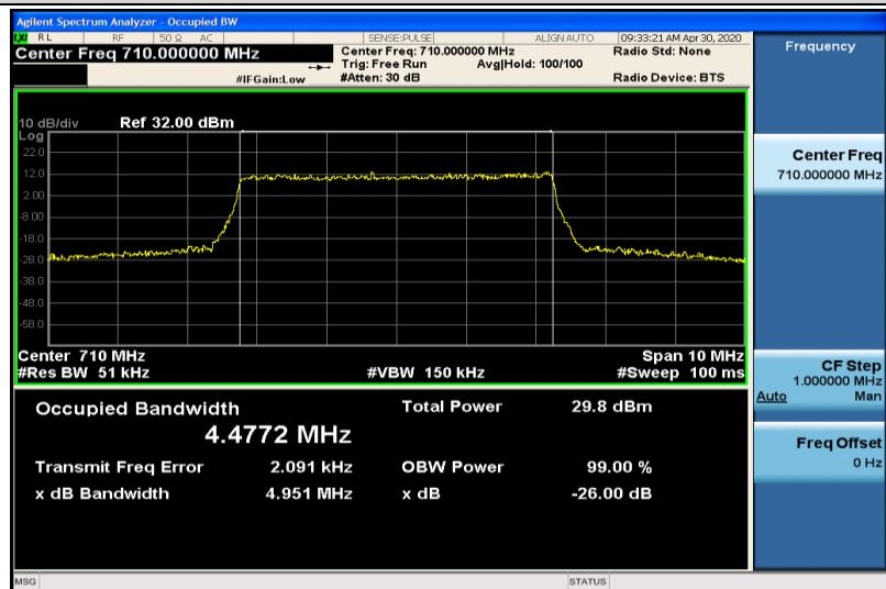
Band17-5MHz-QPSK-23790-25RB#0-4.4772
