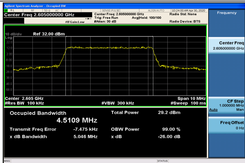
Band41-5MHz-16QAM-40740-25RB#0-4.5109
