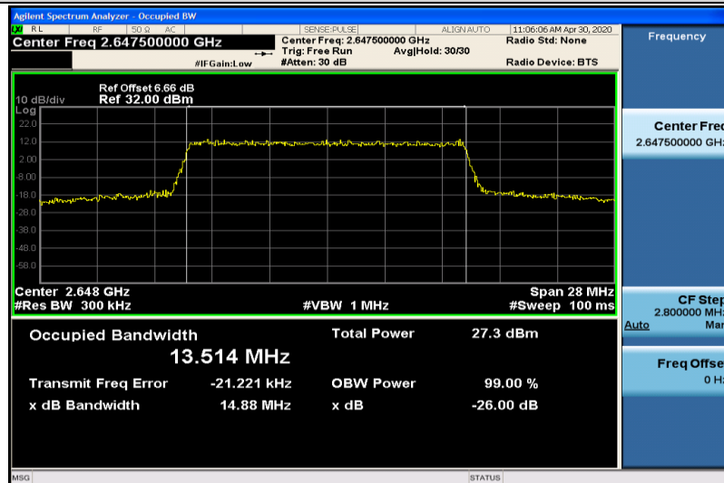
Band41-15MHz-QPSK-41165-75RB#0-13.514
