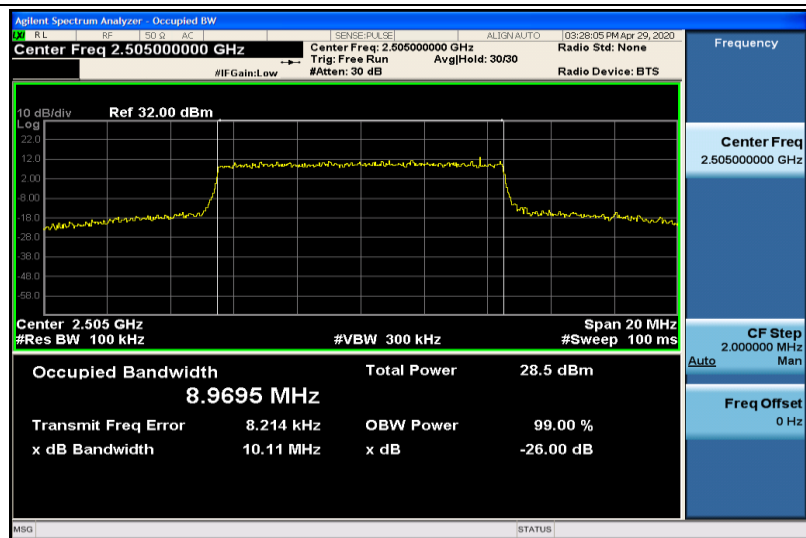
Band7-10MHz-16QAM-20800-50RB#0-8.9695
