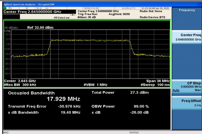
Band41-20MHz-16QAM-41140-100RB#0-17.929
