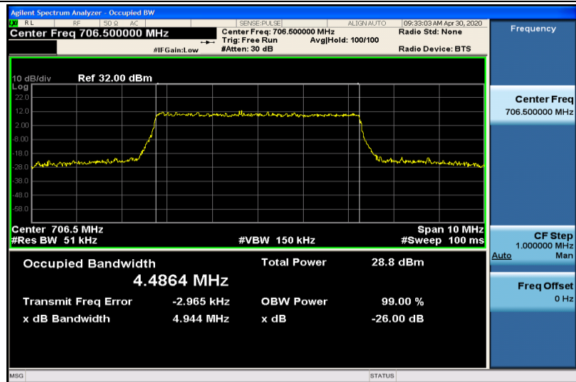
Band17-5MHz-16QAM-23755-25RB#0-4.4864
