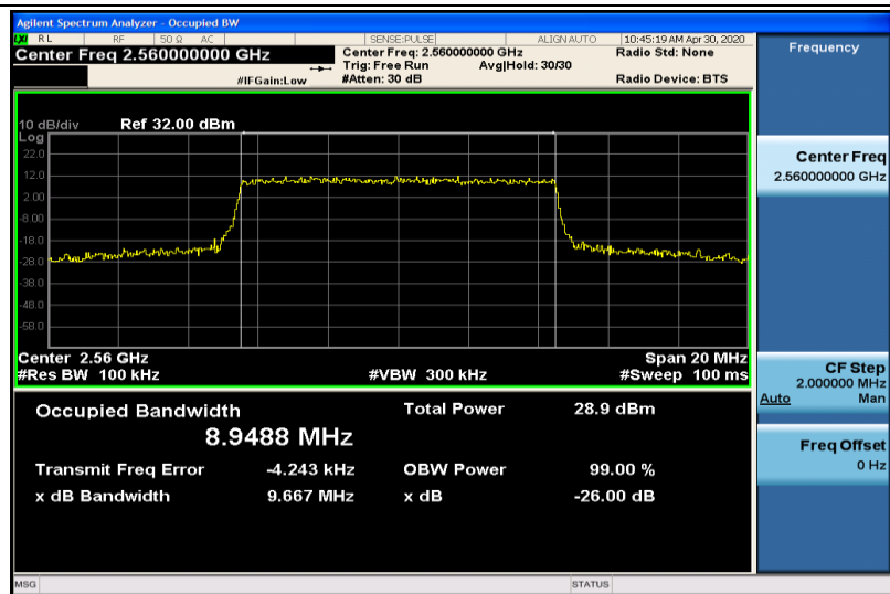
Band41-10MHz-16QAM-40290-50RB#0-8.9488
