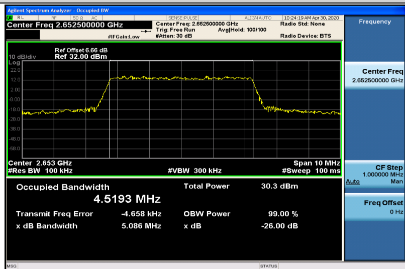
Band41-5MHz-QPSK-41215-25RB#0-4.5193
