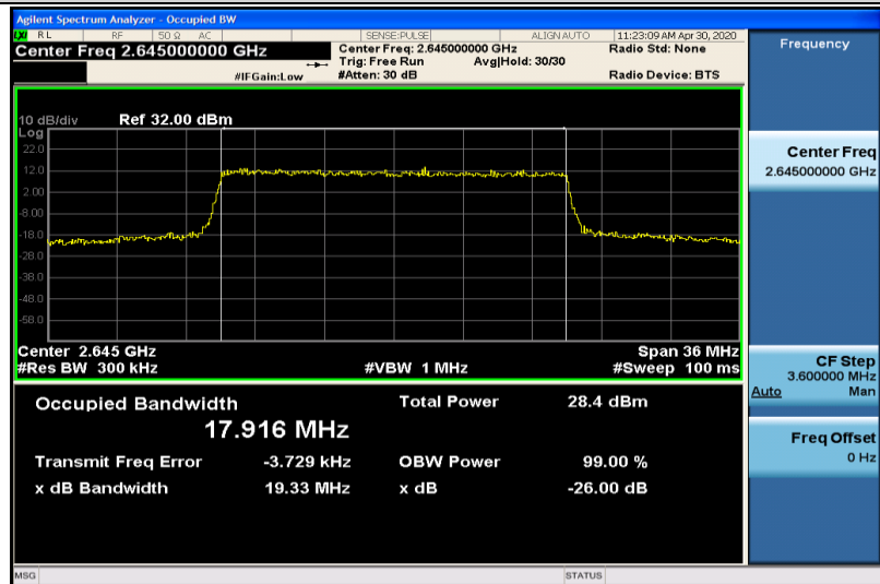
Band41-20MHz-QPSK-41140-100RB#0-17.916
