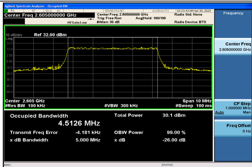
Band41-5MHz-QPSK-40740-25RB#0-4.5126
