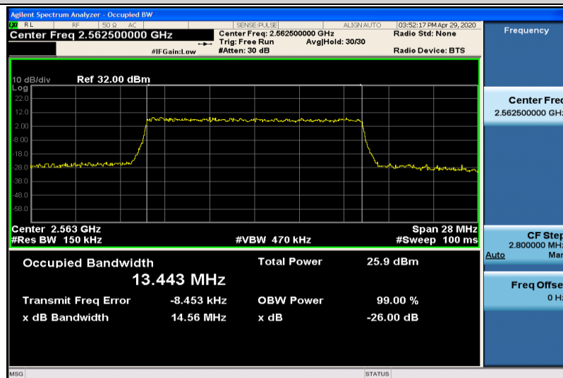
Band7-15MHz-16QAM-21375-75RB#0-13.443
