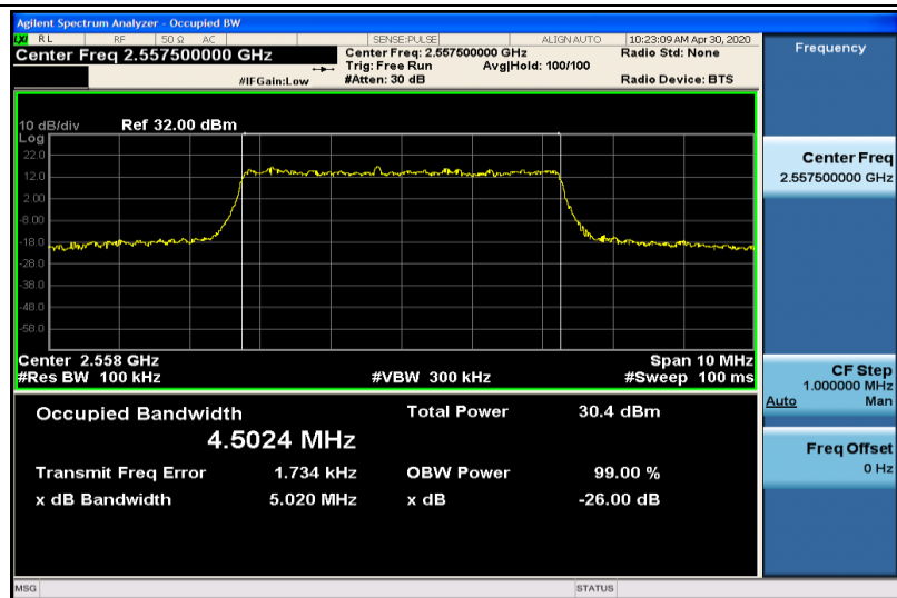
Band41-5MHz-QPSK-40265-25RB#0-4.5024
