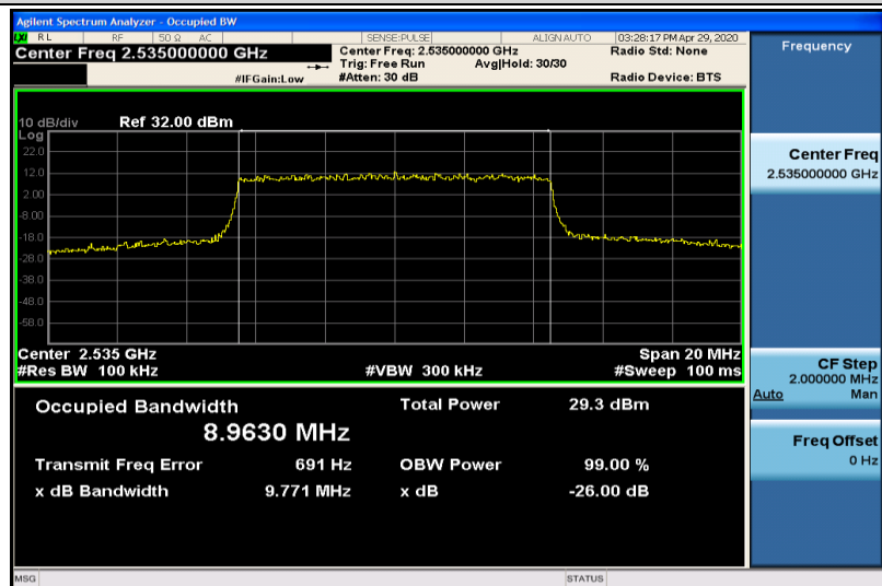
Band7-10MHz-QPSK-21100-50RB#0-8.9630
