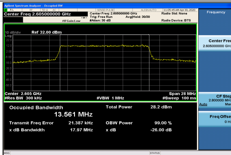
Band41-15MHz-QPSK-40740-75RB#0-13.561
