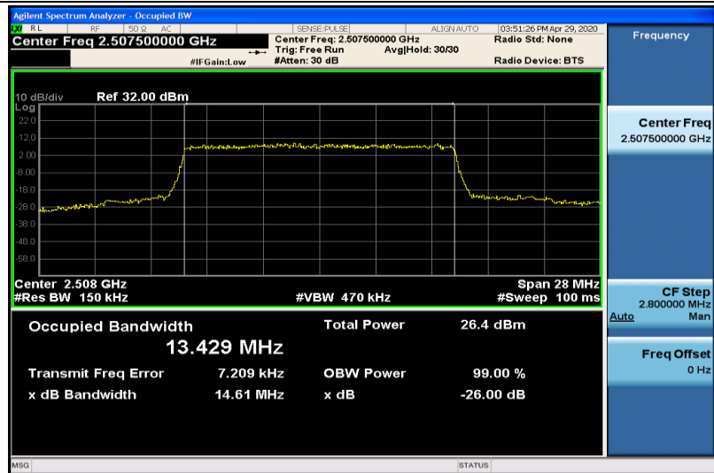
Band7-15MHz-QPSK-20825-75RB#0-13.429
