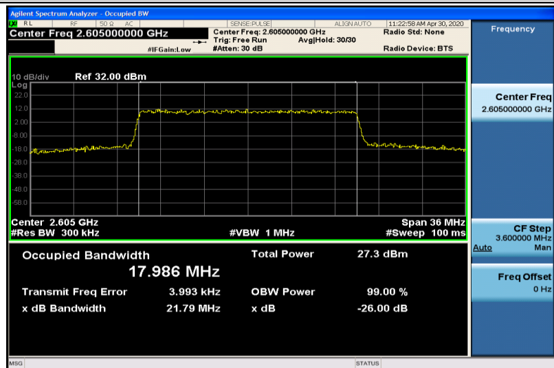
Band41-20MHz-16QAM-40740-100RB#0-17.986
