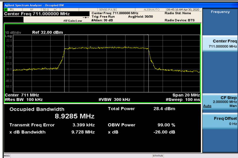
Band17-10MHz-16QAM-23800-50RB#0-8.9285
