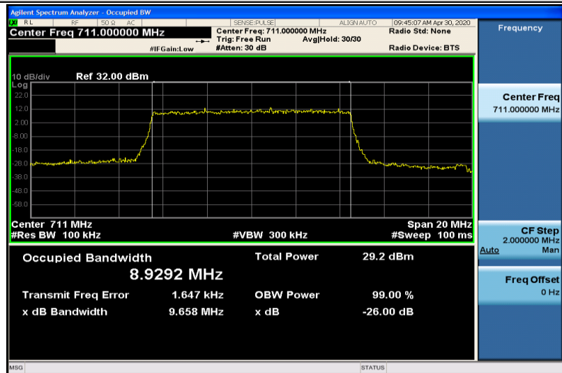
Band17-10MHz-QPSK-23800-50RB#0-8.9292
