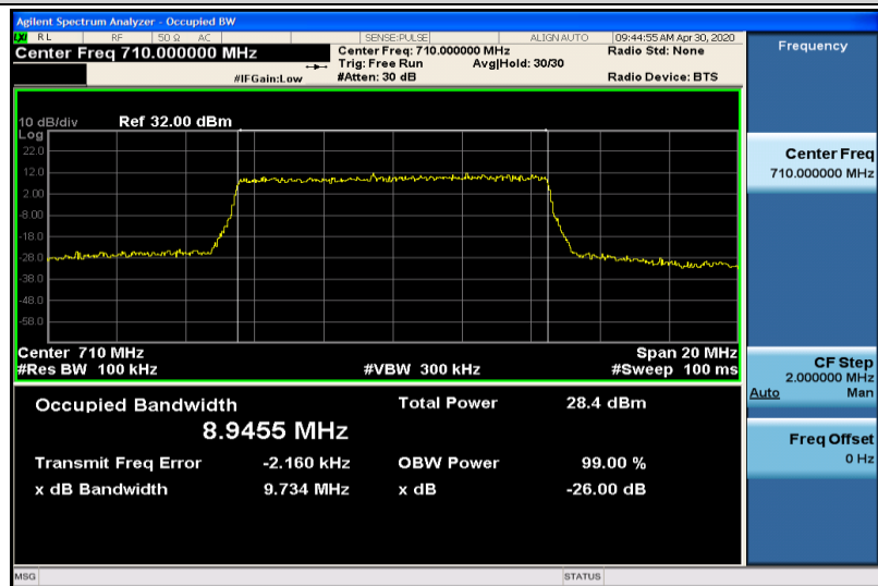
Band17-10MHz-16QAM-23790-50RB#0-8.9455
