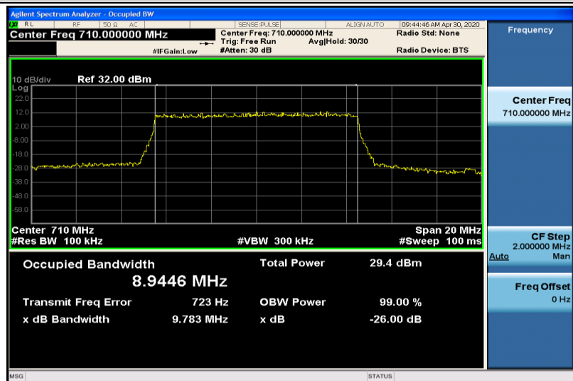
Band17-10MHz-QPSK-23790-50RB#0-8.9446
