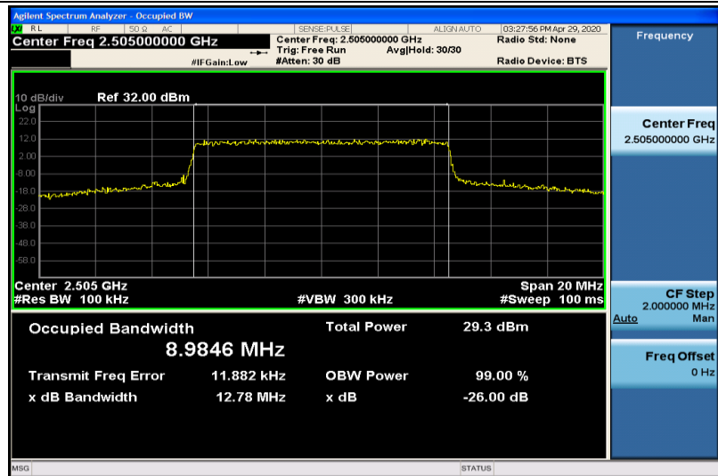
Band7-10MHz-QPSK-20800-50RB#0-8.9846
