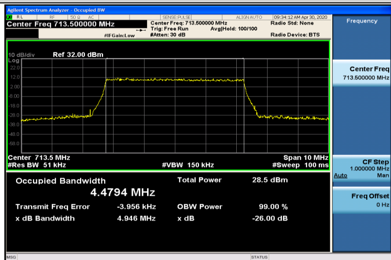
Band17-5MHz-16QAM-23825-25RB#0-4.4794
