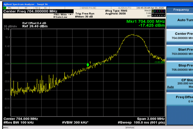
Band17-10MHz-16QAM-23780-1RB#0
