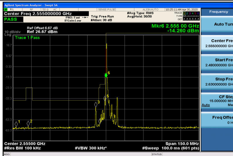
Band41-5MHz-QPSK-40265-1RB#0
