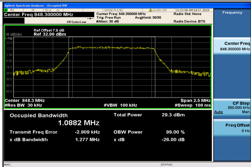
Band26-1.4MHz-QPSK-27033-6RB#0-1.0882
