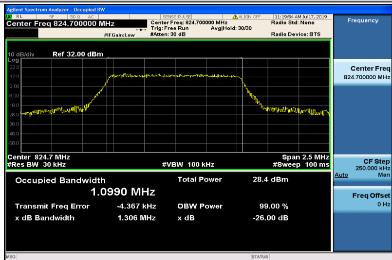
Band26-1.4MHz-16QAM-26797-6RB#0-1.0990
