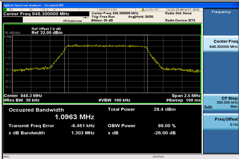
Band26-1.4MHz-16QAM-27033-6RB#0-1.0963
