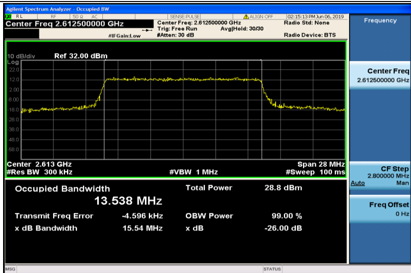
Band38-15MHz-16QAM-38175-75RB#0-13.538
