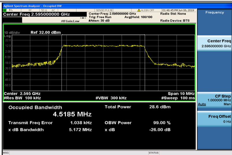
Band38-5MHz-16QAM-38000-25RB#0-4.5185
