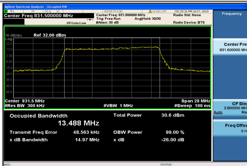
Band26-15MHz-QPSK-26915-75RB#0-13.488
