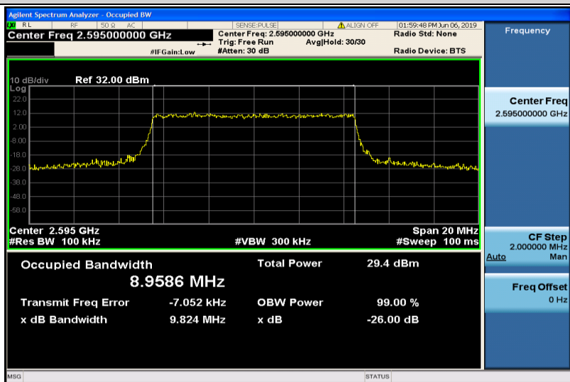
Band38-10MHz-QPSK-38000-50RB#0-8.9586
