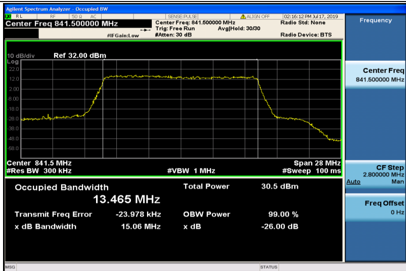
Band26-15MHz-QPSK-26965-75RB#0-13.465
