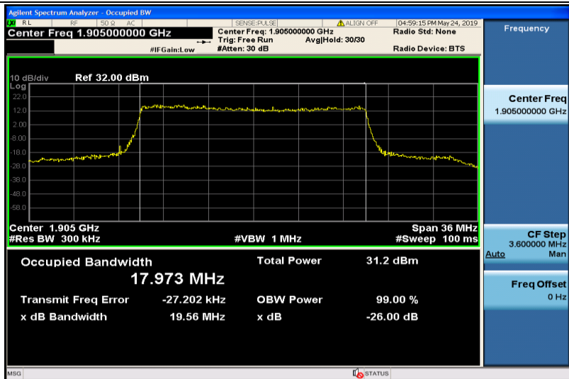
Band25-20MHz-QPSK-26590-100RB#0-17.973
