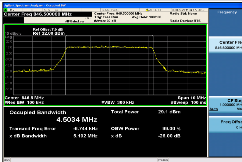
Band26-5MHz-16QAM-27015-25RB#0-4.5034
