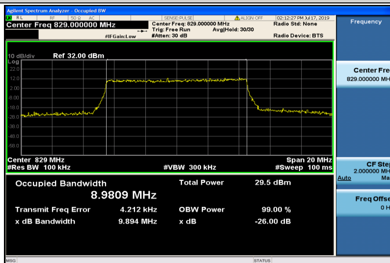
Band26-10MHz-16QAM-26840-50RB#0-8.9809
