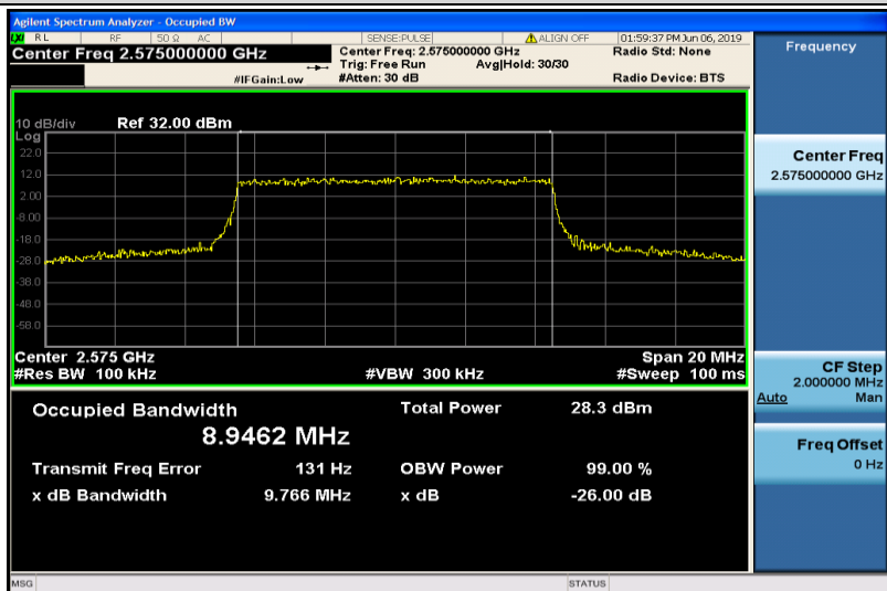
Band38-10MHz-16QAM-37800-50RB#0-8.9462
