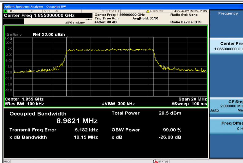
Band25-10MHz-16QAM-26090-50RB#0-8.9621
