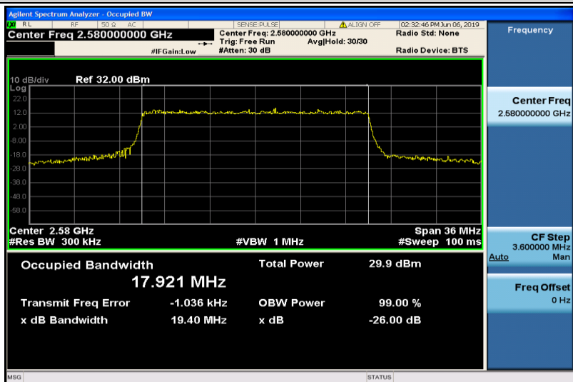
Band38-20MHz-QPSK-37850-100RB#0-17.921
