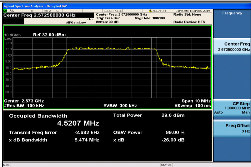
Band38-5MHz-QPSK-37775-25RB#0-4.5207
