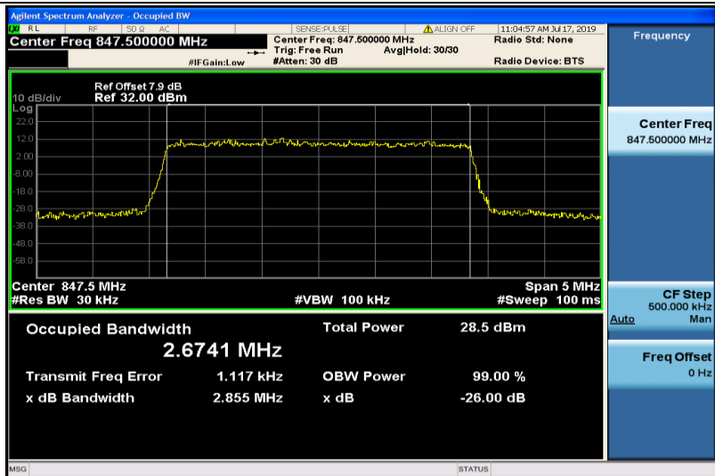
Band26-3MHz-16QAM-27025-15RB#0-2.6741
