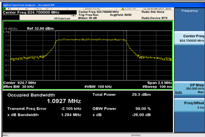
Band26-1.4MHz-QPSK-26797-6RB#0-1.0927
