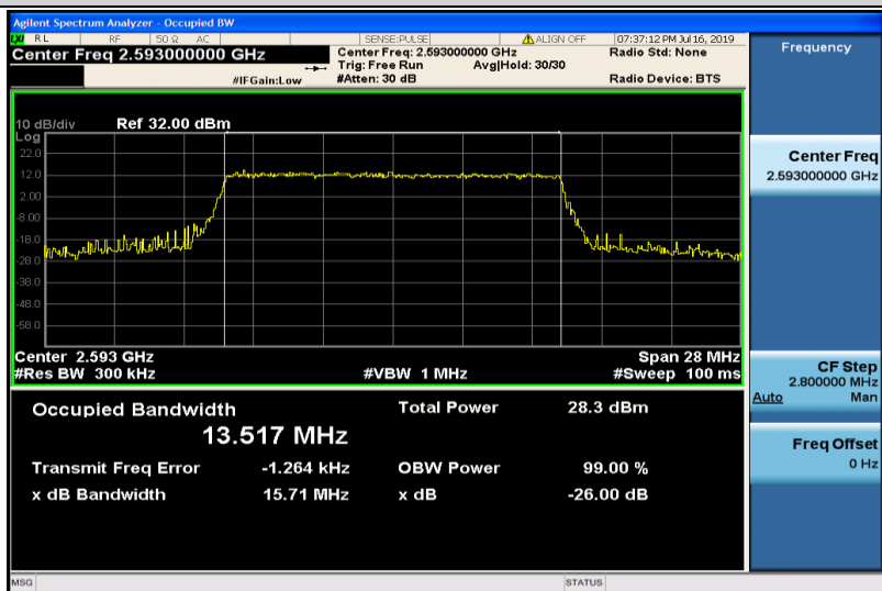
Band41-15MHz-16QAM-40620-75RB#0-13.517
