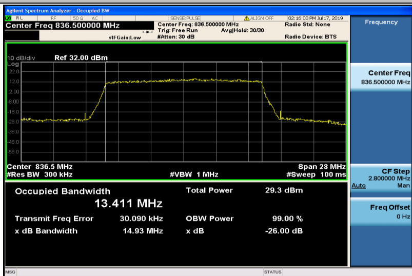
Band26-15MHz-16QAM-26915-75RB#0-13.411
