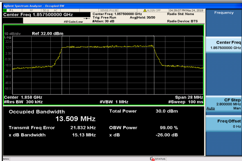
Band25-15MHz-16QAM-26115-75RB#0-13.509
