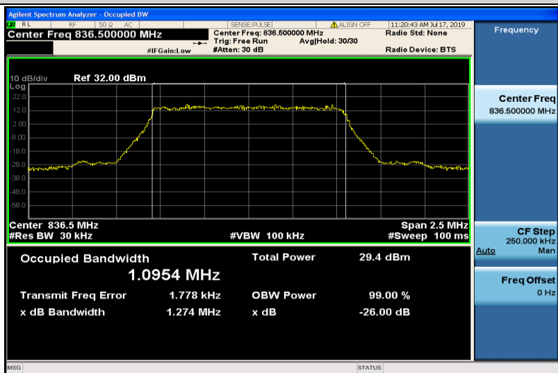
Band26-1.4MHz-QPSK-26915-6RB#0-1.0954
