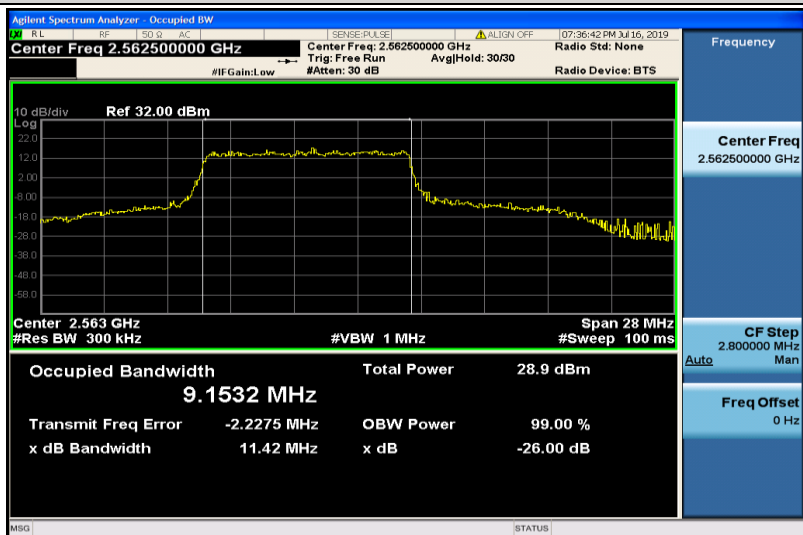
Band41-15MHz-QPSK-40315-75RB#0-9.1532
