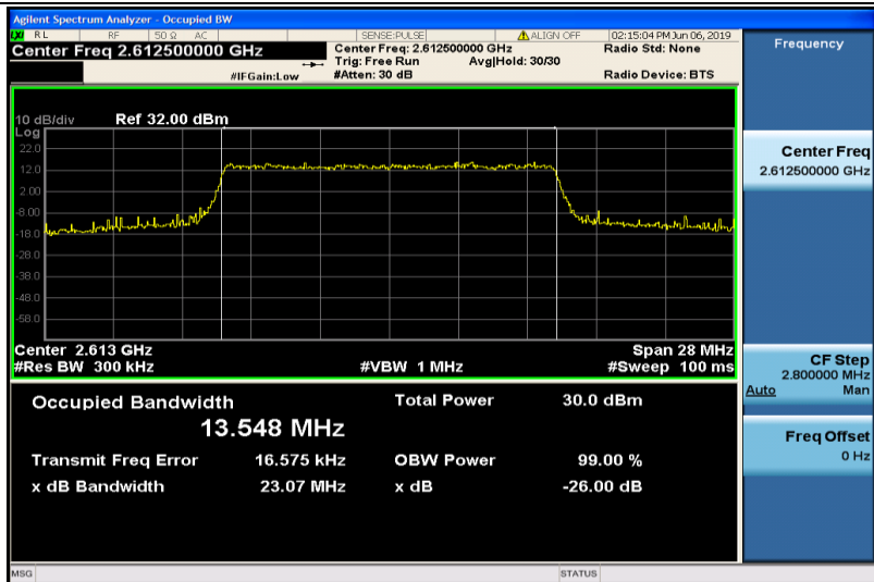
Band38-15MHz-QPSK-38175-75RB#0-13.548
