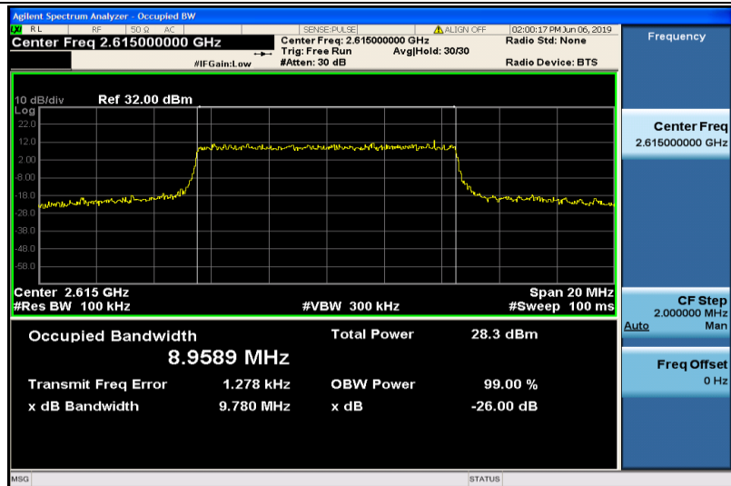
Band38-10MHz-16QAM-38200-50RB#0-8.9589
