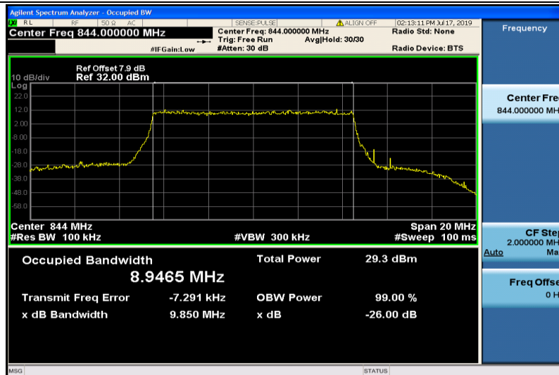
Band26-10MHz-16QAM-26990-50RB#0-8.9465
