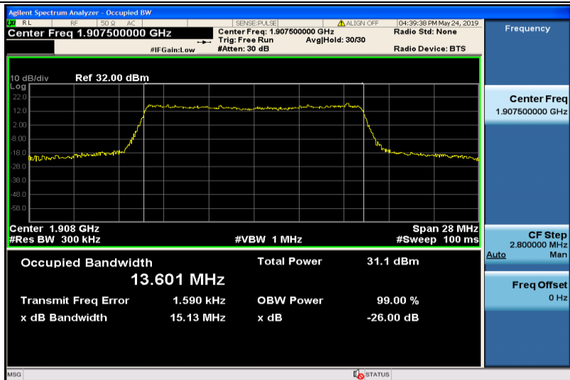
Band25-15MHz-QPSK-26615-75RB#0-13.601
