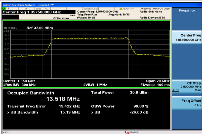
Band25-15MHz-QPSK-26115-75RB#0-13.518
