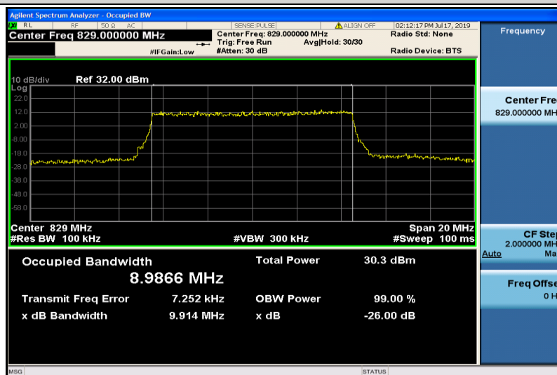
Band26-10MHz-QPSK-26840-50RB#0-8.9866
