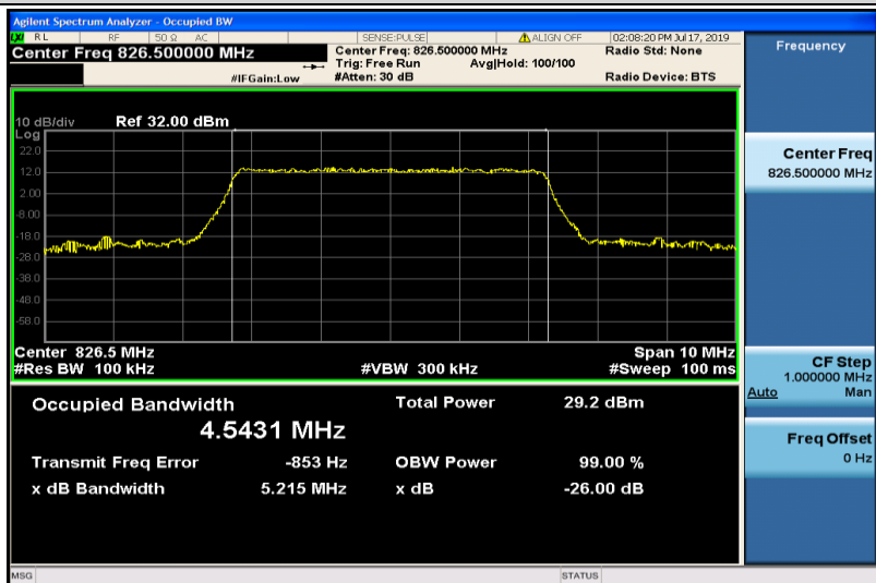
Band26-5MHz-16QAM-26815-25RB#0-4.5431
