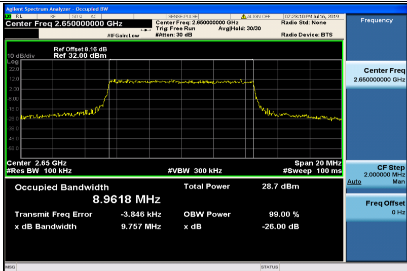
Band41-10MHz-QPSK-41190-50RB#0-8.9618
