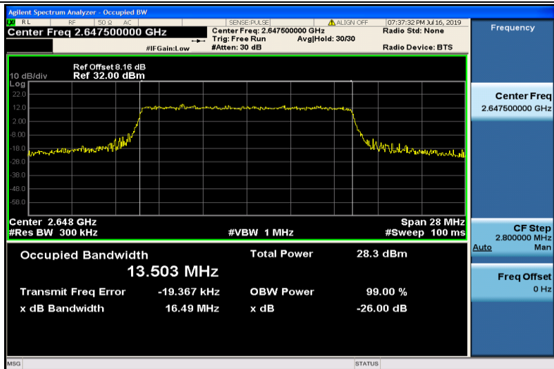
Band41-15MHz-16QAM-41165-75RB#0-13.503
