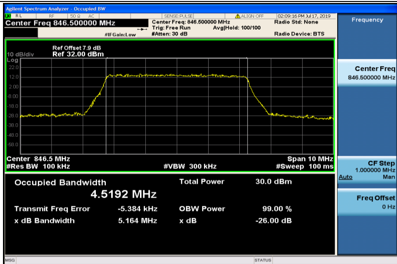
Band26-5MHz-QPSK-27015-25RB#0-4.5192
