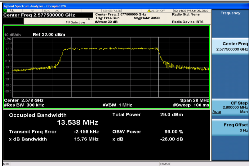
Band38-15MHz-16QAM-37825-75RB#0-13.538
