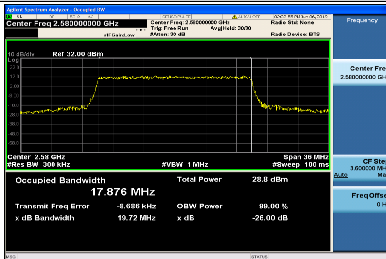
Band38-20MHz-16QAM-37850-100RB#0-17.876
