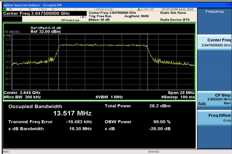
Band41-15MHz-QPSK-41165-75RB#0-13.517
