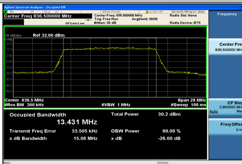
Band26-15MHz-QPSK-26915-75RB#0-13.431
