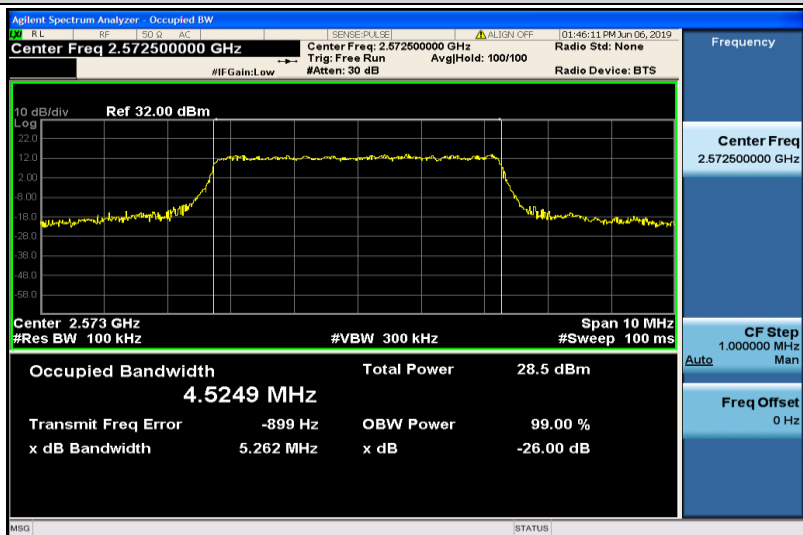
Band38-5MHz-16QAM-37775-25RB#0-4.5249
