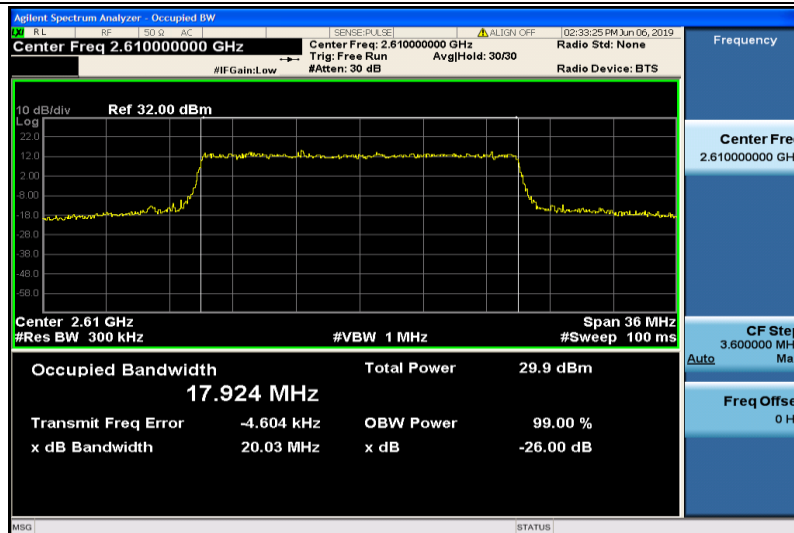
Band38-20MHz-QPSK-38150-100RB#0-17.924
