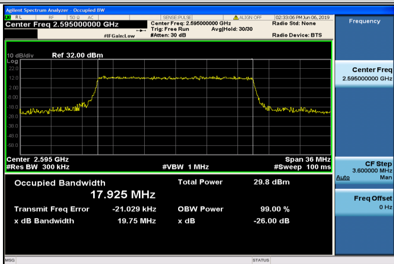
Band38-20MHz-QPSK-38000-100RB#0-17.925
