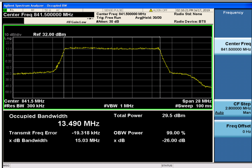
Band26-15MHz-16QAM-26965-75RB#0-13.490
