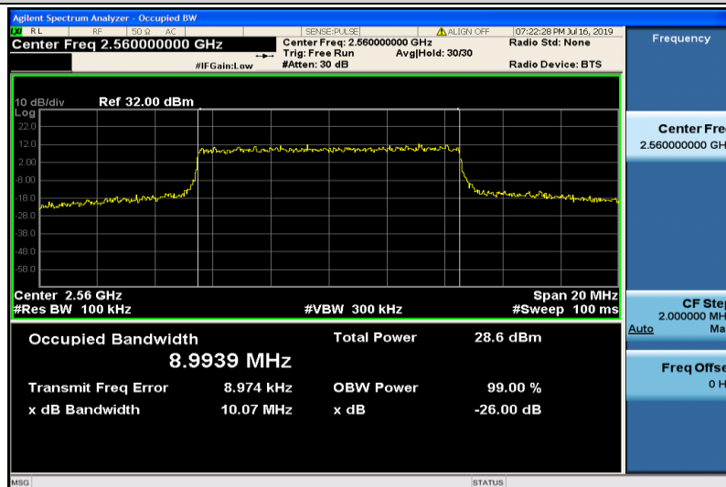
Band41-10MHz-QPSK-40290-50RB#0-8.9939
