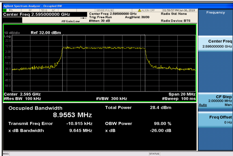
Band38-10MHz-16QAM-38000-50RB#0-8.9553
