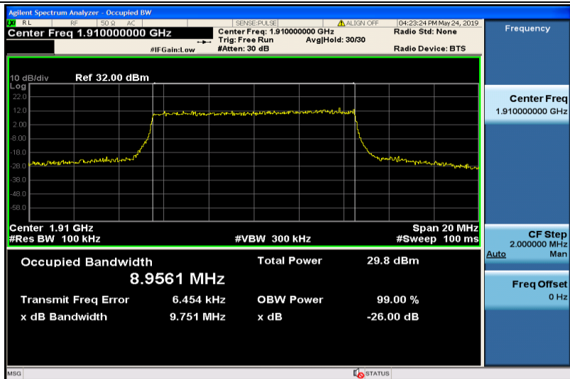
Band25-10MHz-16QAM-26640-50RB#0-8.9561
