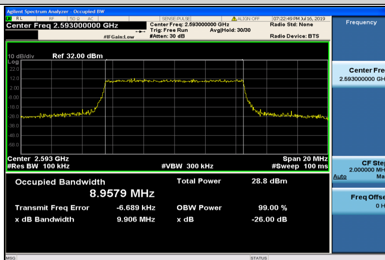
Band41-10MHz-QPSK-40620-50RB#0-8.9579
