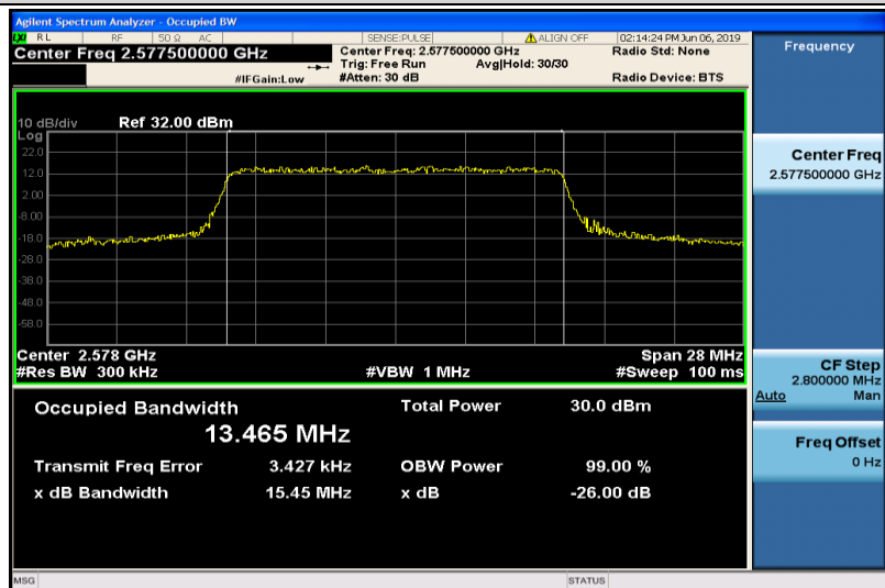
Band38-15MHz-QPSK-37825-75RB#0-13.465
