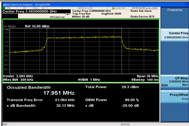
Band41-20MHz-QPSK-40340-100RB#0-17.951
