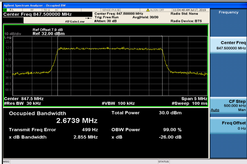
Band26-3MHz-QPSK-27025-15RB#0-2.6739
