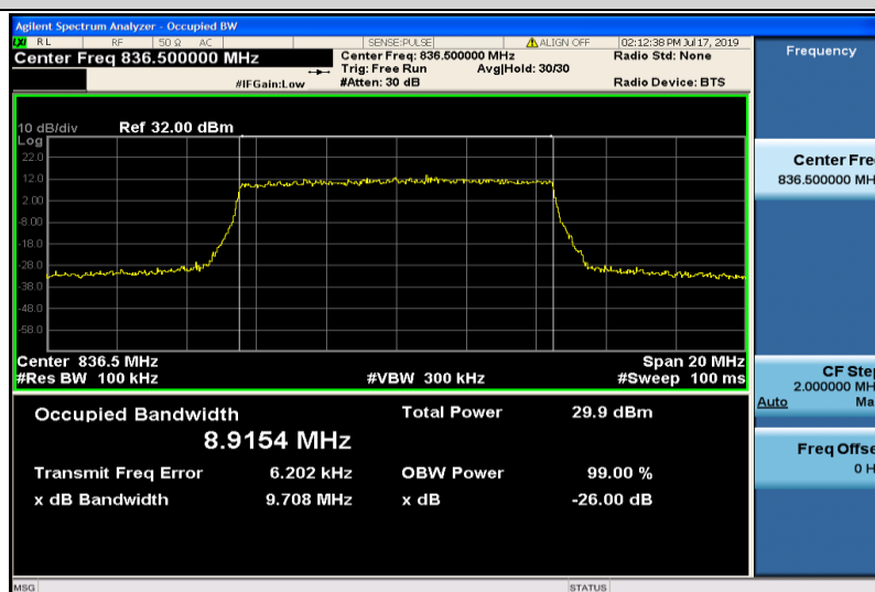
Band26-10MHz-QPSK-26915-50RB#0-8.9154
