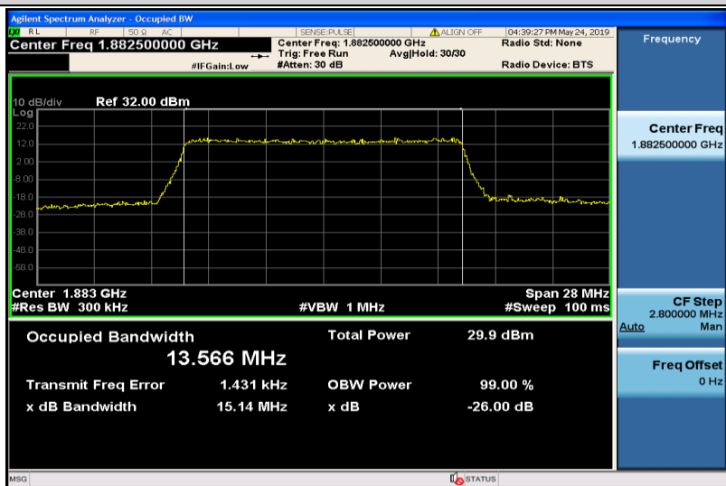
Band25-15MHz-16QAM-26365-75RB#0-13.566
