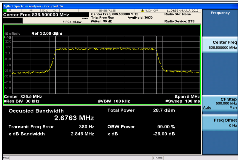
Band26-3MHz-16QAM-26915-15RB#0-2.6763
