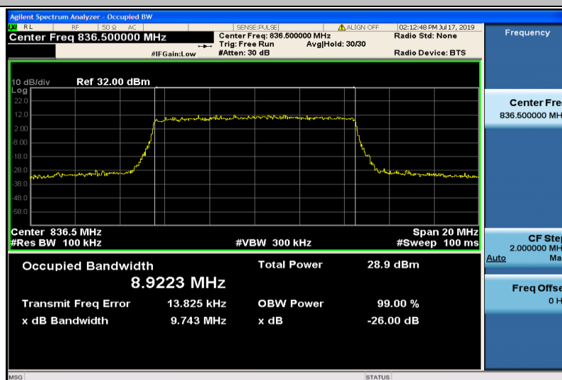
Band26-10MHz-16QAM-26915-50RB#0-8.9223
