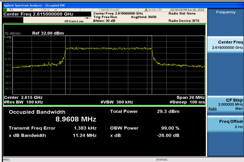
Band38-10MHz-QPSK-38200-50RB#0-8.9608
