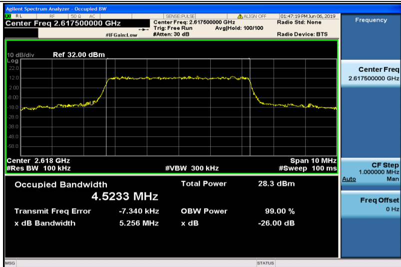
Band38-5MHz-16QAM-38225-25RB#0-4.5233
