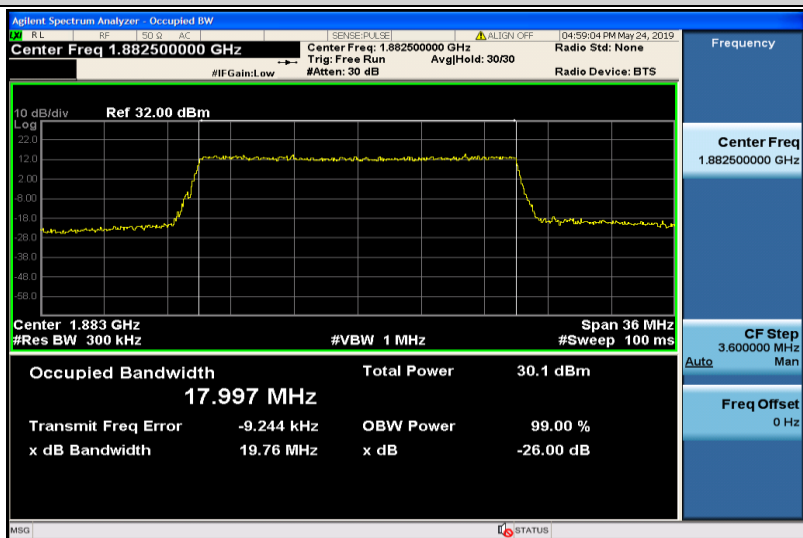
Band25-20MHz-16QAM-26365-100RB#0-17.997
