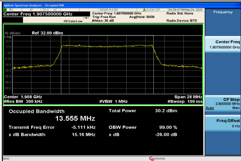
Band25-15MHz-16QAM-26615-75RB#0-13.555
