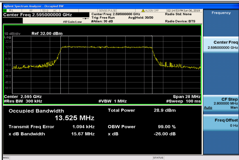
Band38-15MHz-16QAM-38000-75RB#0-13.525
