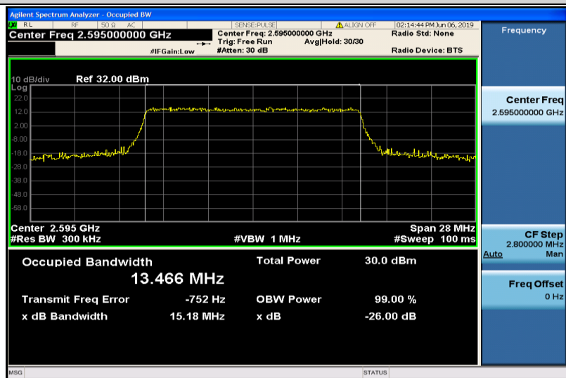
Band38-15MHz-QPSK-38000-75RB#0-13.466
