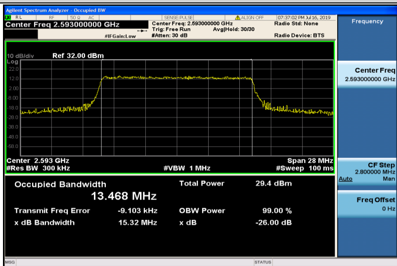
Band41-15MHz-QPSK-40620-75RB#0-13.468
