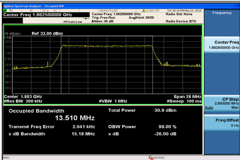
Band25-15MHz-QPSK-26365-75RB#0-13.510
