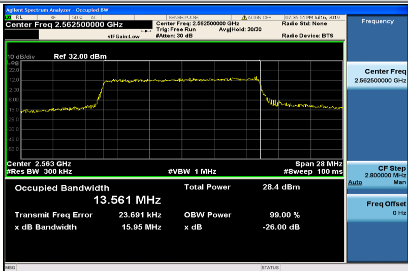
Band41-15MHz-16QAM-40315-75RB#0-13.561
