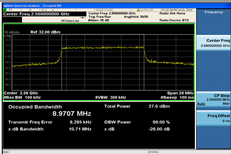
Band41-10MHz-16QAM-40290-50RB#0-8.9707
