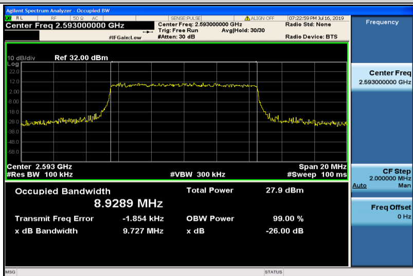
Band41-10MHz-16QAM-40620-50RB#0-8.9289
