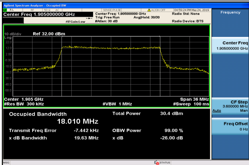
Band25-20MHz-16QAM-26590-100RB#0-18.010
