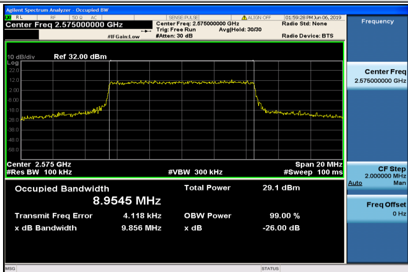
Band38-10MHz-QPSK-37800-50RB#0-8.9545
