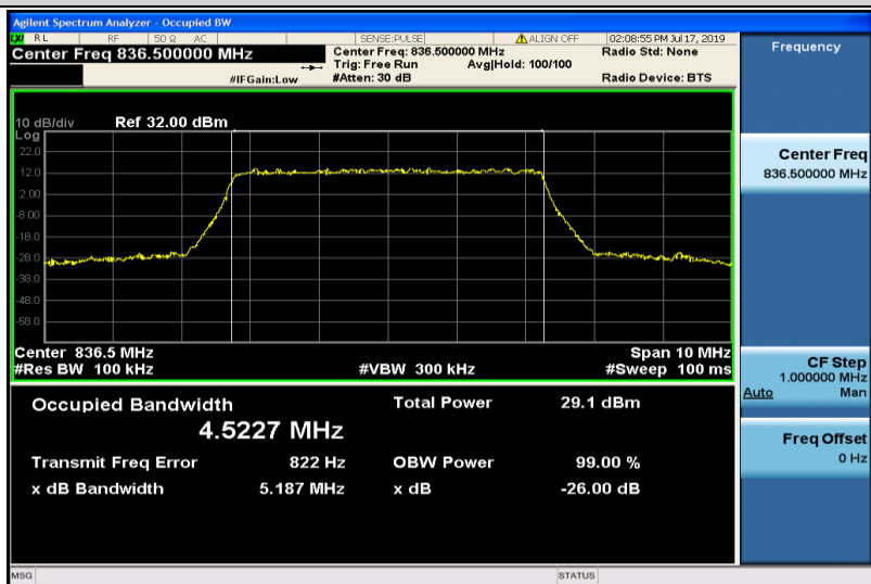
Band26-5MHz-16QAM-26915-25RB#0-4.5227
