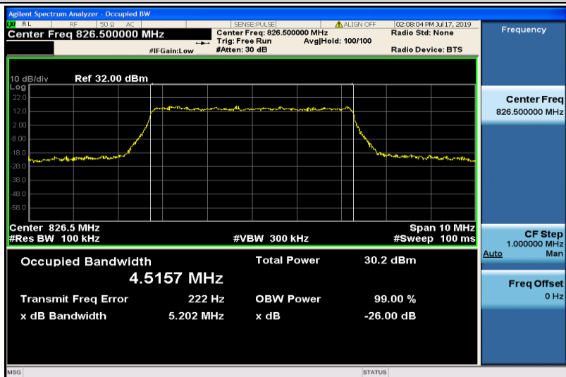
Band26-5MHz-QPSK-26815-25RB#0-4.5157
