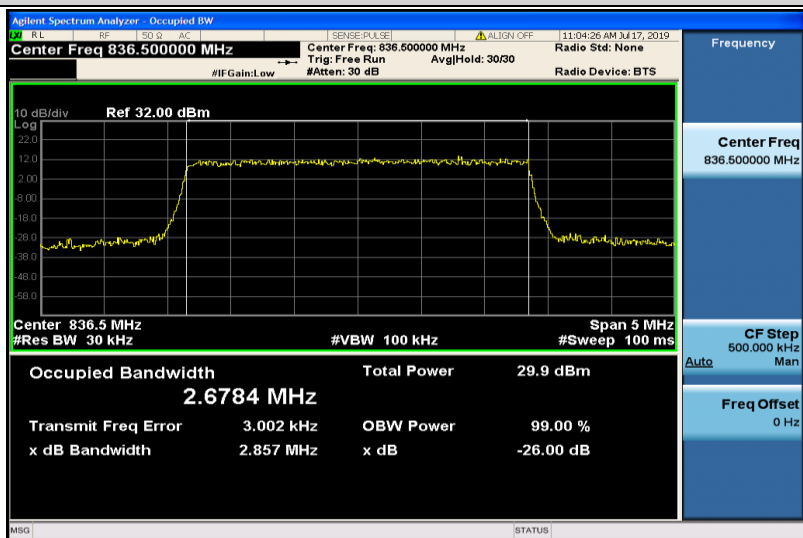
Band26-3MHz-QPSK-26915-15RB#0-2.6784
