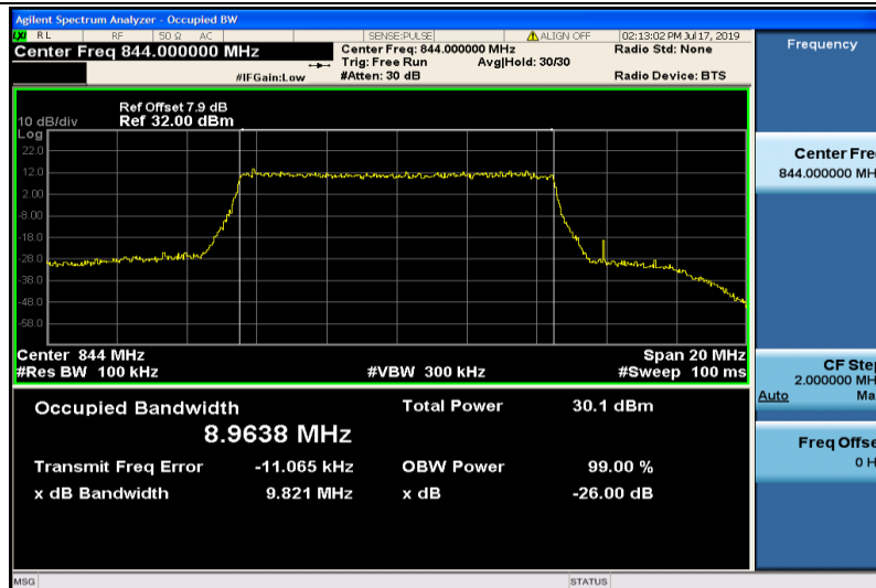
Band26-10MHz-QPSK-26990-50RB#0-8.9638
