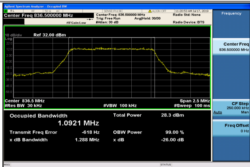
Band26-1.4MHz-16QAM-26915-6RB#0-1.0921
