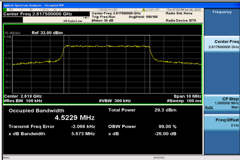
Band38-5MHz-QPSK-38225-25RB#0-4.5229
