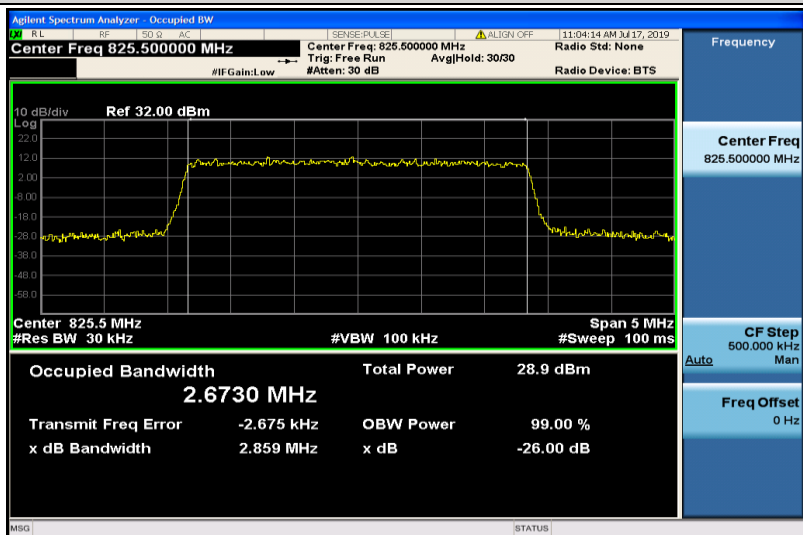
Band26-3MHz-16QAM-26805-15RB#0-2.6730
