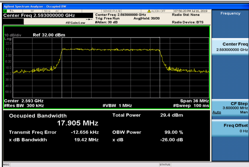
Band41-20MHz-QPSK-40620-100RB#0-17.905
