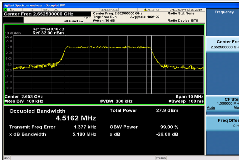
Band41-5MHz-16QAM-41215-25RB#0-4.5162
