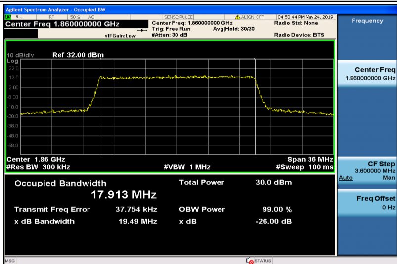
Band25-20MHz-16QAM-26140-100RB#0-17.913
