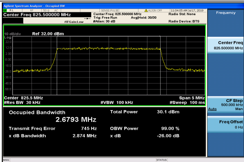
Band26-3MHz-QPSK-26805-15RB#0-2.6793
