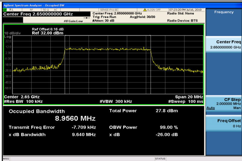
Band41-10MHz-16QAM-41190-50RB#0-8.9560
