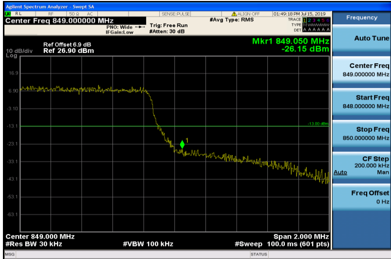
Band5-1.4MHz-QPSK-20643-6RB#0
