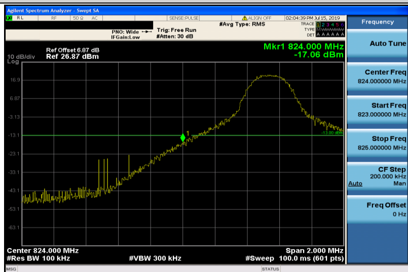
Band5-5MHz-16QAM-20425-1RB#0
