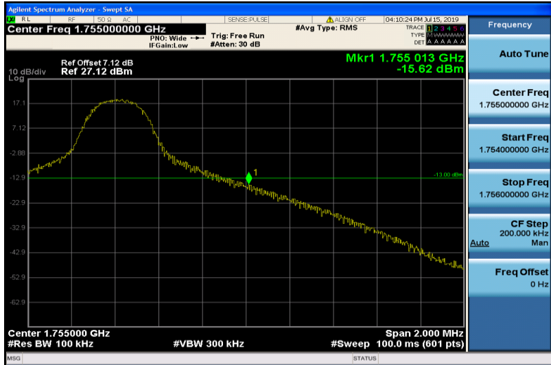
Band4-10MHz-16QAM-20350-1RB#49
