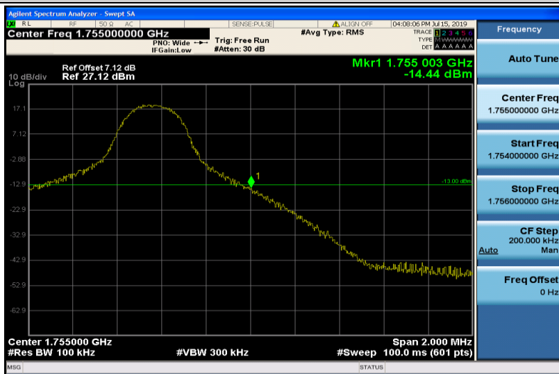
Band4-5MHz-16QAM-20375-1RB#24
