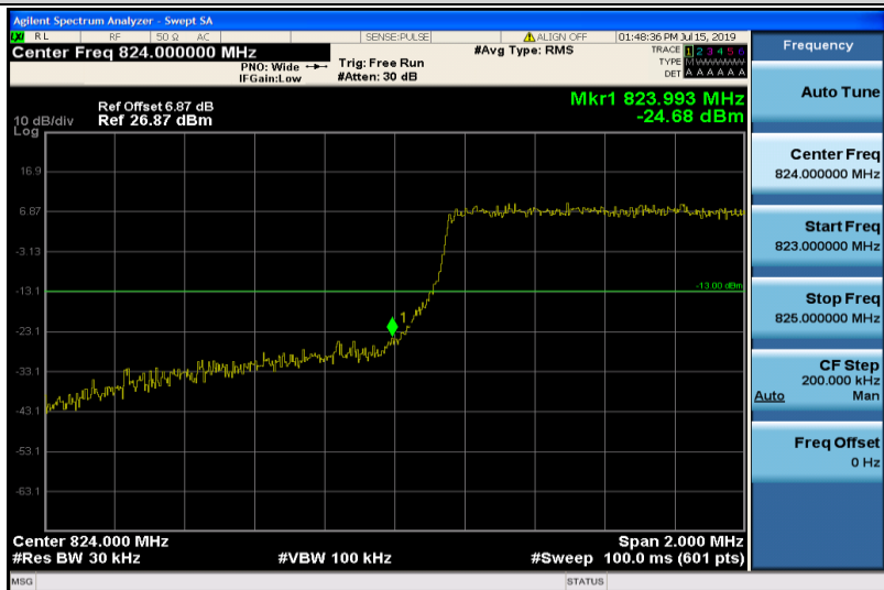
Band5-1.4MHz-16QAM-20407-6RB#0
