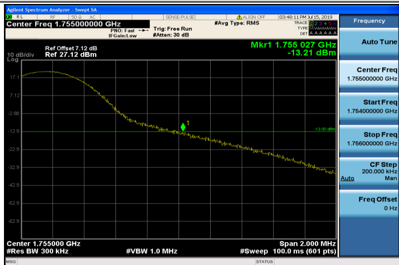
Band4-15MHz-QPSK-20325-1RB#74
