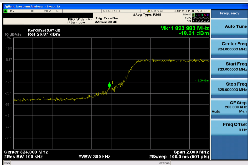
Band5-5MHz-QPSK-20425-25RB#0
