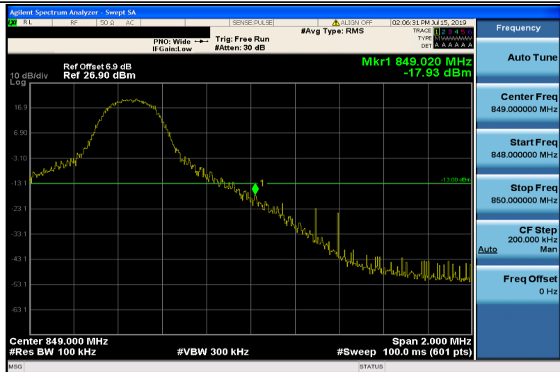
Band5-5MHz-QPSK-20625-1RB#24
