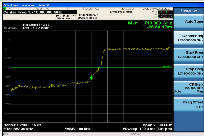
Band4-1.4MHz-QPSK-19957-6RB#0
