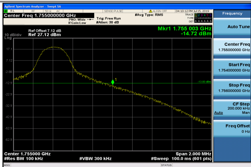
Band4-10MHz-QPSK-20350-1RB#49
