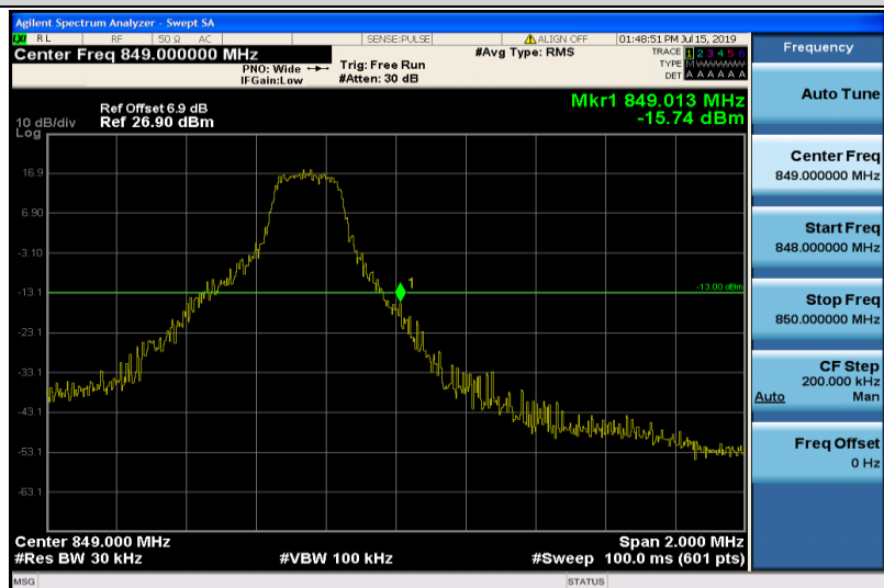
Band5-1.4MHz-QPSK-20643-1RB#5
