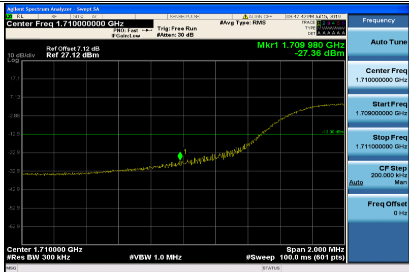
Band4-15MHz-QPSK-20025-75RB#0
