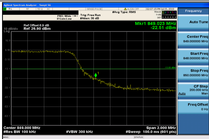
Band5-5MHz-QPSK-20625-25RB#0
