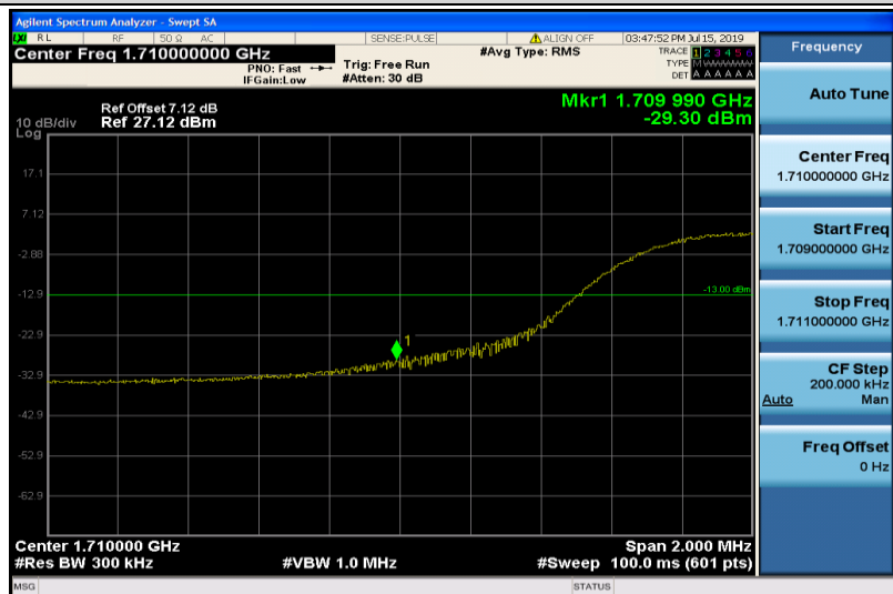
Band4-15MHz-16QAM-20025-75RB#0
