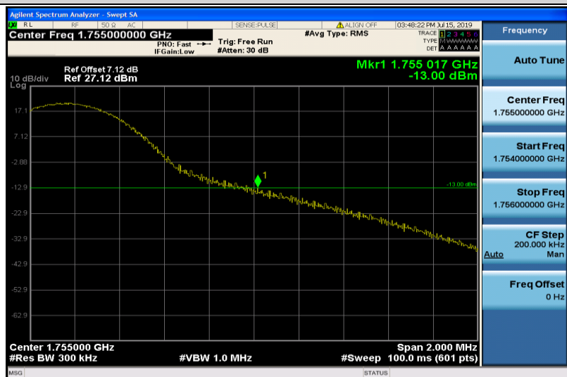
Band4-15MHz-16QAM-20325-1RB#74
