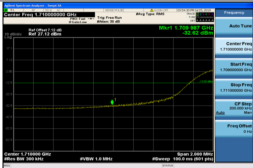
Band4-20MHz-16QAM-20050-100RB#0
