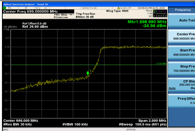
Band12-1.4MHz-16QAM-23017-6RB#0
