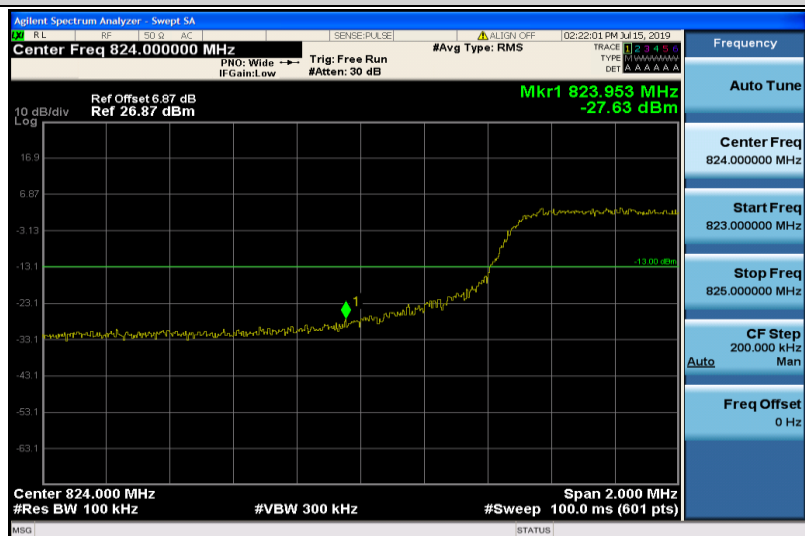
Band5-10MHz-16QAM-20450-50RB#0
