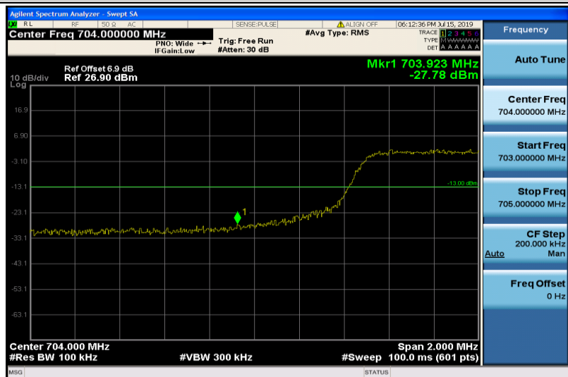
Band17-10MHz-16QAM-23780-50RB#0
