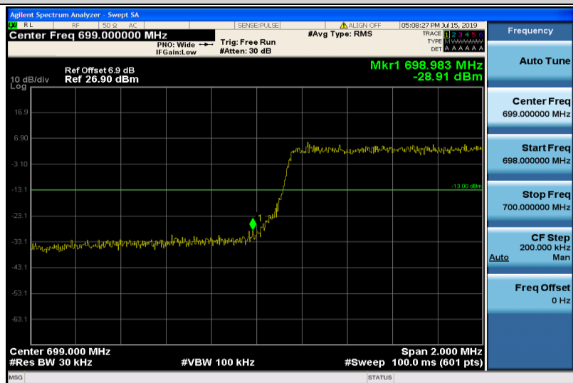
Band12-3MHz-16QAM-23025-15RB#0
