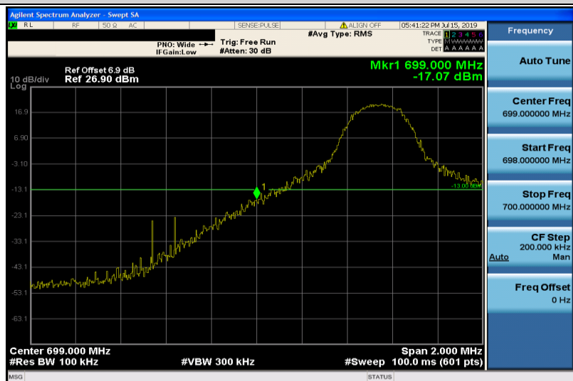
Band12-5MHz-QPSK-23035-1RB#0
