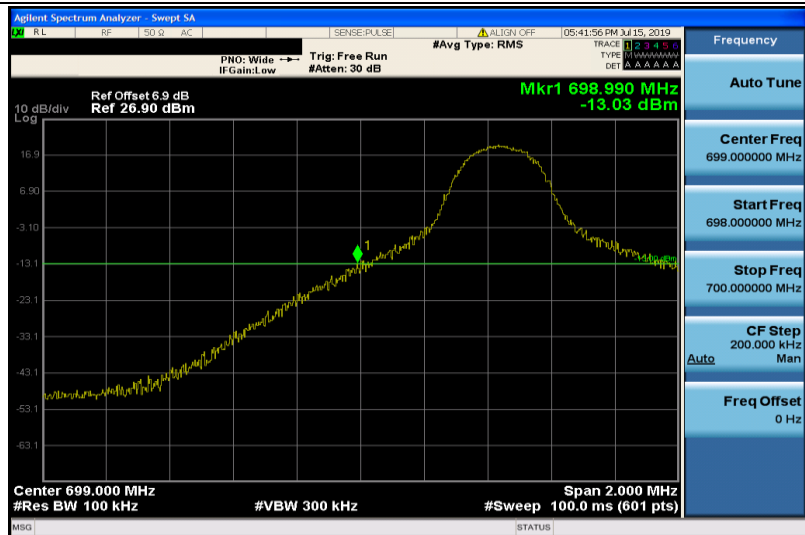
Band12-5MHz-16QAM-23035-1RB#0
