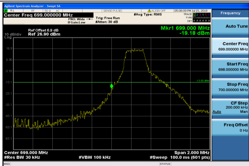
Band12-3MHz-16QAM-23025-1RB#0
