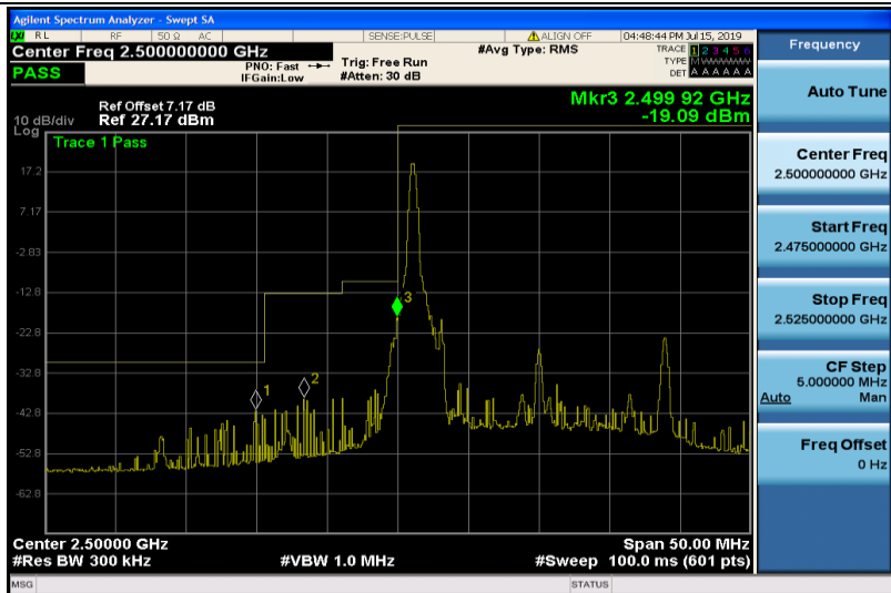
Band7-20MHz-16QAM-20850-1RB#0
