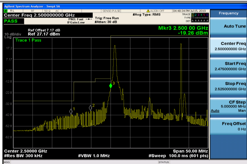
Band7-20MHz-QPSK-20850-1RB#0
