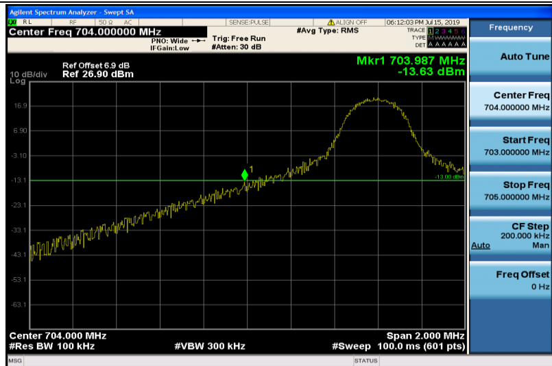
Band17-10MHz-16QAM-23780-1RB#0
