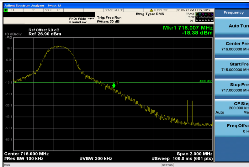
Band17-5MHz-16QAM-23825-1RB#24
