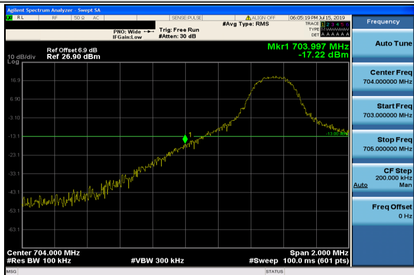
Band17-5MHz-16QAM-23755-1RB#0
