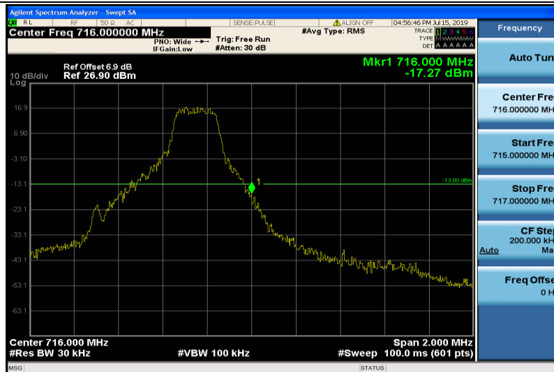
Band12-1.4MHz-QPSK-23173-1RB#5
