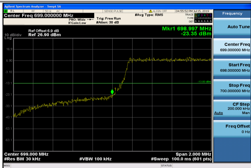
Band12-1.4MHz-QPSK-23017-6RB#0
