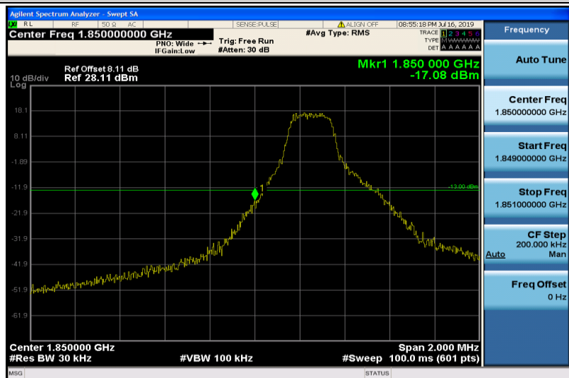
Band25-1.4MHz-QPSK-26047-1RB#0
