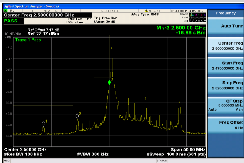
Band7-10MHz-16QAM-20800-1RB#0
