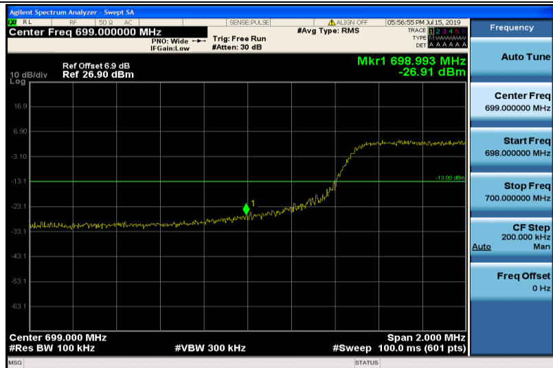
Band12-10MHz-16QAM-23060-50RB#0
