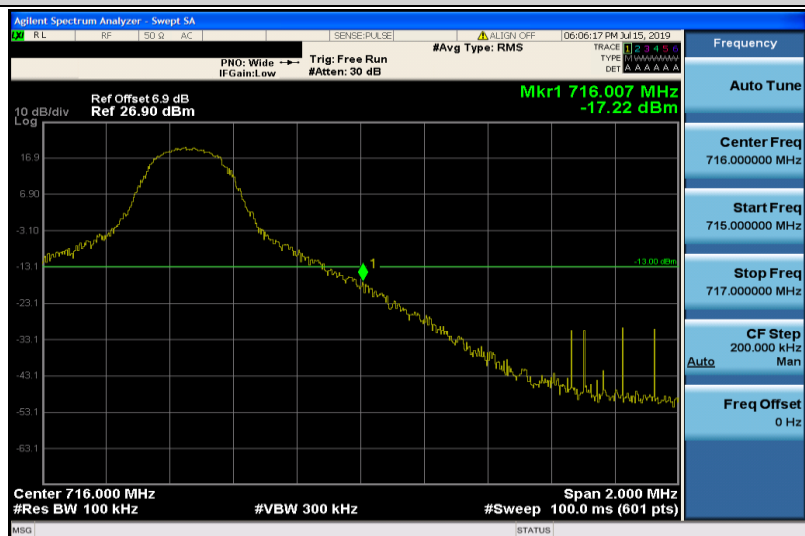
Band17-5MHz-QPSK-23825-1RB#24
