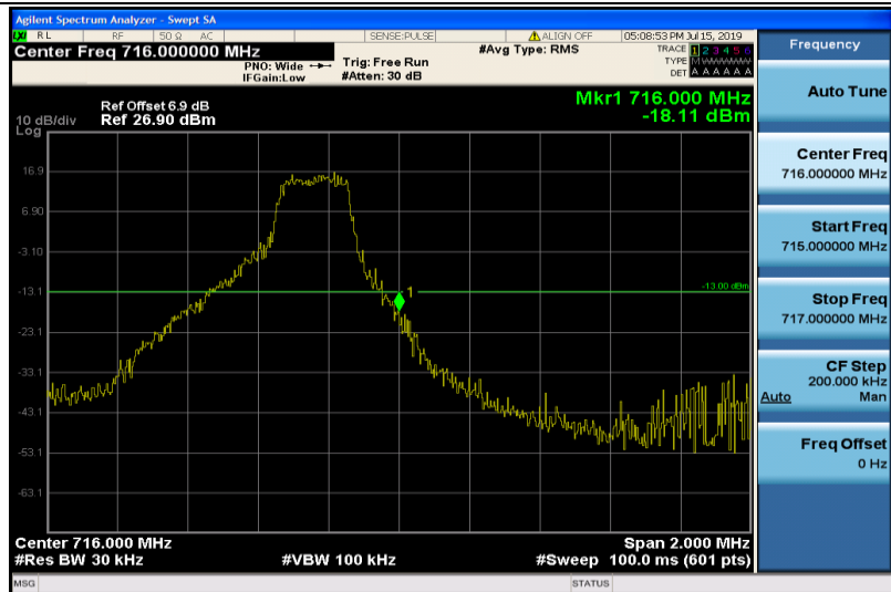
Band12-3MHz-16QAM-23165-1RB#14
