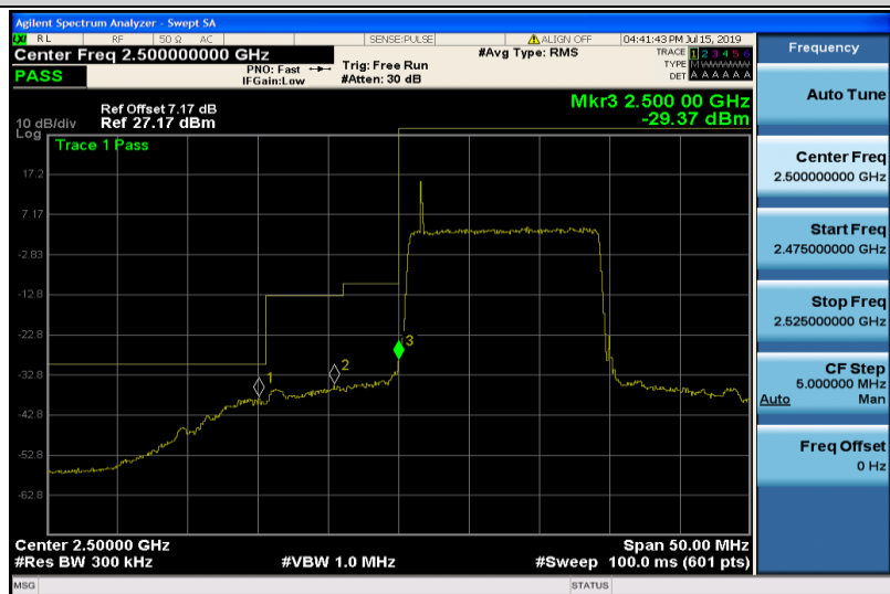
Band7-15MHz-16QAM-20825-75RB#0
