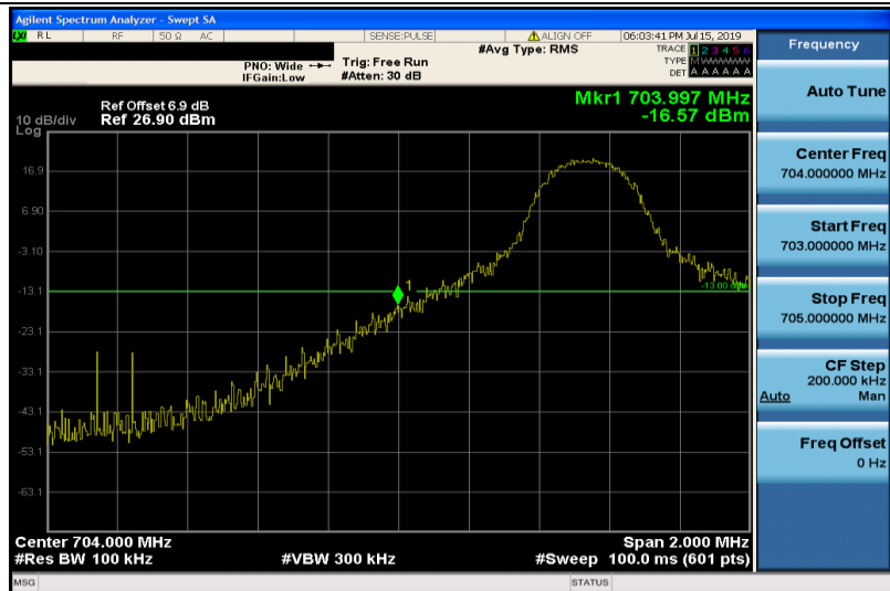
Band17-5MHz-QPSK-23755-1RB#0
