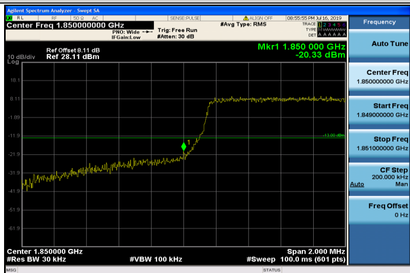
Band25-1.4MHz-QPSK-26047-6RB#0
