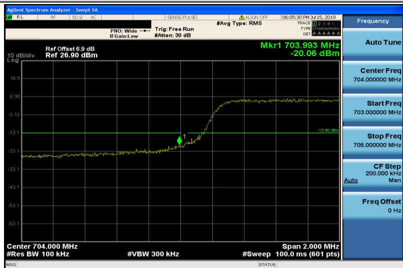
Band17-5MHz-QPSK-23755-25RB#0
