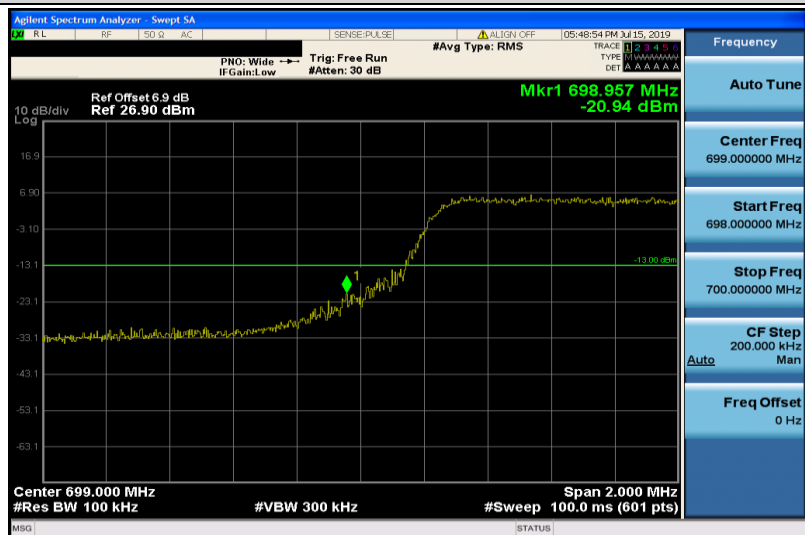
Band12-5MHz-16QAM-23035-25RB#0
