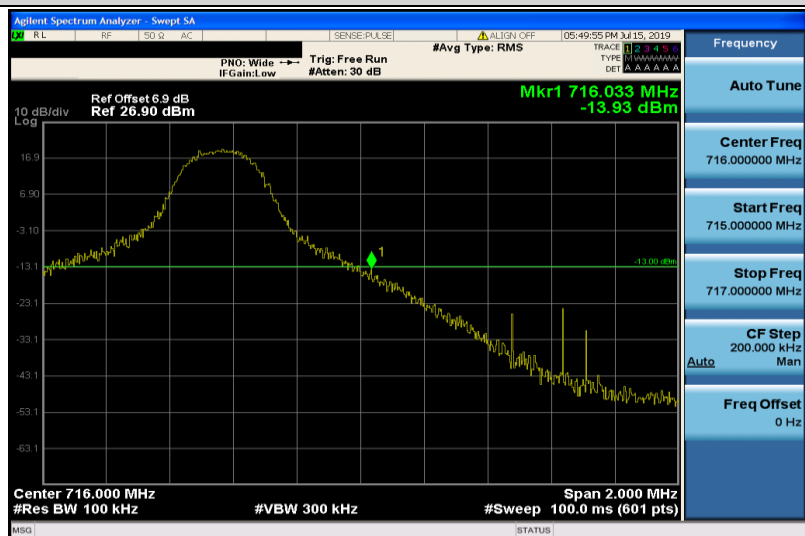
Band12-5MHz-16QAM-23155-1RB#24
