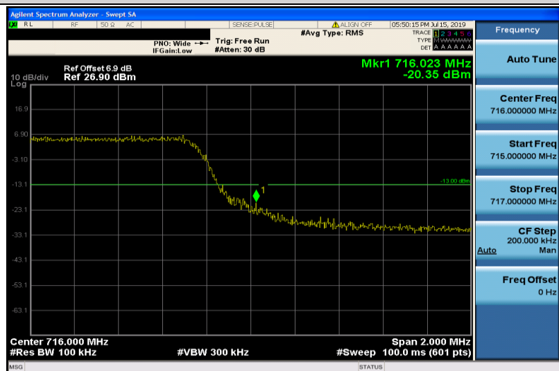
Band12-5MHz-QPSK-23155-25RB#0
