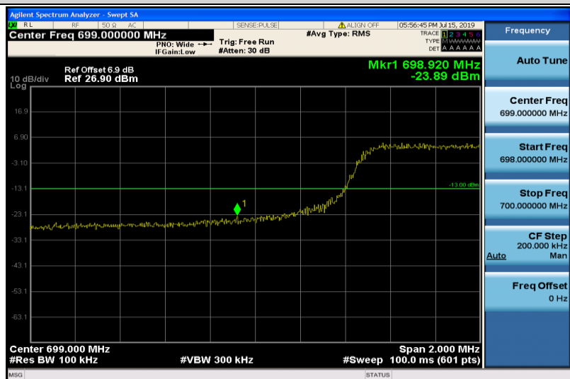
Band12-10MHz-QPSK-23060-50RB#0
