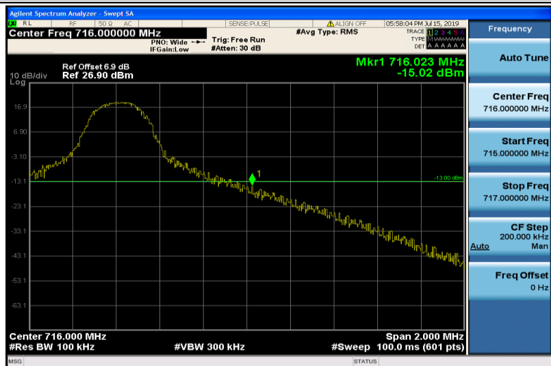
Band12-10MHz-16QAM-23130-1RB#49
