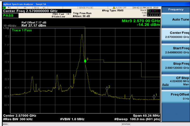
Band7-15MHz-16QAM-21375-1RB#74
