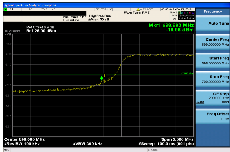
Band12-5MHz-QPSK-23035-25RB#0
