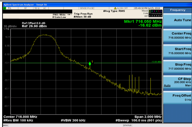
Band12-5MHz-QPSK-23155-1RB#24
