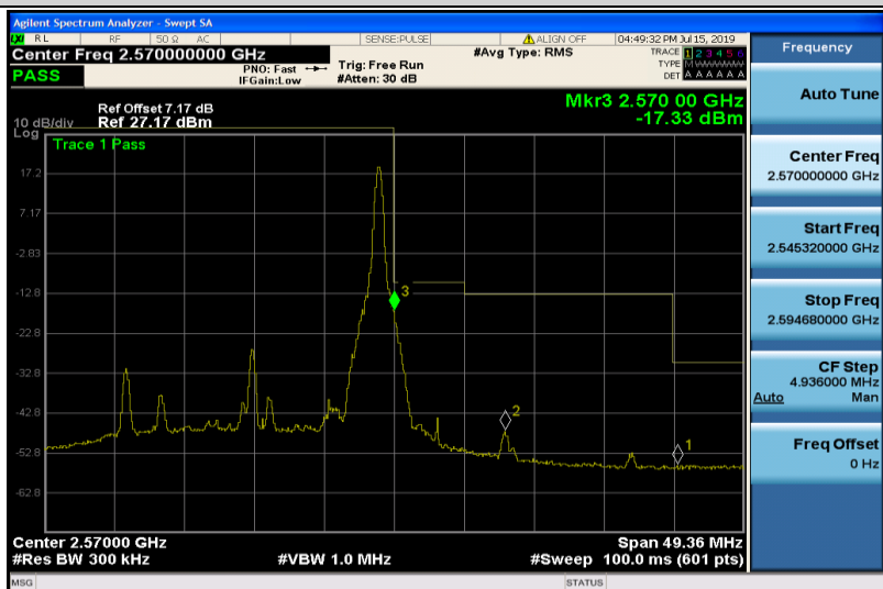
Band7-20MHz-16QAM-21350-1RB#99
