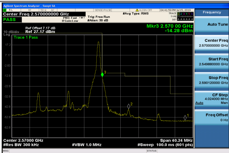
Band7-15MHz-QPSK-21375-1RB#74
