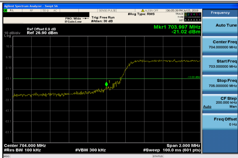
Band17-5MHz-16QAM-23755-25RB#0
