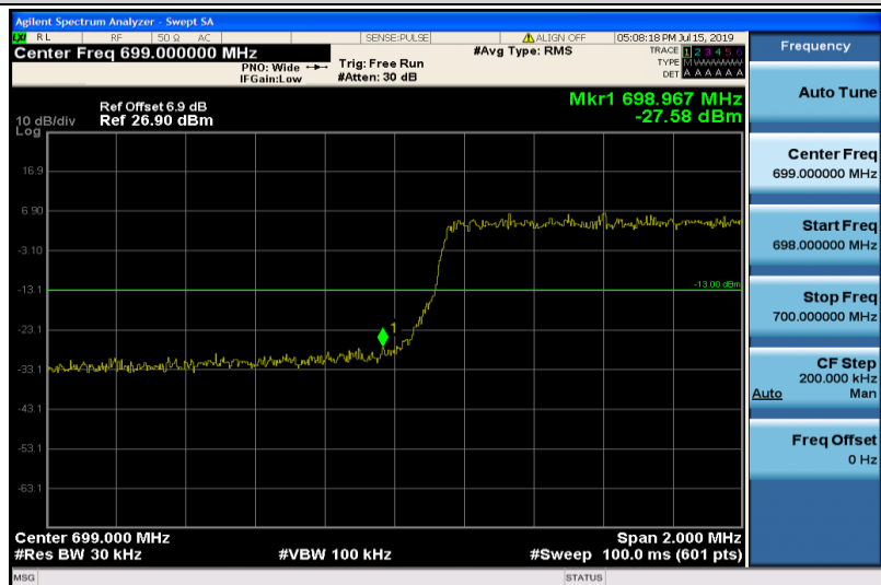
Band12-3MHz-QPSK-23025-15RB#0
