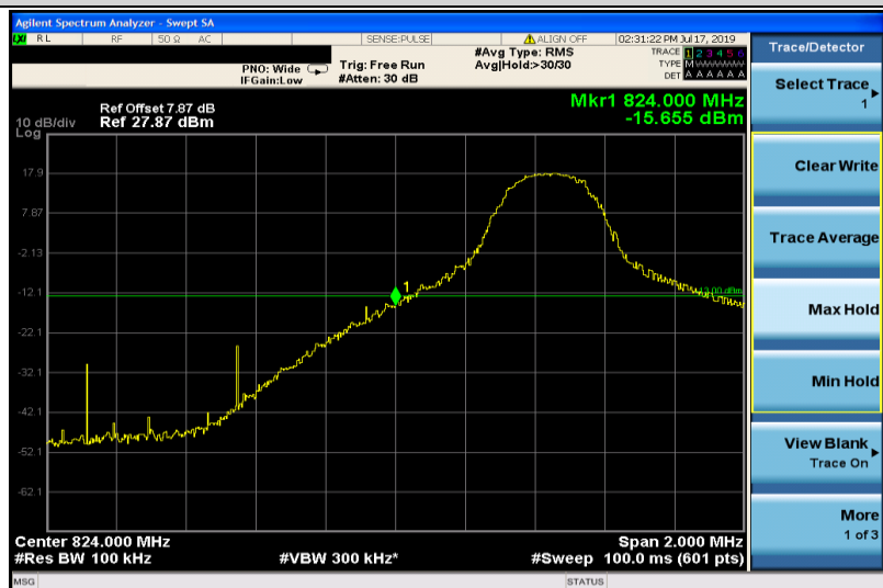
Band26-5MHz-QPSK-26815-1RB#0
