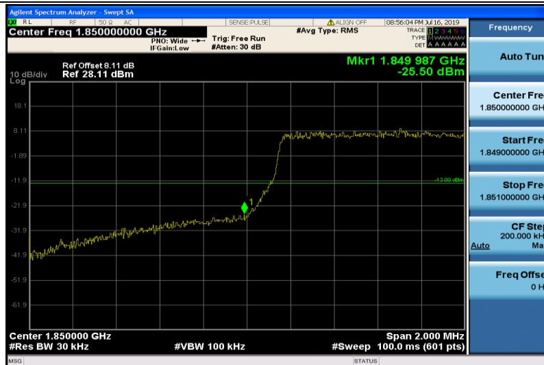
Band25-1.4MHz-16QAM-26047-6RB#0
