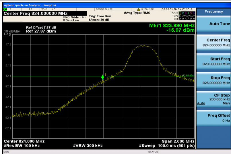
Band26-5MHz-16QAM-26815-1RB#0
