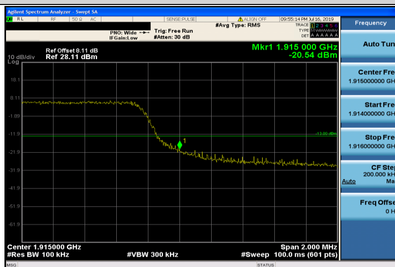
Band25-5MHz-QPSK-26665-25RB#0
