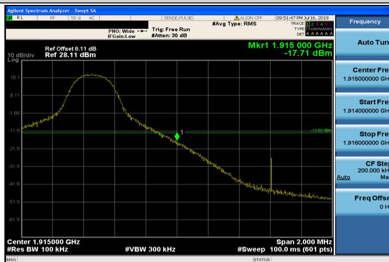
Band25-5MHz-QPSK-26665-1RB#24
