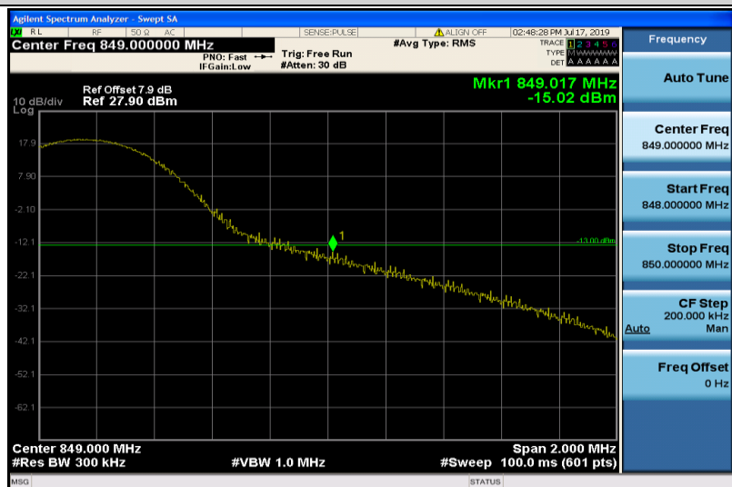
Band26-15MHz-QPSK-26965-1RB#74
