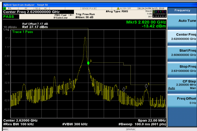
Band38-5MHz-QPSK-38225-1RB#24
