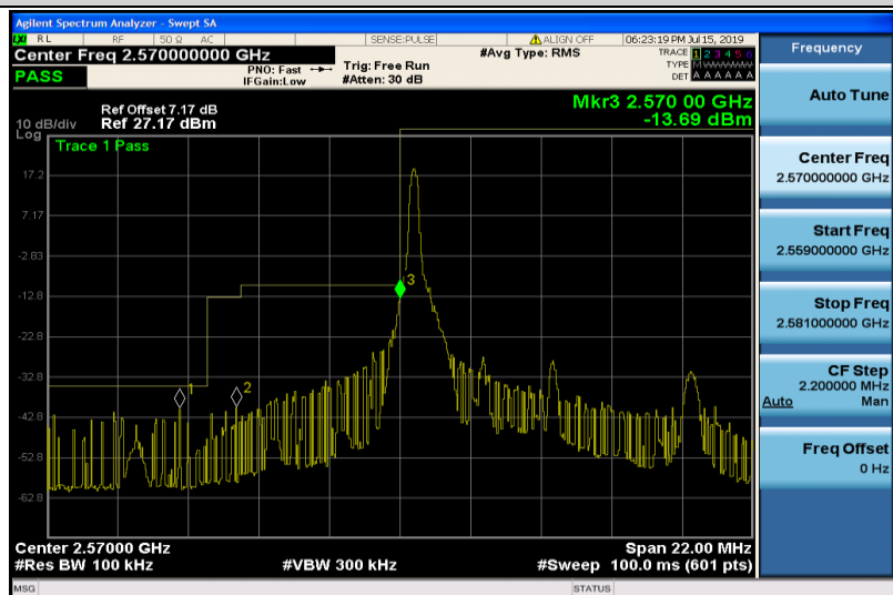
Band38-5MHz-QPSK-37775-1RB#0
