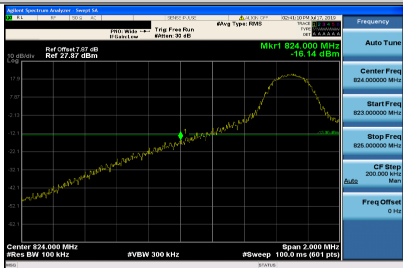
Band26-10MHz-16QAM-26840-1RB#0
