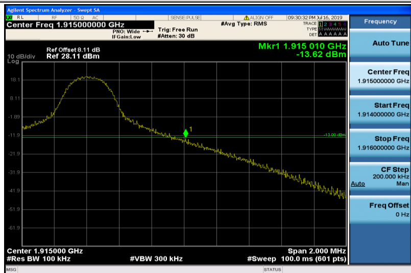
Band25-10MHz-16QAM-26640-1RB#49
