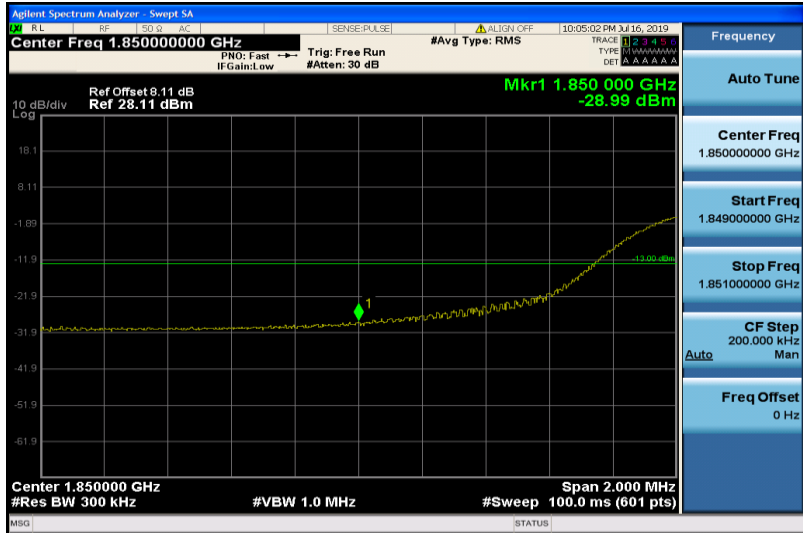
Band25-20MHz-QPSK-26140-100RB#0
