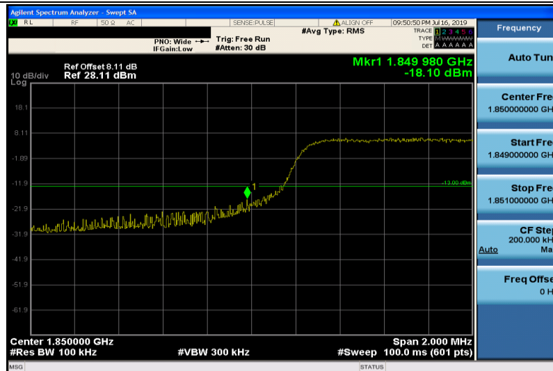
Band25-5MHz-QPSK-26065-25RB#0
