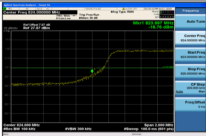
Band26-5MHz-16QAM-26815-25RB#0
