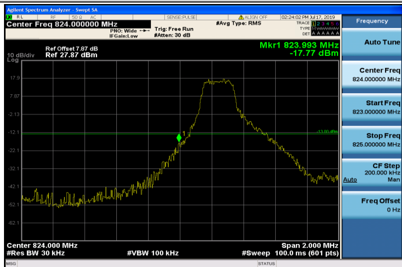
Band26-3MHz-16QAM-26805-1RB#0
