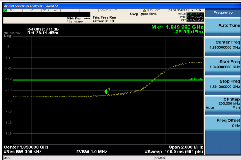
Band25-15MHz-QPSK-26115-75RB#0
