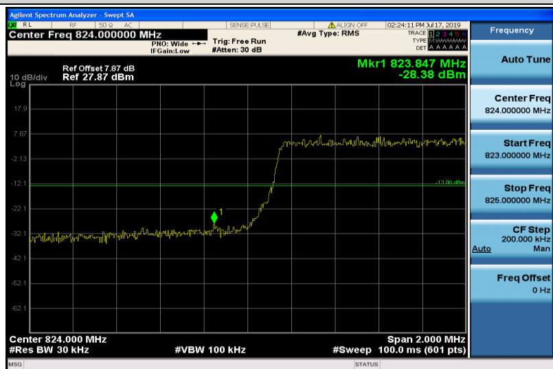
Band26-3MHz-QPSK-26805-15RB#0
