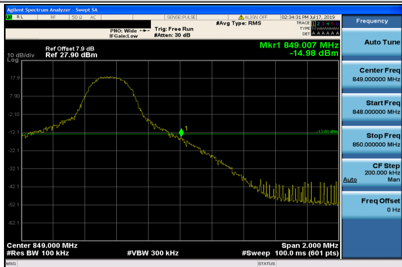
Band26-5MHz-QPSK-27015-1RB#24
