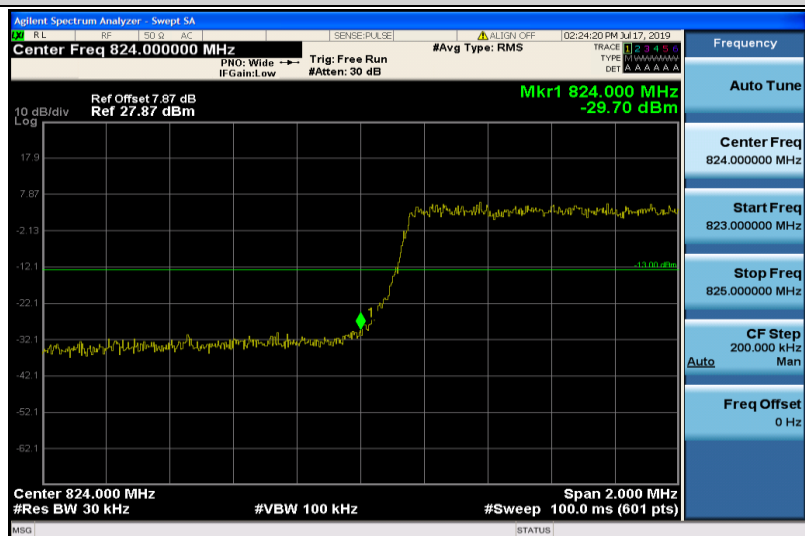
Band26-3MHz-16QAM-26805-15RB#0
