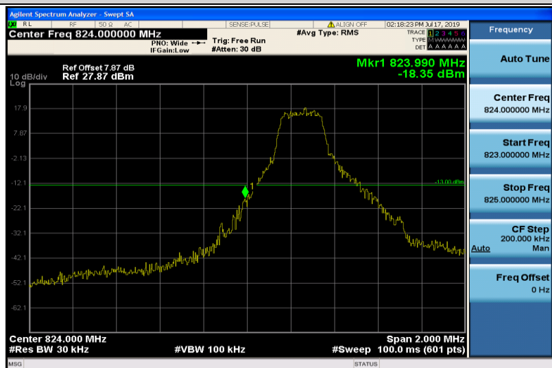
Band26-1.4MHz-16QAM-26797-1RB#0
