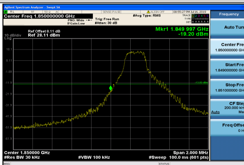
Band25-1.4MHz-16QAM-26047-1RB#0
