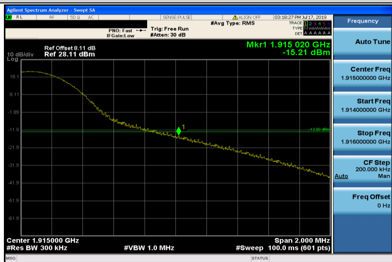
Band25-15MHz-QPSK-26615-1RB#74
