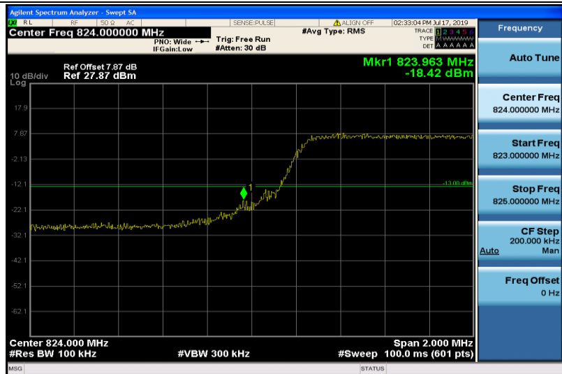
Band26-5MHz-QPSK-26815-25RB#0
