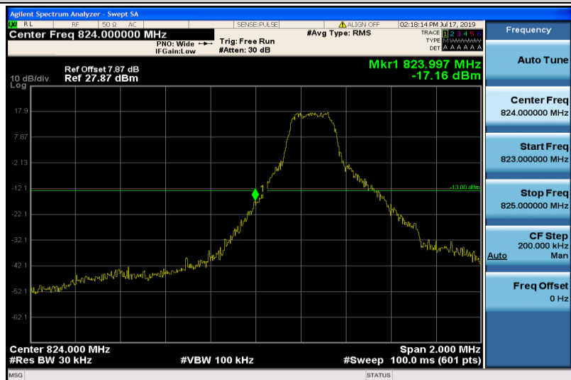
Band26-1.4MHz-QPSK-26797-1RB#0
