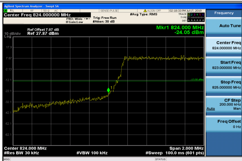
Band26-1.4MHz-QPSK-26797-6RB#0
