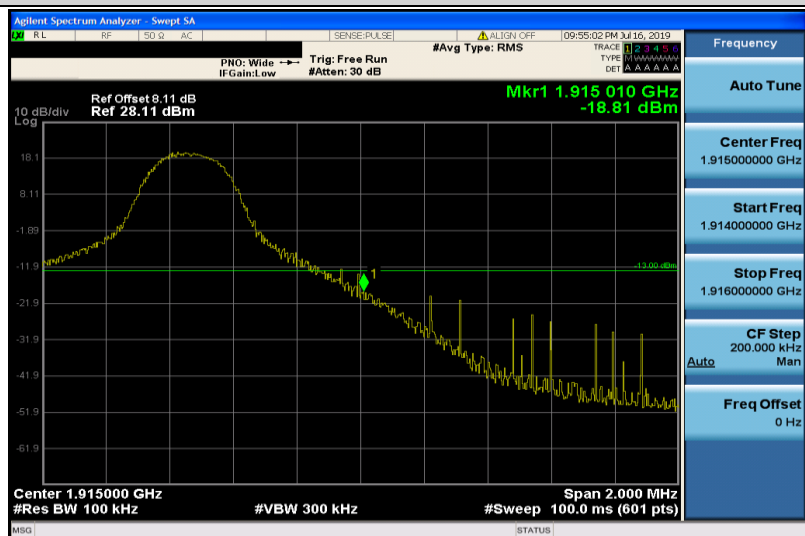
Band25-5MHz-16QAM-26665-1RB#24
