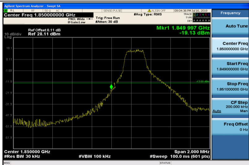
Band25-3MHz-16QAM-26055-1RB#0
