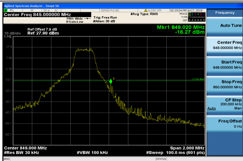
Band26-1.4MHz-16QAM-27033-1RB#5
