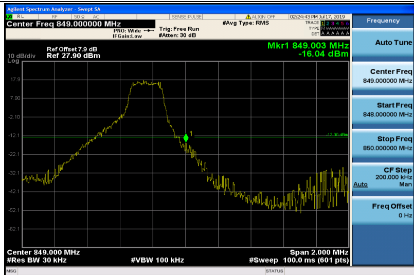
Band26-3MHz-16QAM-27025-1RB#14
