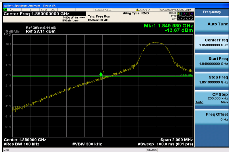
Band25-10MHz-QPSK-26090-1RB#0
