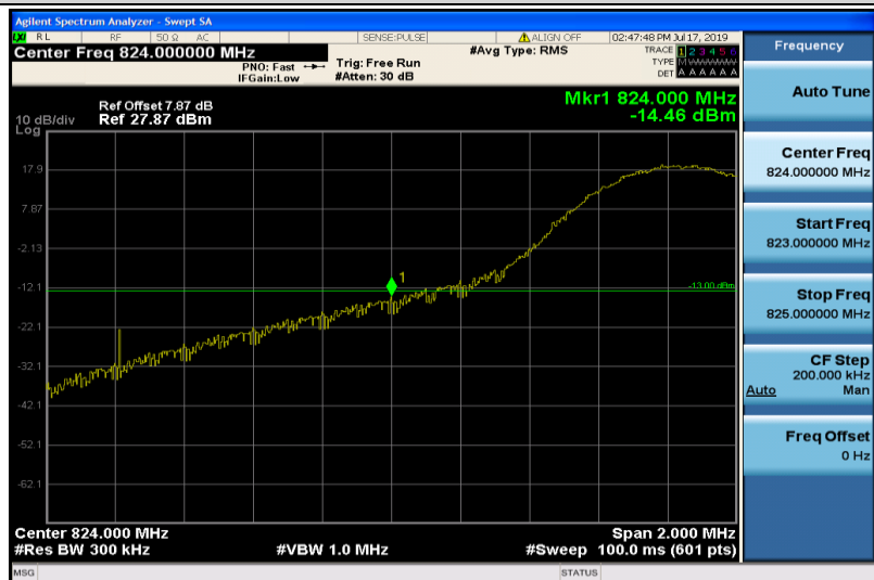
Band26-15MHz-16QAM-26915-1RB#0
