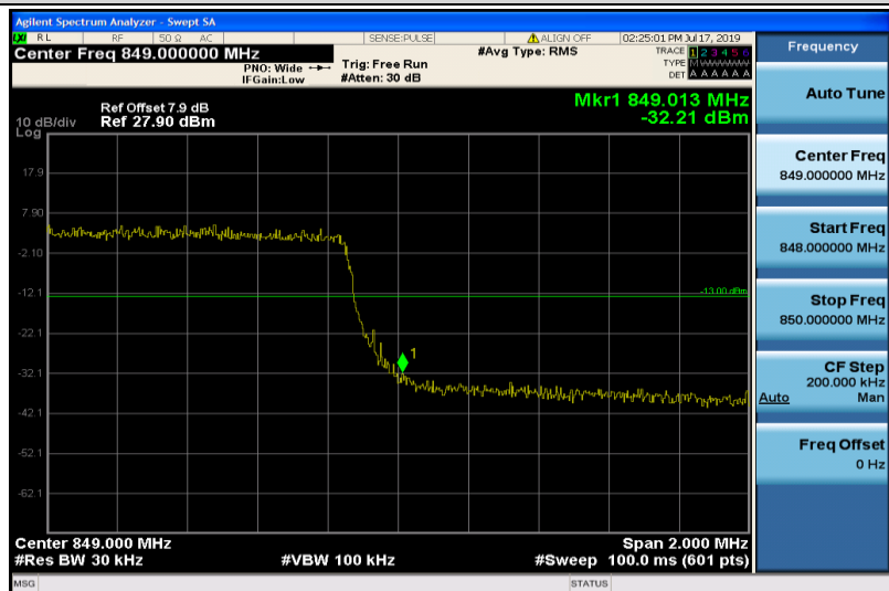
Band26-3MHz-16QAM-27025-15RB#0
