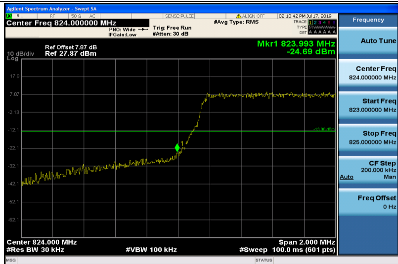
Band26-1.4MHz-16QAM-26797-6RB#0
