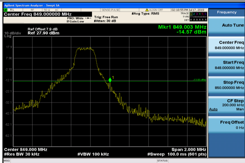
Band26-1.4MHz-QPSK-27033-1RB#5
