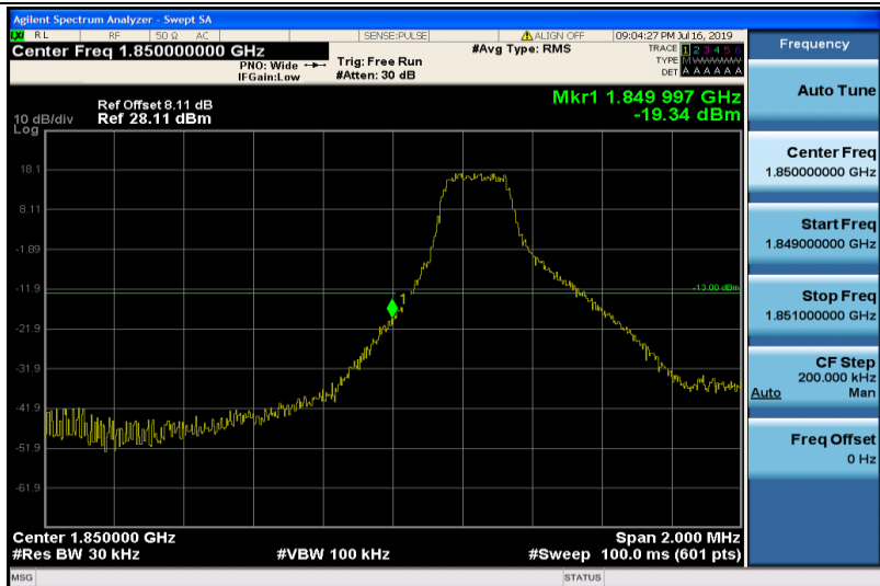
Band25-3MHz-QPSK-26055-1RB#0
