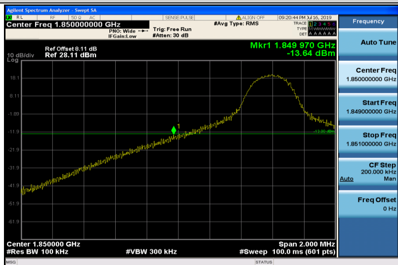
Band25-10MHz-16QAM-26090-1RB#0
