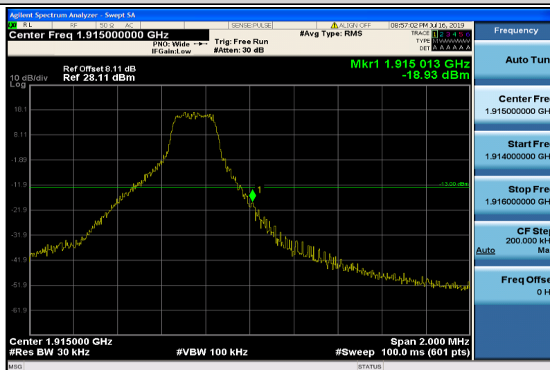
Band25-1.4MHz-16QAM-26683-1RB#5
