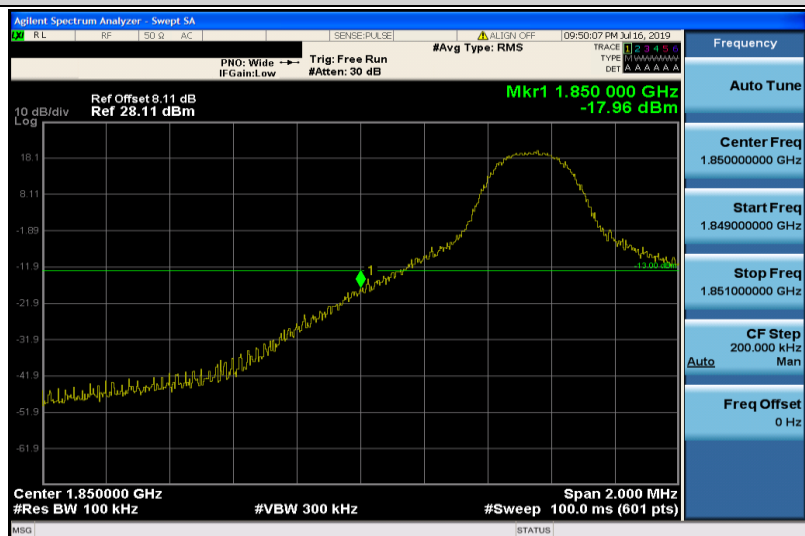
Band25-5MHz-QPSK-26065-1RB#0
