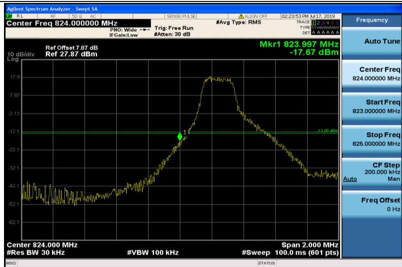
Band26-3MHz-QPSK-26805-1RB#0
