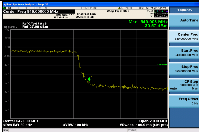
Band26-3MHz-QPSK-27025-15RB#0
