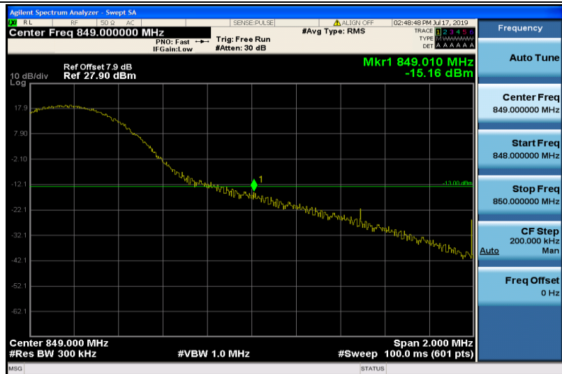
Band26-15MHz-16QAM-26965-1RB#74
