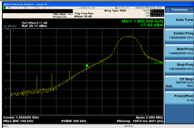
Band25-5MHz-16QAM-26065-1RB#0
