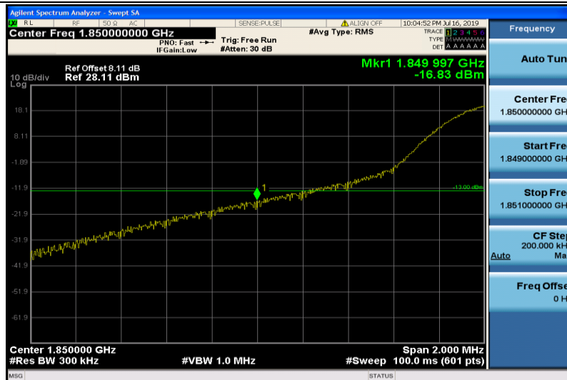
Band25-20MHz-16QAM-26140-1RB#0
