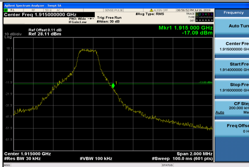
Band25-1.4MHz-QPSK-26683-1RB#5
