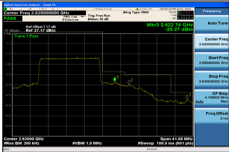
Band38-15MHz-16QAM-38175-75RB#0
