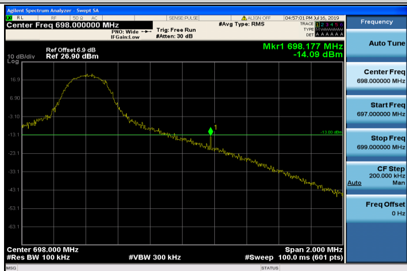
Band71-10MHz-16QAM-133422-1RB#49
