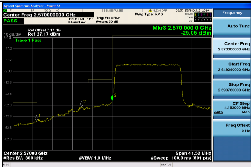
Band38-15MHz-16QAM-37825-75RB#0
