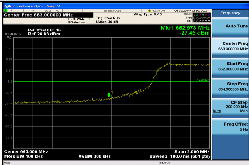
Band71-10MHz-16QAM-133172-50RB#0
