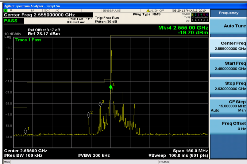
Band41-10MHz-16QAM-40290-1RB#0
