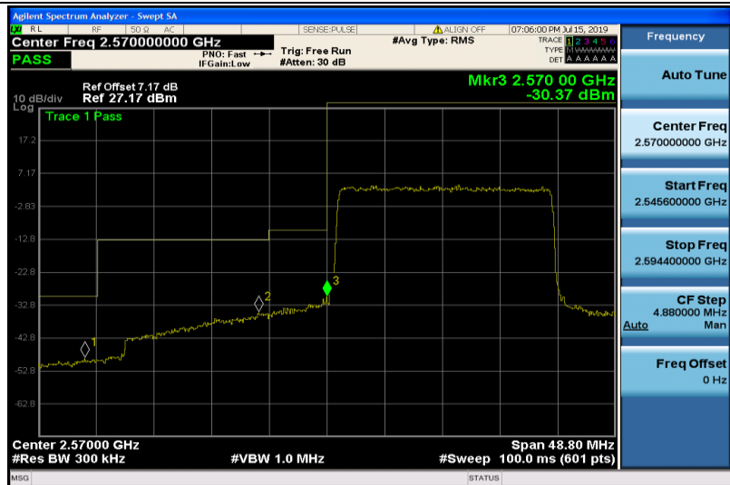
Band38-20MHz-QPSK-37850-100RB#0
