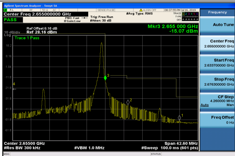
Band41-15MHz-QPSK-41165-1RB#74
