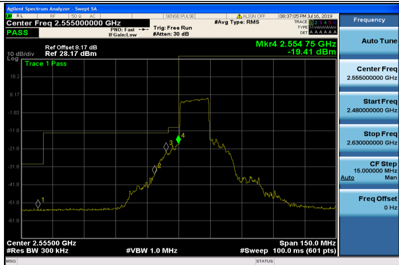
Band41-15MHz-QPSK-40315-75RB#0
