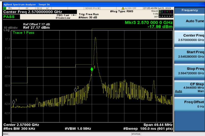
Band38-20MHz-16QAM-37850-1RB#0
