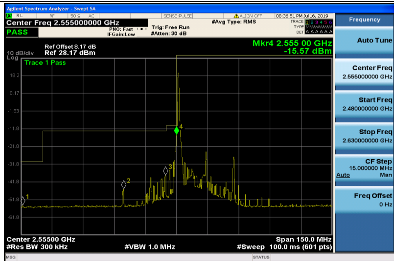
Band41-15MHz-16QAM-40315-1RB#0
