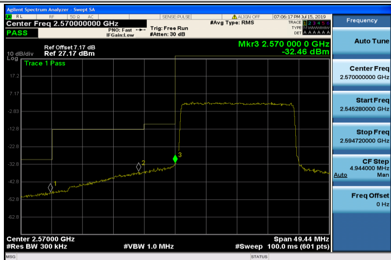
Band38-20MHz-16QAM-37850-100RB#0
