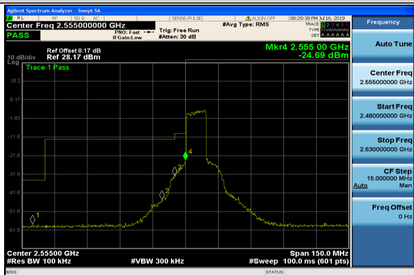
Band41-10MHz-16QAM-40290-50RB#0
