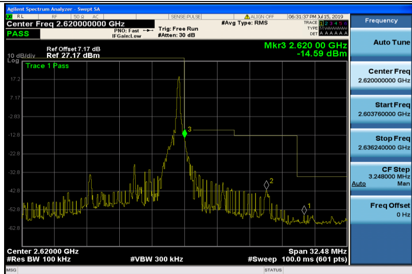
Band38-10MHz-QPSK-38200-1RB#49
