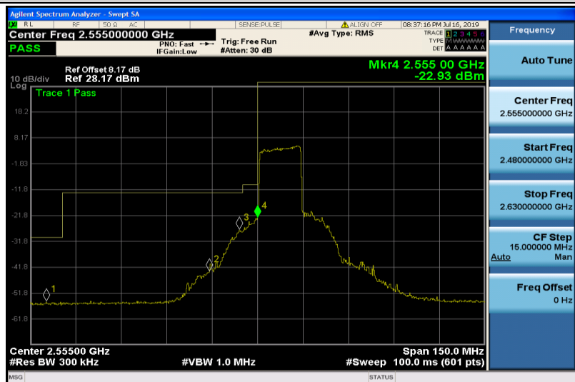
Band41-15MHz-16QAM-40315-75RB#0
