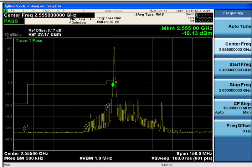
Band41-20MHz-QPSK-40340-1RB#0
