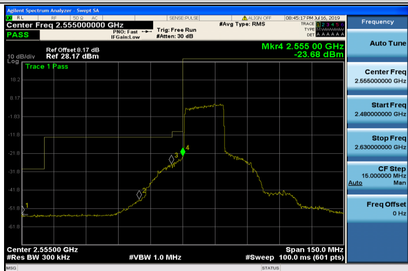
Band41-20MHz-QPSK-40340-100RB#0
