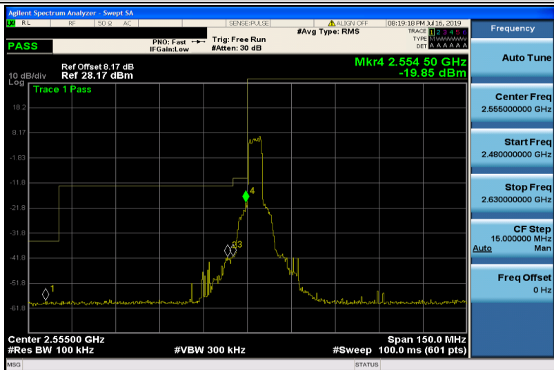
Band41-5MHz-QPSK-40265-25RB#0
