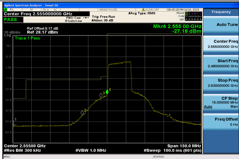
Band41-20MHz-16QAM-40340-100RB#0
