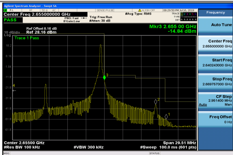
Band41-10MHz-QPSK-41190-1RB#49
