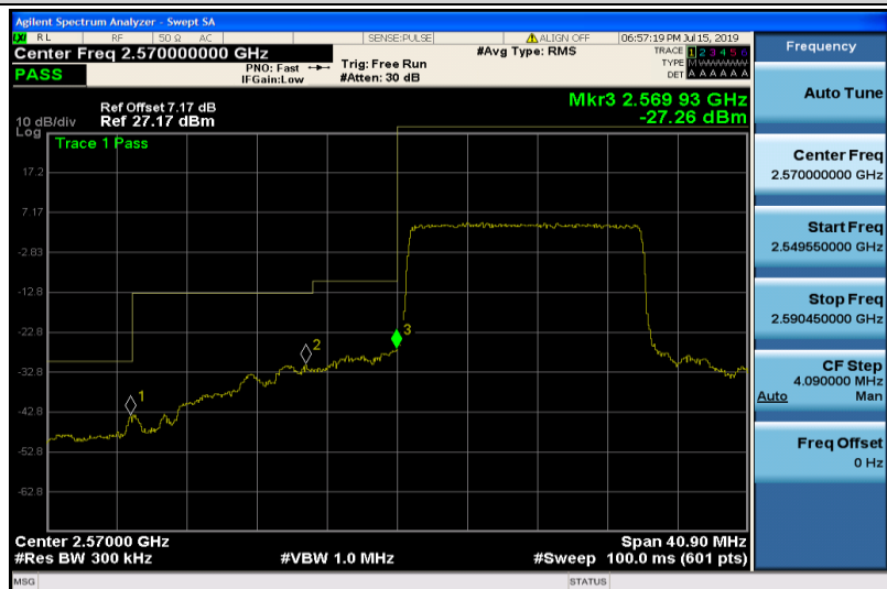
Band38-15MHz-QPSK-37825-75RB#0
