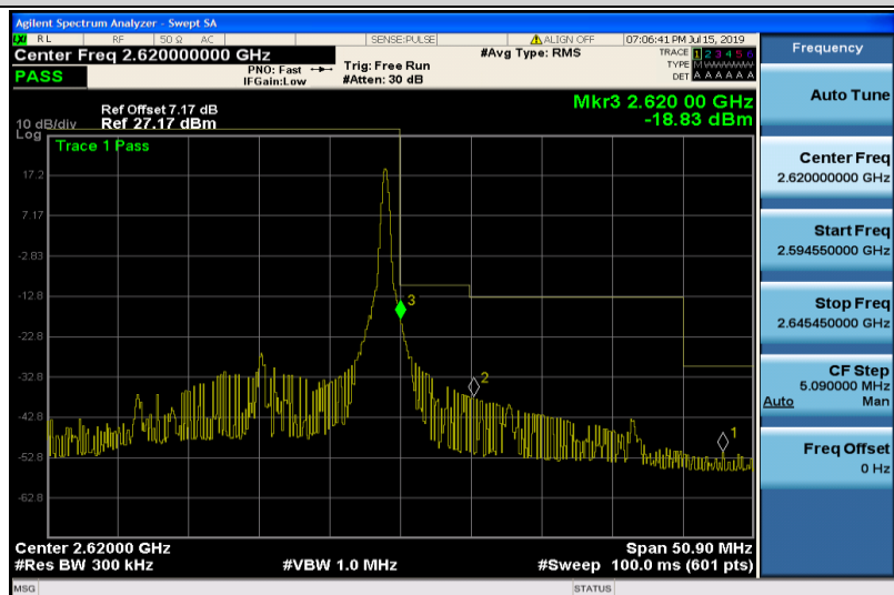
Band38-20MHz-16QAM-38150-1RB#99
