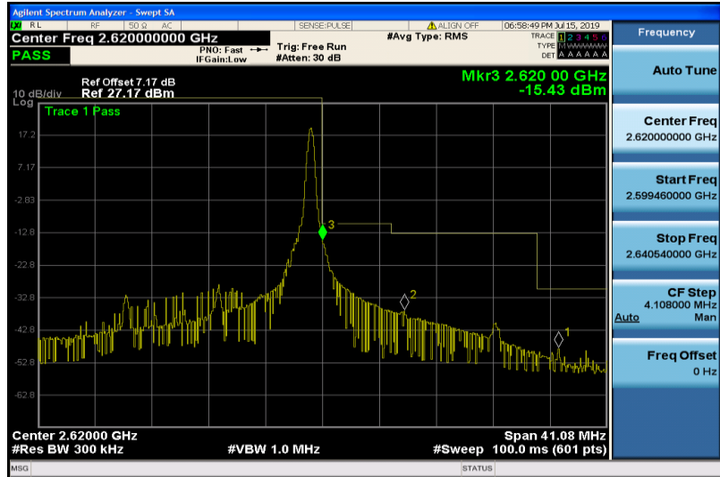
Band38-15MHz-16QAM-38175-1RB#74
