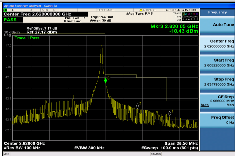
Band38-10MHz-16QAM-38200-1RB#49
