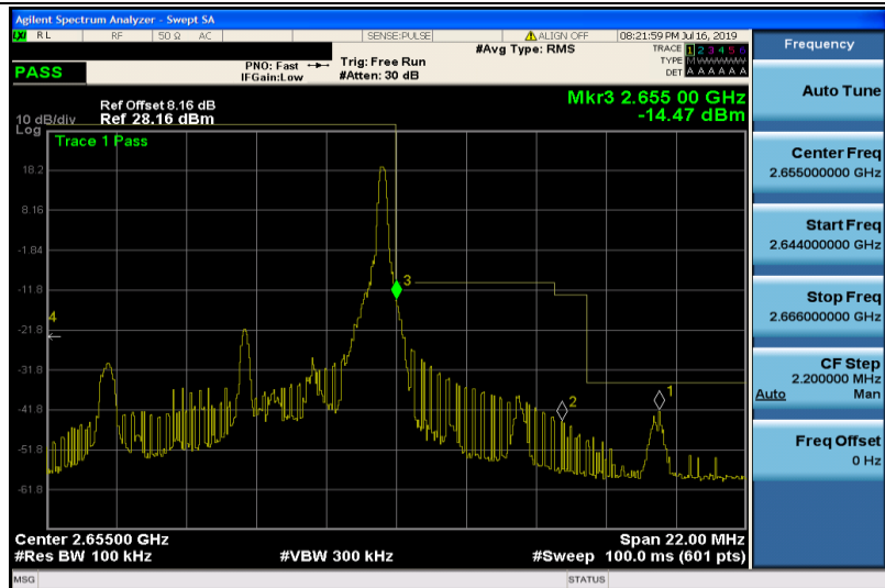
Band41-5MHz-QPSK-41215-1RB#24
