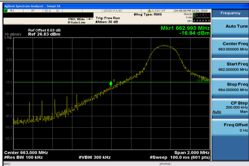
Band71-5MHz-16QAM-133147-1RB#0
