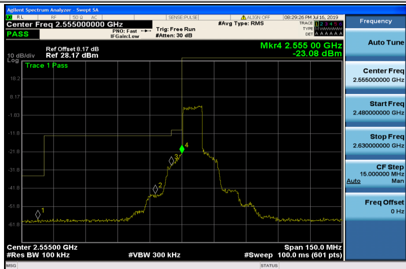
Band41-10MHz-QPSK-40290-50RB#0
