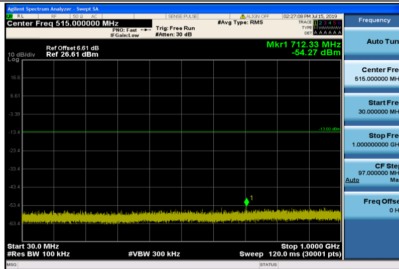
Band2-1.4MHz-QPSK-18607-1RB#0-Range1:30~1000MHz
