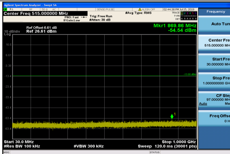
Band2-5MHz-16QAM-18625-1RB#0-Range1:30~1000MHz
