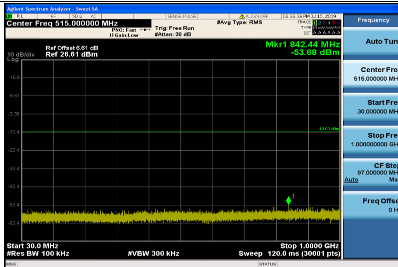
Band2-3MHz-QPSK-18615-1RB#0-Range1:30~1000MHz
