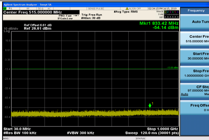
Band2-3MHz-16QAM-18615-1RB#0-Range1:30~1000MHz
