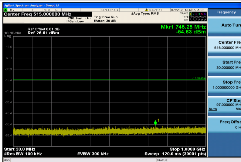
Band2-10MHz-16QAM-18650-1RB#0-Range1:30~1000MHz
