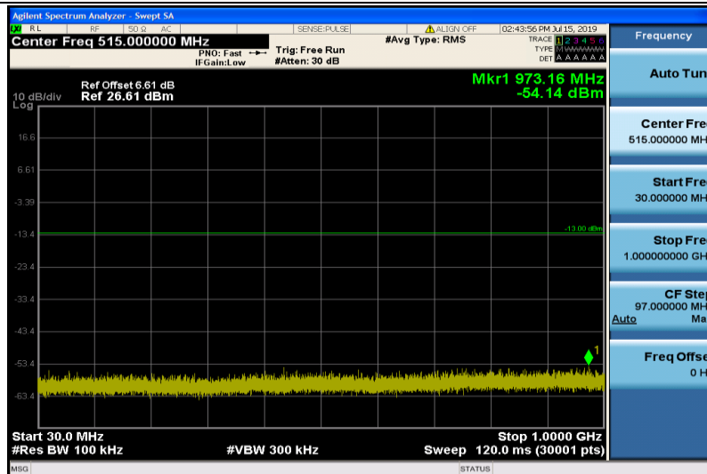
Band2-5MHz-QPSK-18625-1RB#0-Range1:30~1000MHz
