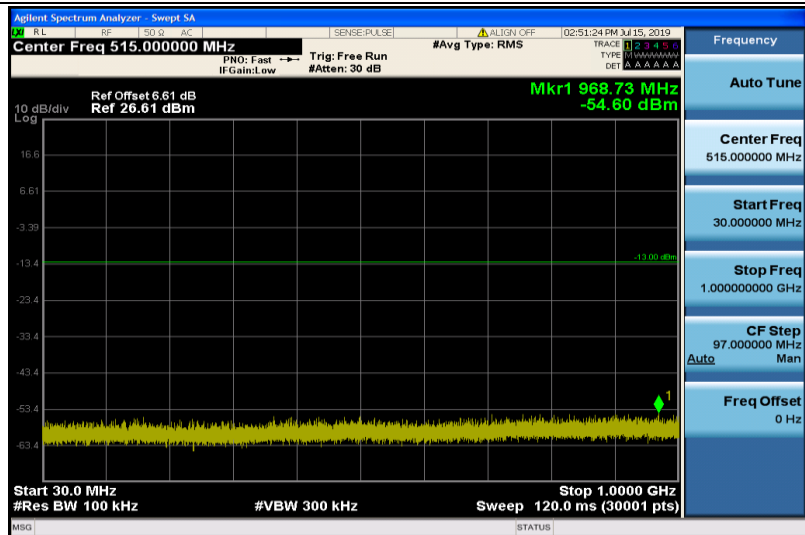
Band2-10MHz-QPSK-18650-1RB#0-Range1:30~1000MHz
