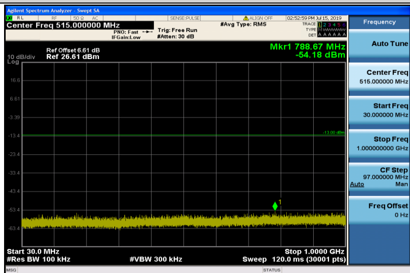
Band2-10MHz-QPSK-18900-1RB#0-Range1:30~1000MHz
