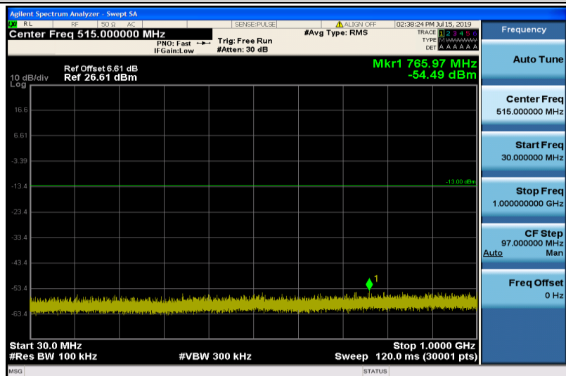
Band2-3MHz-16QAM-19185-1RB#0-Range1:30~1000MHz
