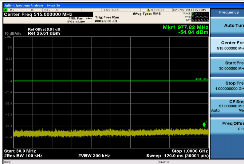
Band2-1.4MHz-16QAM-18607-1RB#0-Range1:30~1000MHz
