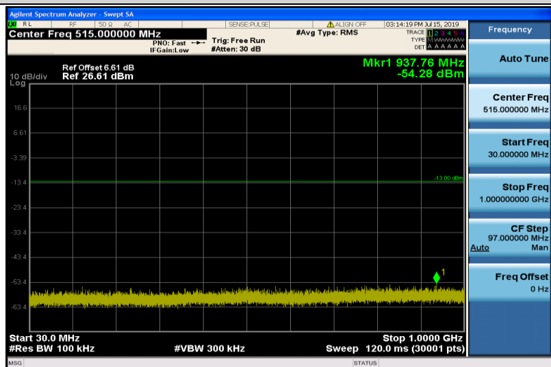
Band2-20MHz-16QAM-18900-1RB#0-Range1:30~1000MHz
