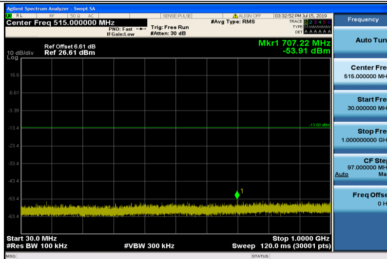
Band4-3MHz-16QAM-19965-1RB#0-Range1:30~1000MHz
