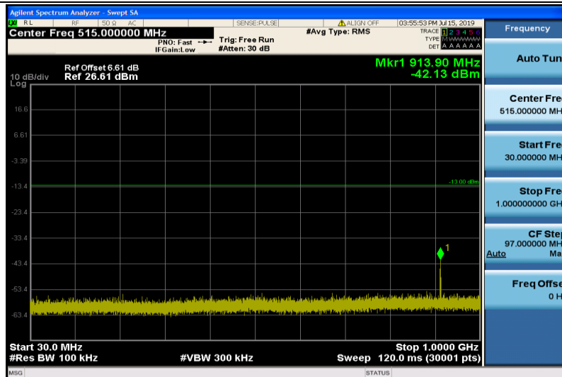
Band4-20MHz-QPSK-20050-1RB#0-Range1:30~1000MHz
