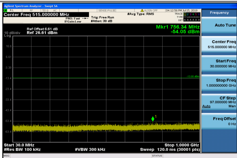
Band4-10MHz-16QAM-20175-1RB#0-Range1:30~1000MHz
