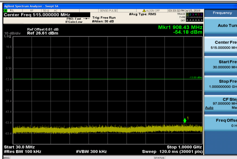
Band4-3MHz-QPSK-20175-1RB#0-Range1:30~1000MHz
