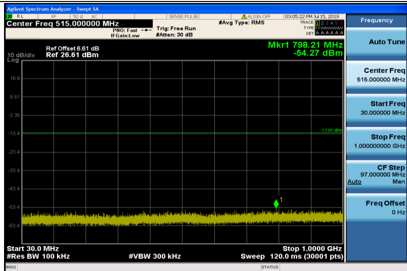
Band2-15MHz-16QAM-18675-1RB#0-Range1:30~1000MHz
