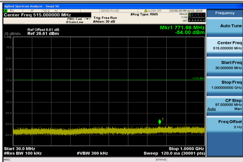
Band4-15MHz-QPSK-20175-1RB#0-Range1:30~1000MHz
