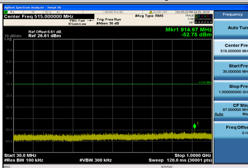
Band4-1.4MHz-16QAM-20175-1RB#0-Range1:30~1000MHz
