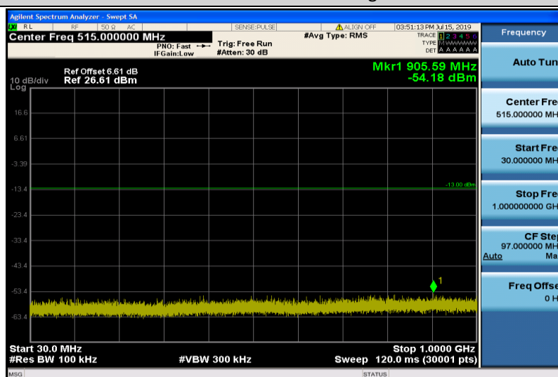
Band4-15MHz-16QAM-20175-1RB#0-Range1:30~1000MHz
