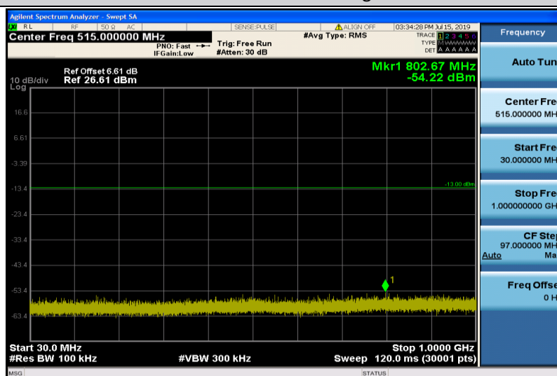
Band4-3MHz-16QAM-20175-1RB#0-Range1:30~1000MHz
