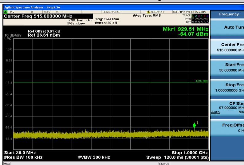
Band4-1.4MHz-QPSK-20175-1RB#0-Range1:30~1000MHz
