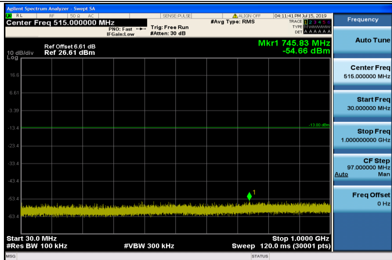
Band4-10MHz-16QAM-20000-1RB#0-Range1:30~1000MHz
