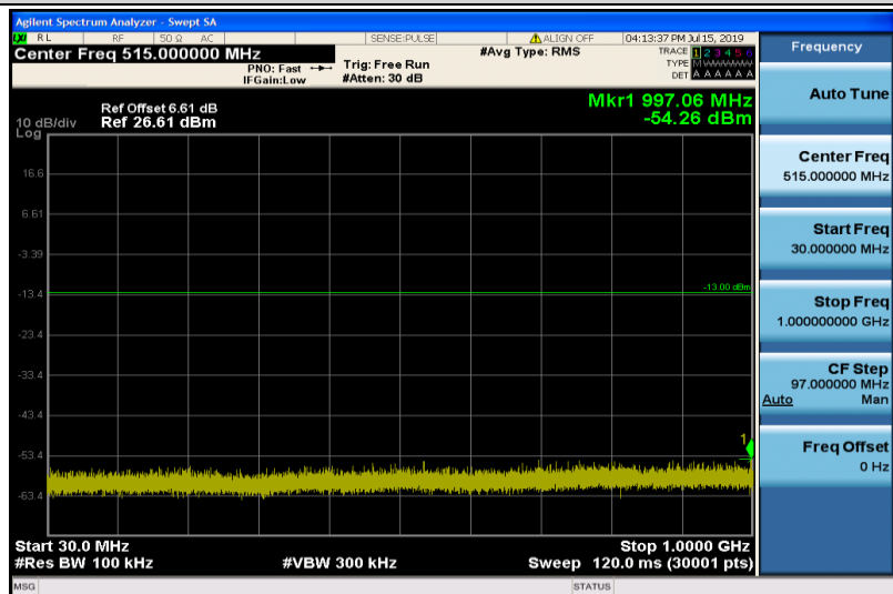
Band4-10MHz-QPSK-20350-1RB#0-Range1:30~1000MHz
