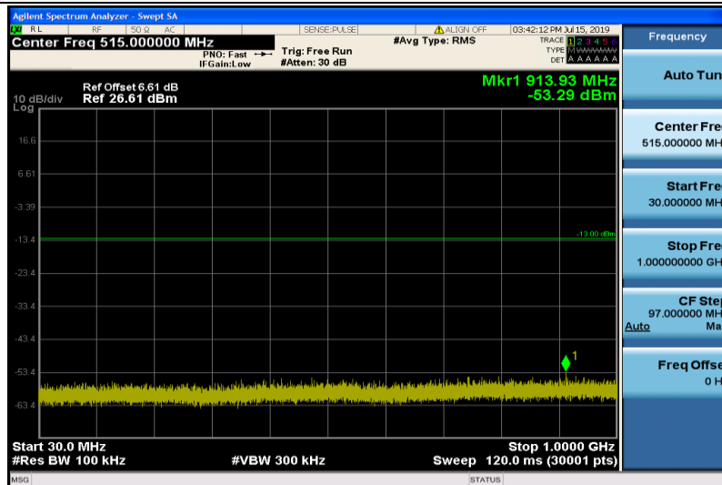
Band4-5MHz-QPSK-19975-1RB#0-Range1:30~1000MHz
