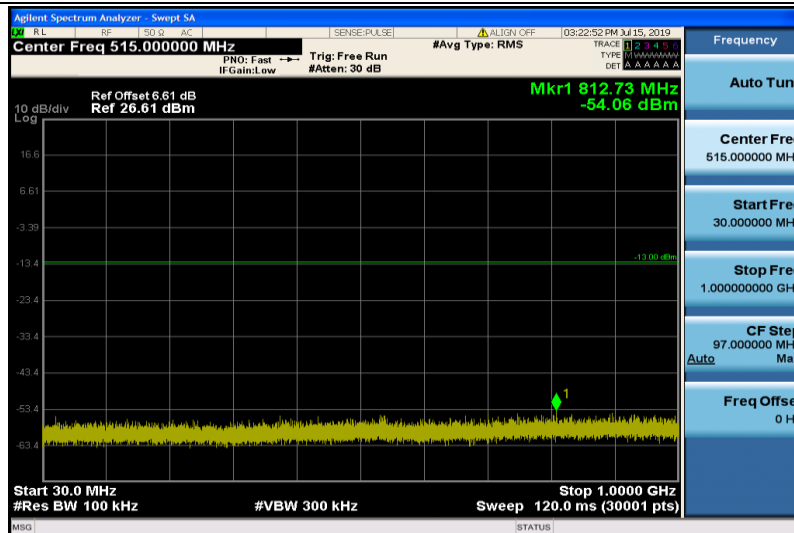
Band4-1.4MHz-QPSK-19957-1RB#0-Range1:30~1000MHz
