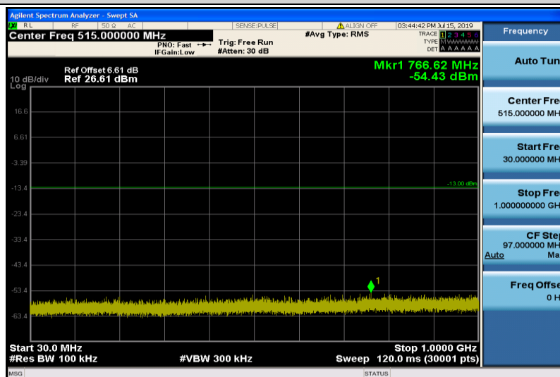
Band4-5MHz-QPSK-20375-1RB#0-Range1:30~1000MHz
