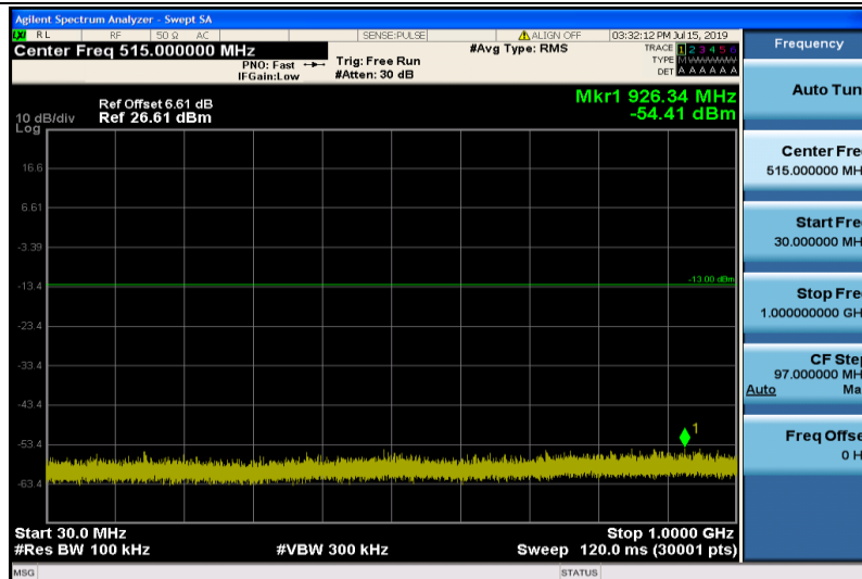
Band4-3MHz-QPSK-19965-1RB#0-Range1:30~1000MHz
