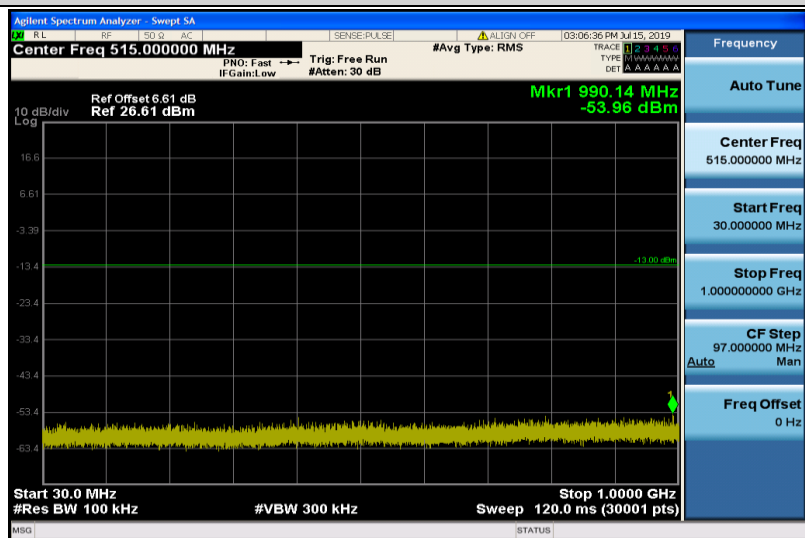
Band2-15MHz-16QAM-18900-1RB#0-Range1:30~1000MHz
