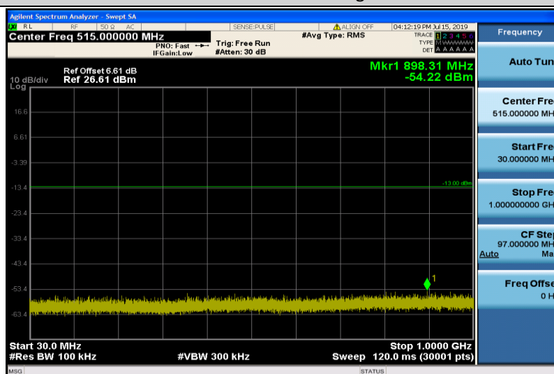
Band4-10MHz-QPSK-20175-1RB#0-Range1:30~1000MHz
