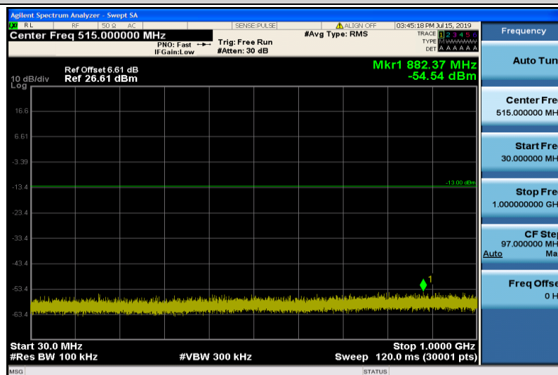
Band4-5MHz-16QAM-20375-1RB#0-Range1:30~1000MHz
