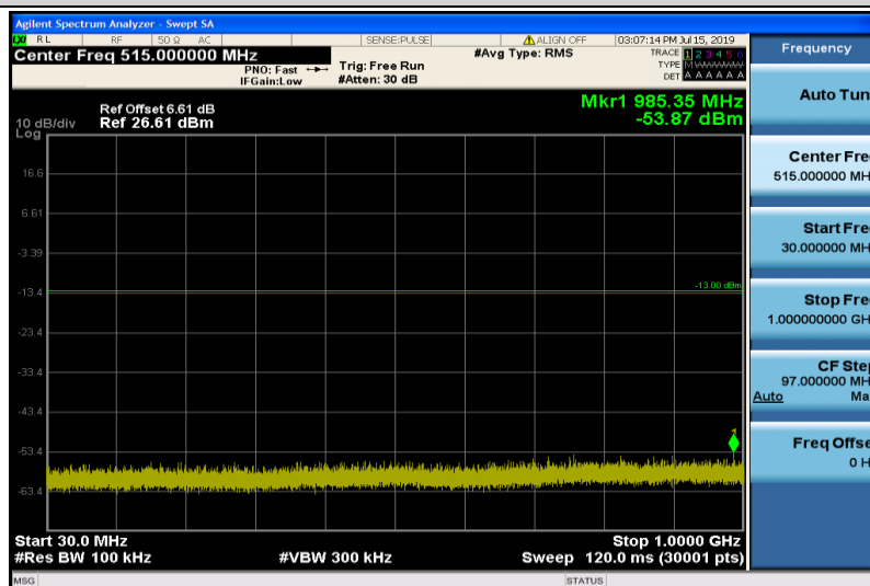
Band2-15MHz-QPSK-19125-1RB#0-Range1:30~1000MHz
