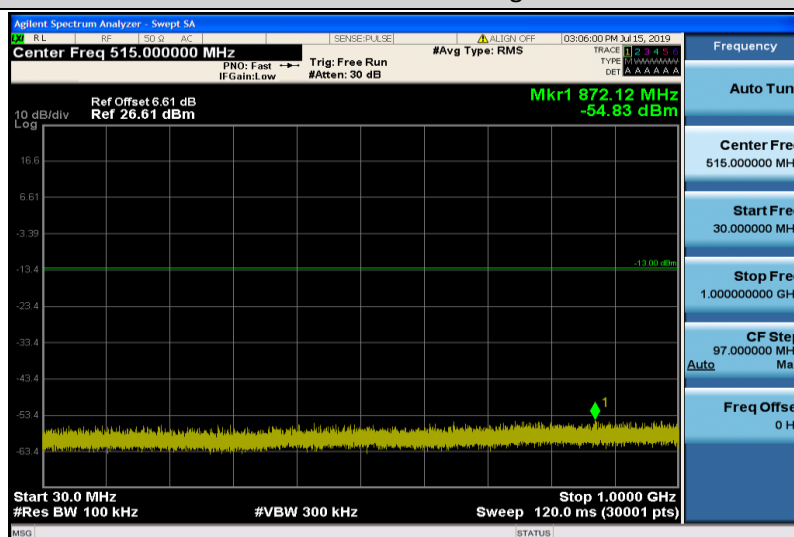
Band2-15MHz-QPSK-18900-1RB#0-Range1:30~1000MHz
