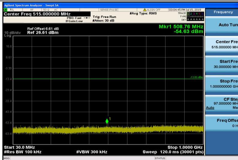
Band2-15MHz-QPSK-18675-1RB#0-Range1:30~1000MHz
