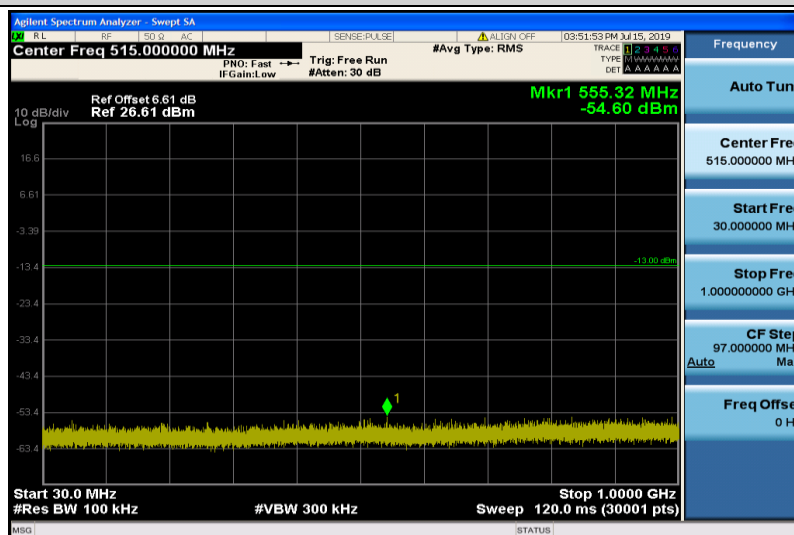
Band4-15MHz-QPSK-20325-1RB#0-Range1:30~1000MHz
