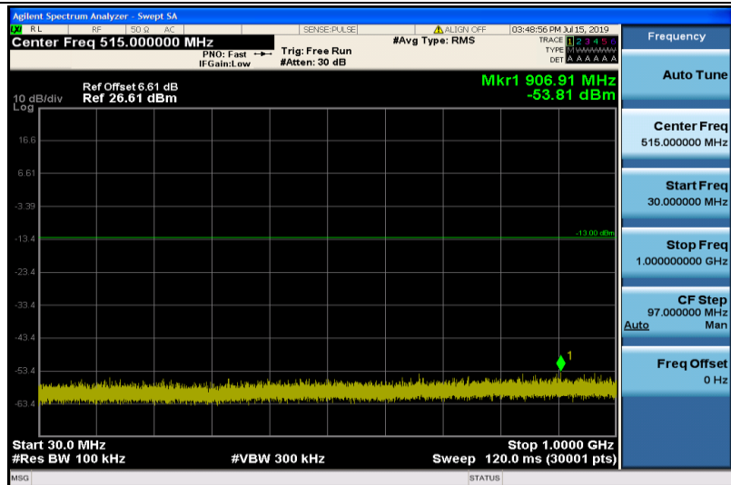
Band4-15MHz-QPSK-20025-1RB#0-Range1:30~1000MHz
