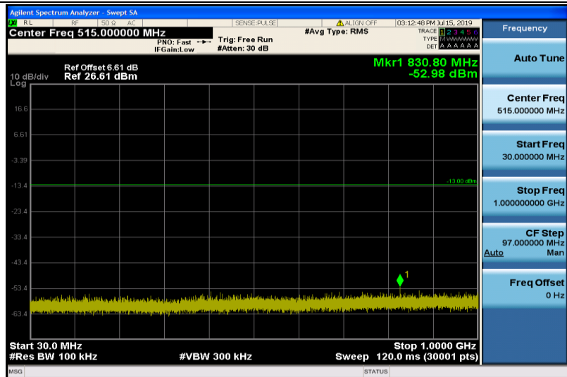
Band2-20MHz-16QAM-18700-1RB#0-Range1:30~1000MHz
