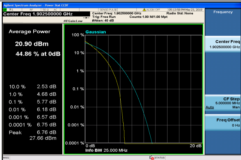
Band2-15MHz-QPSK-19125-75RB#0
