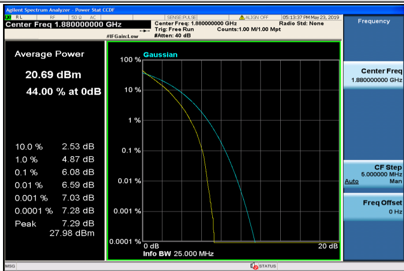
Band2-15MHz-QPSK-18900-75RB#0
