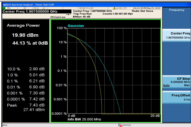
Band2-5MHz-16QAM-19175-25RB#0
