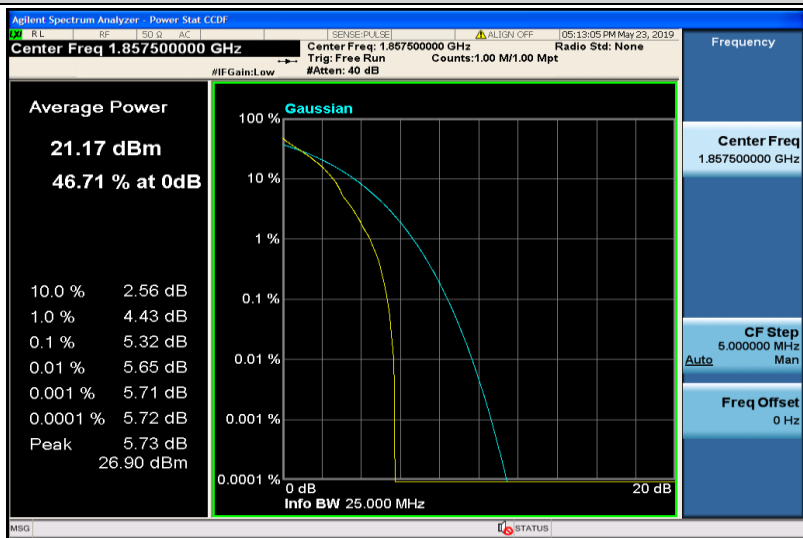
Band2-15MHz-QPSK-18675-1RB#0
