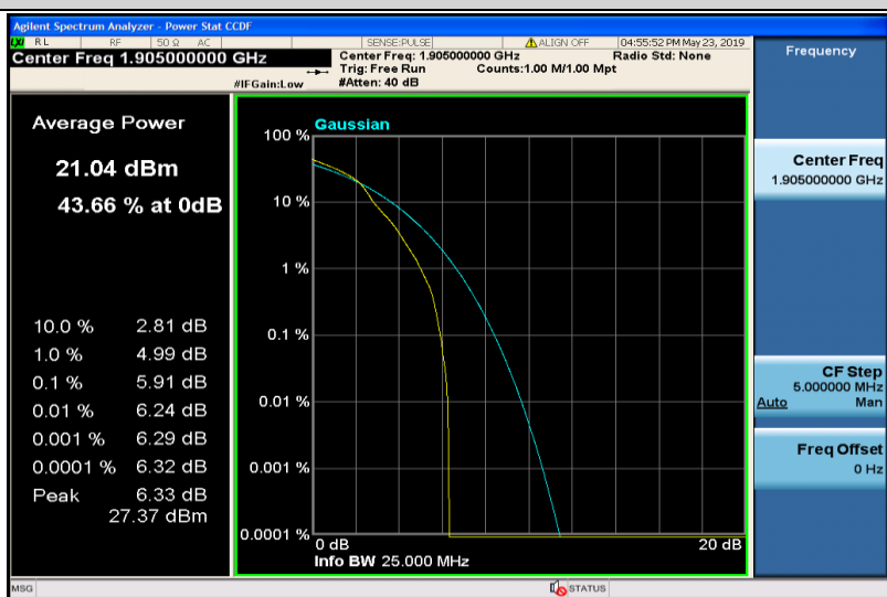
Band2-10MHz-16QAM-19150-1RB#0
