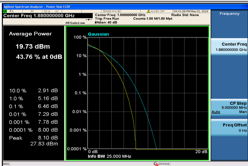
Band2-5MHz-16QAM-18900-25RB#0
