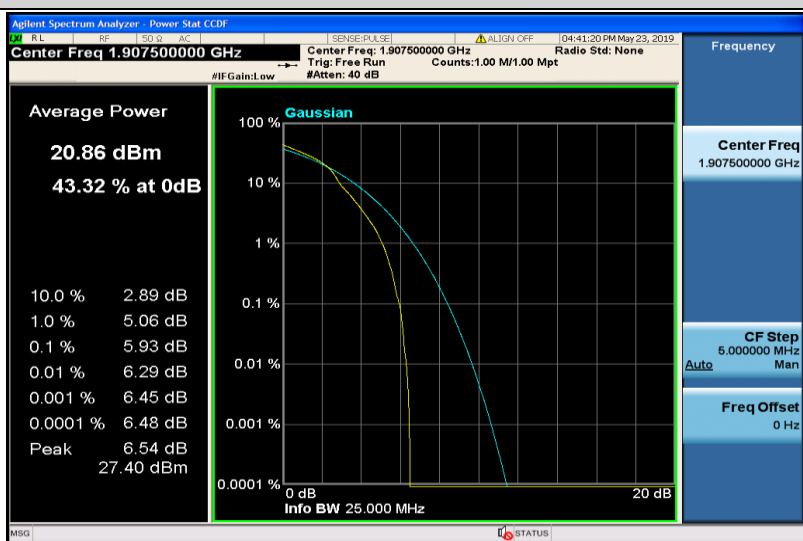
Band2-5MHz-16QAM-19175-1RB#0
