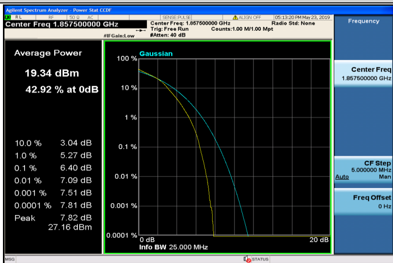
Band2-15MHz-16QAM-18675-75RB#0
