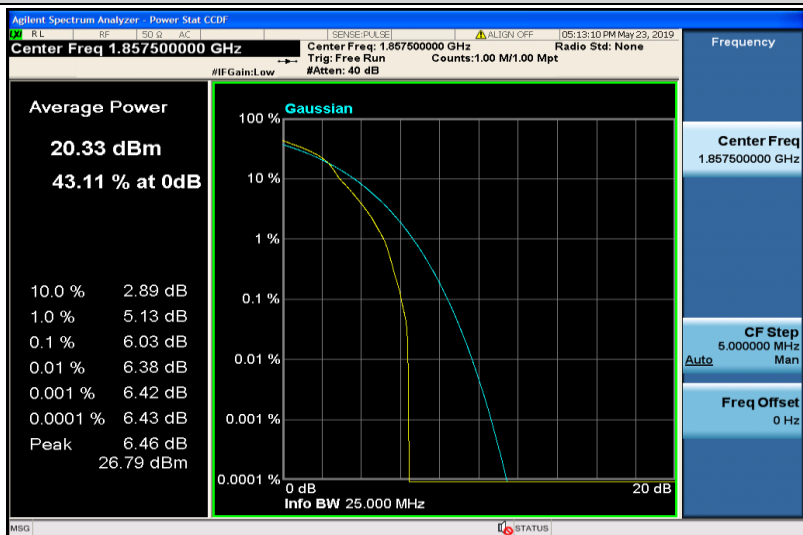
Band2-15MHz-16QAM-18675-1RB#0
