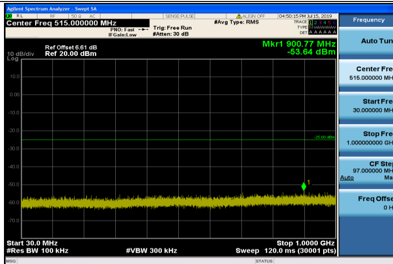
Band7-20MHz-QPSK-20850-1RB#0-Range1:30~1000MHz
