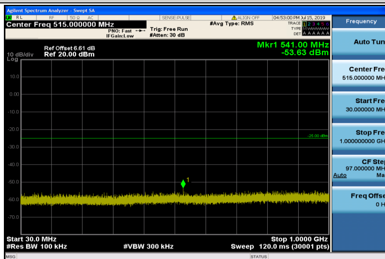
Band7-20MHz-QPSK-21350-1RB#0-Range1:30~1000MHz
