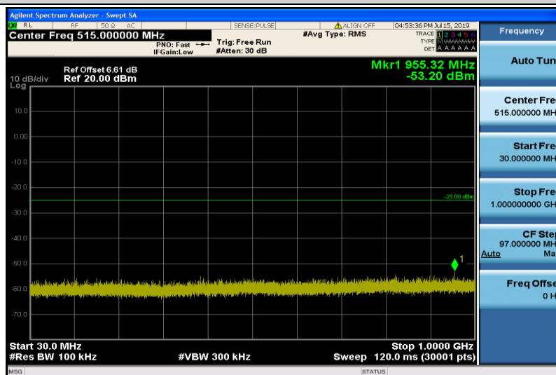
Band7-20MHz-16QAM-21350-1RB#0-Range1:30~1000MHz
