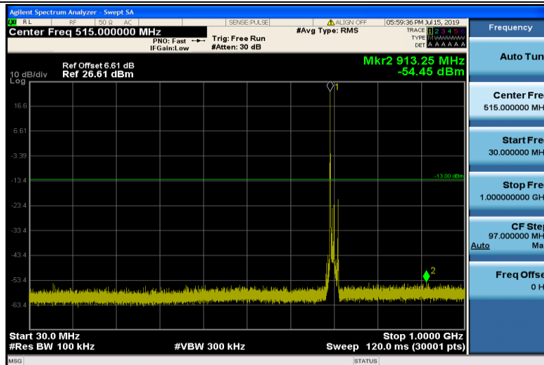
Band12-10MHz-16QAM-23060-1RB#0-Range1:30~1000MHz
