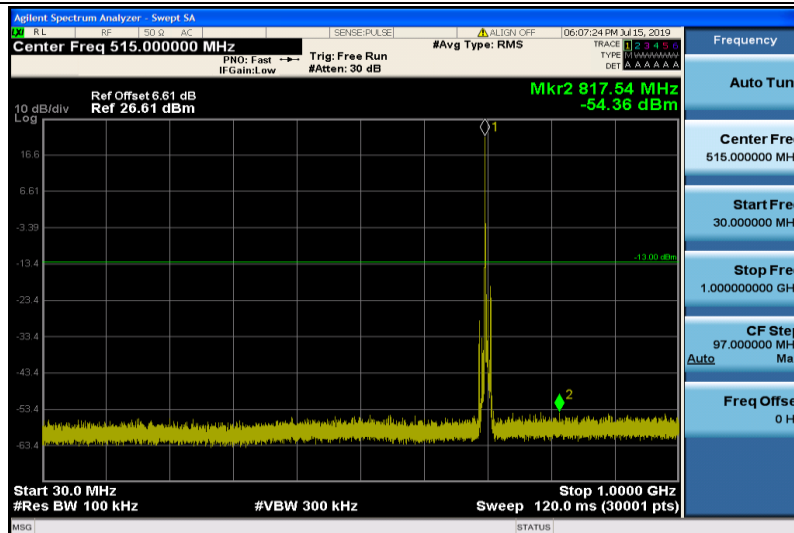
Band17-5MHz-QPSK-23755-1RB#0-Range1:30~1000MHz
