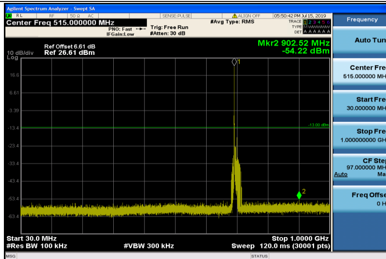
Band12-5MHz-QPSK-23035-1RB#0-Range1:30~1000MHz
