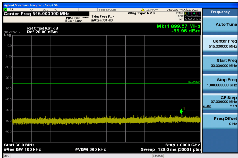
Band7-20MHz-16QAM-20850-1RB#0-Range1:30~1000MHz
