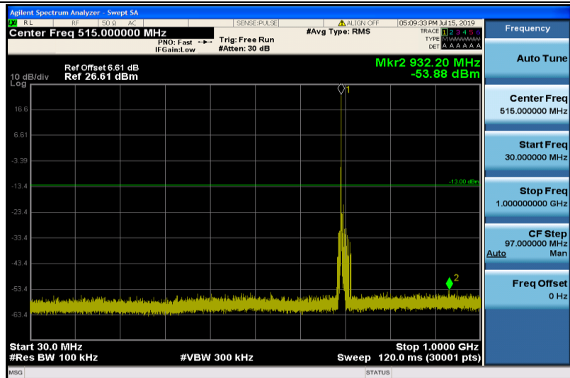
Band12-3MHz-QPSK-23025-1RB#0-Range1:30~1000MHz
