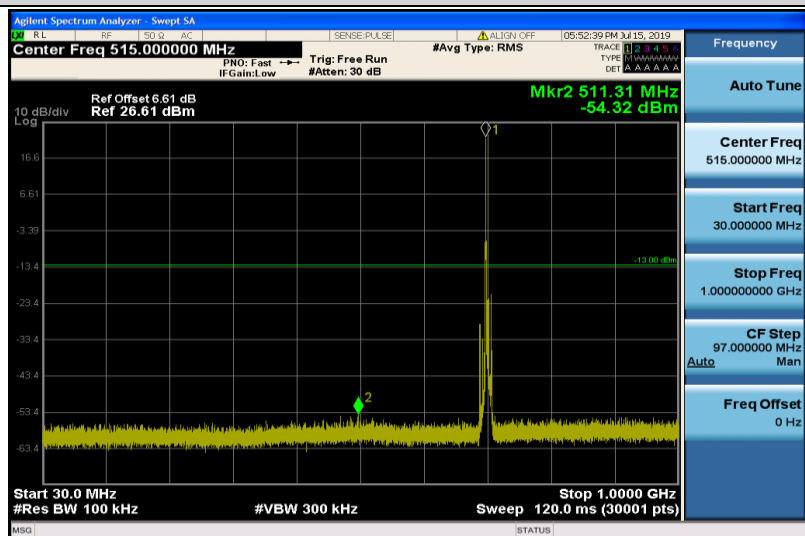
Band12-5MHz-16QAM-23095-1RB#0-Range1:30~1000MHz
