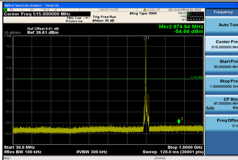
Band17-10MHz-QPSK-23780-1RB#0-Range1:30~1000MHz
