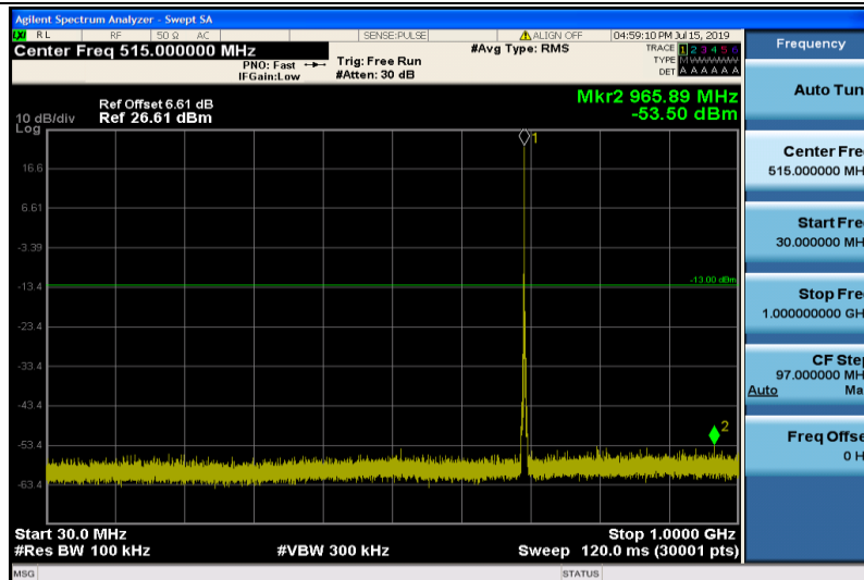
Band12-1.4MHz-16QAM-23017-1RB#0-Range1:30~1000MHz
