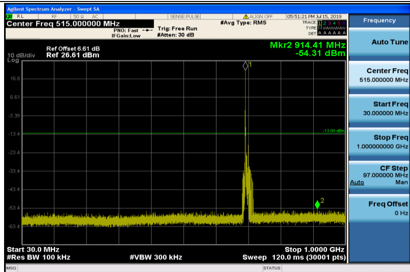
Band12-5MHz-16QAM-23035-1RB#0-Range1:30~1000MHz
