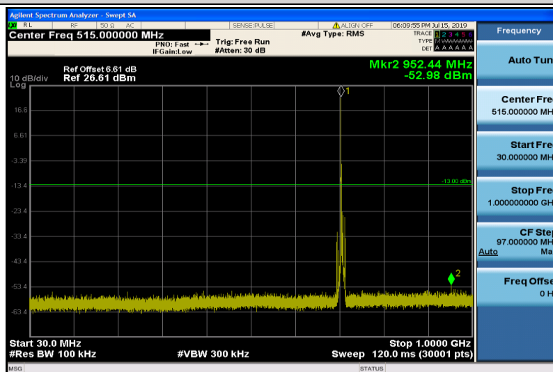
Band17-5MHz-QPSK-23825-1RB#0-Range1:30~1000MHz
