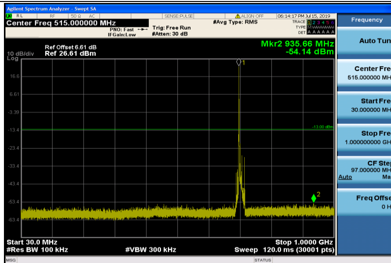
Band17-10MHz-16QAM-23780-1RB#0-Range1:30~1000MHz
