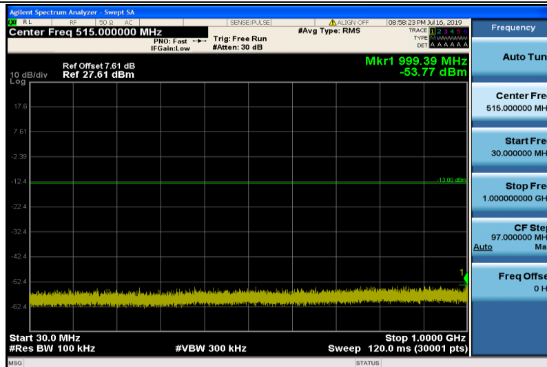
Band25-1.4MHz-QPSK-26047-1RB#0-30~1000MHz
