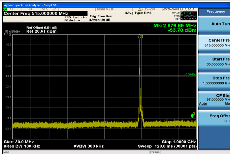
Band12-10MHz-QPSK-23060-1RB#0-Range1:30~1000MHz
