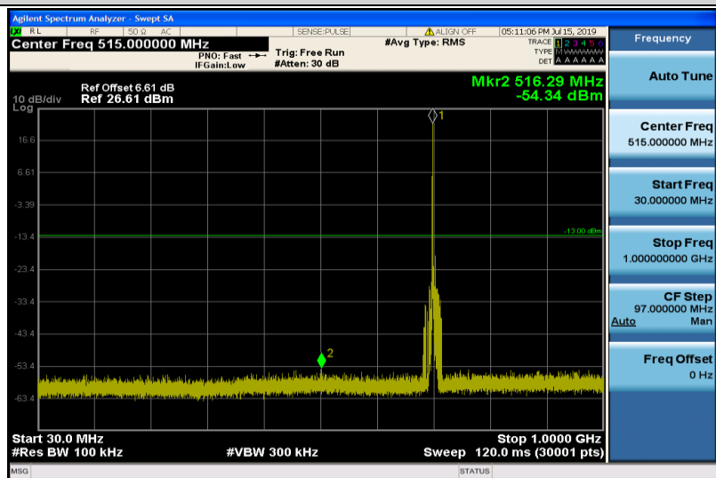
Band12-3MHz-QPSK-23095-1RB#0-Range1:30~1000MHz
