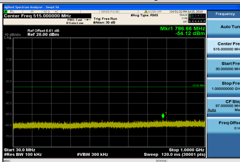
Band7-20MHz-QPSK-21100-1RB#0-Range1:30~1000MHz
