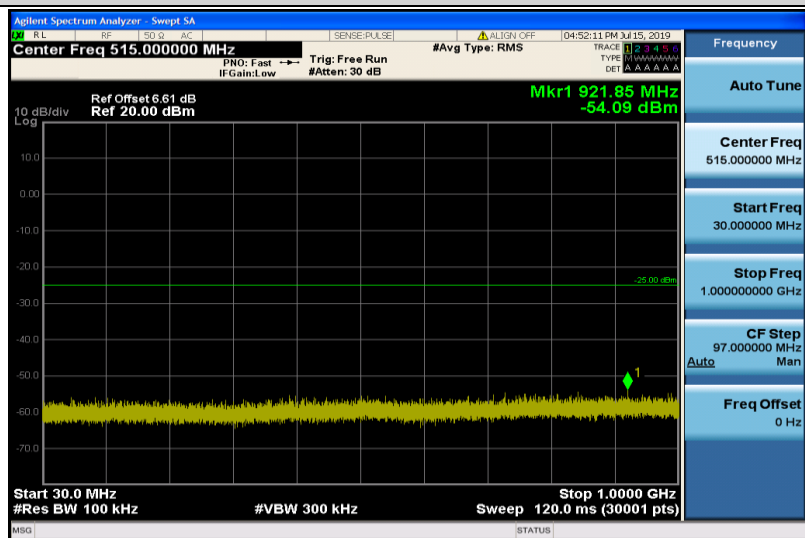
Band7-20MHz-16QAM-21100-1RB#0-Range1:30~1000MHz
