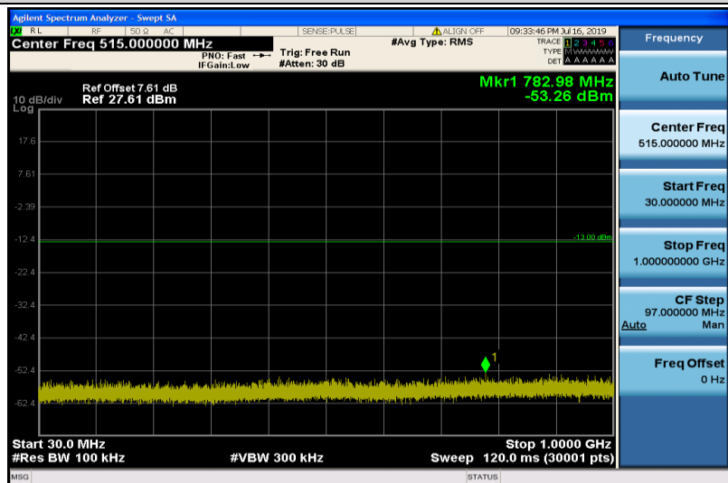
Band25-10MHz-QPSK-26640-1RB#0-30~1000MHz
