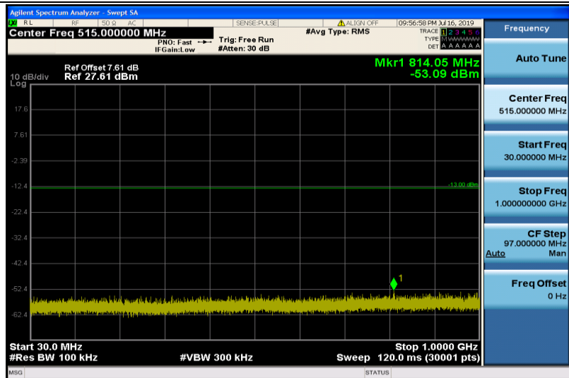
Band25-5MHz-16QAM-26065-1RB#0-30~1000MHz
