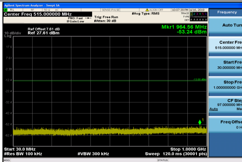
Band25-20MHz-16QAM-26140-1RB#0-30~1000MHz
