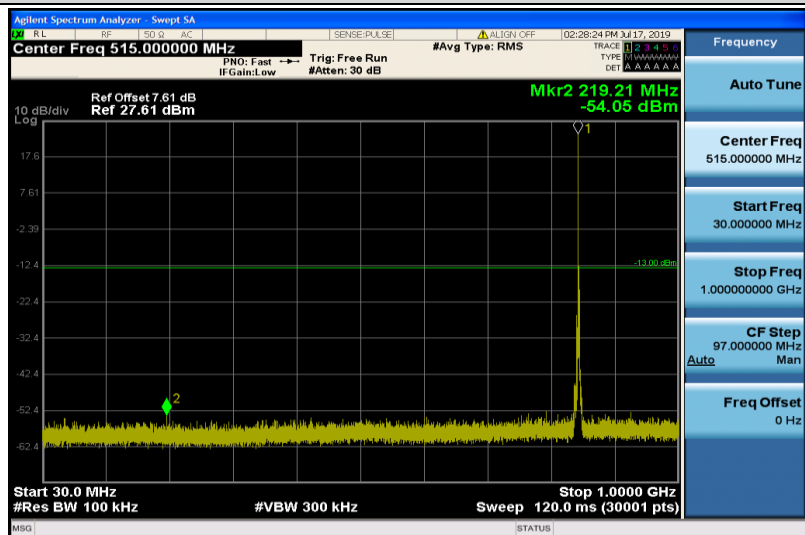
Band26-3MHz-16QAM-27025-1RB#0-30~1000MHz
