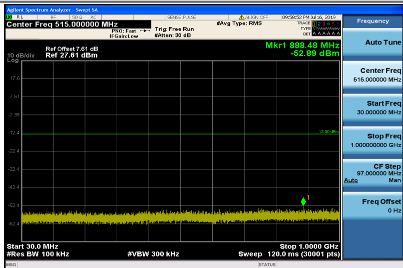
Band25-5MHz-QPSK-26665-1RB#0-30~1000MHz
