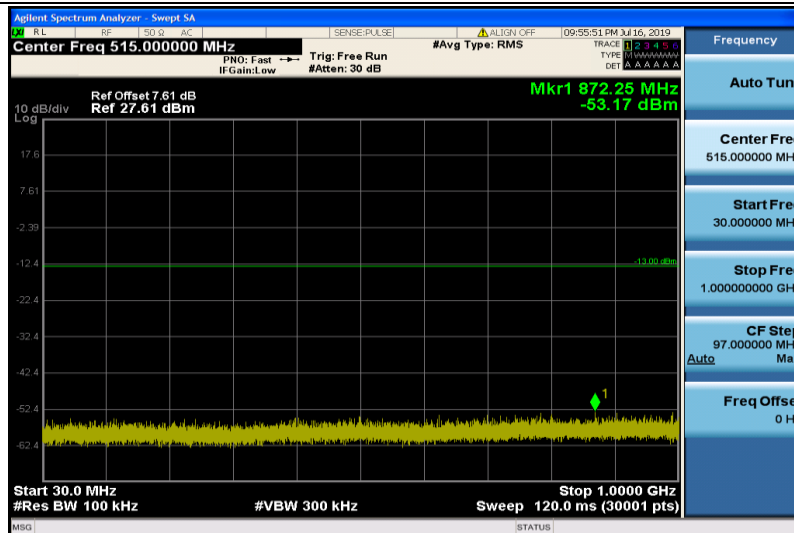
Band25-5MHz-QPSK-26065-1RB#0-30~1000MHz
