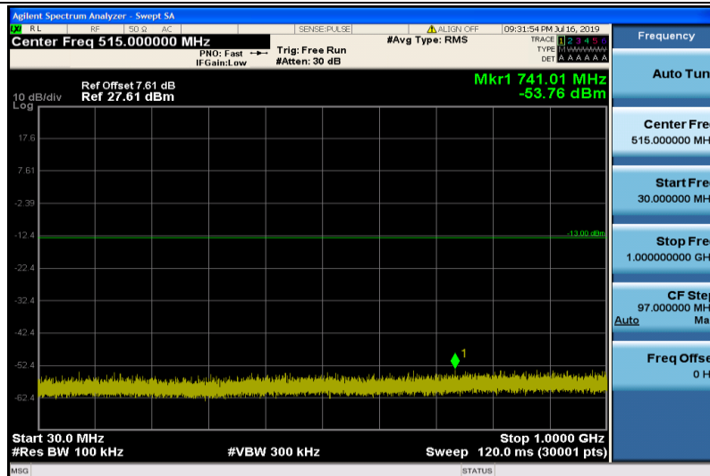
Band25-10MHz-16QAM-26090-1RB#0-30~1000MHz
