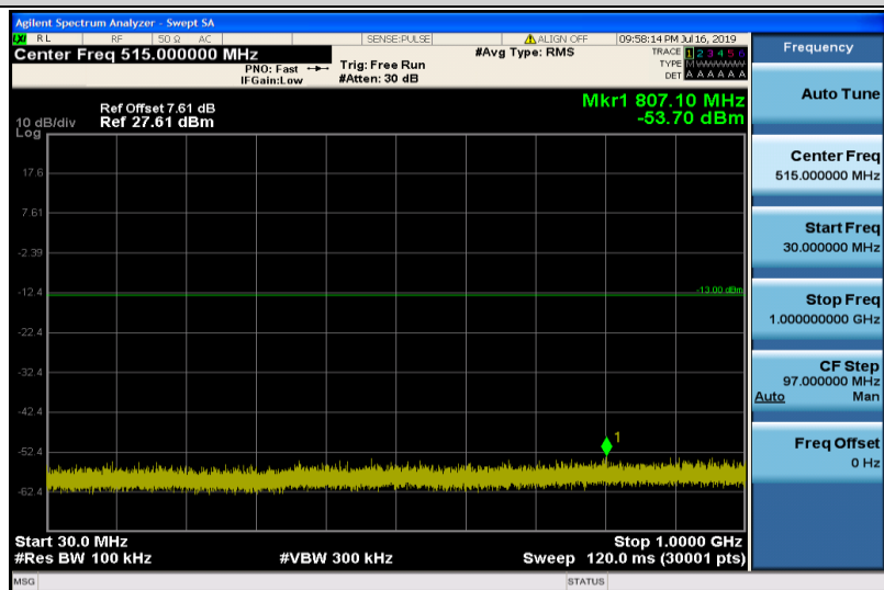
Band25-5MHz-16QAM-26365-1RB#0-30~1000MHz
