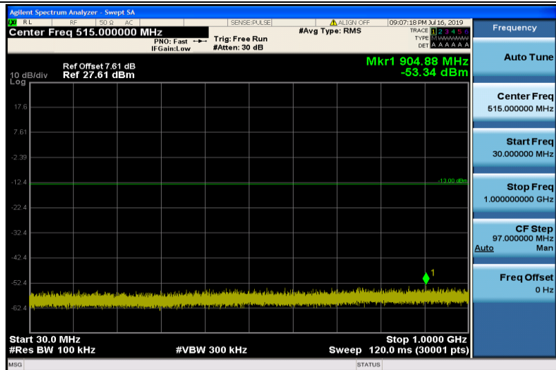
Band25-3MHz-16QAM-26055-1RB#0-30~1000MHz
