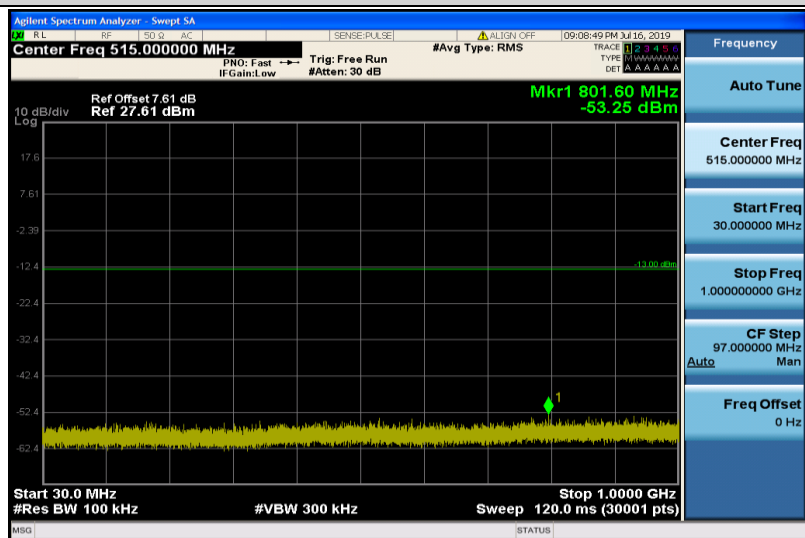
Band25-3MHz-16QAM-26365-1RB#0-30~1000MHz
