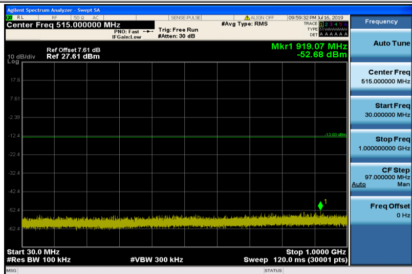
Band25-5MHz-16QAM-26665-1RB#0-30~1000MHz
