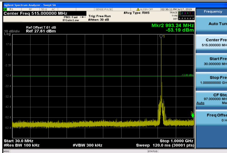
Band26-5MHz-QPSK-26815-1RB#0-30~1000MHz
