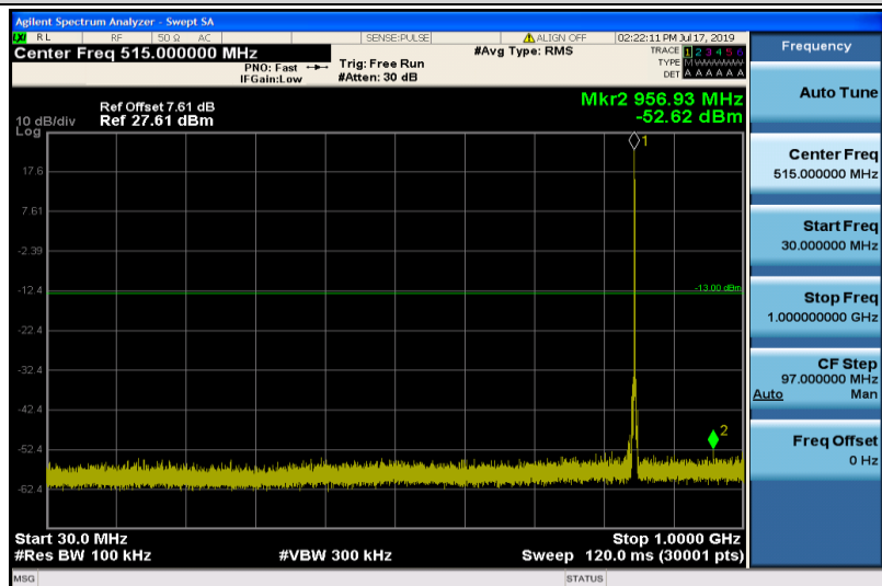
Band26-1.4MHz-QPSK-27033-1RB#0-30~1000MHz
