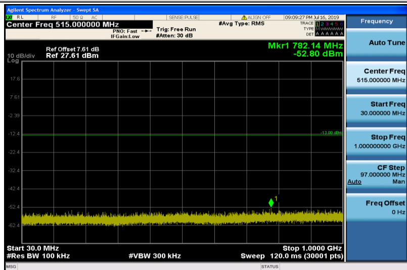
Band25-3MHz-QPSK-26675-1RB#0-30~1000MHz
