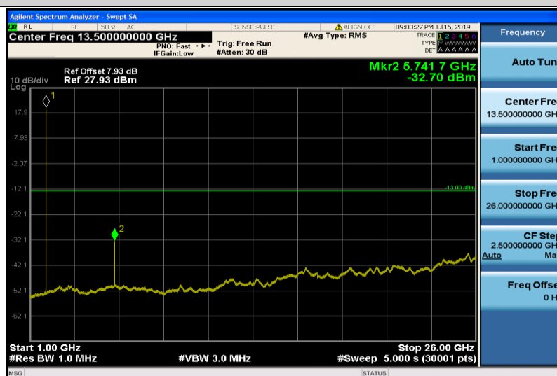
Band25-1.4MHz-16QAM-26683-1RB#0-1000~26000MHz
