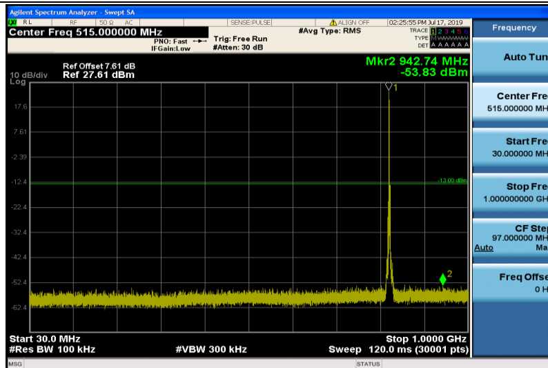
Band26-3MHz-16QAM-26805-1RB#0-30~1000MHz
