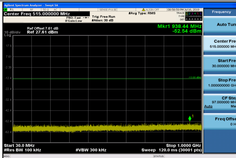
Band25-1.4MHz-16QAM-26047-1RB#0-30~1000MHz
