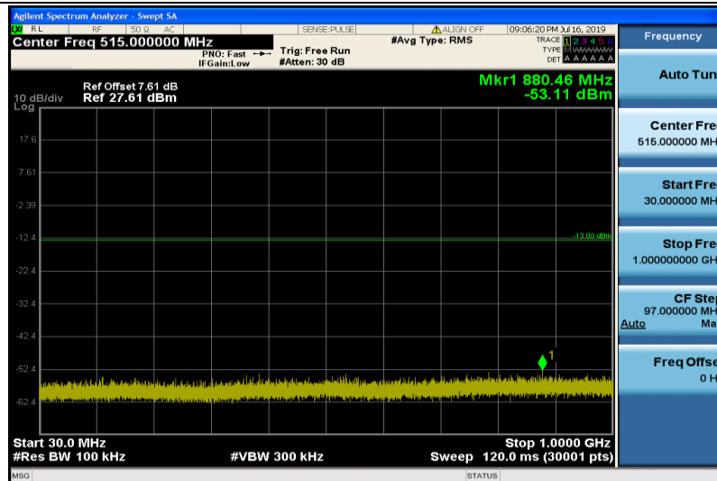
Band25-3MHz-QPSK-26055-1RB#0-30~1000MHz
