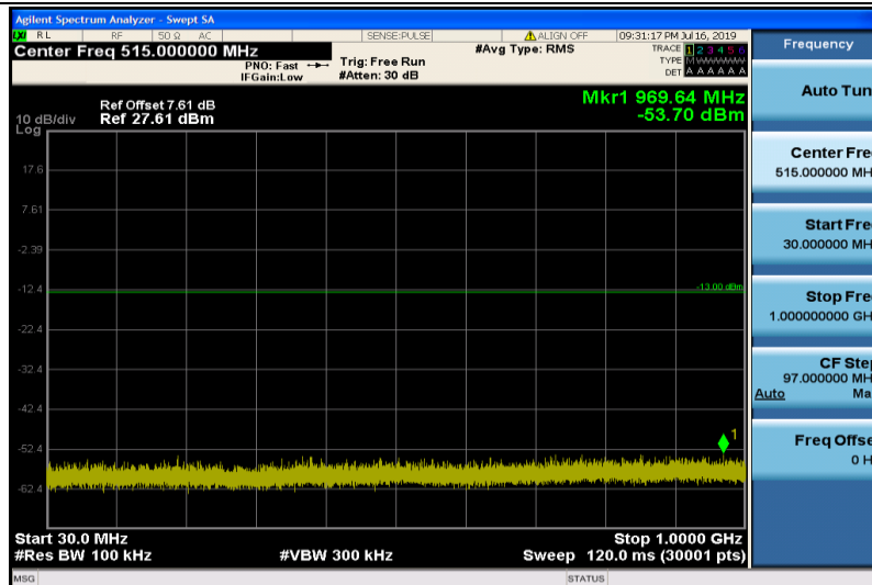
Band25-10MHz-QPSK-26090-1RB#0-30~1000MHz
