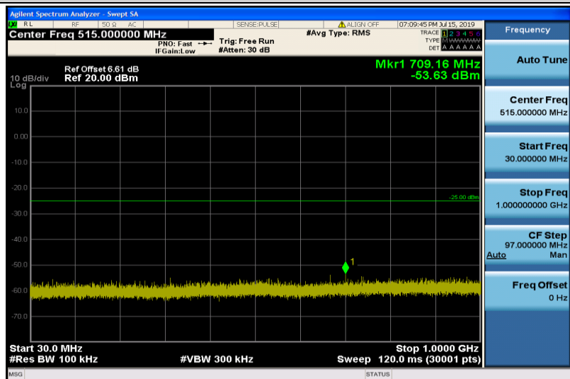
Band38-20MHz-QPSK-38150-1RB#0-Range1:30~1000MHz
