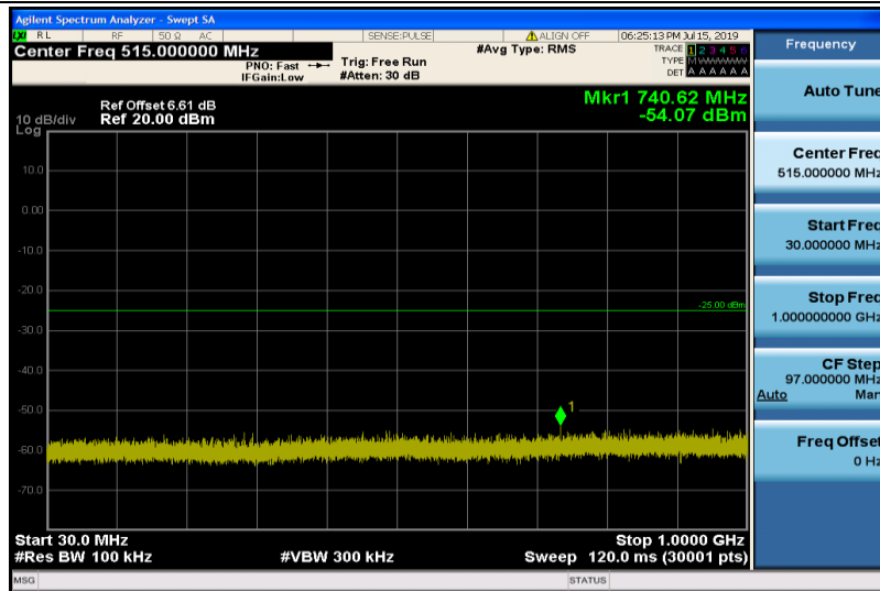
Band38-5MHz-QPSK-37775-1RB#0-Range1:30~1000MHz
