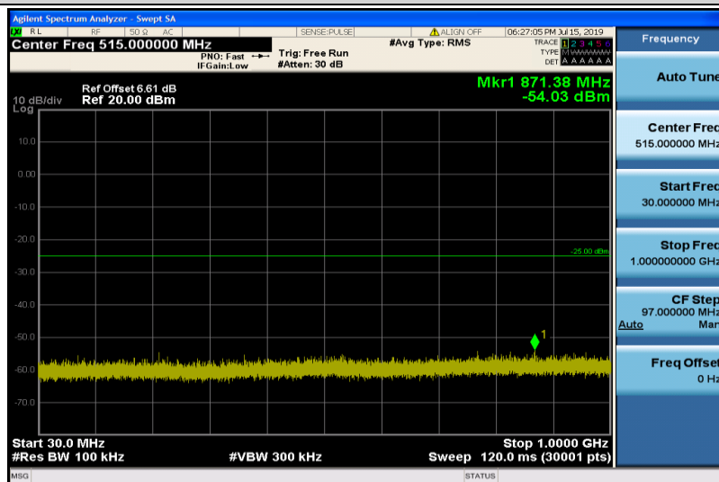
Band38-5MHz-QPSK-38000-1RB#0-Range1:30~1000MHz
