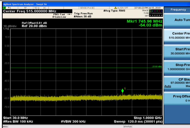
Band38-15MHz-16QAM-37825-1RB#0-Range1:30~1000MHz
