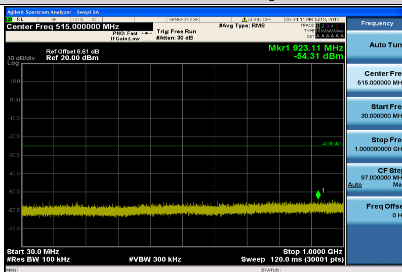
Band38-10MHz-16QAM-38000-1RB#0-Range1:30~1000MHz
