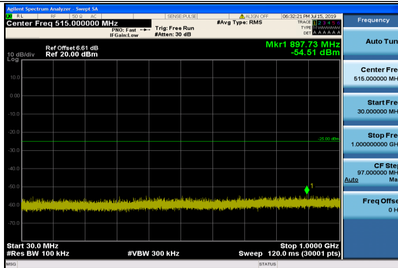
Band38-10MHz-QPSK-37800-1RB#0-Range1:30~1000MHz
