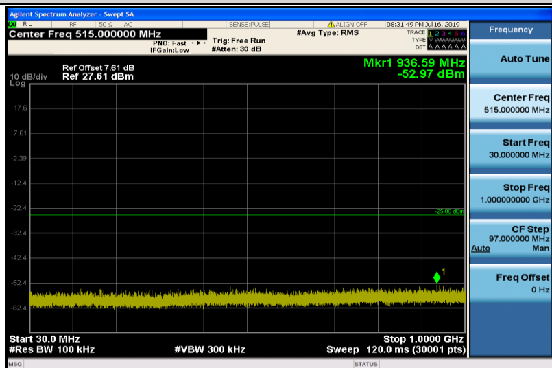
Band41-10MHz-QPSK-40620-1RB#0-30~1000MHz
