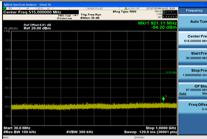
Band38-20MHz-16QAM-37850-1RB#0-Range1:30~1000MHz
