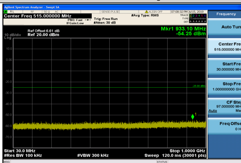
Band38-20MHz-QPSK-38000-1RB#0-Range1:30~1000MHz
