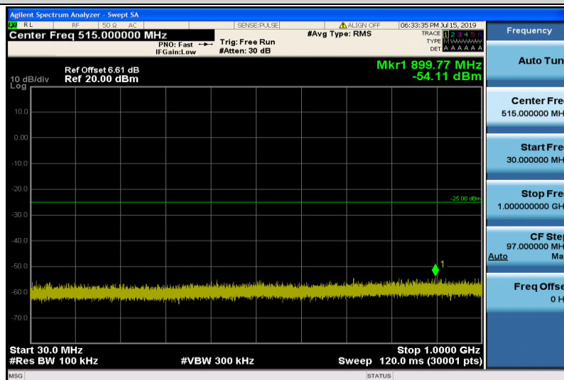
Band38-10MHz-QPSK-38000-1RB#0-Range1:30~1000MHz
