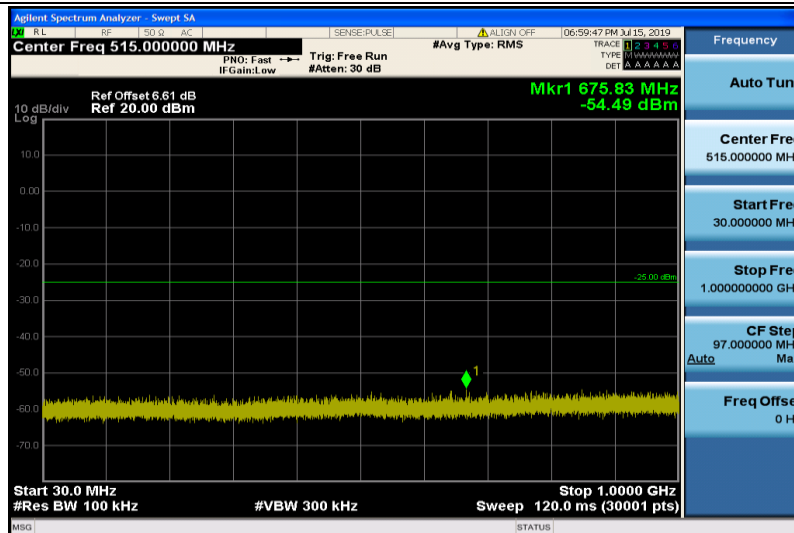
Band38-15MHz-QPSK-37825-1RB#0-Range1:30~1000MHz
