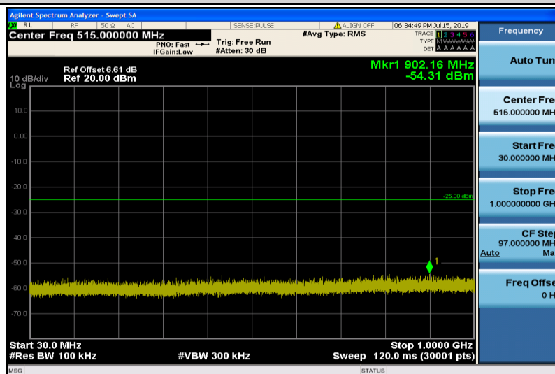
Band38-10MHz-QPSK-38200-1RB#0-Range1:30~1000MHz
