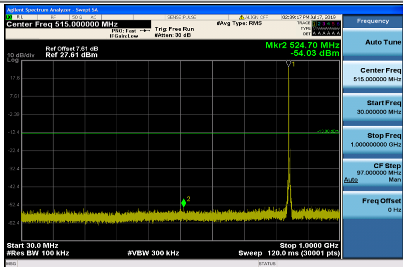
Band26-5MHz-16QAM-27015-1RB#0-30~1000MHz
