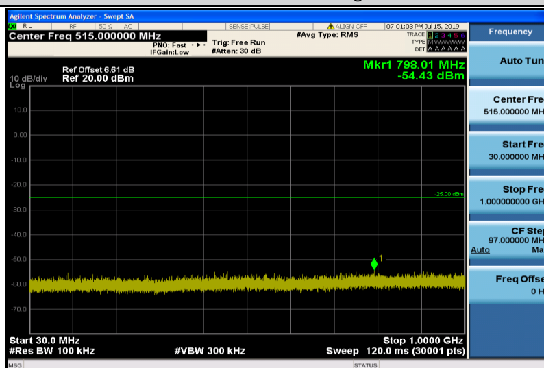
Band38-15MHz-QPSK-38000-1RB#0-Range1:30~1000MHz
