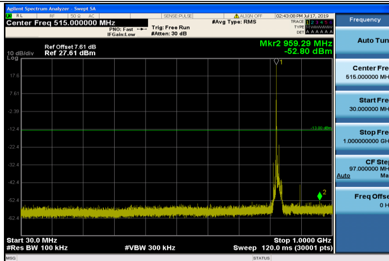
Band26-10MHz-16QAM-26840-1RB#0-30~1000MHz
