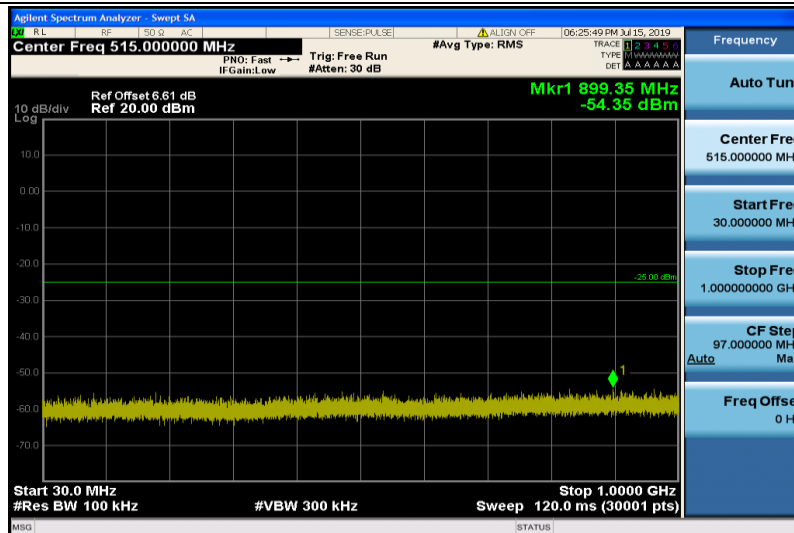
Band38-5MHz-16QAM-37775-1RB#0-Range1:30~1000MHz
