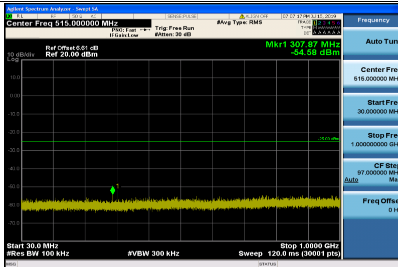
Band38-20MHz-QPSK-37850-1RB#0-Range1:30~1000MHz
