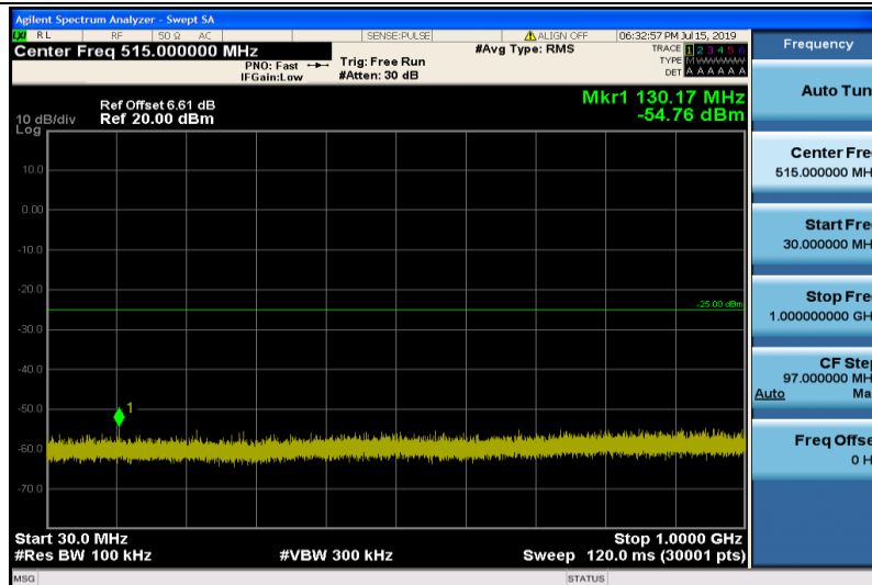
Band38-10MHz-16QAM-37800-1RB#0-Range1:30~1000MHz
