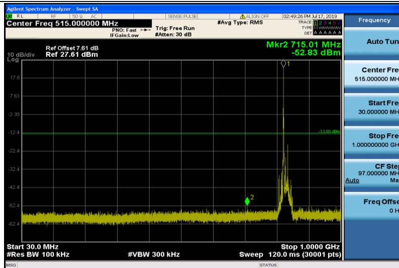
Band26-15MHz-QPSK-26915-1RB#0-30~1000MHz
