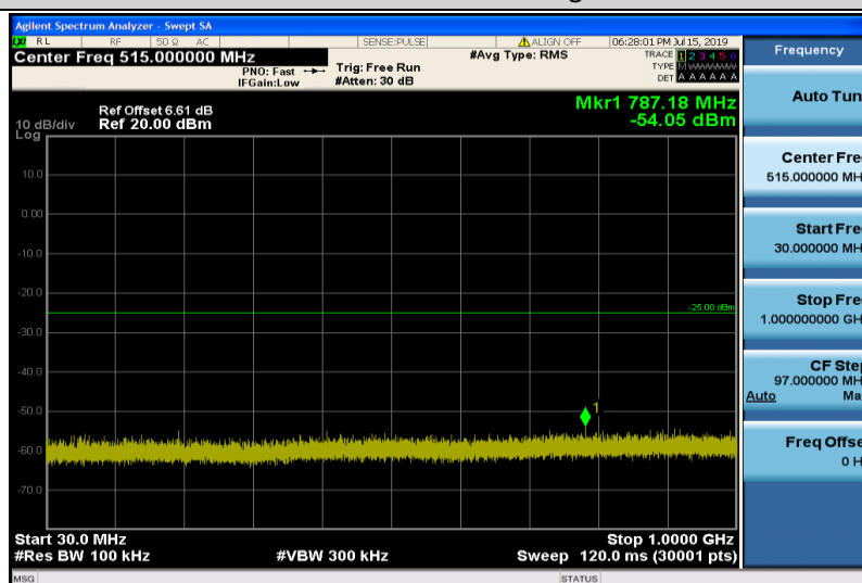
Band38-5MHz-16QAM-38000-1RB#0-Range1:30~1000MHz
