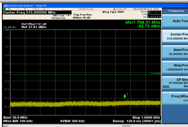
Band41-5MHz-16QAM-40620-1RB#0-30~1000MHz
