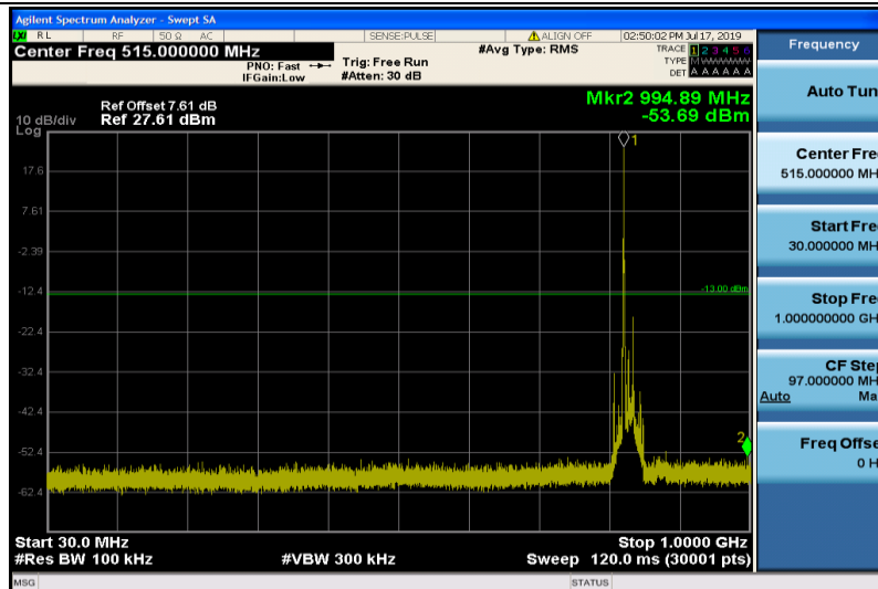
Band26-15MHz-16QAM-26915-1RB#0-30~1000MHz
