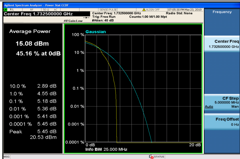
Band4-15MHz-16QAM-20175-1RB#0
