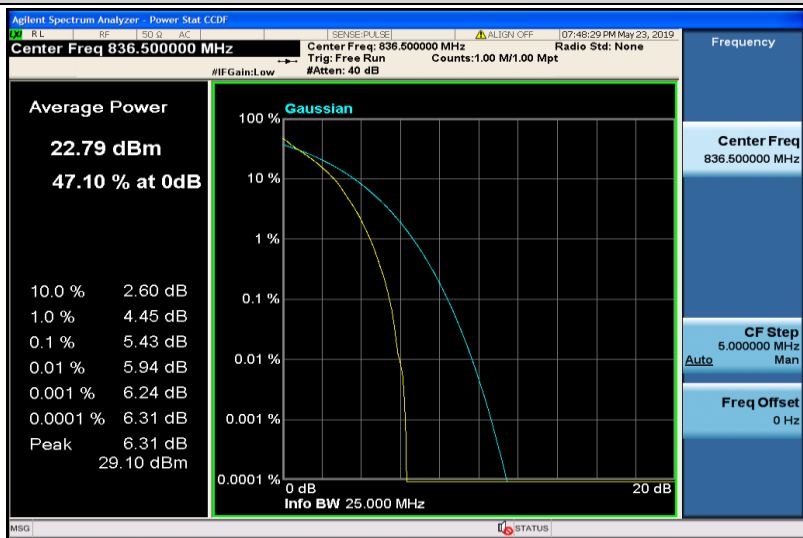
Band5-1.4MHz-QPSK-20525-6RB#0
