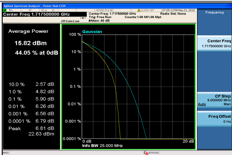
Band4-15MHz-QPSK-20025-75RB#0
