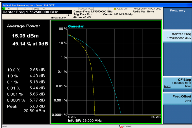
Band4-15MHz-QPSK-20175-75RB#0
