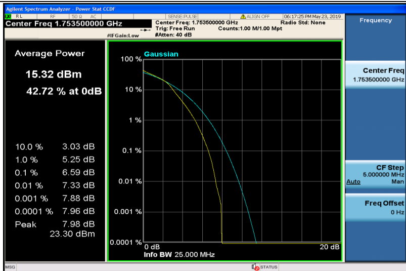
Band4-3MHz-16QAM-20385-15RB#0
