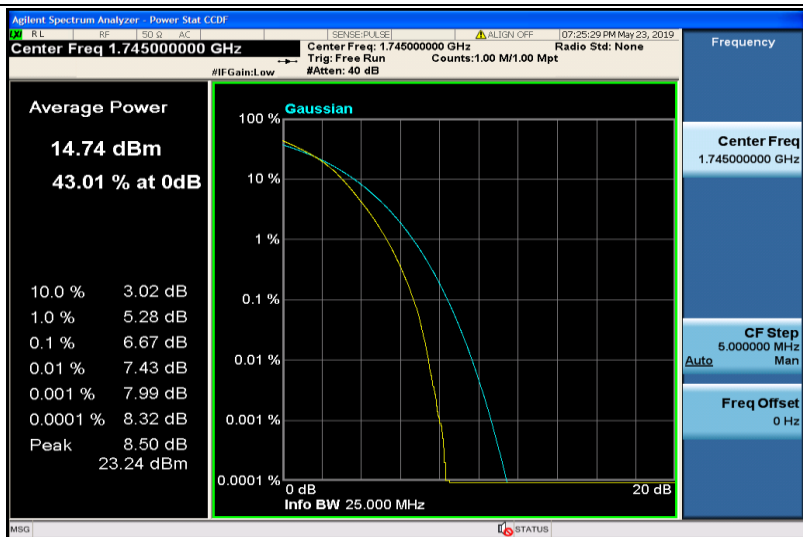
Band4-20MHz-16QAM-20300-100RB#0
