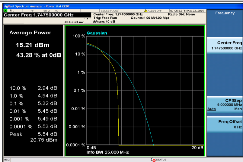
Band4-15MHz-16QAM-20325-1RB#0
