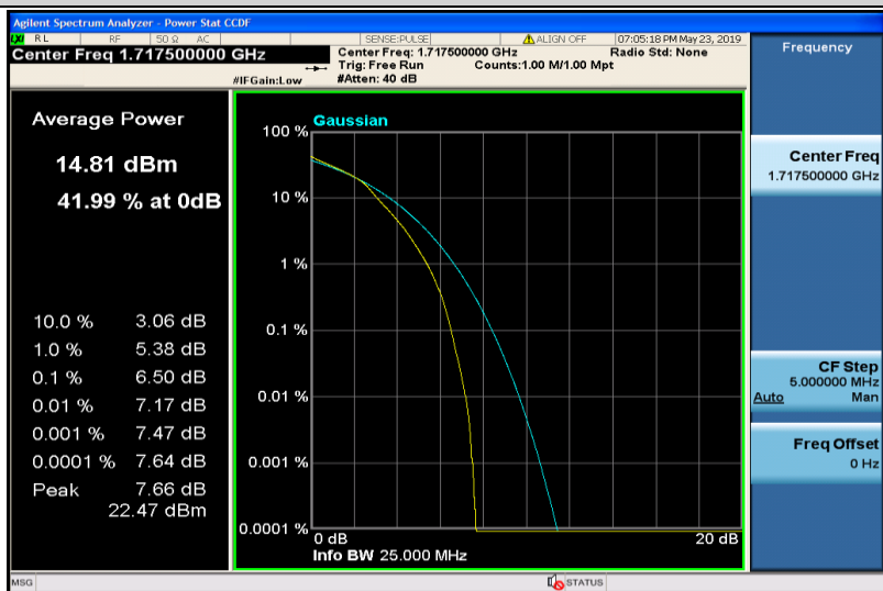
Band4-15MHz-16QAM-20025-75RB#0
