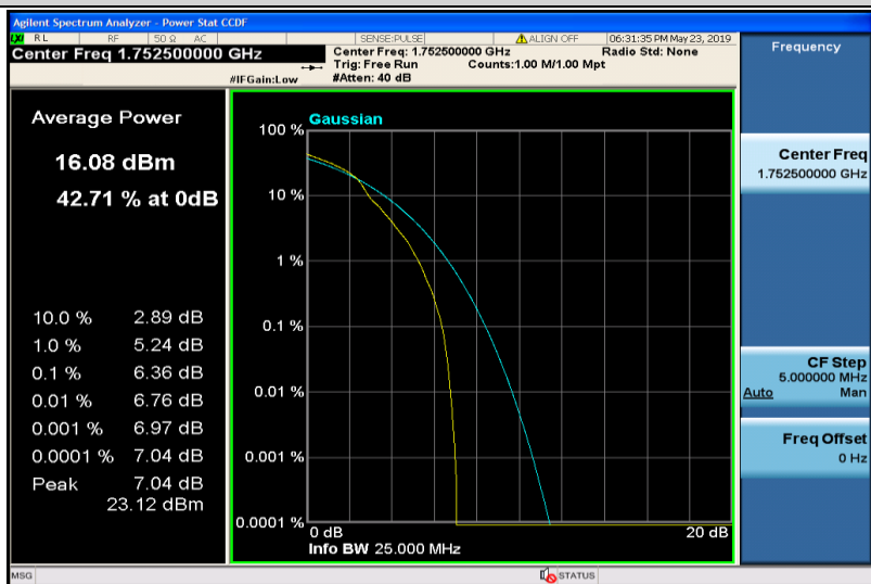
Band4-5MHz-16QAM-20375-1RB#0
