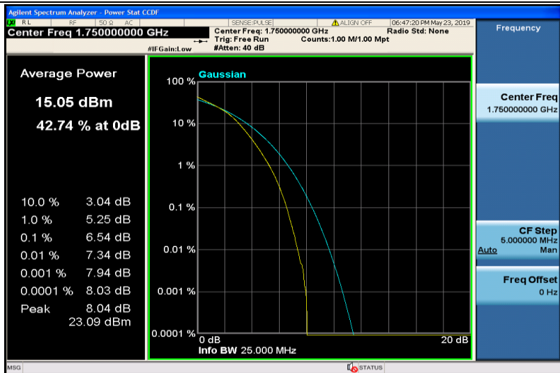
Band4-10MHz-16QAM-20350-50RB#0
