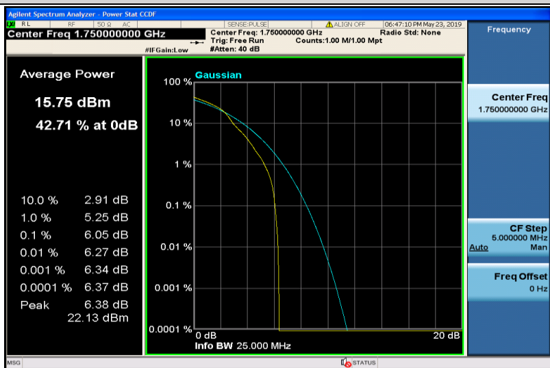
Band4-10MHz-16QAM-20350-1RB#0
