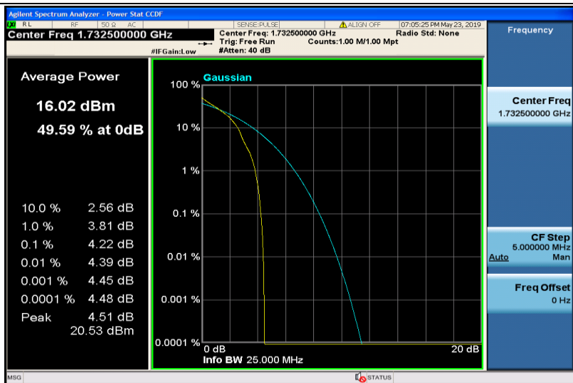
Band4-15MHz-QPSK-20175-1RB#0
