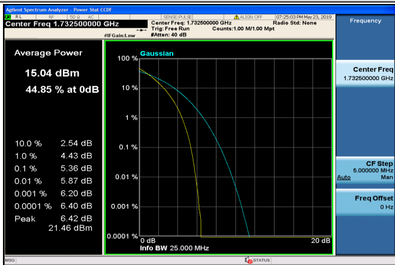
Band4-20MHz-QPSK-20175-100RB#0
