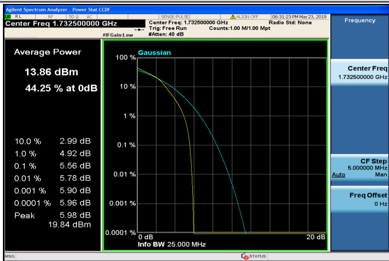
Band4-5MHz-16QAM-20175-25RB#0
