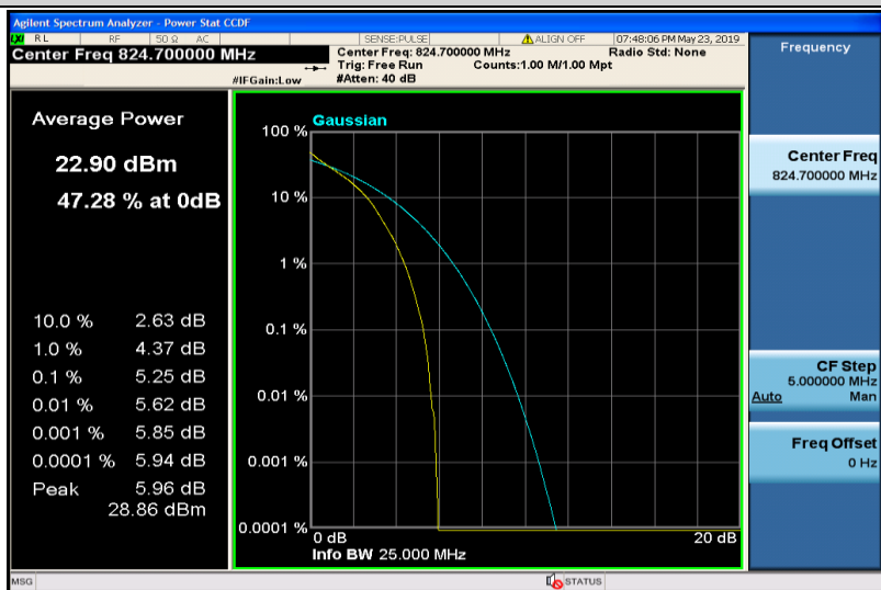
Band5-1.4MHz-QPSK-20407-6RB#0
