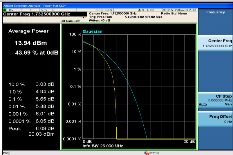
Band4-10MHz-16QAM-20175-50RB#0
