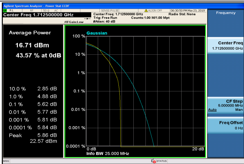
Band4-5MHz-16QAM-19975-1RB#0
