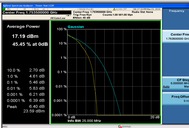
Band4-3MHz-QPSK-20385-1RB#0
