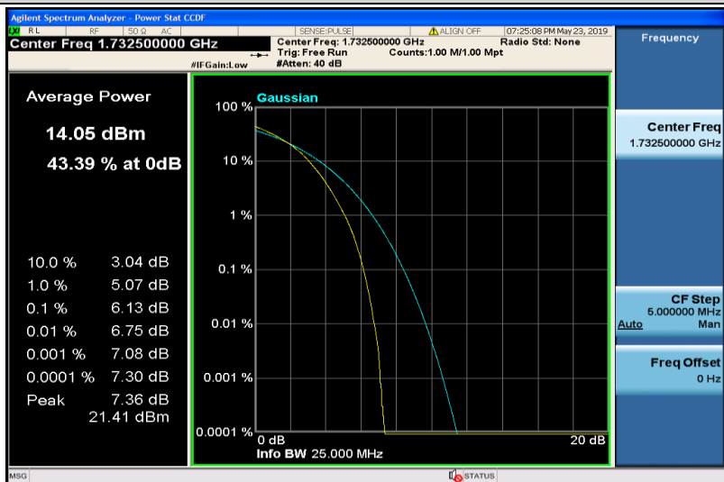
Band4-20MHz-16QAM-20175-100RB#0
