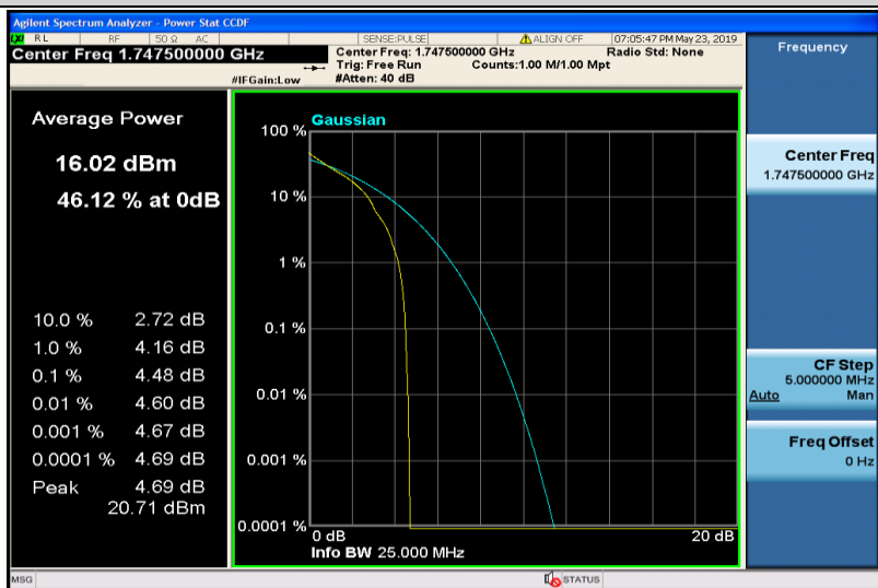
Band4-15MHz-QPSK-20325-1RB#0
