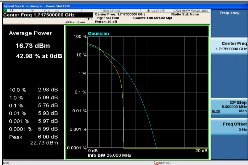
Band4-15MHz-16QAM-20025-1RB#0
