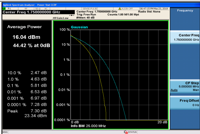
Band4-10MHz-QPSK-20350-50RB#0
