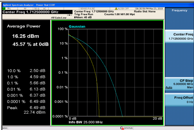
Band4-5MHz-QPSK-19975-25RB#0
