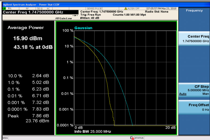
Band4-15MHz-QPSK-20325-75RB#0
