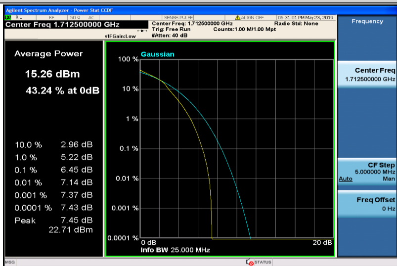
Band4-5MHz-16QAM-19975-25RB#0
