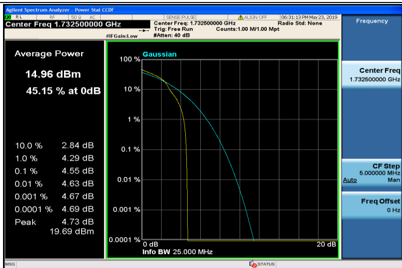
Band4-5MHz-16QAM-20175-1RB#0
