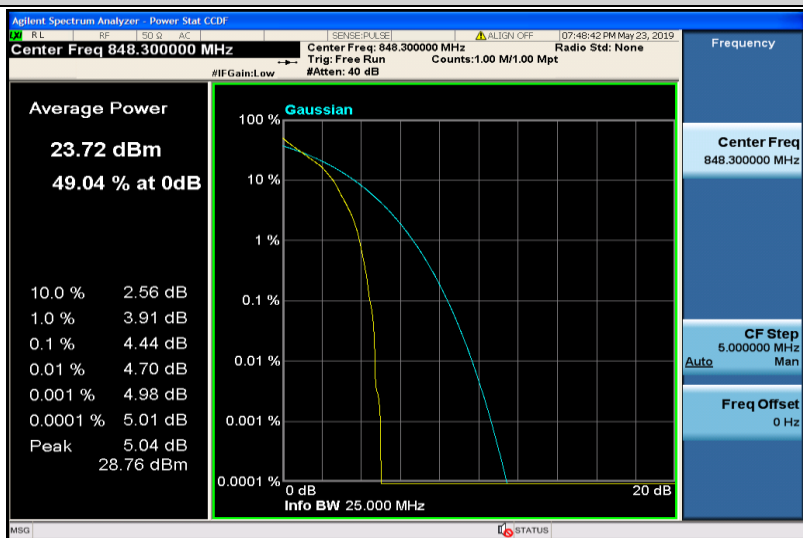
Band5-1.4MHz-QPSK-20643-1RB#0
