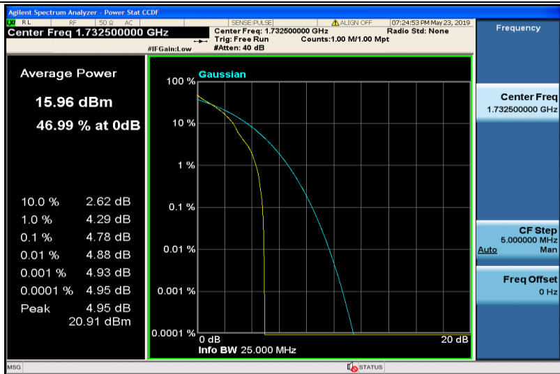
Band4-20MHz-QPSK-20175-1RB#0
