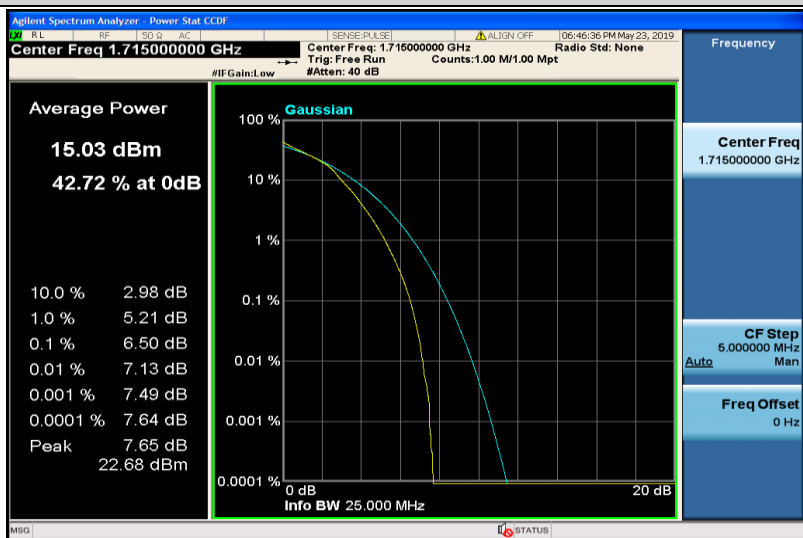
Band4-10MHz-16QAM-20000-50RB#0
