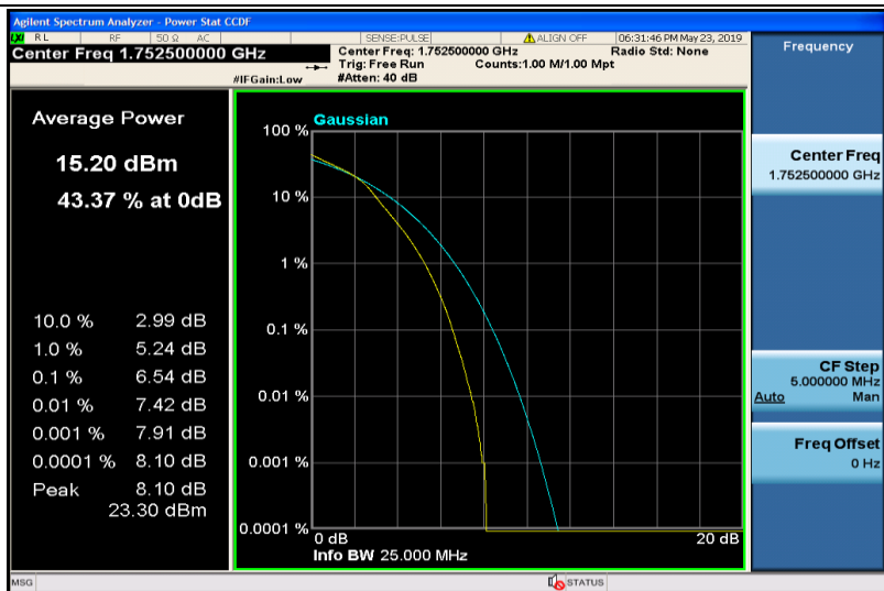
Band4-5MHz-16QAM-20375-25RB#0
