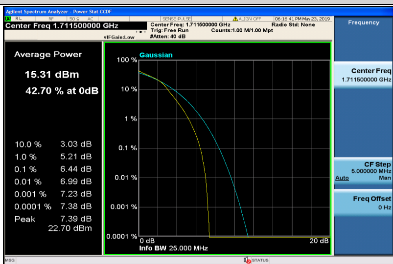
Band4-3MHz-16QAM-19965-15RB#0
