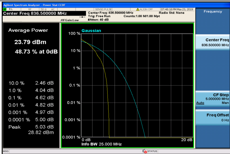
Band5-1.4MHz-QPSK-20525-1RB#0
