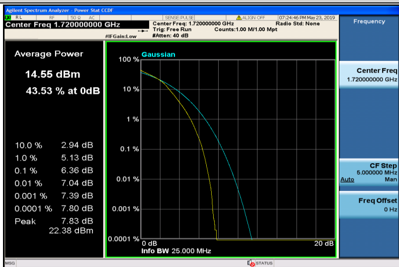
Band4-20MHz-16QAM-20050-100RB#0
