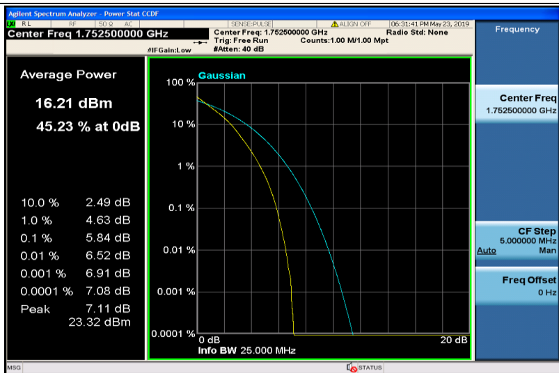
Band4-5MHz-QPSK-20375-25RB#0
