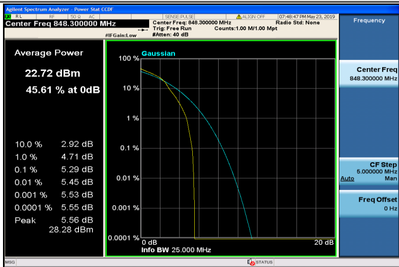
Band5-1.4MHz-16QAM-20643-1RB#0
