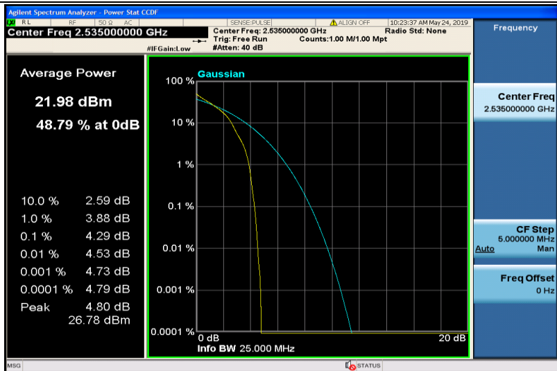
Band7-10MHz-QPSK-21100-1RB#0
