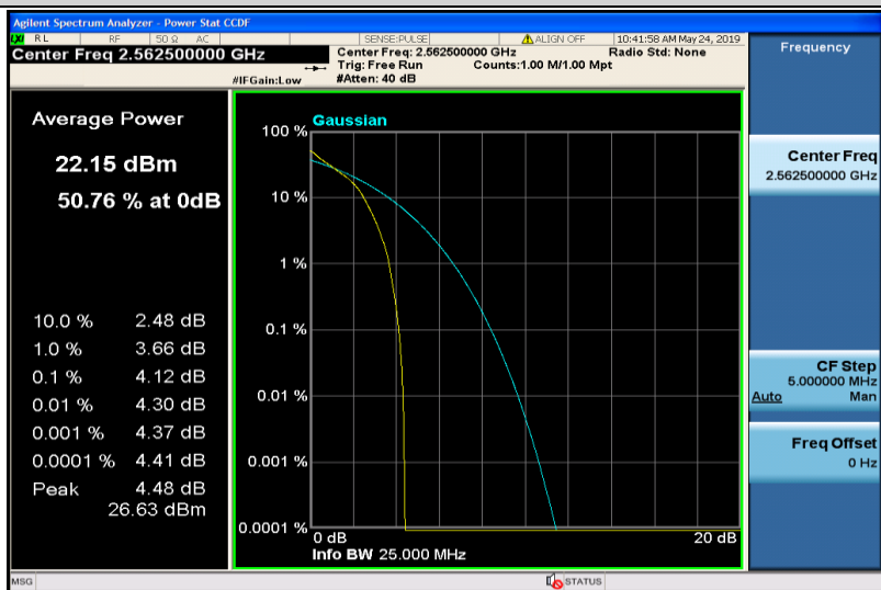
Band7-15MHz-QPSK-21375-1RB#0
