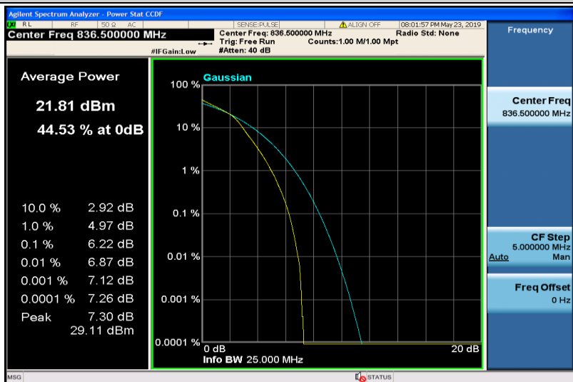
Band5-3MHz-16QAM-20525-15RB#0
