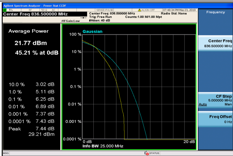
Band5-1.4MHz-16QAM-20525-6RB#0
