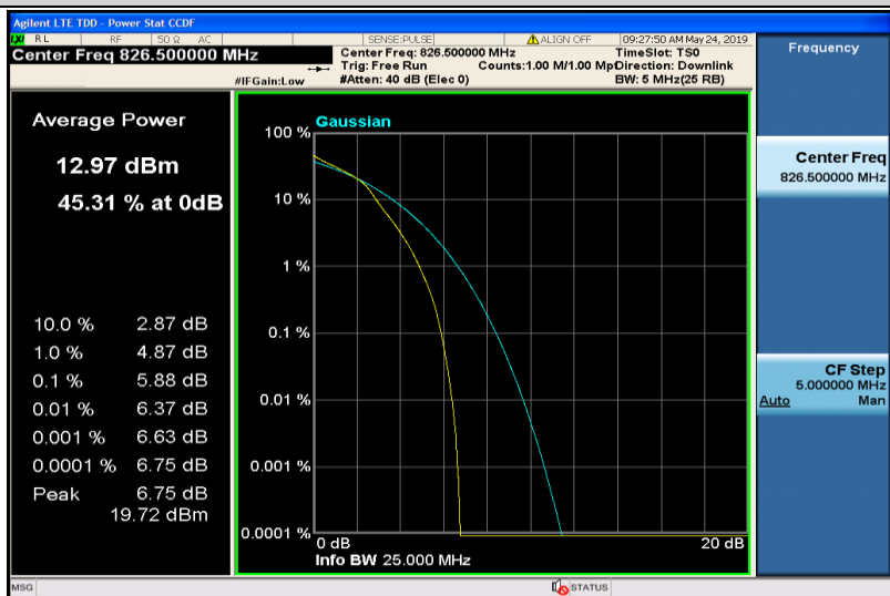
Band5-5MHz-16QAM-20425-25RB#0
