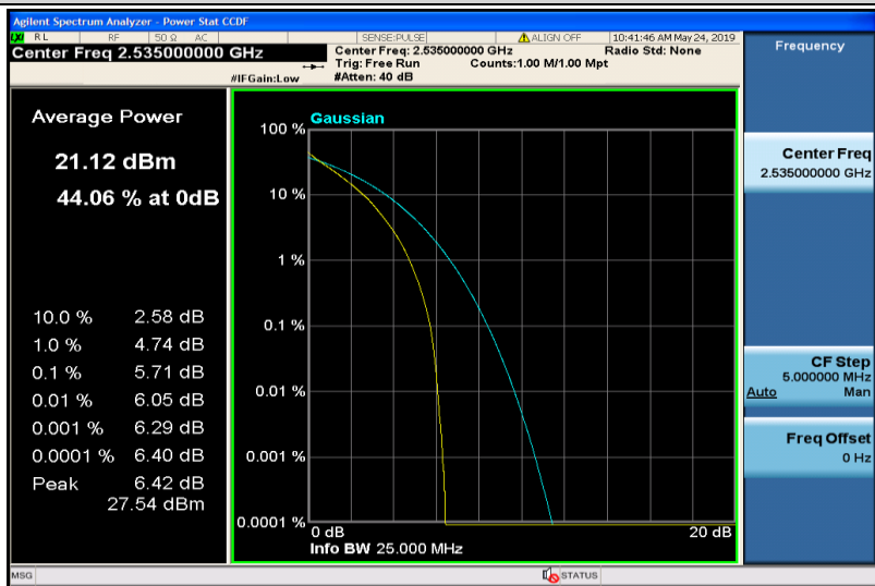
Band7-15MHz-QPSK-21100-75RB#0
