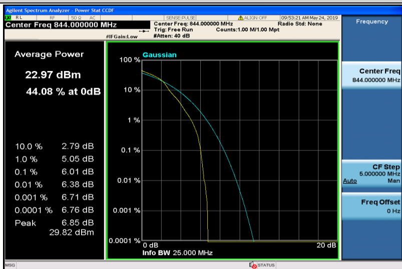
Band5-10MHz-16QAM-20600-1RB#0
