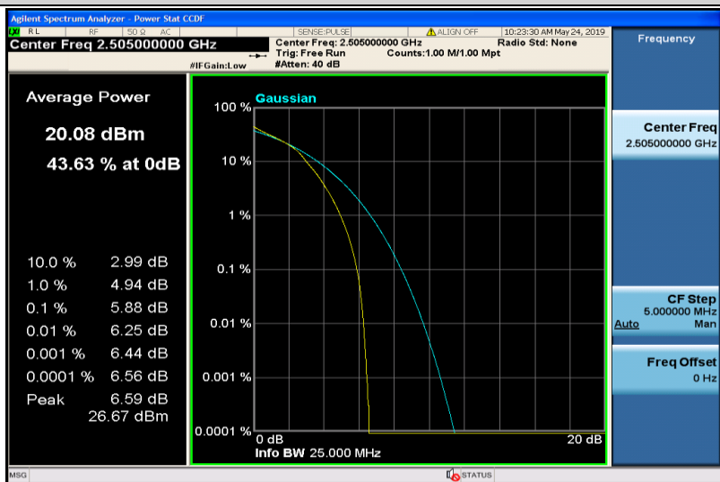
Band7-10MHz-16QAM-20800-50RB#0
