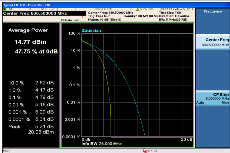
Band5-5MHz-QPSK-20525-1RB#0
