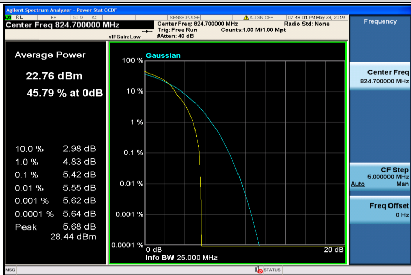
Band5-1.4MHz-16QAM-20407-1RB#0
