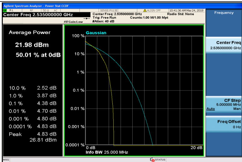
Band7-15MHz-QPSK-21100-1RB#0
