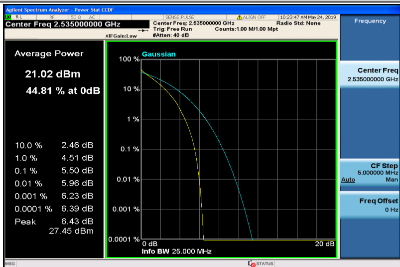
Band7-10MHz-QPSK-21100-50RB#0
