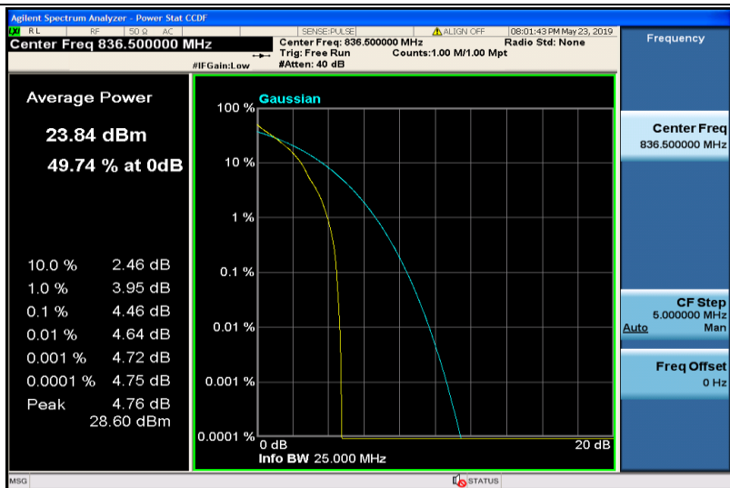
Band5-3MHz-QPSK-20525-1RB#0
