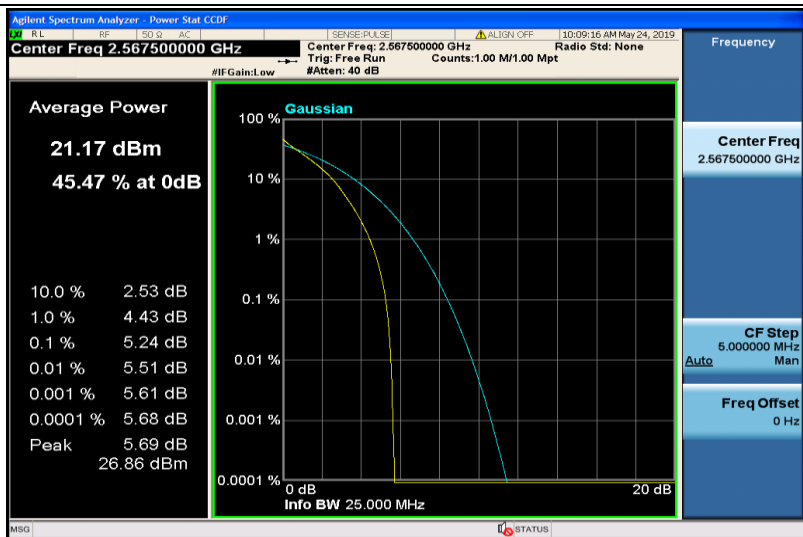
Band7-5MHz-QPSK-21425-25RB#0
