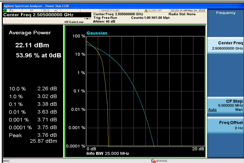
Band7-10MHz-QPSK-20800-1RB#0
