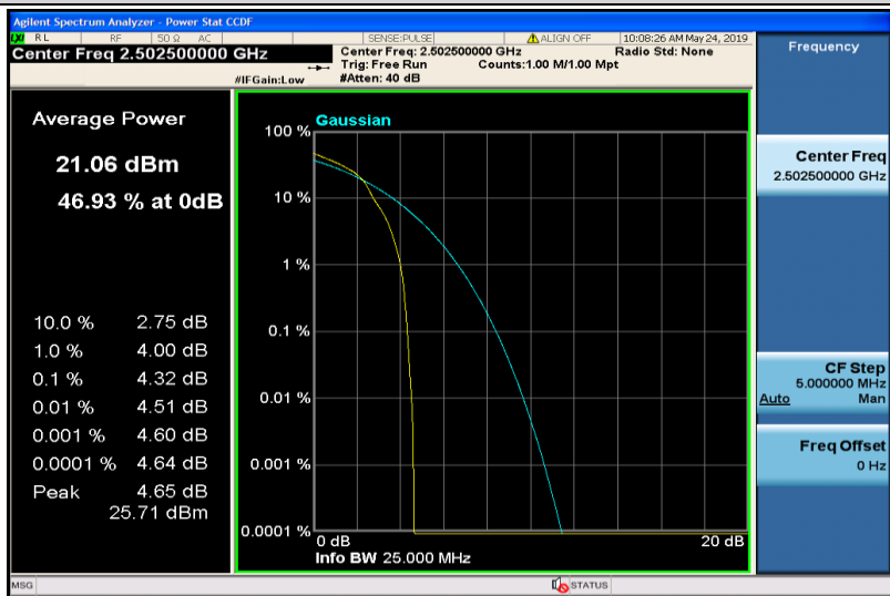
Band7-5MHz-16QAM-20775-1RB#0
