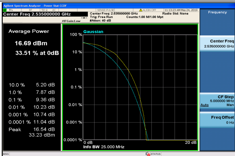
Band7-20MHz-16QAM-21100-100RB#0
