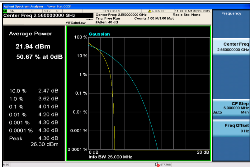
Band7-20MHz-QPSK-21350-1RB#0
