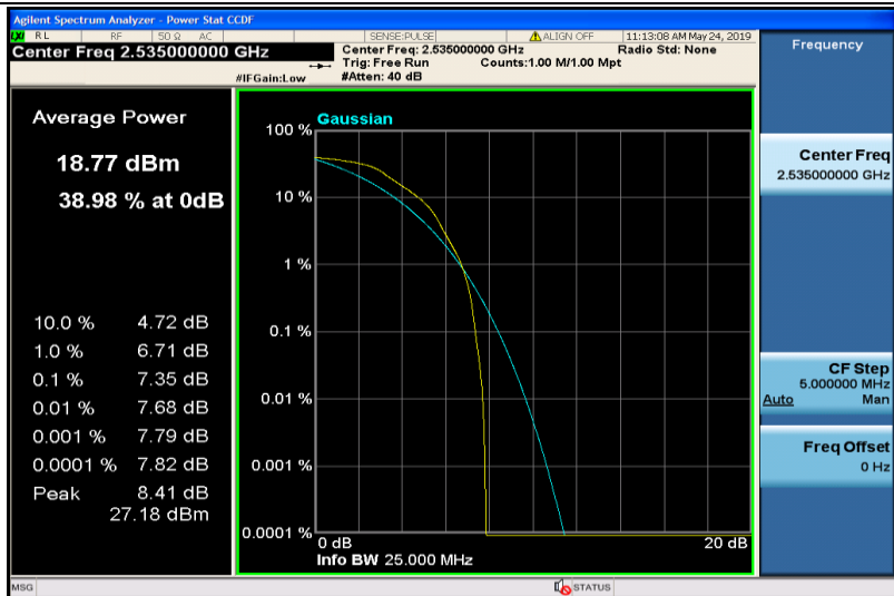
Band7-20MHz-QPSK-21100-1RB#0
