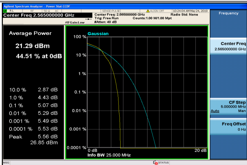
Band7-10MHz-16QAM-21400-1RB#0
