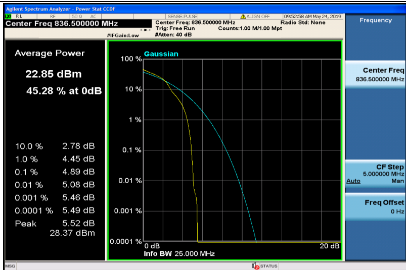
Band5-10MHz-16QAM-20525-1RB#0
