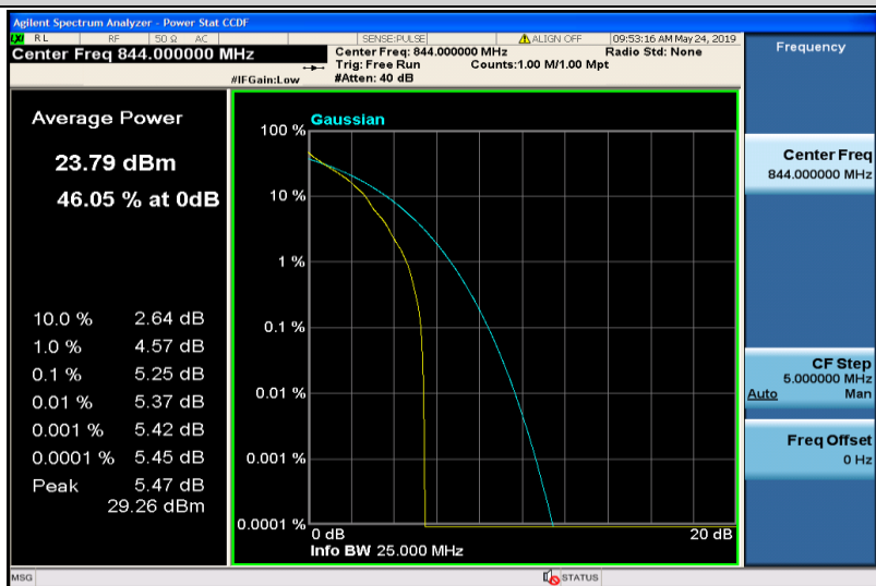
Band5-10MHz-QPSK-20600-1RB#0
