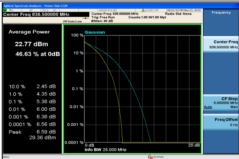
Band5-3MHz-QPSK-20525-15RB#0
