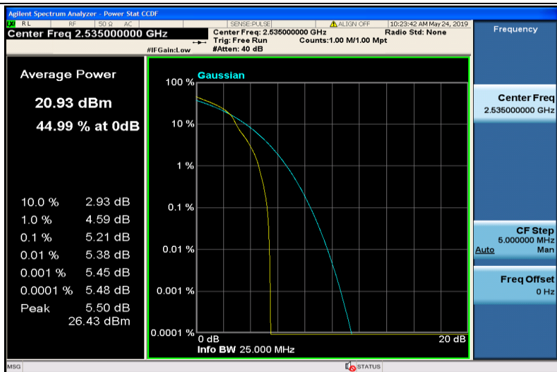
Band7-10MHz-16QAM-21100-1RB#0
