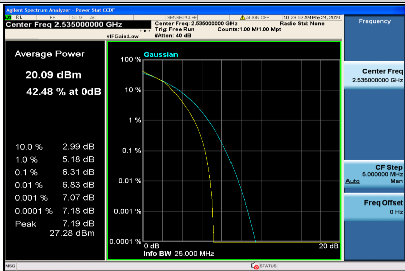
Band7-10MHz-16QAM-21100-50RB#0
