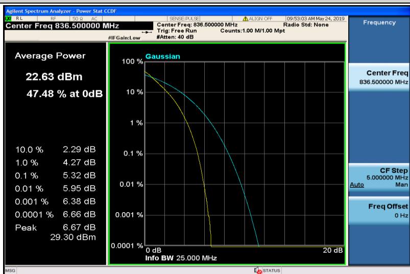
Band5-10MHz-QPSK-20525-50RB#0
