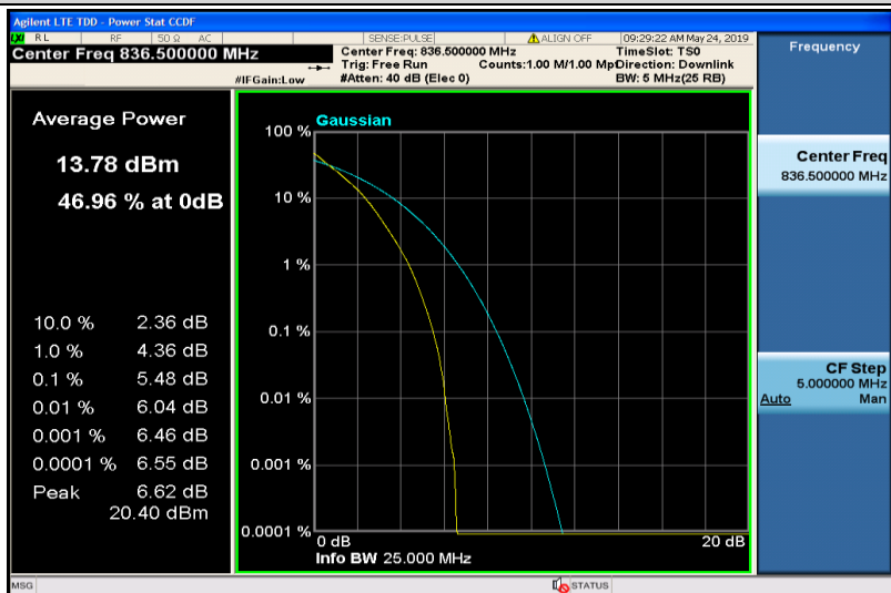
Band5-5MHz-QPSK-20525-25RB#0
