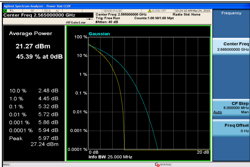
Band7-10MHz-QPSK-21400-50RB#0
