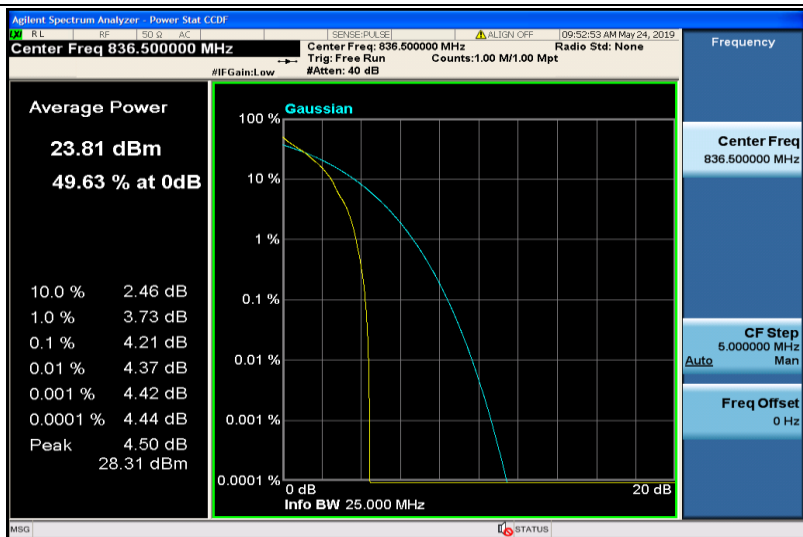
Band5-10MHz-QPSK-20525-1RB#0
