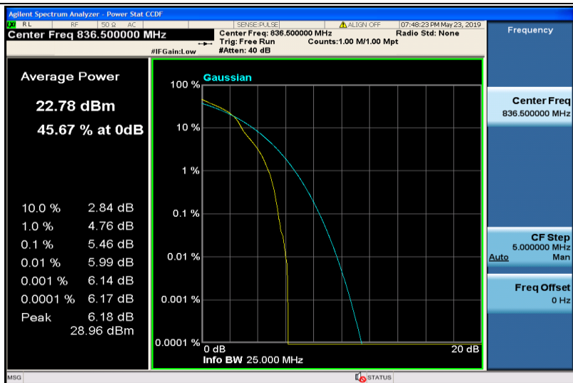
Band5-1.4MHz-16QAM-20525-1RB#0
