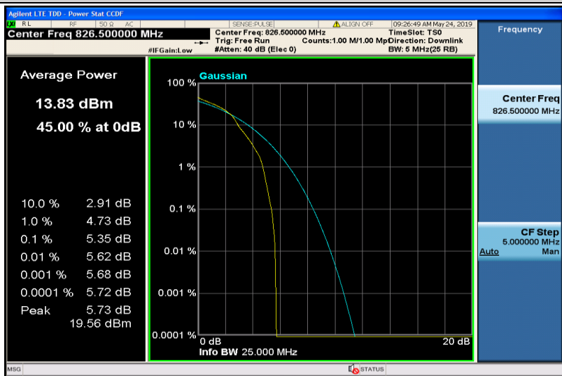
Band5-5MHz-16QAM-20425-1RB#0
