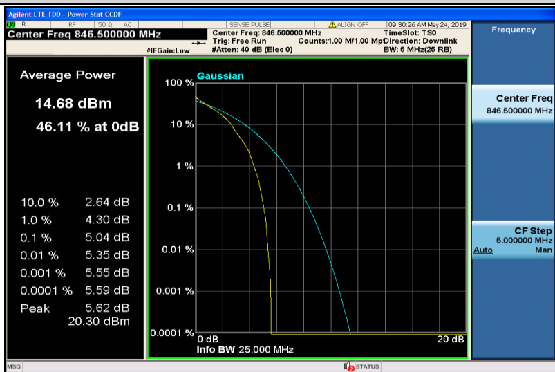
Band5-5MHz-QPSK-20625-1RB#0
