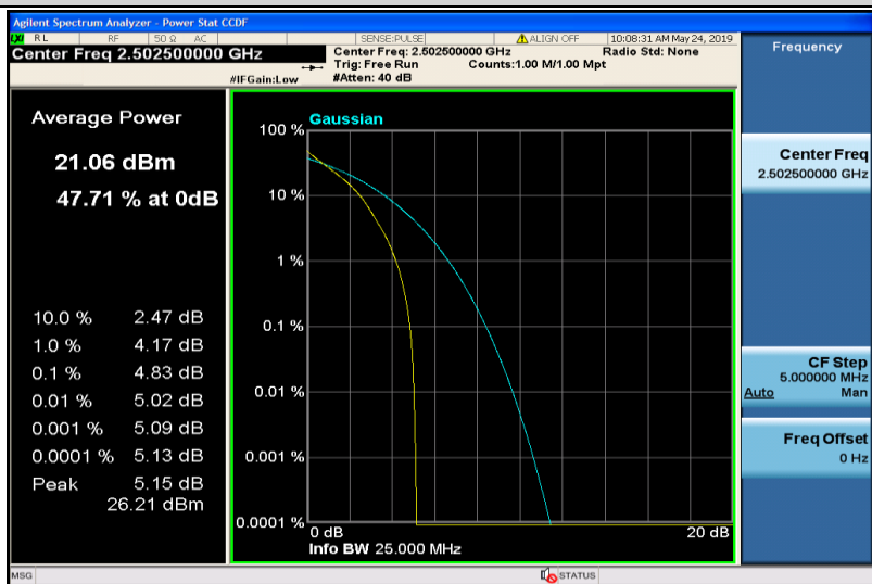
Band7-5MHz-QPSK-20775-25RB#0
