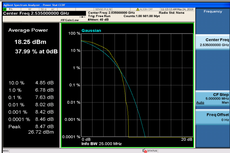
Band7-20MHz-16QAM-21100-1RB#0
