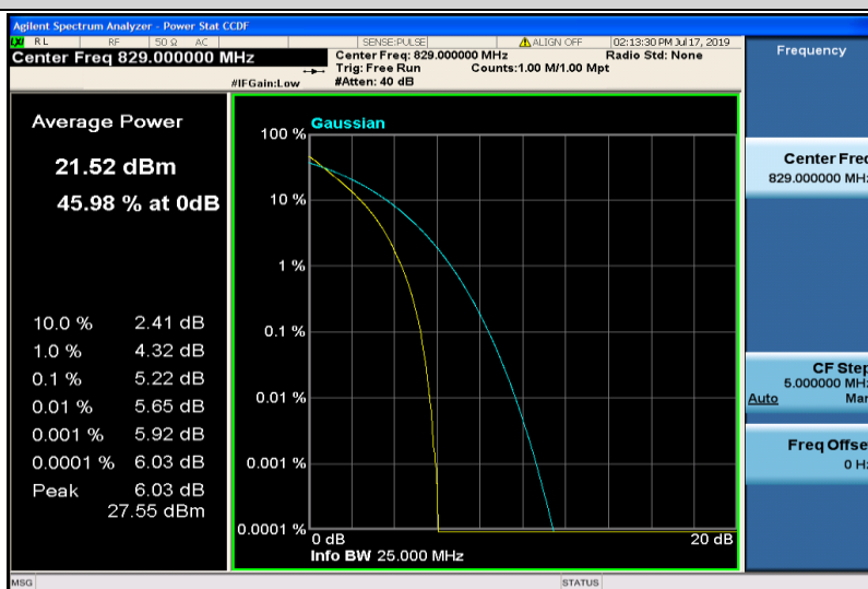
Band26-10MHz-QPSK-26840-50RB#0
