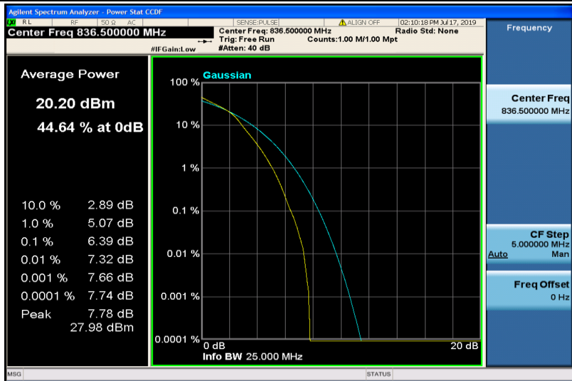
Band26-5MHz-16QAM-26915-25RB#0
