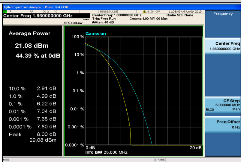
Band25-20MHz-16QAM-26140-100RB#0
