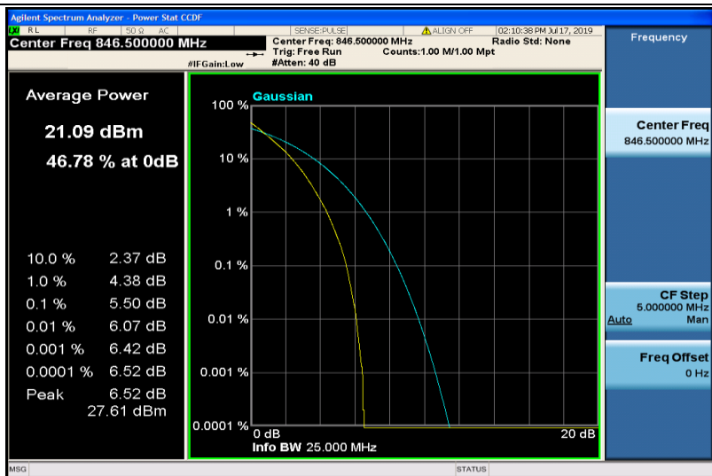
Band26-5MHz-QPSK-27015-25RB#0
