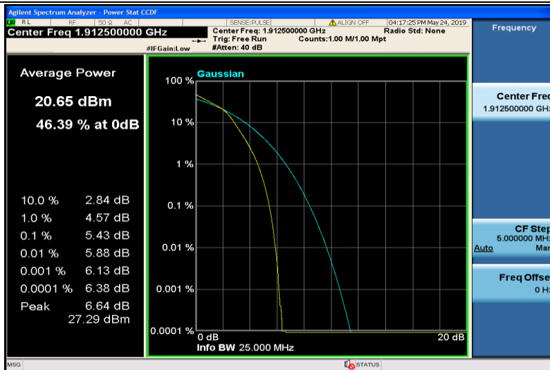
Band25-5MHz-16QAM-26665-25RB#0
