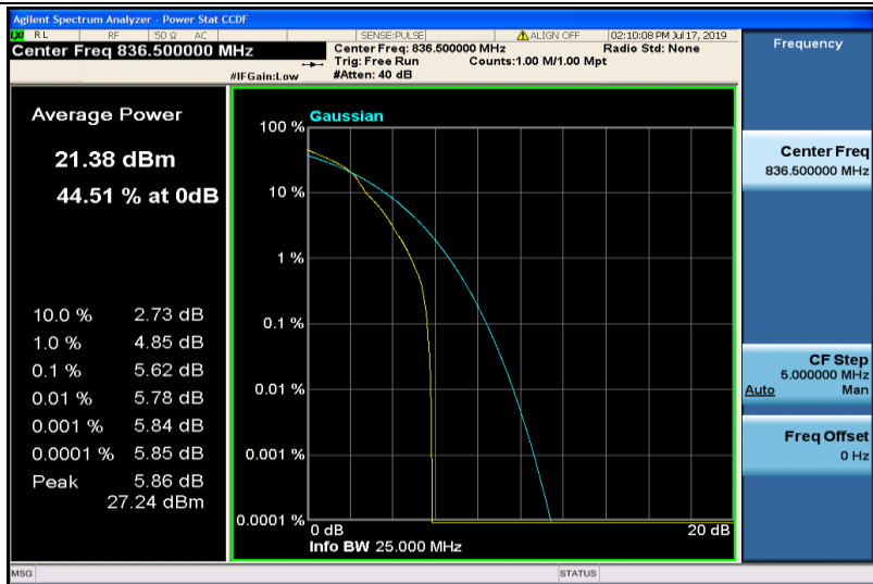
Band26-5MHz-16QAM-26915-1RB#0
