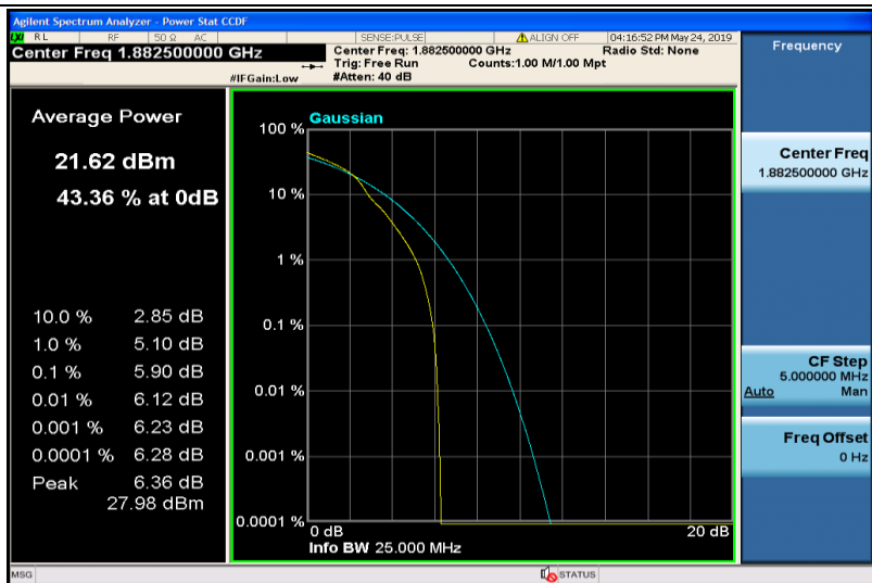
Band25-5MHz-16QAM-26365-1RB#0
