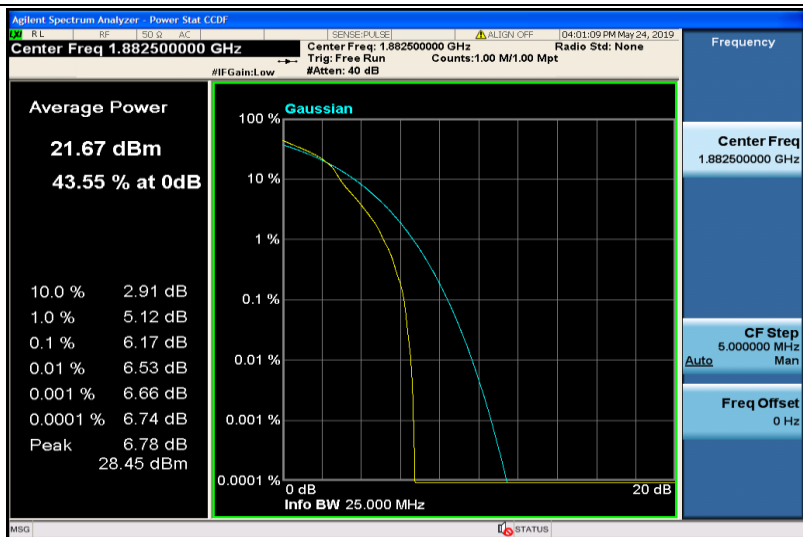
Band25-3MHz-16QAM-26365-1RB#0
