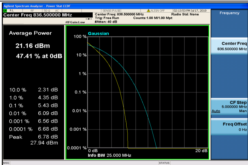
Band26-10MHz-QPSK-26915-50RB#0
