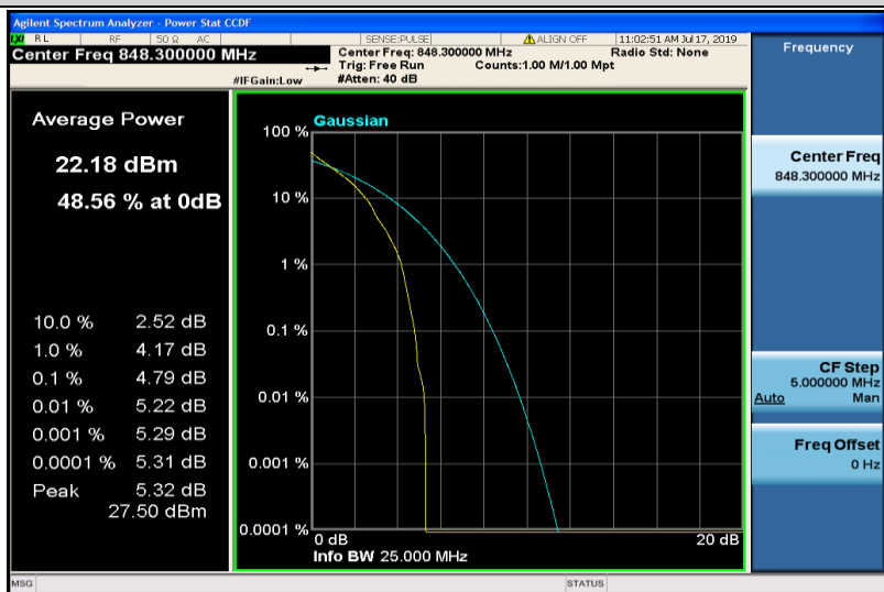
Band26-1.4MHz-QPSK-27033-1RB#0
