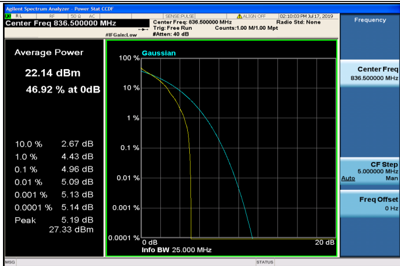
Band26-5MHz-QPSK-26915-1RB#0
