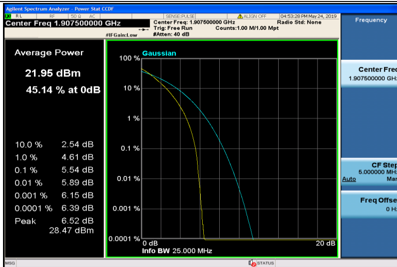
Band25-15MHz-QPSK-26615-75RB#0
