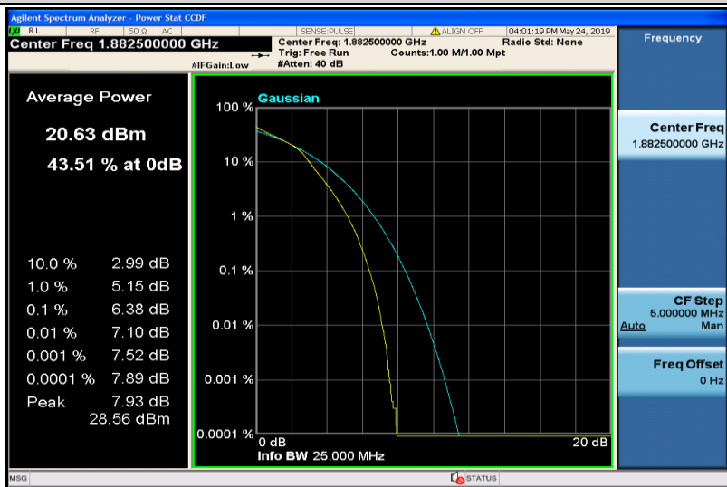
Band25-3MHz-16QAM-26365-15RB#0
