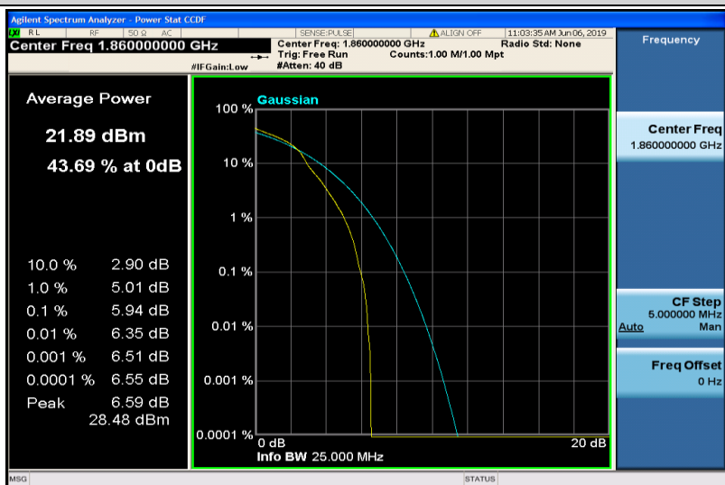
Band25-20MHz-16QAM-26140-1RB#0
