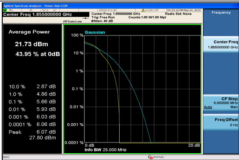
Band25-10MHz-16QAM-26090-1RB#0
