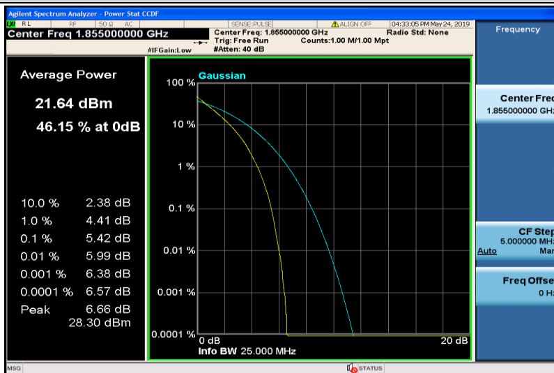
Band25-10MHz-QPSK-26090-1RB#0
