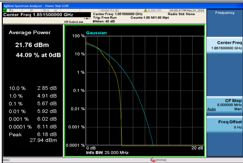
Band25-3MHz-16QAM-26055-1RB#0
