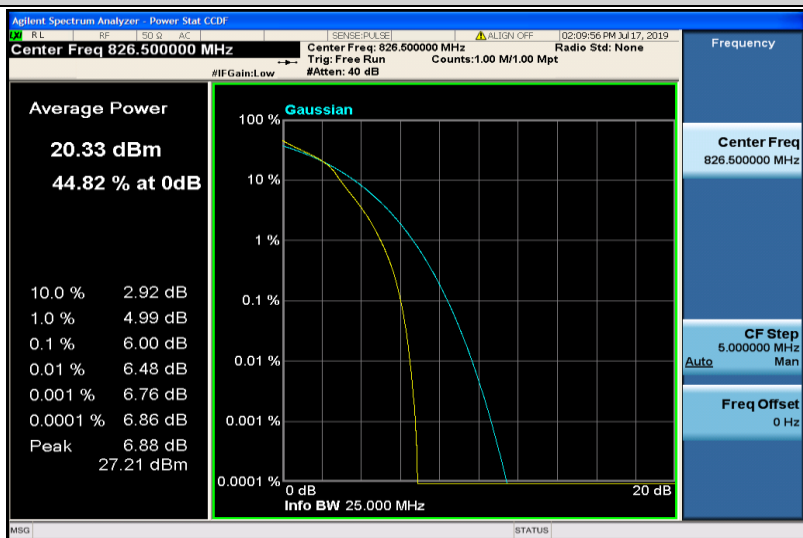
Band26-5MHz-16QAM-26815-25RB#0
