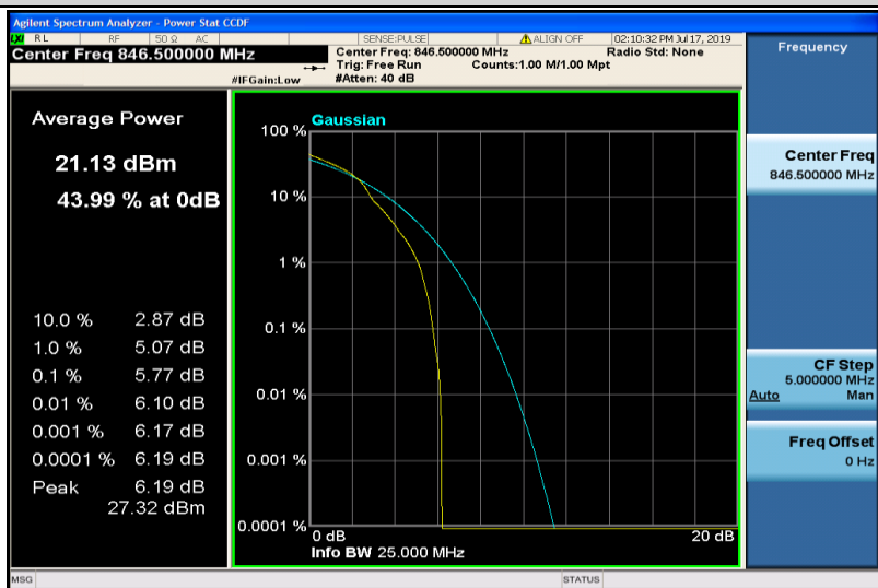
Band26-5MHz-16QAM-27015-1RB#0
