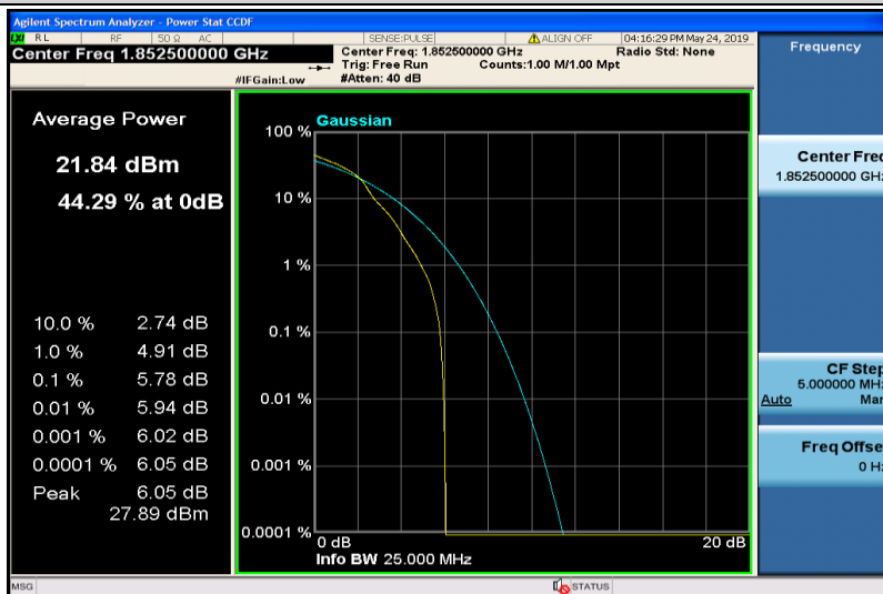
Band25-5MHz-16QAM-26065-1RB#0
