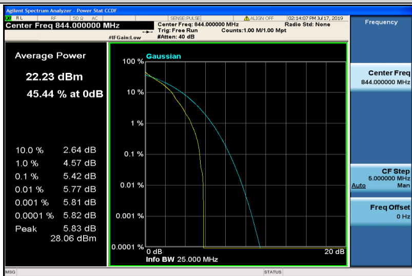
Band26-10MHz-QPSK-26990-1RB#0
