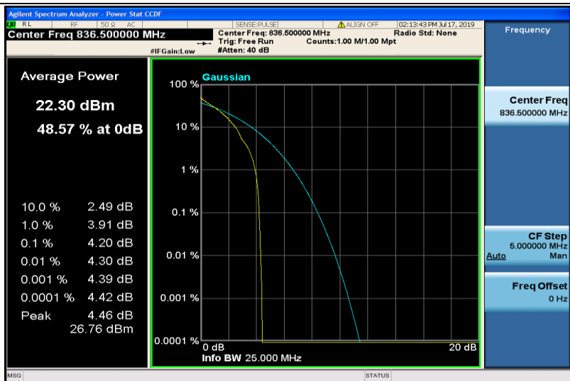
Band26-10MHz-QPSK-26915-1RB#0
