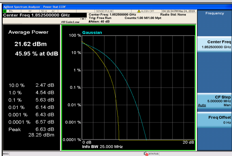
Band25-5MHz-QPSK-26065-25RB#0
