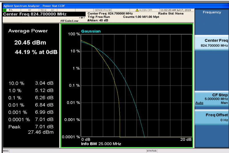
Band26-1.4MHz-16QAM-26797-6RB#0
