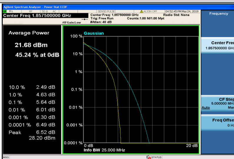
Band25-15MHz-QPSK-26115-75RB#0
