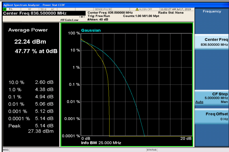
Band26-1.4MHz-QPSK-26915-1RB#0
