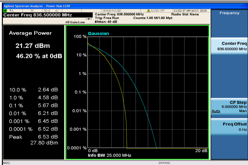
Band26-1.4MHz-QPSK-26915-6RB#0
