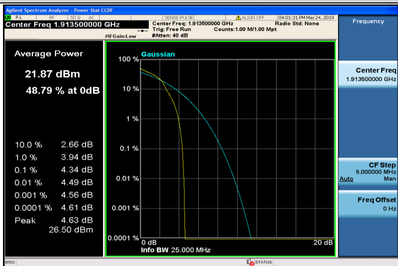
Band25-3MHz-16QAM-26675-1RB#0
