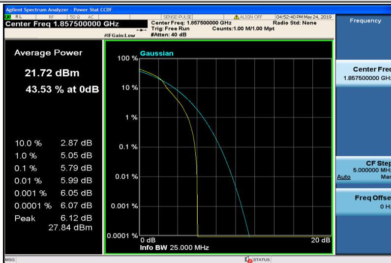
Band25-15MHz-16QAM-26115-1RB#0
