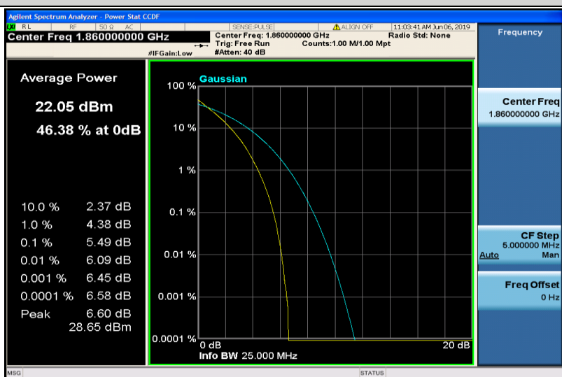
Band25-20MHz-QPSK-26140-100RB#0
