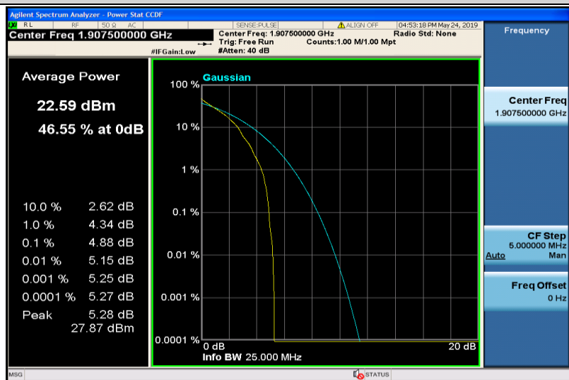
Band25-15MHz-QPSK-26615-1RB#0
