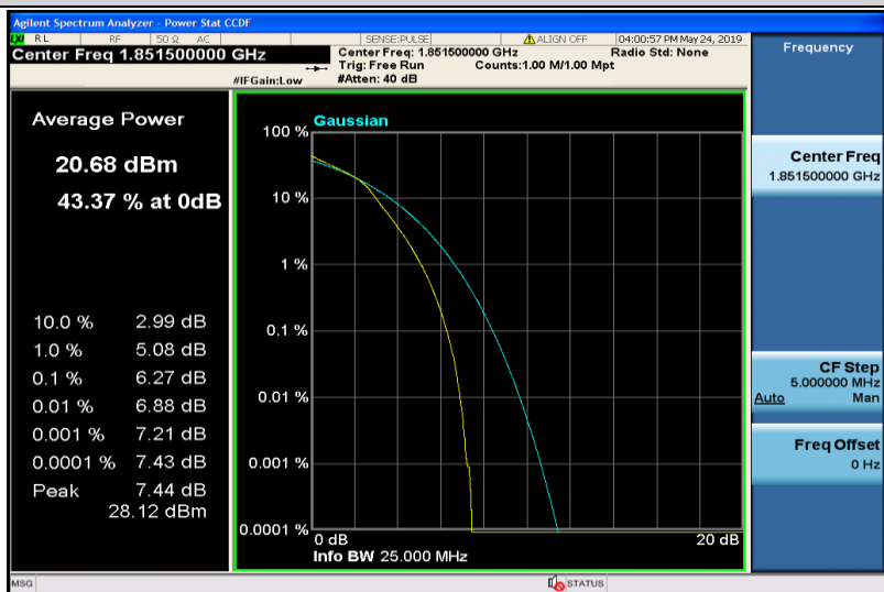
Band25-3MHz-16QAM-26055-15RB#0
