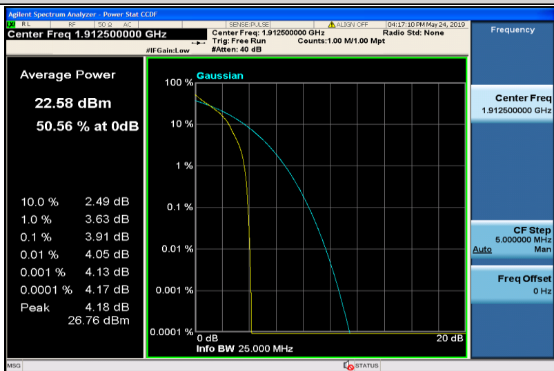
Band25-5MHz-QPSK-26665-1RB#0
