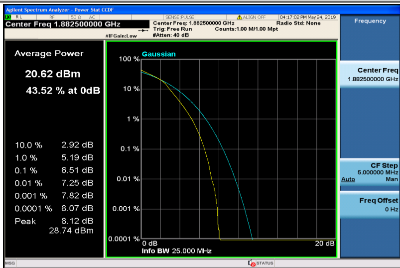
Band25-5MHz-16QAM-26365-25RB#0
