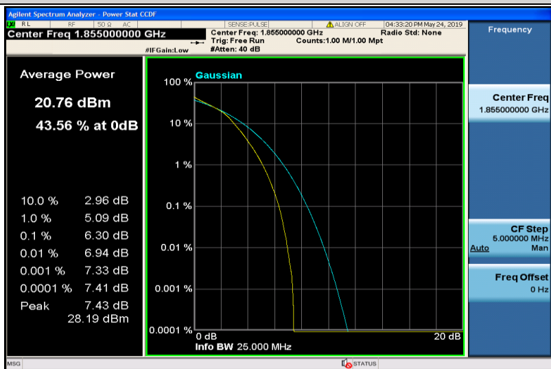
Band25-10MHz-16QAM-26090-50RB#0
