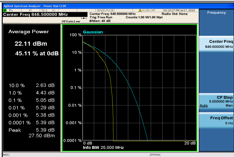
Band26-5MHz-QPSK-27015-1RB#0
