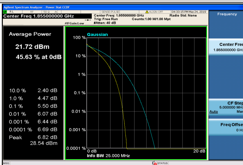
Band25-10MHz-QPSK-26090-50RB#0
