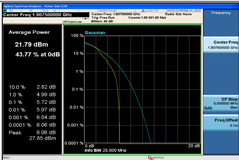
Band25-15MHz-16QAM-26615-1RB#0
