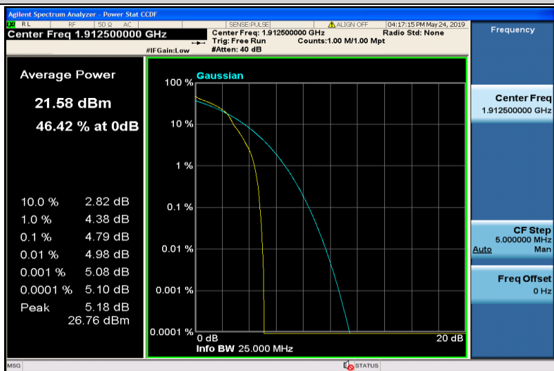
Band25-5MHz-16QAM-26665-1RB#0
