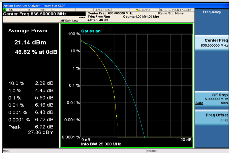
Band26-5MHz-QPSK-26915-25RB#0
