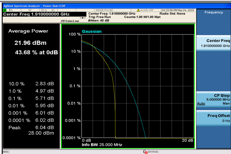
Band25-10MHz-16QAM-26640-1RB#0
