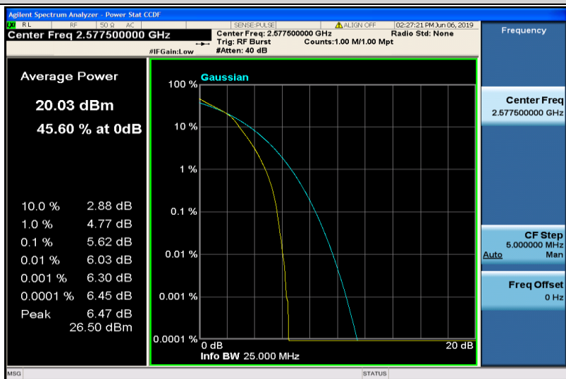
Band38-15MHz-16QAM-37825-75RB#0
