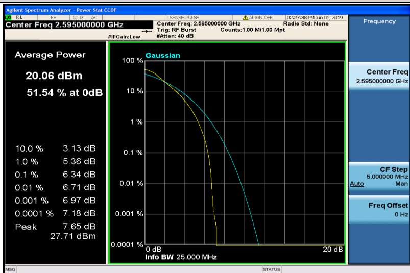
Band38-15MHz-QPSK-38000-75RB#0
