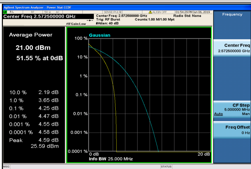
Band38-5MHz-QPSK-37775-25RB#0
