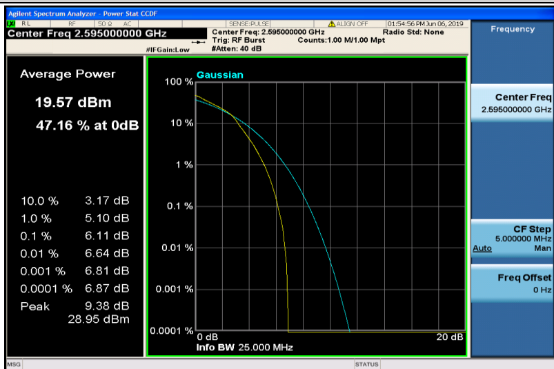
Band38-5MHz-16QAM-38000-25RB#0
