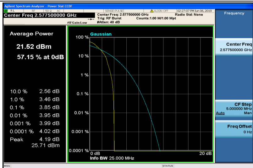
Band38-15MHz-QPSK-37825-1RB#0
