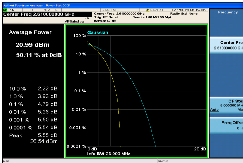
Band38-20MHz-QPSK-38150-100RB#0
