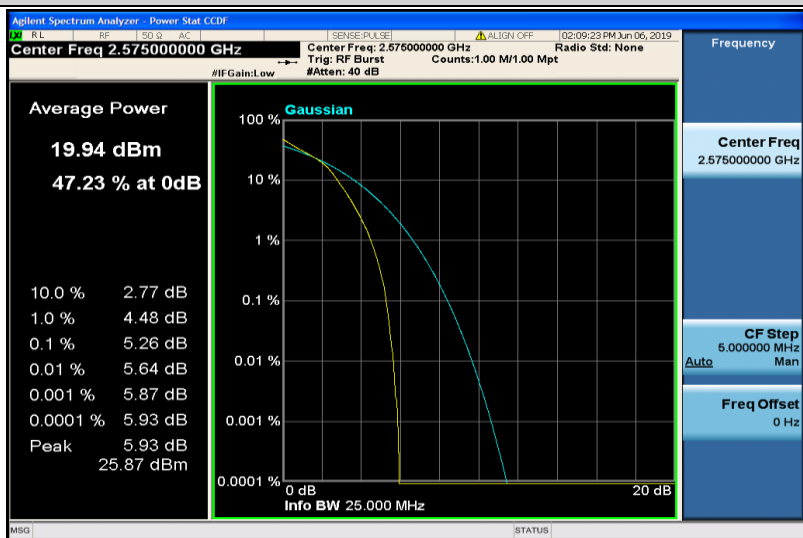
Band38-10MHz-16QAM-37800-50RB#0
