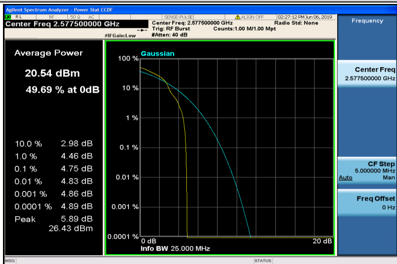
Band38-15MHz-16QAM-37825-1RB#0
