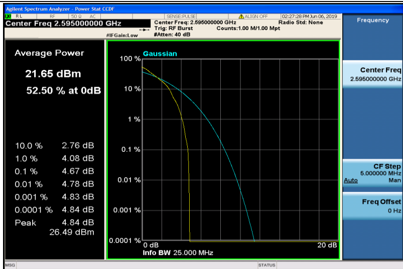
Band38-15MHz-QPSK-38000-1RB#0
