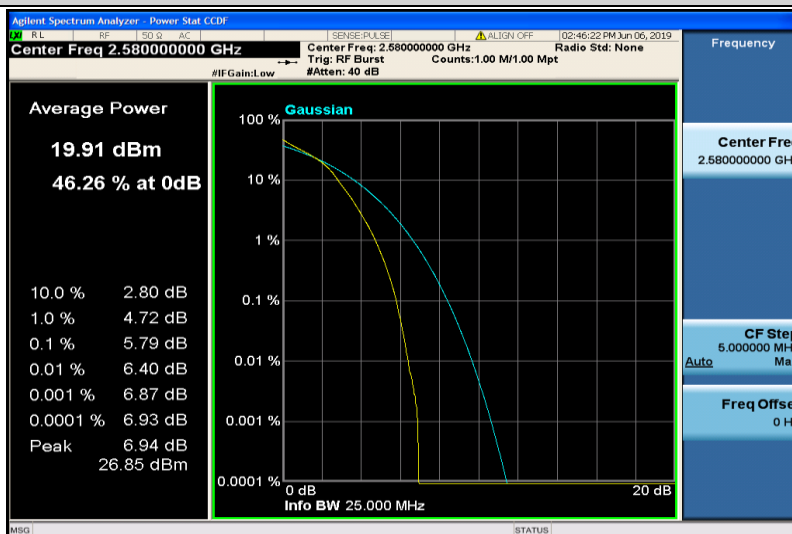
Band38-20MHz-16QAM-37850-100RB#0
