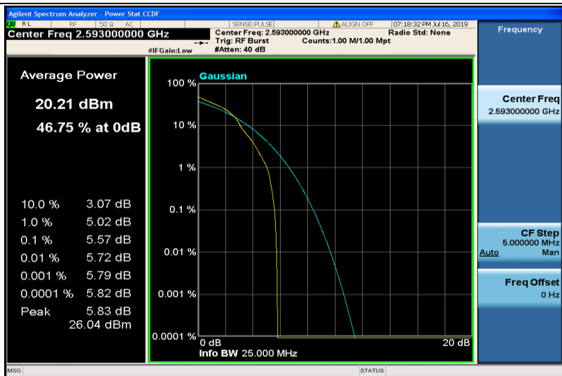
Band41-5MHz-16QAM-40620-1RB#0
