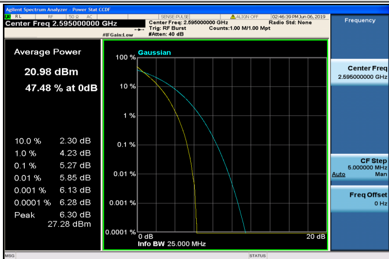
Band38-20MHz-QPSK-38000-100RB#0
