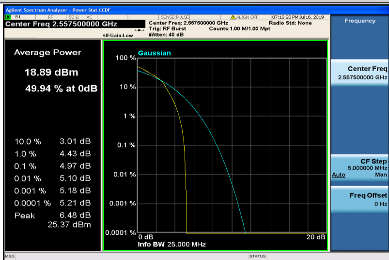
Band41-5MHz-16QAM-40265-25RB#0
