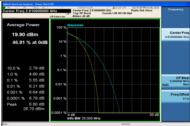
Band38-20MHz-16QAM-38150-100RB#0
