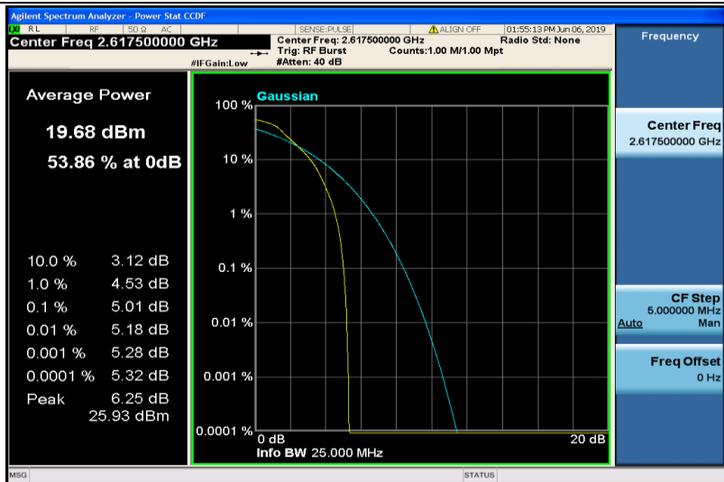
Band38-5MHz-QPSK-38225-25RB#0
