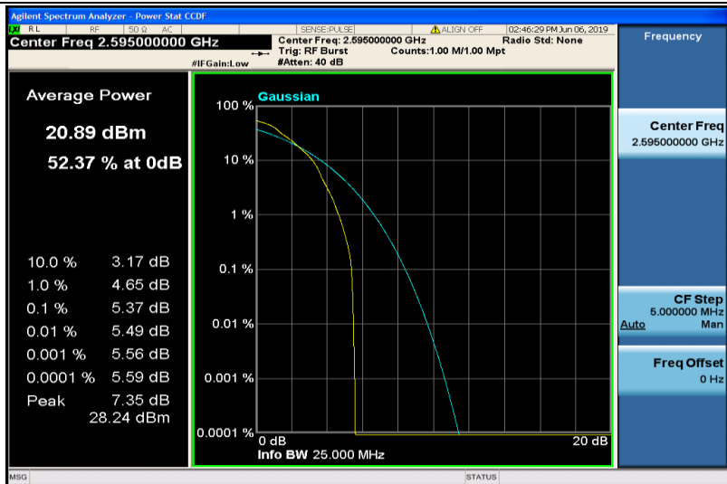
Band38-20MHz-QPSK-38000-1RB#0
