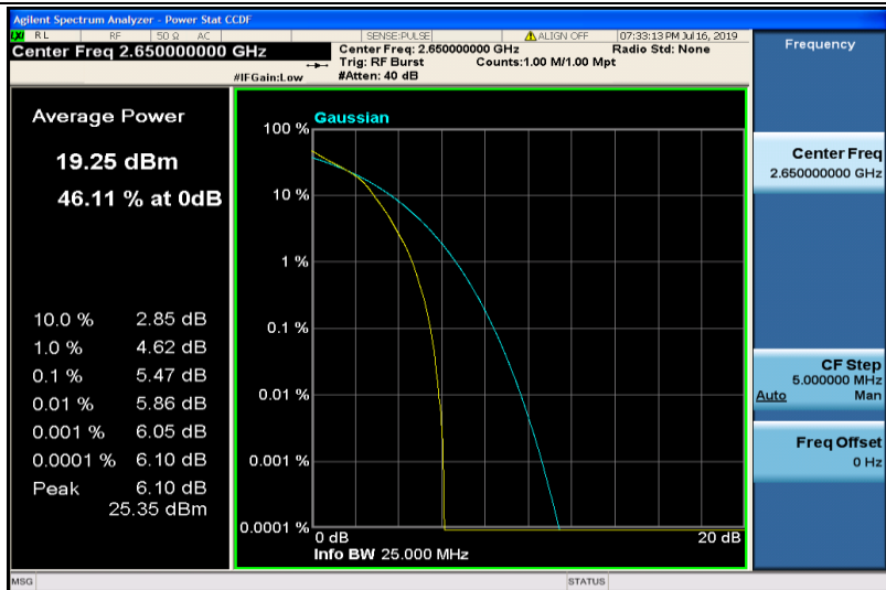
Band41-10MHz-16QAM-41190-50RB#0
