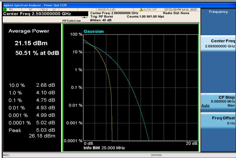
Band41-15MHz-QPSK-40620-1RB#0
