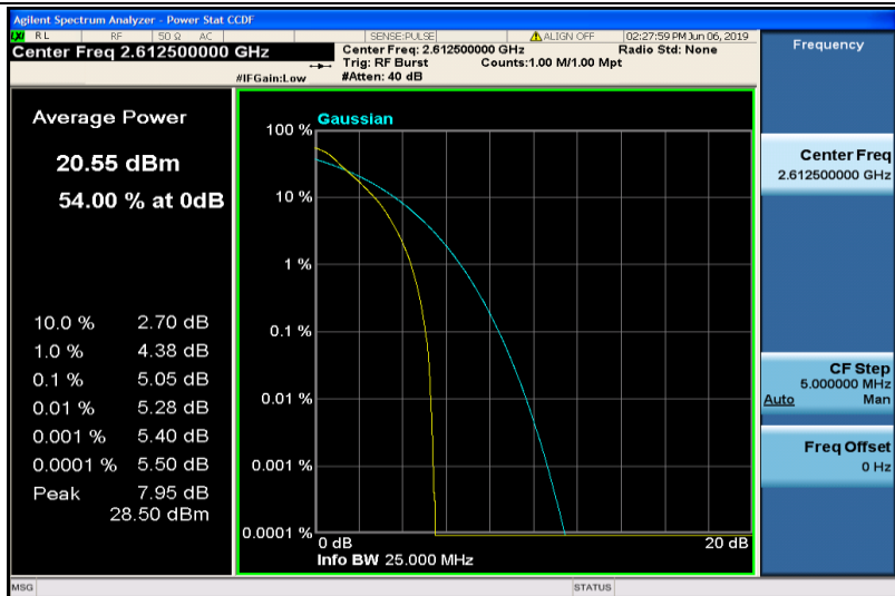
Band38-15MHz-QPSK-38175-75RB#0
