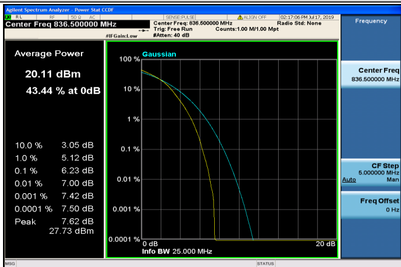
Band26-15MHz-16QAM-26915-75RB#0
