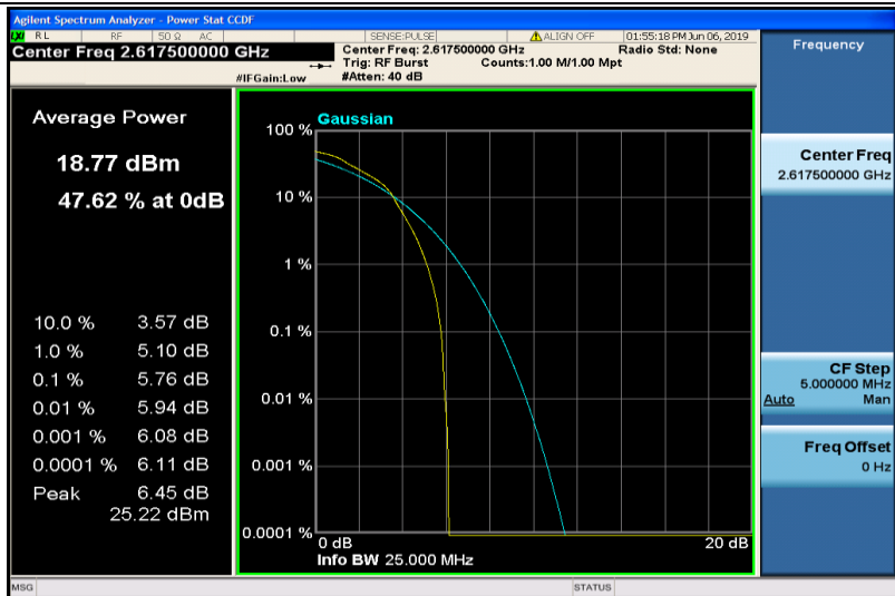
Band38-5MHz-16QAM-38225-25RB#0
