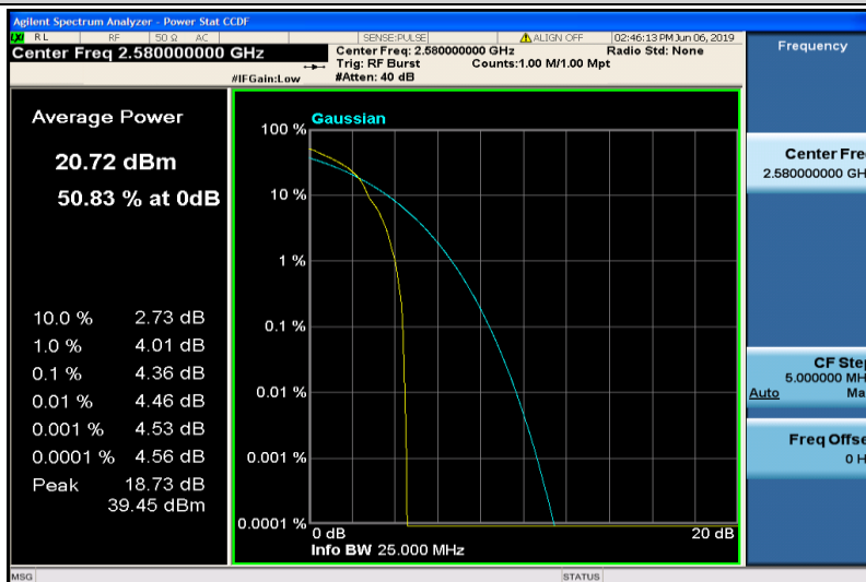
Band38-20MHz-16QAM-37850-1RB#0
