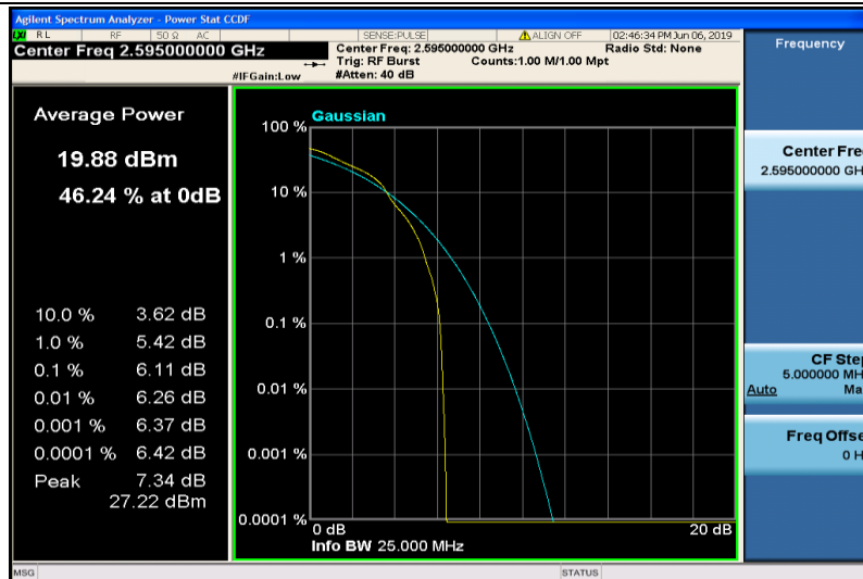
Band38-20MHz-16QAM-38000-1RB#0
