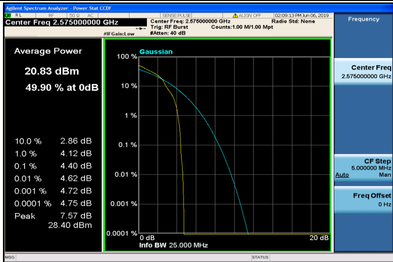
Band38-10MHz-16QAM-37800-1RB#0
