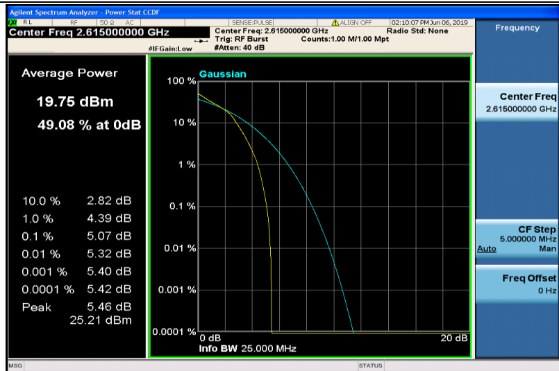
Band38-10MHz-16QAM-38200-50RB#0
