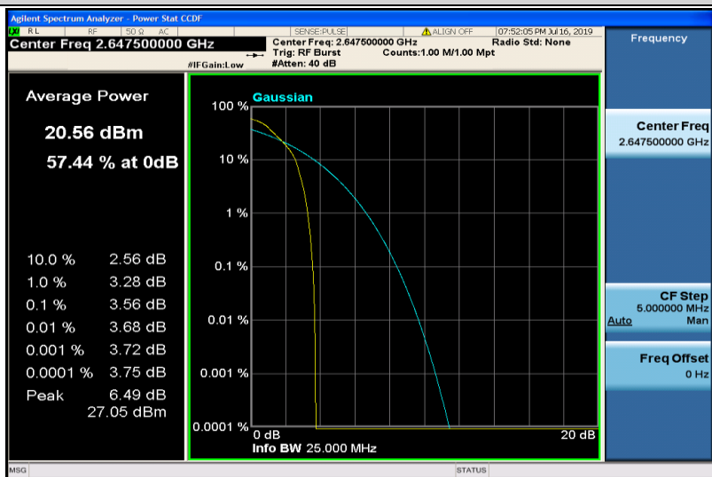
Band41-15MHz-QPSK-41165-1RB#0
