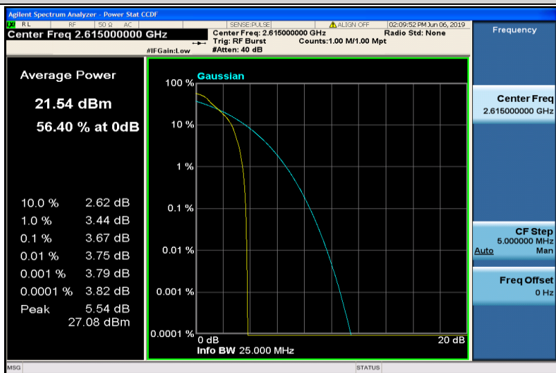
Band38-10MHz-QPSK-38200-1RB#0
