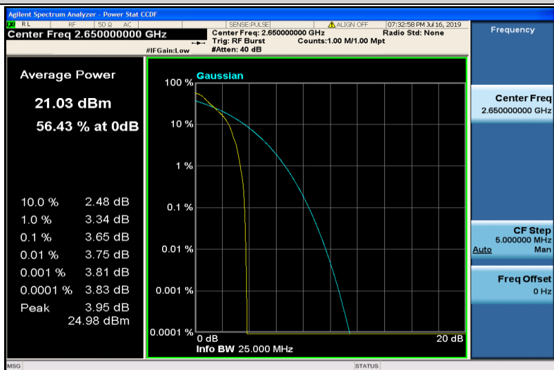
Band41-10MHz-QPSK-41190-1RB#0
