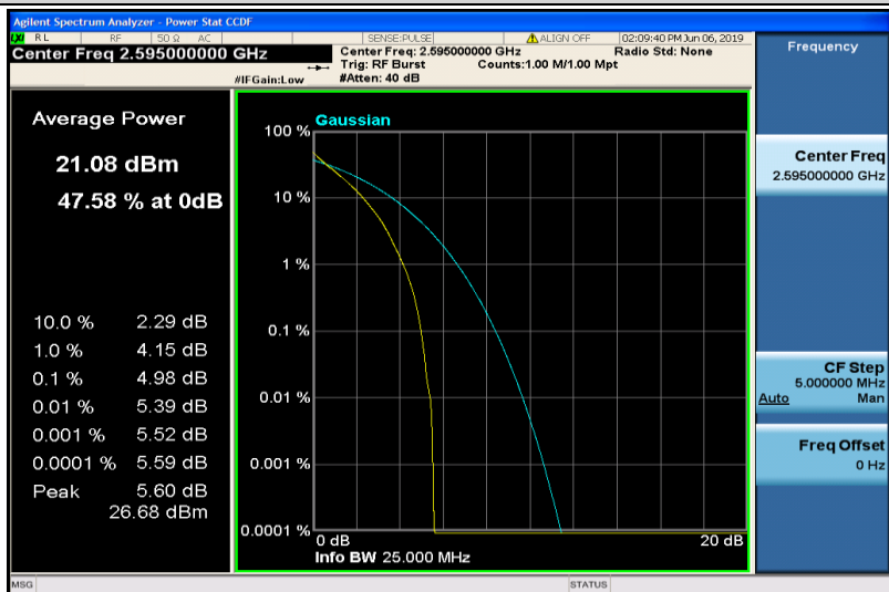
Band38-10MHz-QPSK-38000-50RB#0
