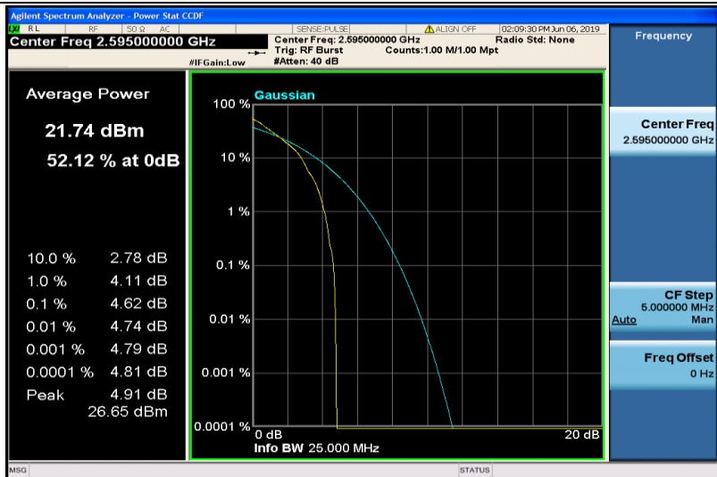
Band38-10MHz-QPSK-38000-1RB#0
