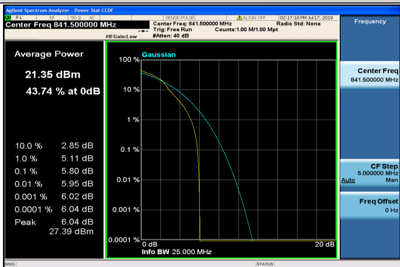
Band26-15MHz-16QAM-26965-1RB#0
