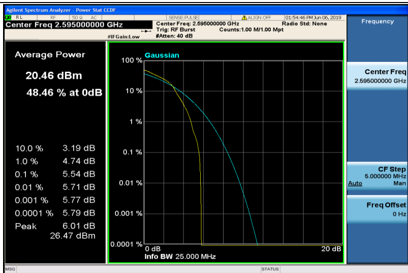
Band38-5MHz-16QAM-38000-1RB#0
