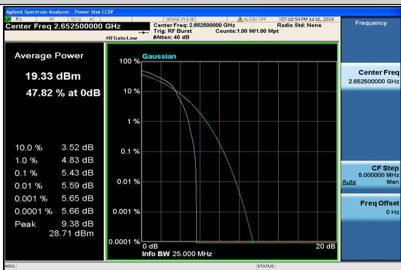
Band41-5MHz-16QAM-41215-1RB#0
