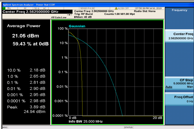
Band41-15MHz-QPSK-40315-1RB#0
