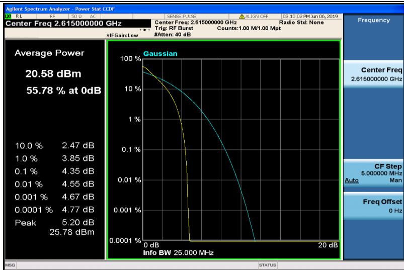
Band38-10MHz-QPSK-38200-50RB#0
