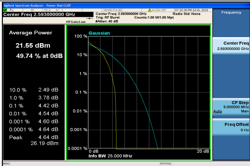
Band41-10MHz-QPSK-40620-1RB#0
