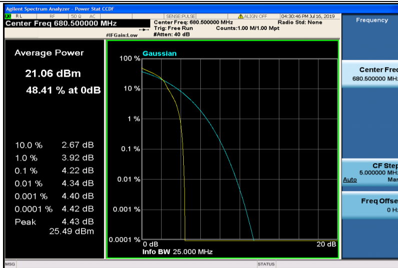
Band71-15MHz-16QAM-133297-1RB#0
