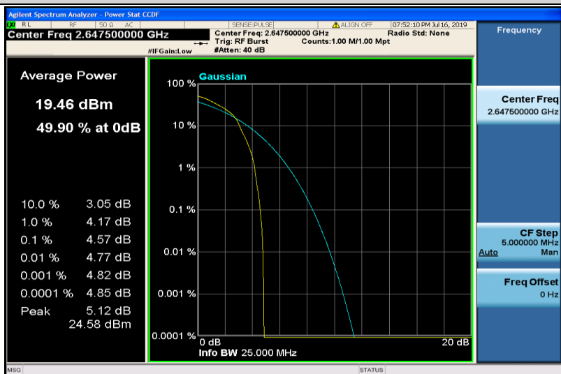
Band41-15MHz-16QAM-41165-1RB#0
