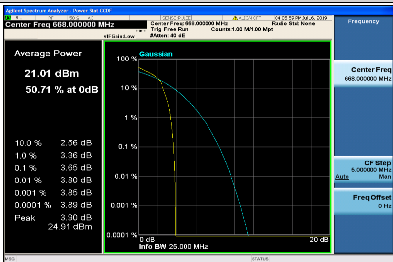
Band71-10MHz-16QAM-133172-1RB#0
