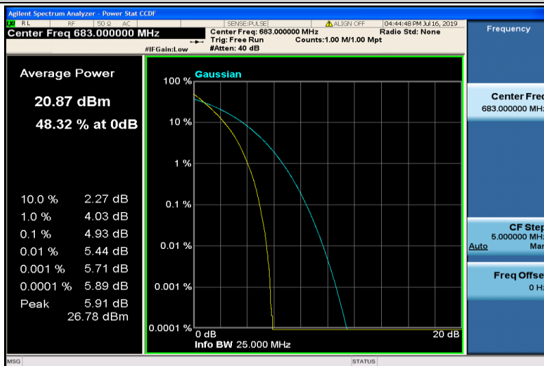
Band71-20MHz-QPSK-133322-100RB#0
