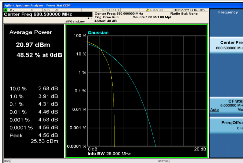
Band71-10MHz-16QAM-133297-1RB#0
