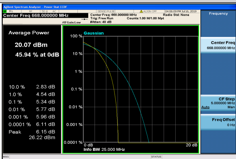
Band71-10MHz-16QAM-133172-50RB#0
