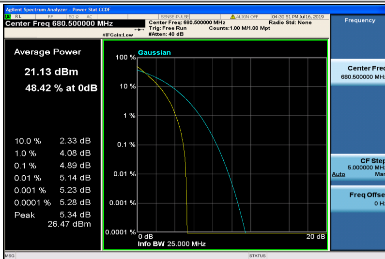
Band71-15MHz-QPSK-133297-75RB#0
