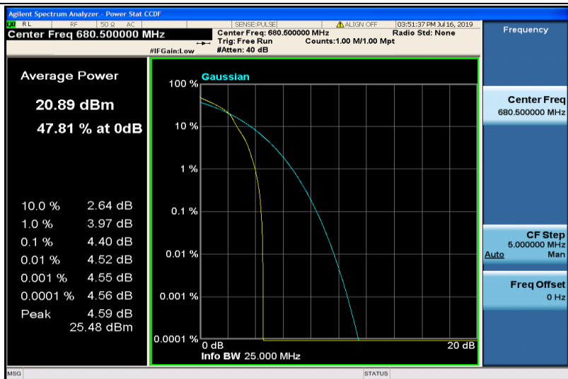
Band71-5MHz-16QAM-133297-1RB#0
