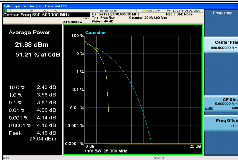
Band71-15MHz-QPSK-133397-1RB#0
