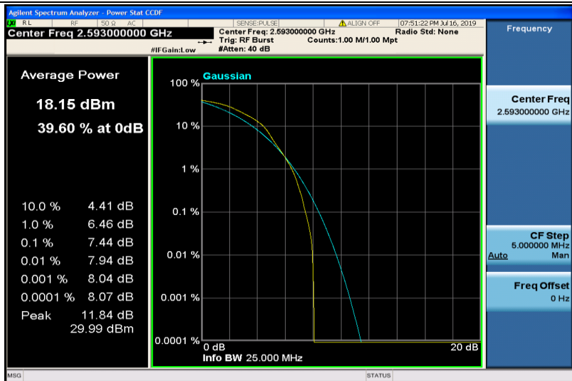
Band41-15MHz-16QAM-40620-1RB#0
