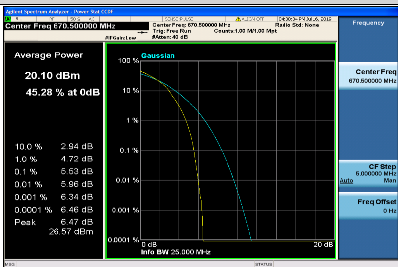
Band71-15MHz-16QAM-133197-75RB#0
