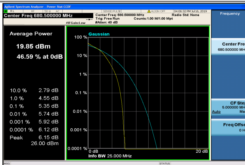
Band71-10MHz-16QAM-133297-50RB#0
