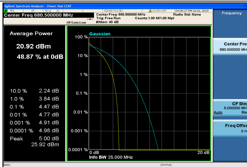
Band71-10MHz-QPSK-133297-50RB#0
