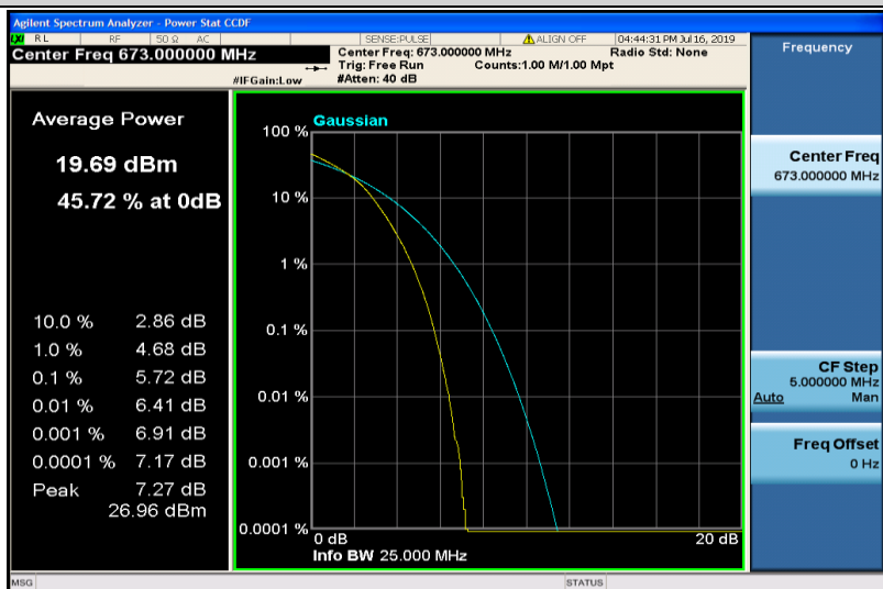
Band71-20MHz-16QAM-133222-100RB#0
