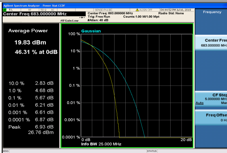
Band71-20MHz-16QAM-133322-100RB#0
