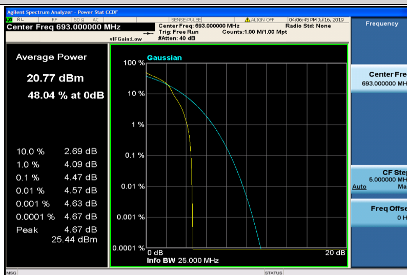
Band71-10MHz-16QAM-133422-1RB#0
