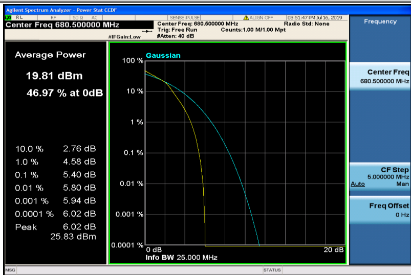
Band71-5MHz-16QAM-133297-25RB#0
