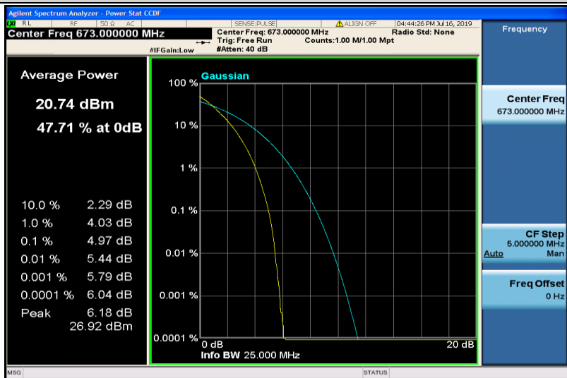
Band71-20MHz-QPSK-133222-100RB#0
