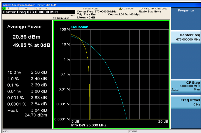
Band71-20MHz-16QAM-133222-1RB#0
