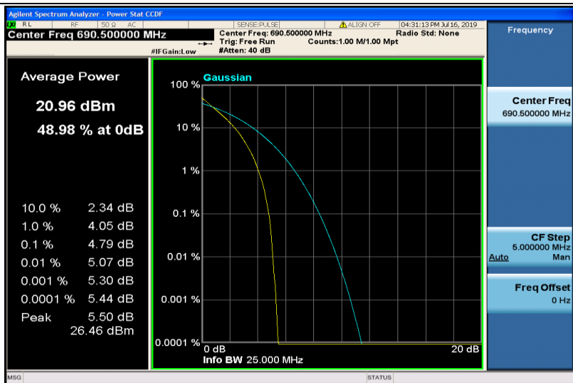
Band71-15MHz-QPSK-133397-75RB#0
