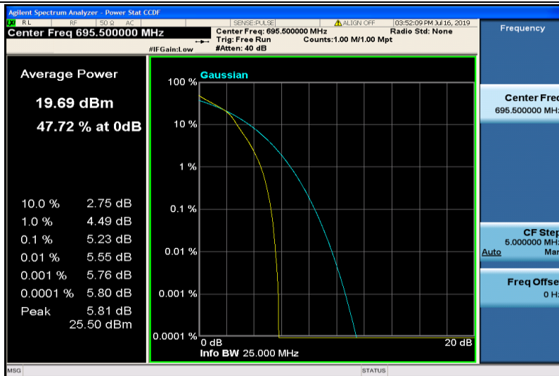
Band71-5MHz-16QAM-133447-25RB#0
