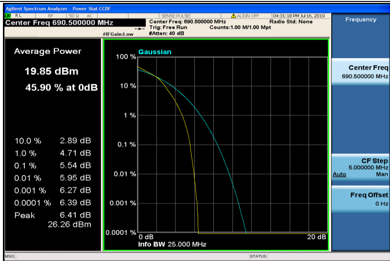
Band71-15MHz-16QAM-133397-75RB#0
