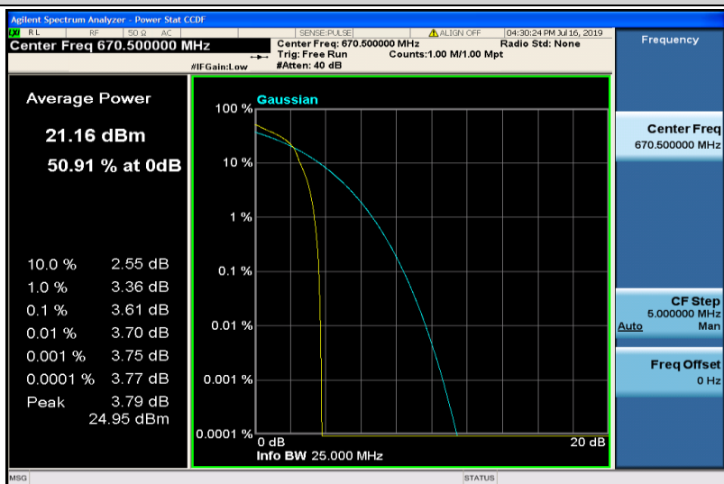
Band71-15MHz-16QAM-133197-1RB#0
