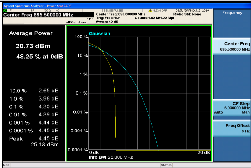
Band71-5MHz-16QAM-133447-1RB#0
