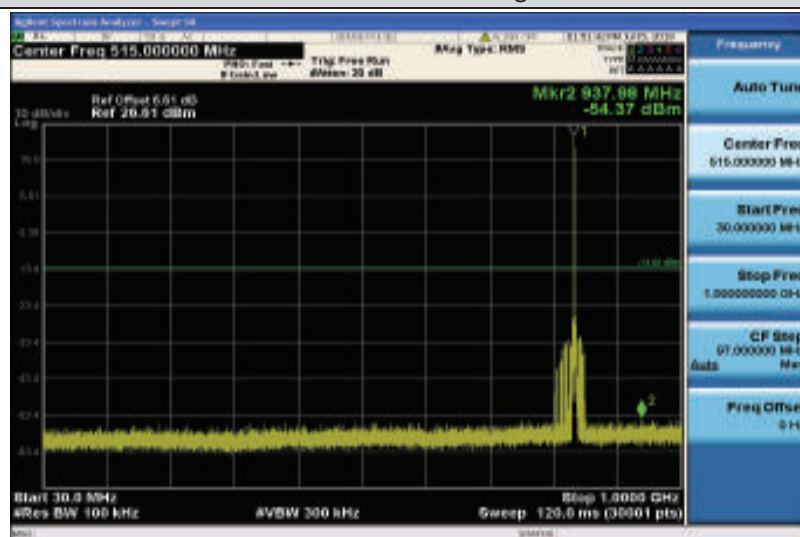
Band5-1.4MHz-QPSK-20525-1RB#0-Range1:30~1000MHz
