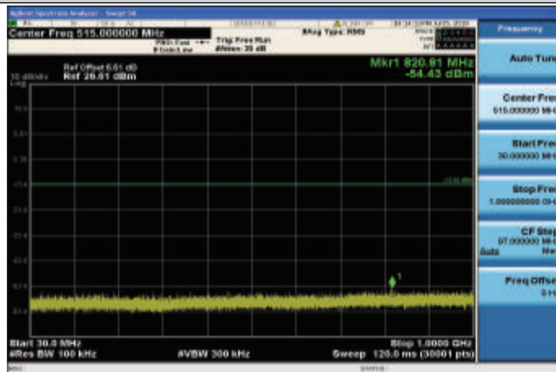
Band4-10MHz-16QAM-20350-1RB#0-Range1:30~1000MHz
