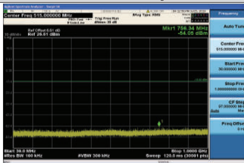
Band4-10MHz-16QAM-20175-1RB#0-Range1:30~1000MHz
