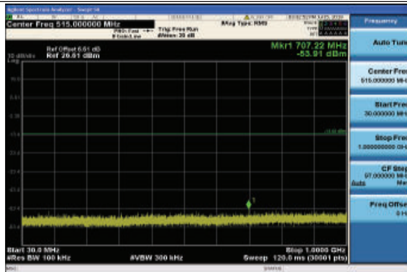
Band4-3MHz-16QAM-19965-1RB#0-Range1:30~1000MHz
