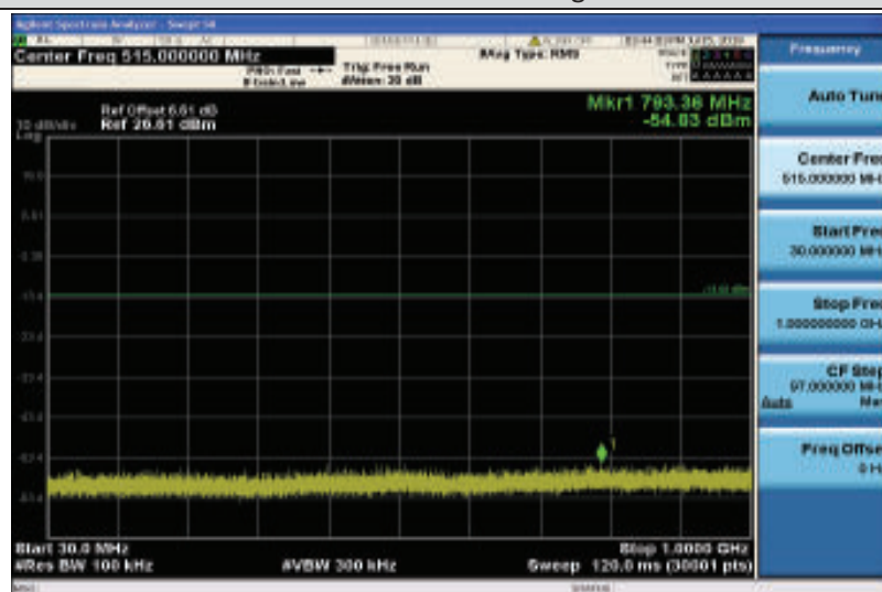
Band4-5MHz-16QAM-20175-1RB#0-Range1:30~1000MHz
