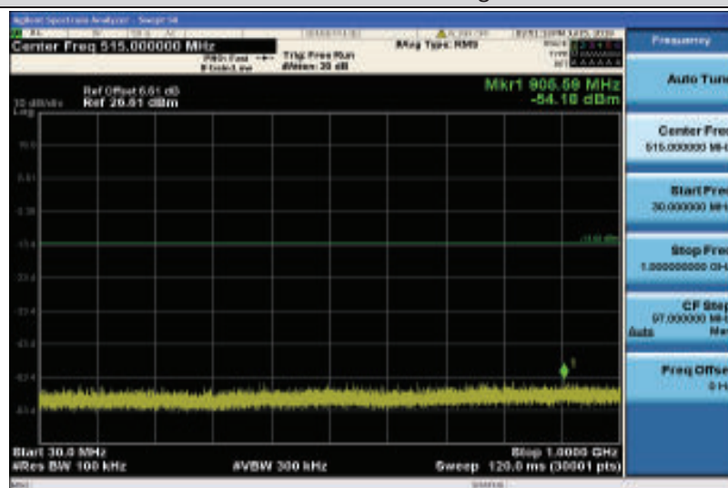
Band4-15MHz-16QAM-20175-1RB#0-Range1:30~1000MHz
