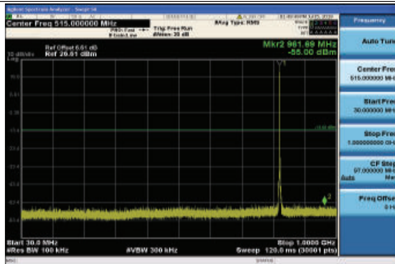
Band5-1.4MHz-QPSK-20407-1RB#0-Range1:30~1000MHz
