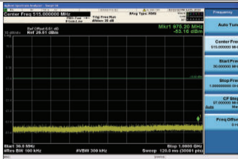
Band4-1.4MHz-16QAM-19957-1RB#0-Range1:30~1000MHz
