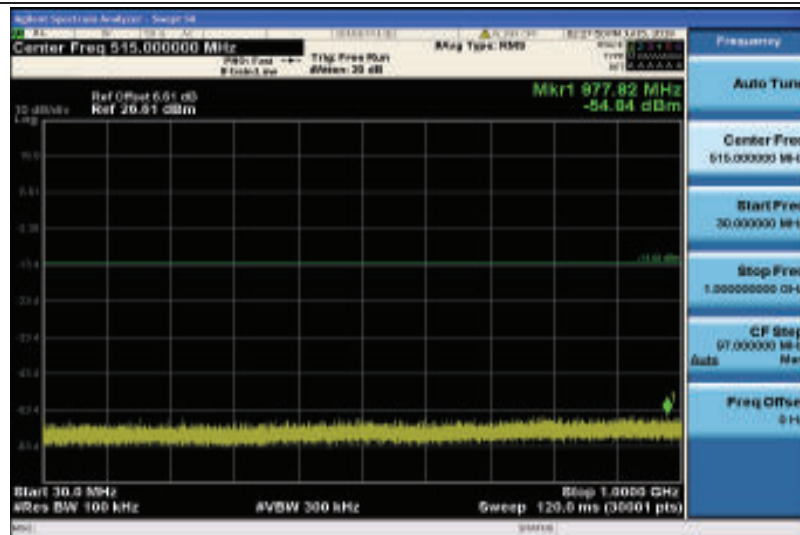
Band2-1.4MHz-16QAM-18607-1RB#0-Range1:30~1000MHz
