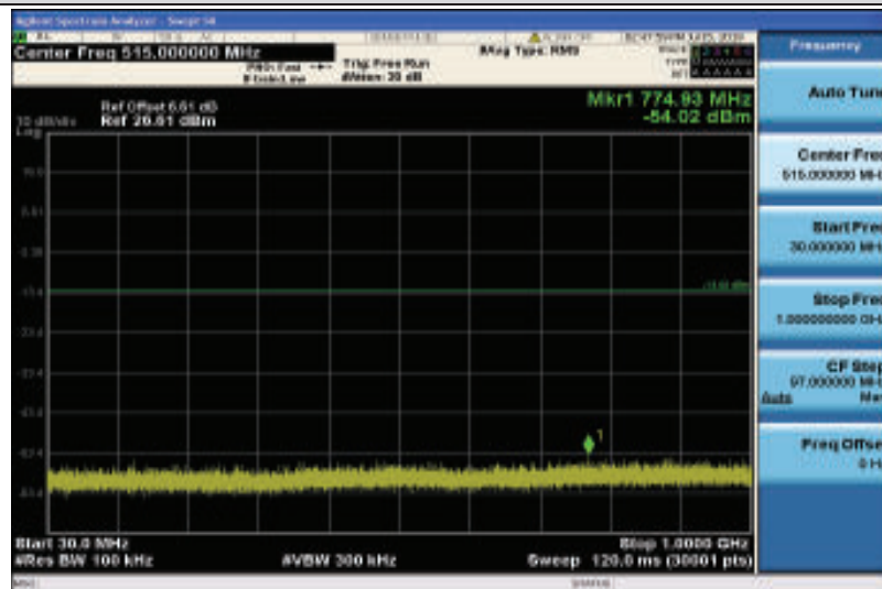
Band2-5MHz-16QAM-19175-1RB#0-Range1:30~1000MHz
