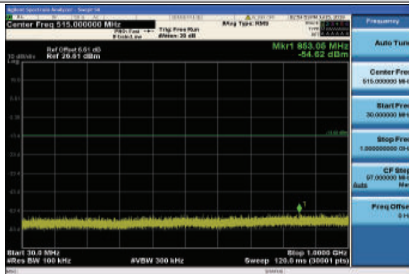
Band2-10MHz-16QAM-19150-1RB#0-Range1:30~1000MHz
