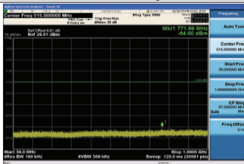
Band4-15MHz-QPSK-20175-1RB#0-Range1:30~1000MHz
