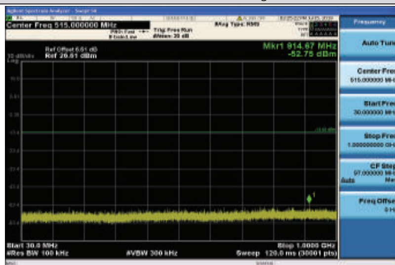
Band4-1.4MHz-16QAM-20175-1RB#0-Range1:30~1000MHz
