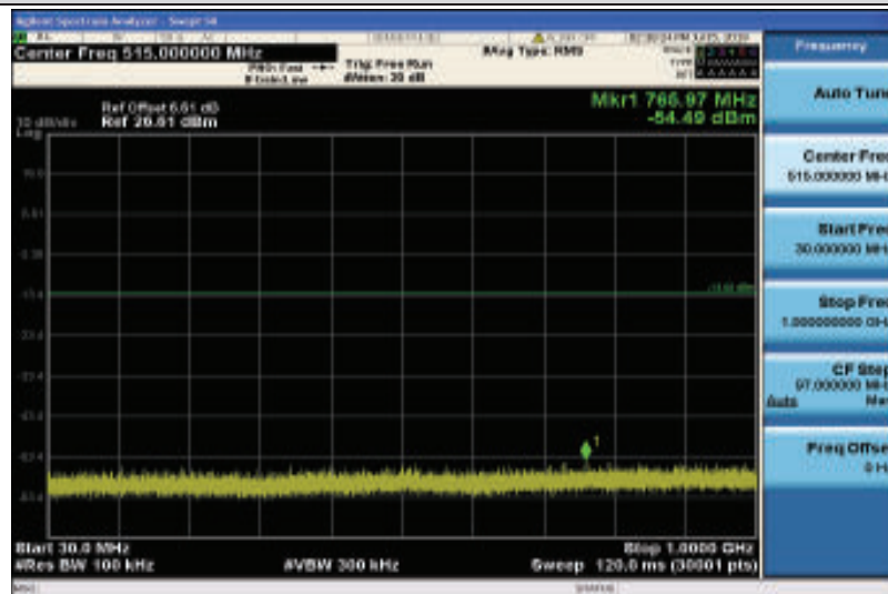
Band2-3MHz-16QAM-19185-1RB#0-Range1:30~1000MHz
