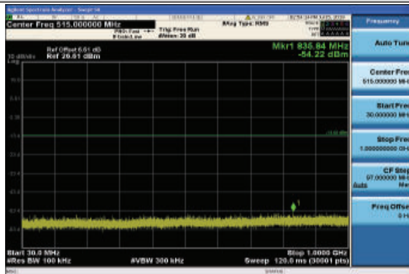
Band2-10MHz-QPSK-19150-1RB#0-Range1:30~1000MHz
