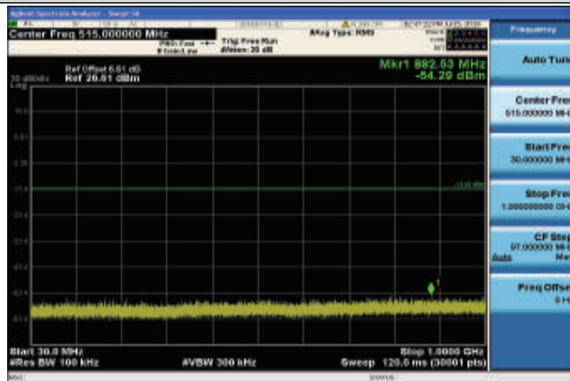
Band2-5MHz-QPSK-19175-1RB#0-Range1:30~1000MHz
