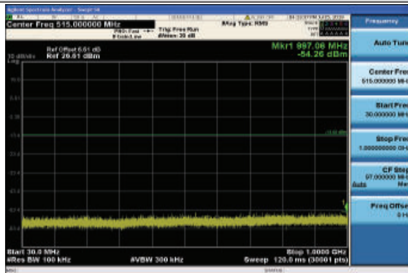
Band4-10MHz-QPSK-20350-1RB#0-Range1:30~1000MHz
