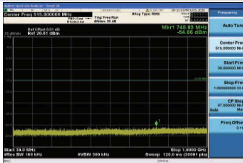
Band4-10MHz-16QAM-20000-1RB#0-Range1:30~1000MHz
