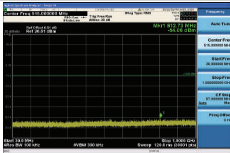
Band4-1.4MHz-QPSK-19957-1RB#0-Range1:30~1000MHz
