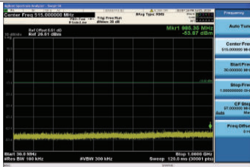
Band2-15MHz-QPSK-19125-1RB#0-Range1:30~1000MHz
