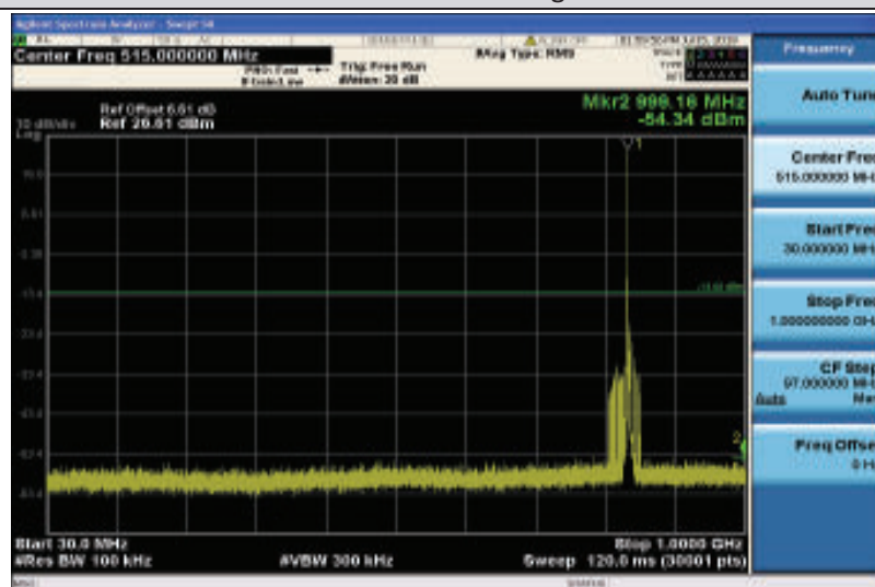
Band5-3MHz-QPSK-20525-1RB#0-Range1:30~1000MHz
