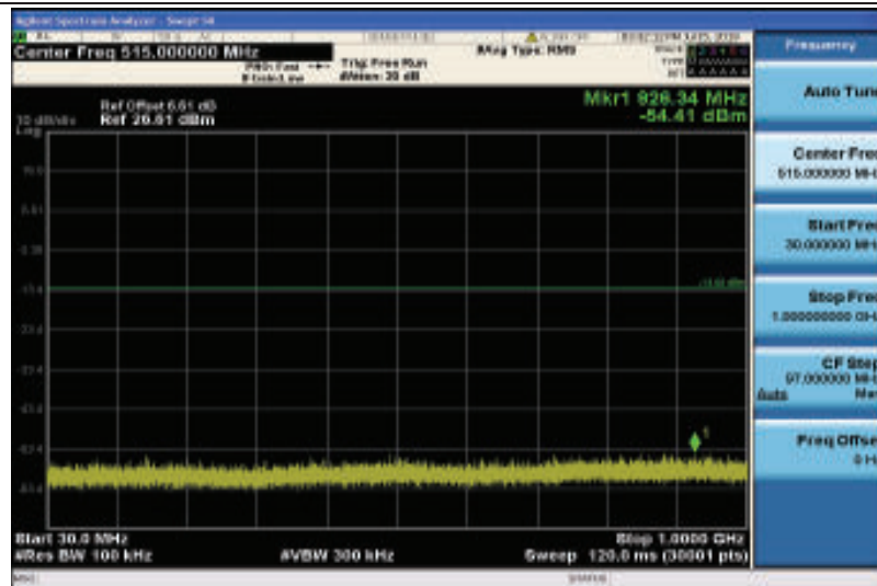
Band4-3MHz-QPSK-19965-1RB#0-Range1:30~1000MHz
