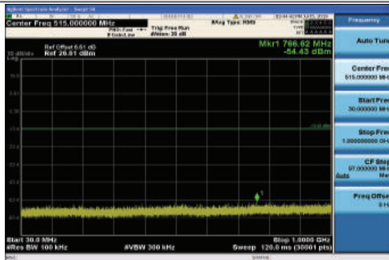
Band4-5MHz-QPSK-20375-1RB#0-Range1:30~1000MHz
