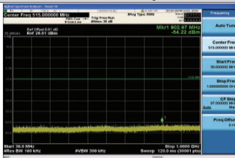
Band4-3MHz-16QAM-20175-1RB#0-Range1:30~1000MHz
