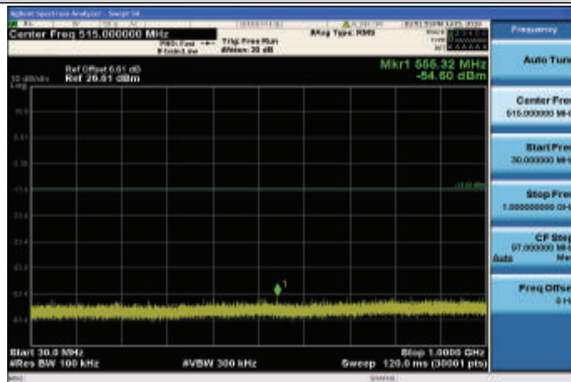
Band4-15MHz-QPSK-20325-1RB#0-Range1:30~1000MHz
