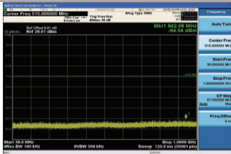
Band4-15MHz-16QAM-20325-1RB#0-Range1:30~1000MHz
