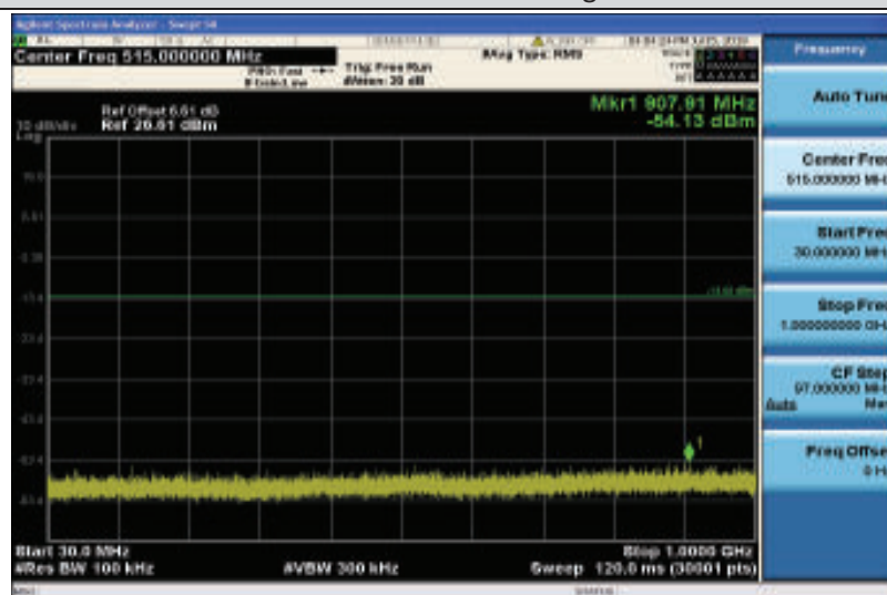
Band4-20MHz-16QAM-20175-1RB#0-Range1:30~1000MHz
