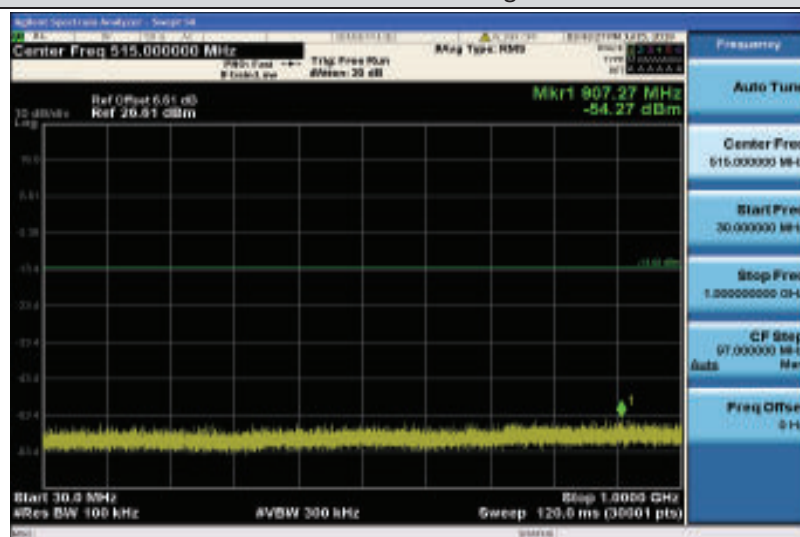
Band4-5MHz-QPSK-20175-1RB#0-Range1:30~1000MHz
