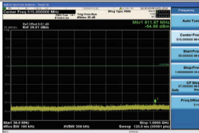
Band2-1.4MHz-16QAM-19193-1RB#0-Range1:30~1000MHz
