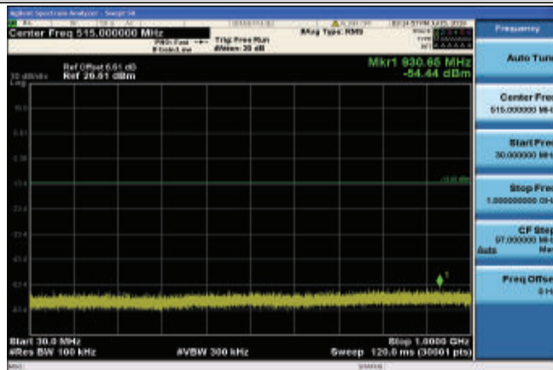
Band2-20MHz-QPSK-19100-1RB#0-Range1:30~1000MHz
