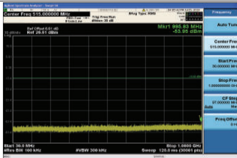
Band4-20MHz-16QAM-20300-1RB#0-Range1:30~1000MHz
