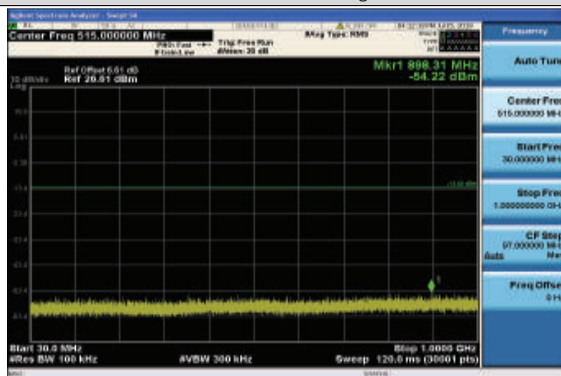
Band4-10MHz-QPSK-20175-1RB#0-Range1:30~1000MHz
