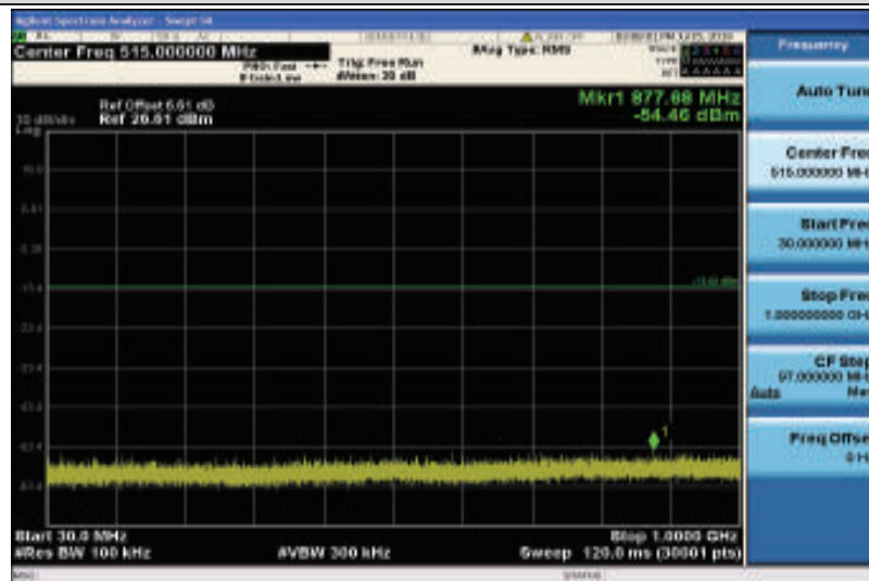
Band2-15MHz-16QAM-19125-1RB#0-Range1:30~1000MHz
