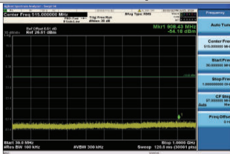
Band4-3MHz-QPSK-20175-1RB#0-Range1:30~1000MHz
