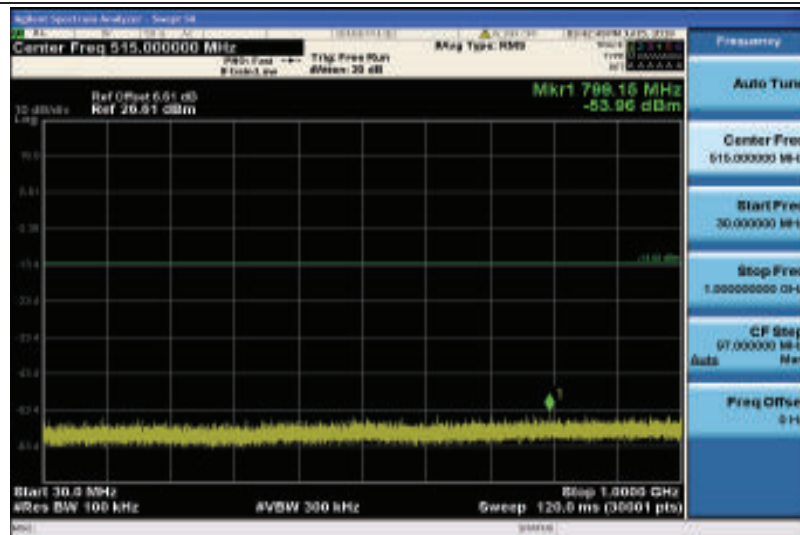
Band4-5MHz-16QAM-19975-1RB#0-Range1:30~1000MHz
