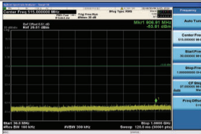
Band4-15MHz-QPSK-20025-1RB#0-Range1:30~1000MHz
