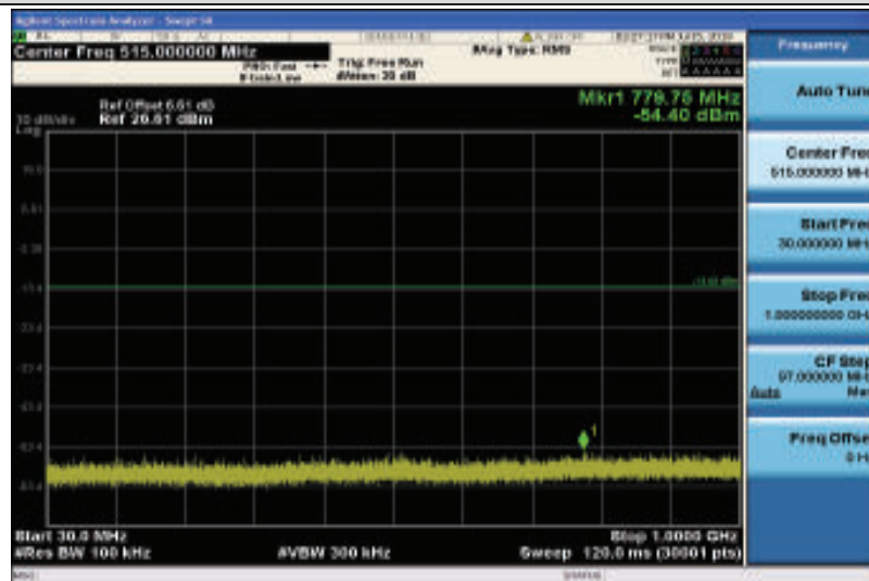
Band4-1.4MHz-16QAM-20393-1RB#0-Range1:30~1000MHz
