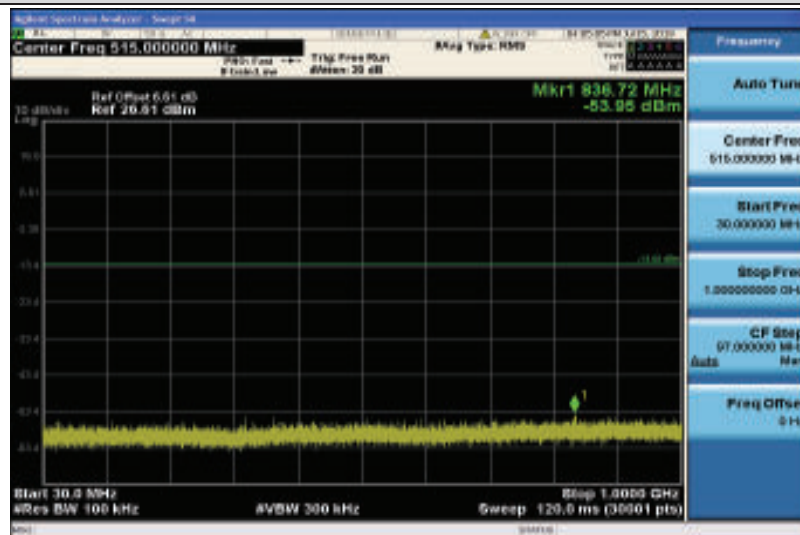
Band4-20MHz-QPSK-20300-1RB#0-Range1:30~1000MHz
