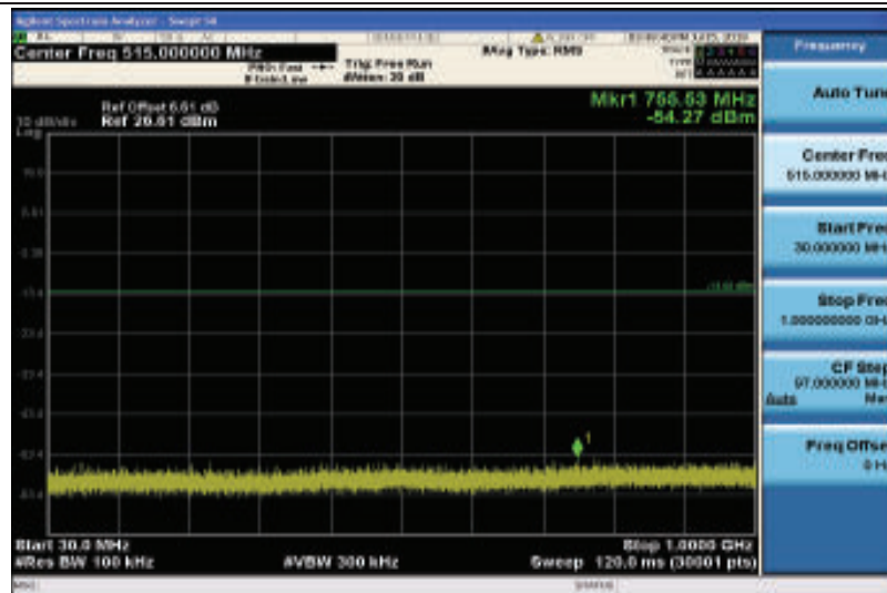
Band4-15MHz-16QAM-20025-1RB#0-Range1:30~1000MHz
