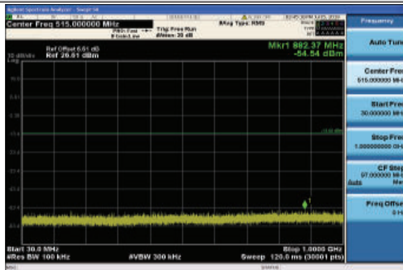
Band4-5MHz-16QAM-20375-1RB#0-Range1:30~1000MHz
