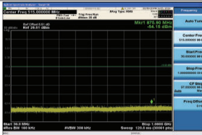
Band4-20MHz-16QAM-20050-1RB#0-Range1:30~1000MHz
