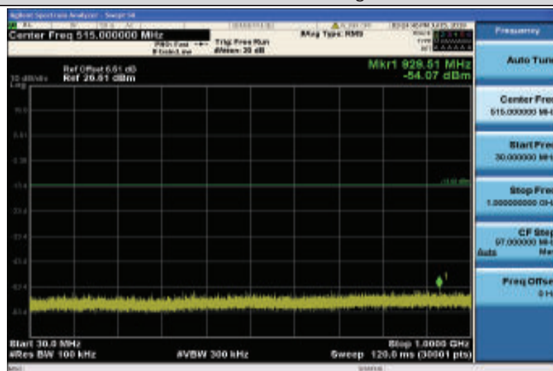
Band4-1.4MHz-QPSK-20175-1RB#0-Range1:30~1000MHz
