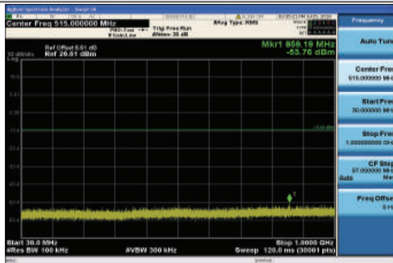
Band4-3MHz-QPSK-20385-1RB#0-Range1:30~1000MHz
