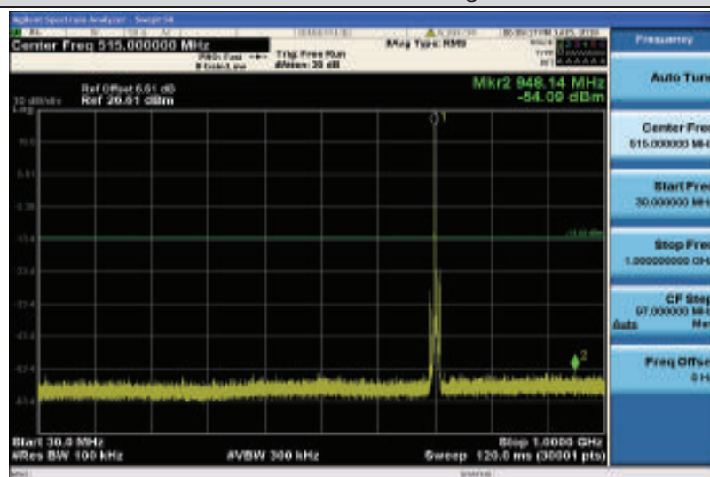
Band17-5MHz-16QAM-23790-1RB#0-Range1:30~1000MHz
