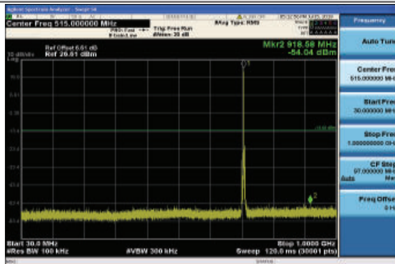
Band12-3MHz-16QAM-23165-1RB#0-Range1:30~1000MHz
