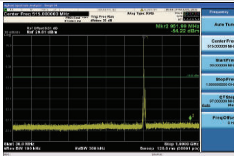
Band12-5MHz-16QAM-23155-1RB#0-Range1:30~1000MHz
