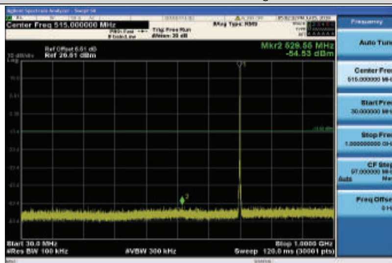
Band12-1.4MHz-16QAM-23095-1RB#0-Range1:30~1000MHz
