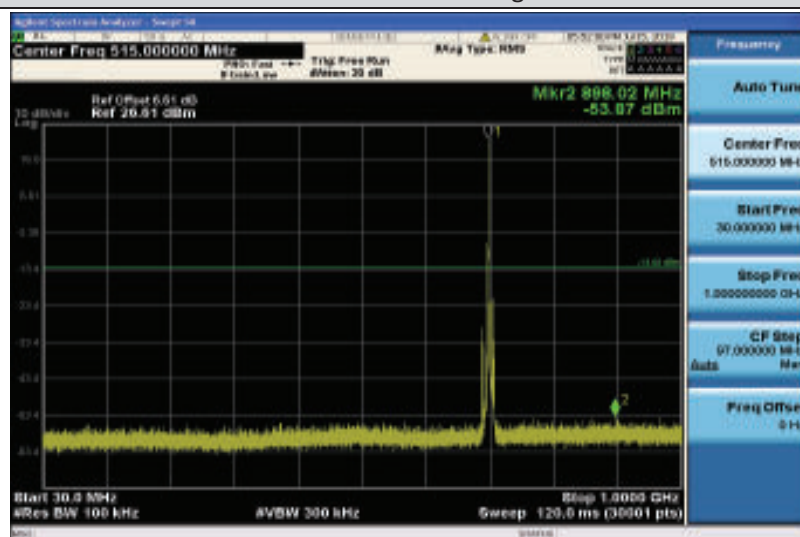
Band12-5MHz-QPSK-23095-1RB#0-Range1:30~1000MHz
