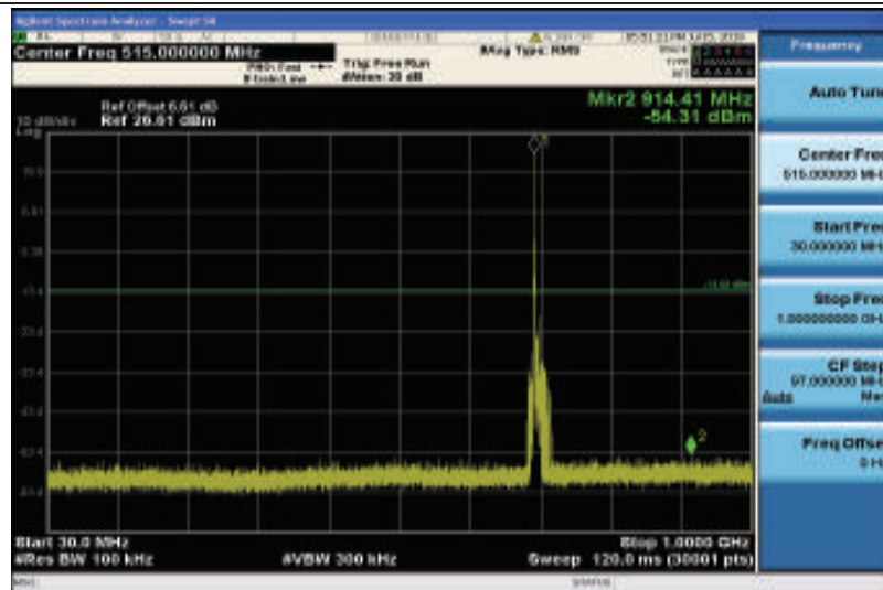
Band12-5MHz-16QAM-23035-1RB#0-Range1:30~1000MHz
