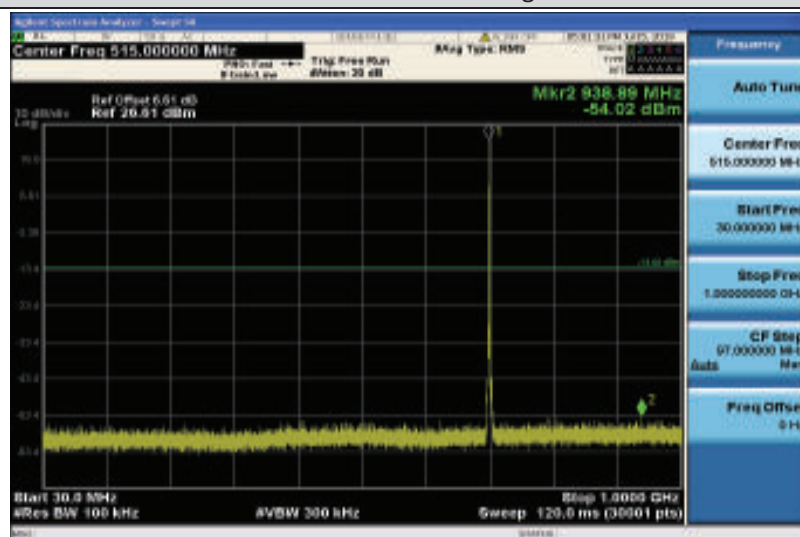
Band12-1.4MHz-QPSK-23095-1RB#0-Range1:30~1000MHz
