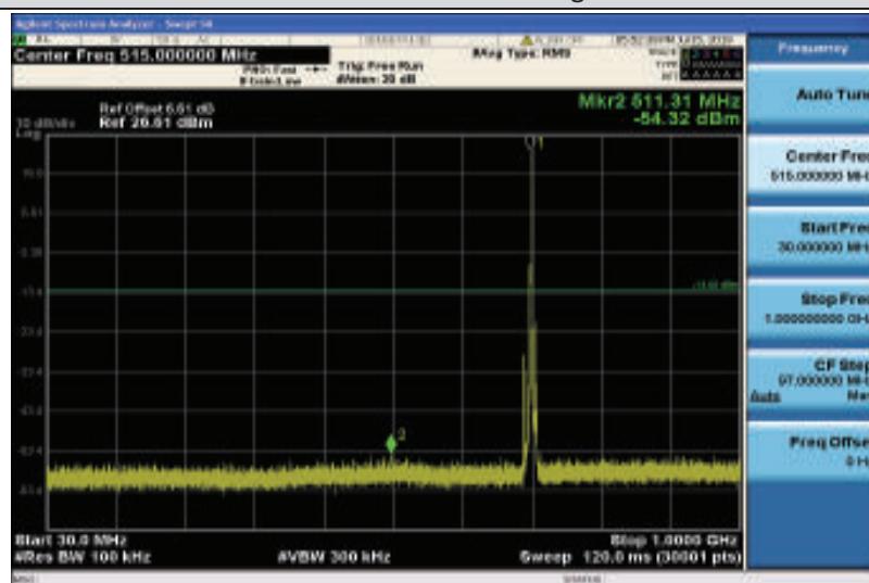
Band12-5MHz-16QAM-23095-1RB#0-Range1:30~1000MHz
