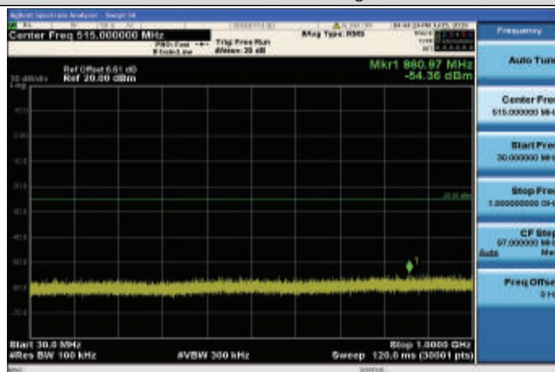
Band7-15MHz-QPSK-21100-1RB#0-Range1:30~1000MHz
