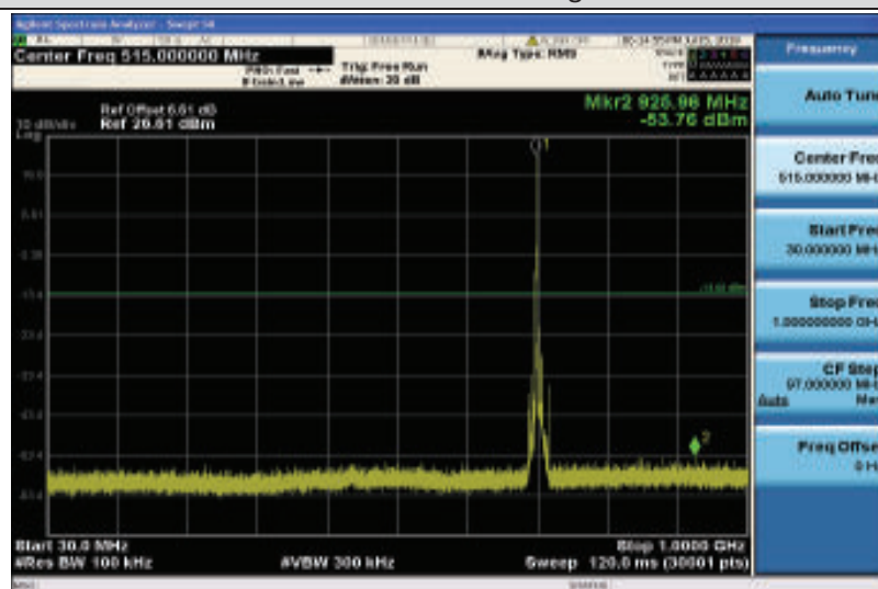
Band17-10MHz-QPSK-23790-1RB#0-Range1:30~1000MHz
