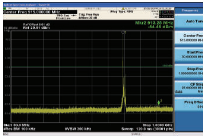
Band12-10MHz-16QAM-23060-1RB#0-Range1:30~1000MHz
