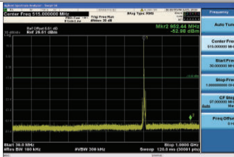
Band17-5MHz-QPSK-23825-1RB#0-Range1:30~1000MHz
