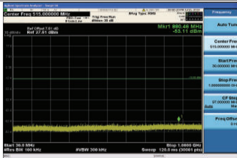
Band25-3MHz-QPSK-26055-1RB#0-30~1000MHz
