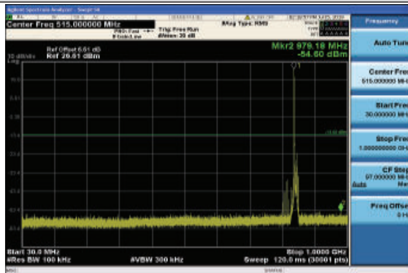
Band5-10MHz-QPSK-20600-1RB#0-Range1:30~1000MHz
