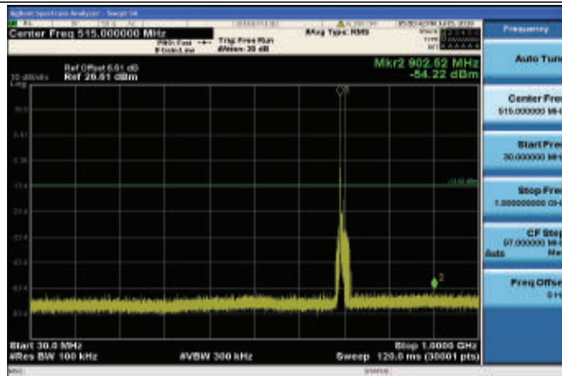
Band12-5MHz-QPSK-23035-1RB#0-Range1:30~1000MHz
