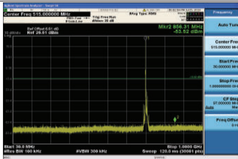
Band12-10MHz-16QAM-23130-1RB#0-Range1:30~1000MHz
