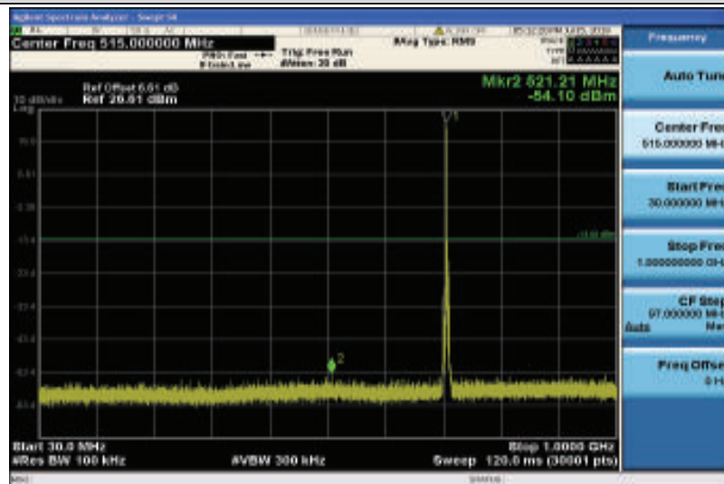
Band12-3MHz-QPSK-23165-1RB#0-Range1:30~1000MHz
