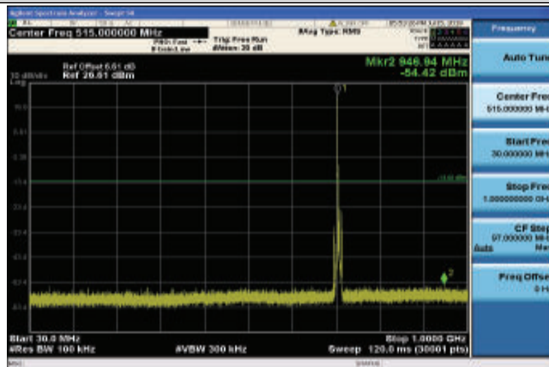
Band12-5MHz-QPSK-23155-1RB#0-Range1:30~1000MHz
