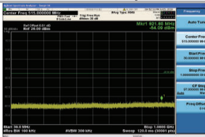
Band7-20MHz-16QAM-21100-1RB#0-Range1:30~1000MHz
