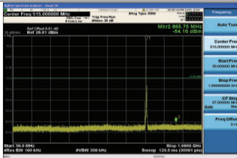
Band12-1.4MHz-QPSK-23173-1RB#0-Range1:30~1000MHz
