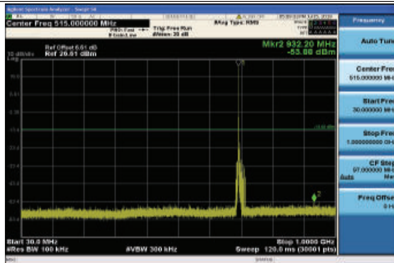
Band12-3MHz-QPSK-23025-1RB#0-Range1:30~1000MHz
