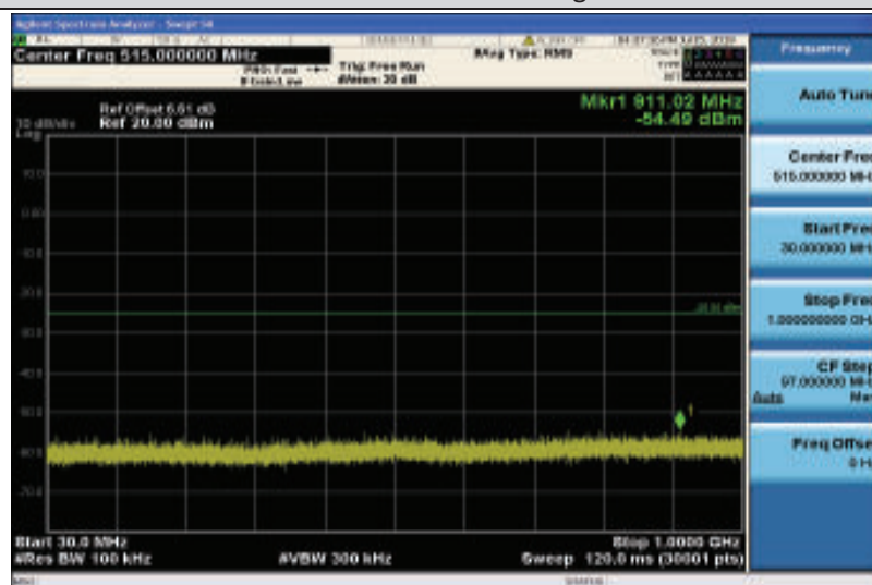
Band7-10MHz-16QAM-21100-1RB#0-Range1:30~1000MHz
