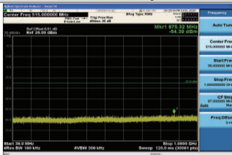
Band7-5MHz-16QAM-21100-1RB#0-Range1:30~1000MHz
