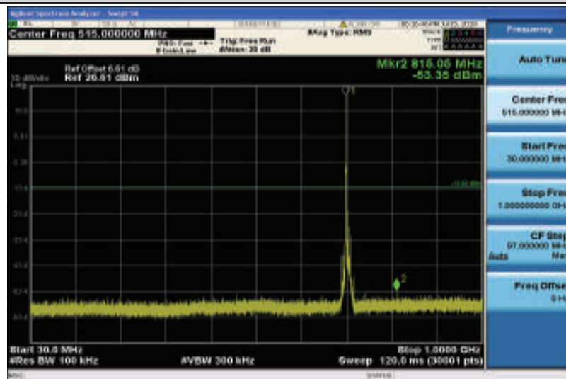
Band17-10MHz-16QAM-23800-1RB#0-Range1:30~1000MHz
