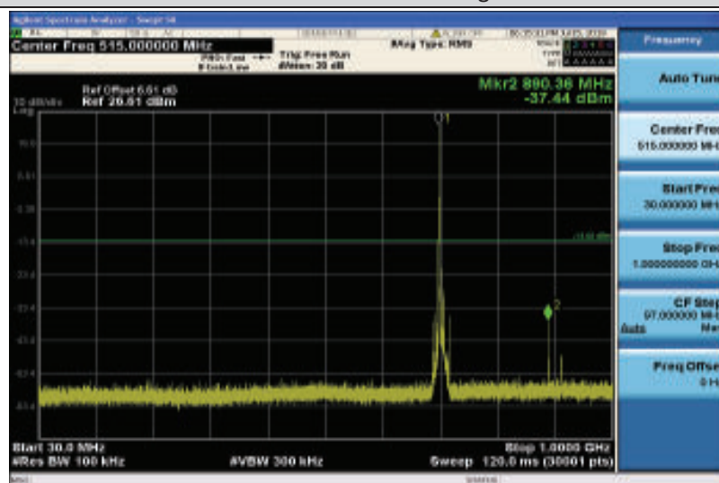
Band17-10MHz-16QAM-23790-1RB#0-Range1:30~1000MHz
