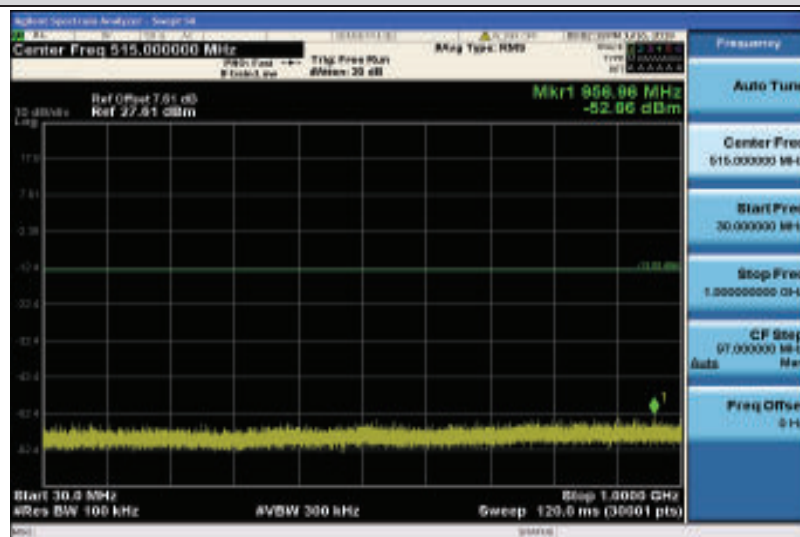
Band25-1.4MHz-QPSK-26683-1RB#0-30~1000MHz
