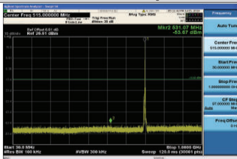
Band12-3MHz-16QAM-23095-1RB#0-Range1:30~1000MHz
