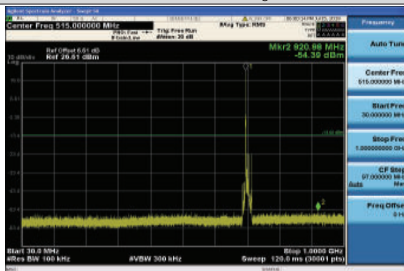
Band12-10MHz-QPSK-23095-1RB#0-Range1:30~1000MHz
