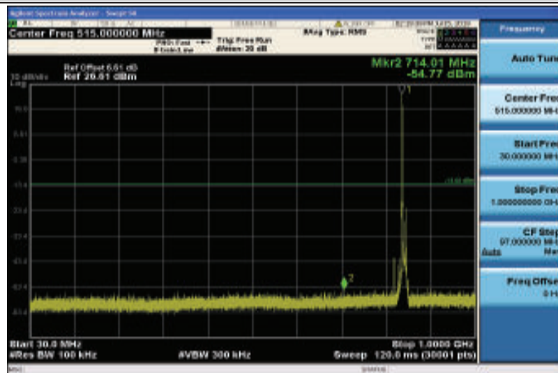
Band5-10MHz-16QAM-20600-1RB#0-Range1:30~1000MHz
