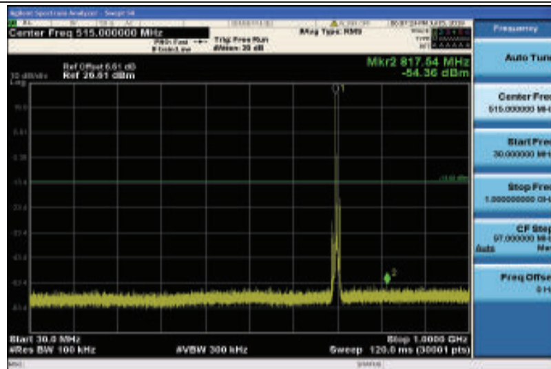
Band17-5MHz-QPSK-23755-1RB#0-Range1:30~1000MHz
