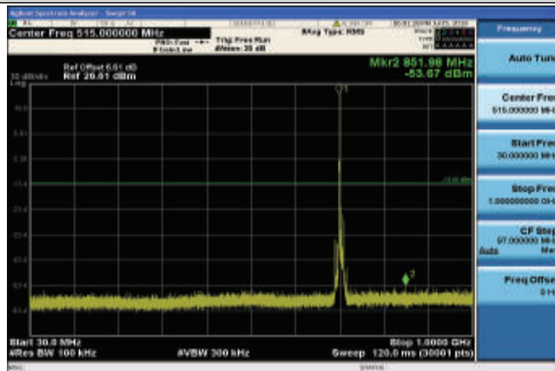
Band12-10MHz-QPSK-23130-1RB#0-Range1:30~1000MHz
