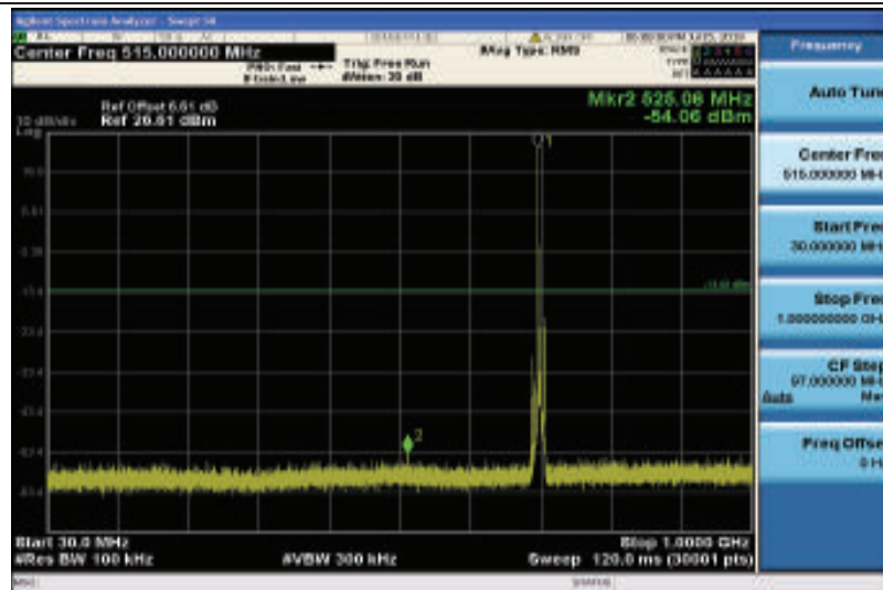
Band17-5MHz-16QAM-23755-1RB#0-Range1:30~1000MHz
