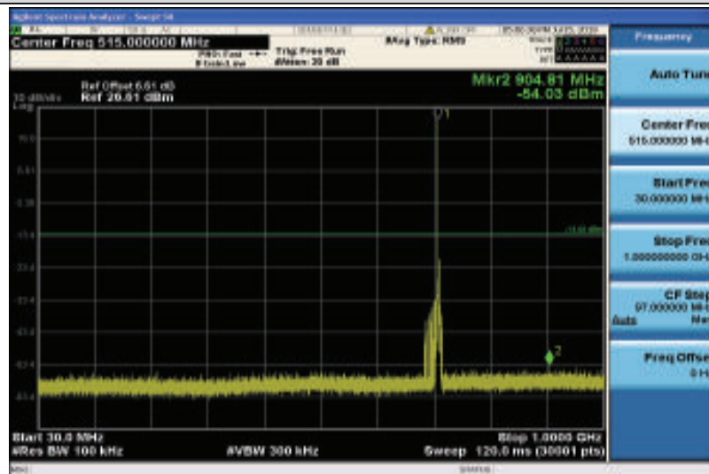
Band12-1.4MHz-16QAM-23173-1RB#0-Range1:30~1000MHz
