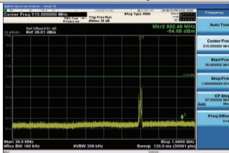
Band17-5MHz-QPSK-23790-1RB#0-Range1:30~1000MHz
