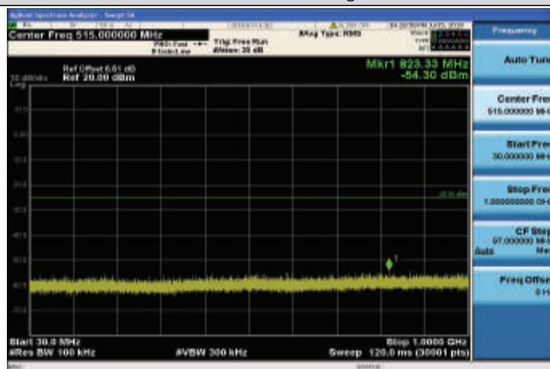
Band7-5MHz-QPSK-21100-1RB#0-Range1:30~1000MHz
