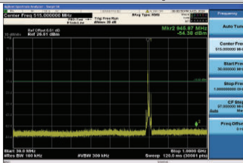
Band12-10MHz-16QAM-23095-1RB#0-Range1:30~1000MHz
