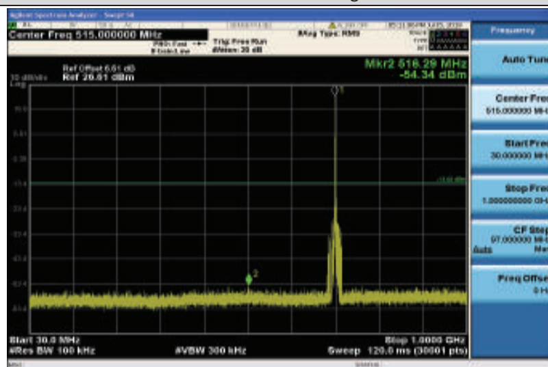
Band12-3MHz-QPSK-23095-1RB#0-Range1:30~1000MHz
