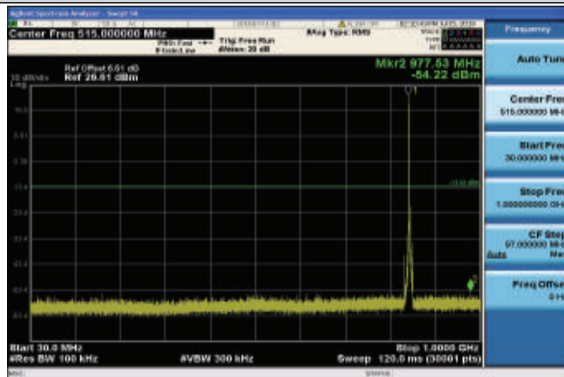
Band5-5MHz-QPSK-20625-1RB#0-Range1:30~1000MHz
