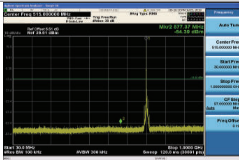
Band17-10MHz-QPSK-23800-1RB#0-Range1:30~1000MHz
