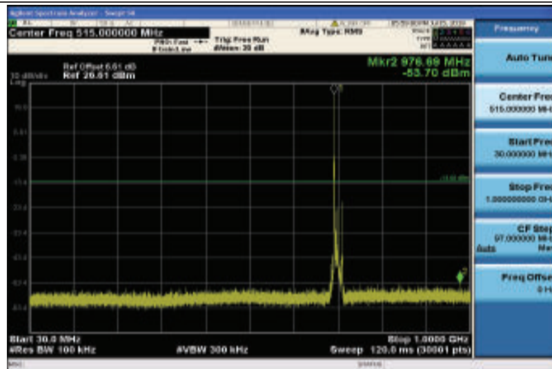
Band12-10MHz-QPSK-23060-1RB#0-Range1:30~1000MHz
