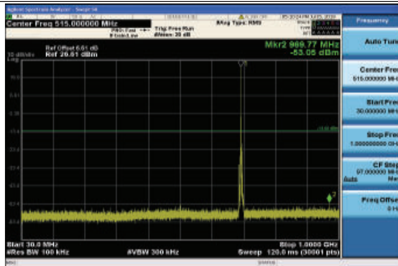
Band12-3MHz-16QAM-23025-1RB#0-Range1:30~1000MHz
