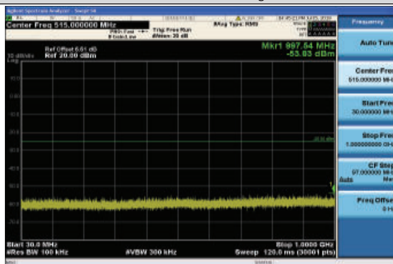
Band7-15MHz-16QAM-21100-1RB#0-Range1:30~1000MHz
