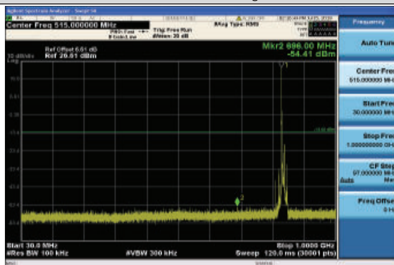
Band5-10MHz-QPSK-20525-1RB#0-Range1:30~1000MHz
