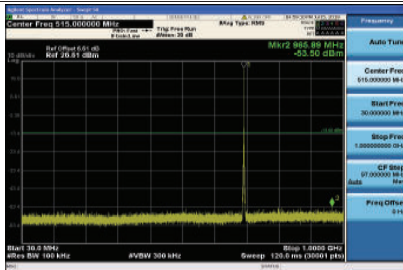
Band12-1.4MHz-16QAM-23017-1RB#0-Range1:30~1000MHz
