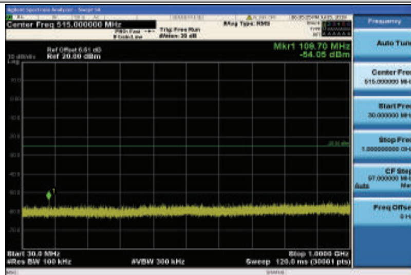
Band38-10MHz-16QAM-38200-1RB#0-Range1:30~1000MHz
