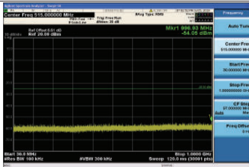
Band38-15MHz-16QAM-38175-1RB#0-Range1:30~1000MHz
