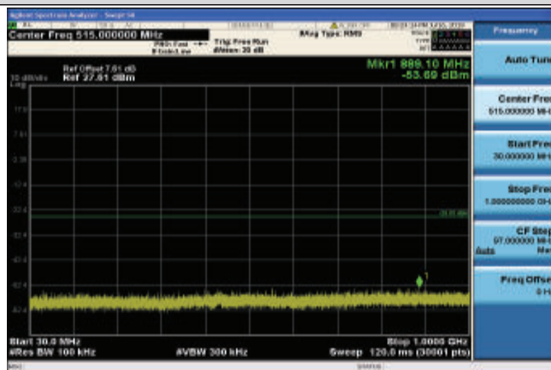
Band41-5MHz-QPSK-40620-1RB#0-30~1000MHz
