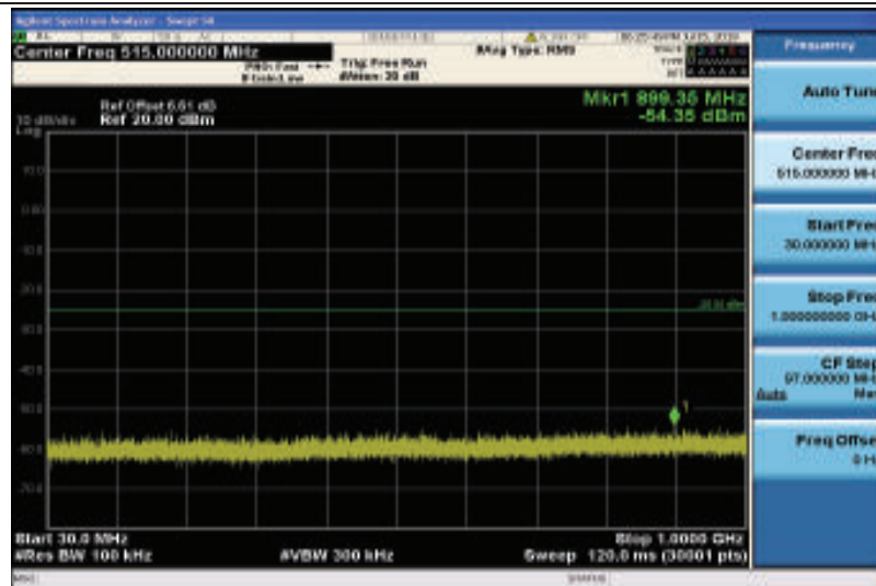
Band38-5MHz-16QAM-37775-1RB#0-Range1:30~1000MHz
