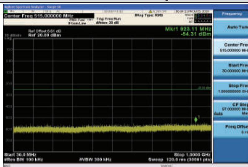
Band38-10MHz-16QAM-38000-1RB#0-Range1:30~1000MHz
