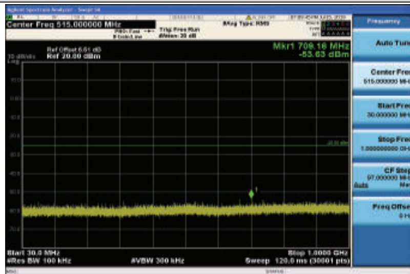
Band38-20MHz-QPSK-38150-1RB#0-Range1:30~1000MHz
