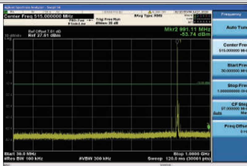
Band26-1.4MHz-QPSK-26915-1RB#0-30~1000MHz
