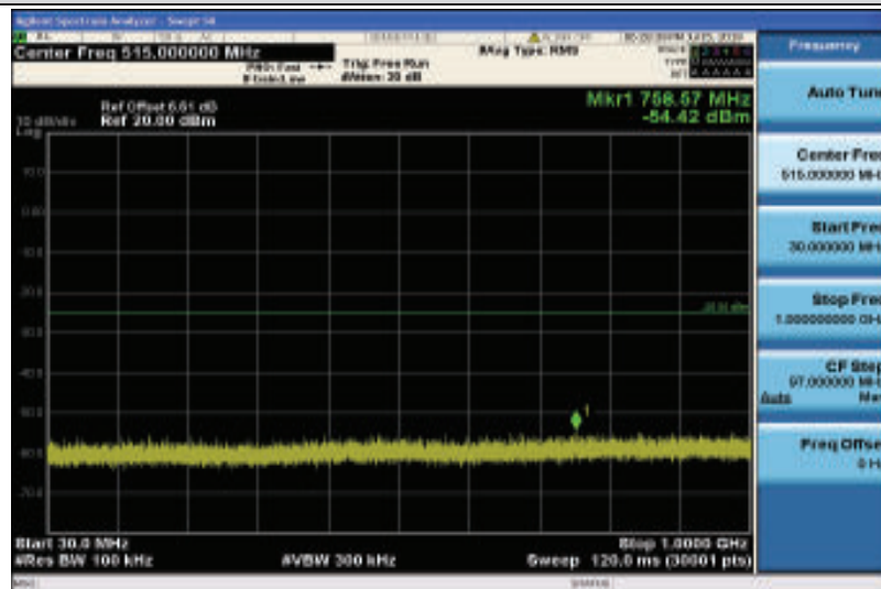
Band38-5MHz-QPSK-38225-1RB#0-Range1:30~1000MHz
