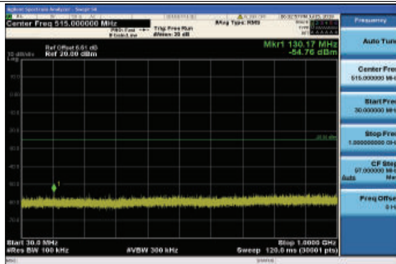
Band38-10MHz-16QAM-37800-1RB#0-Range1:30~1000MHz
