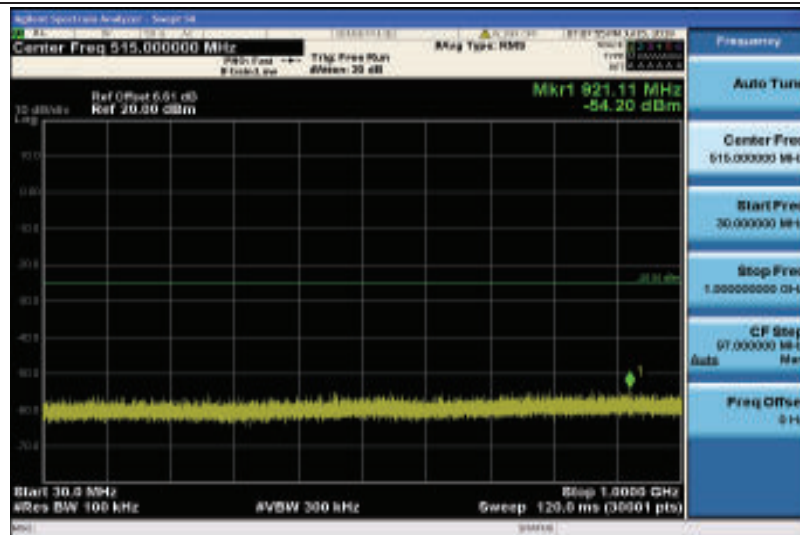
Band38-20MHz-16QAM-37850-1RB#0-Range1:30~1000MHz
