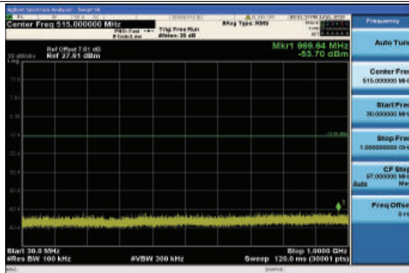
Band25-10MHz-QPSK-26090-1RB#0-30~1000MHz
