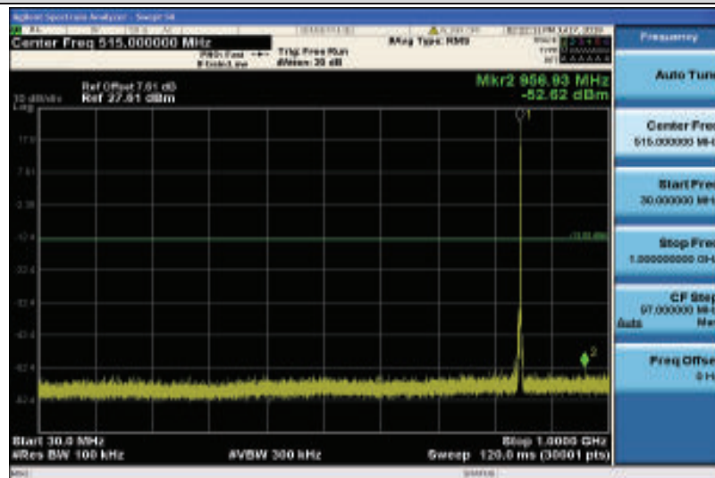
Band26-1.4MHz-QPSK-27033-1RB#0-30~1000MHz
