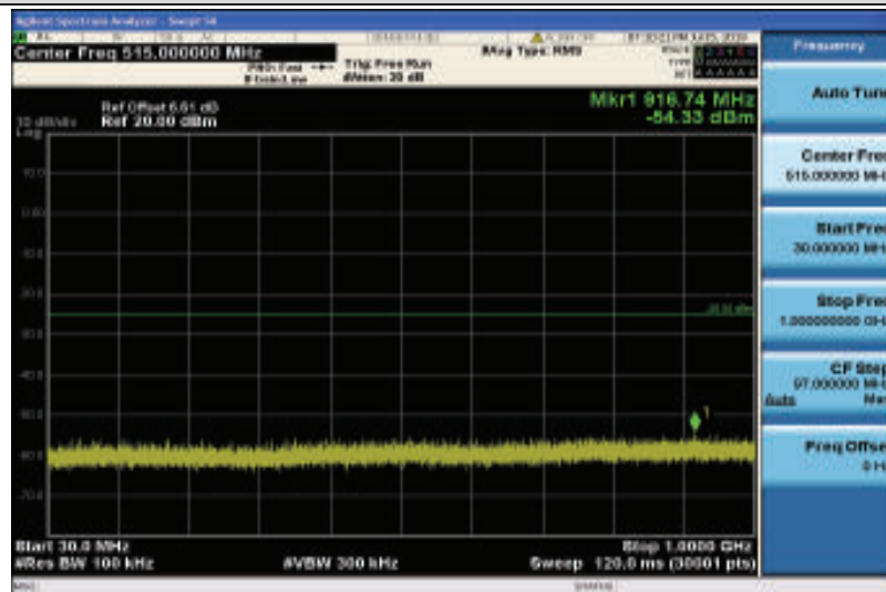
Band38-20MHz-16QAM-38150-1RB#0-Range1:30~1000MHz
