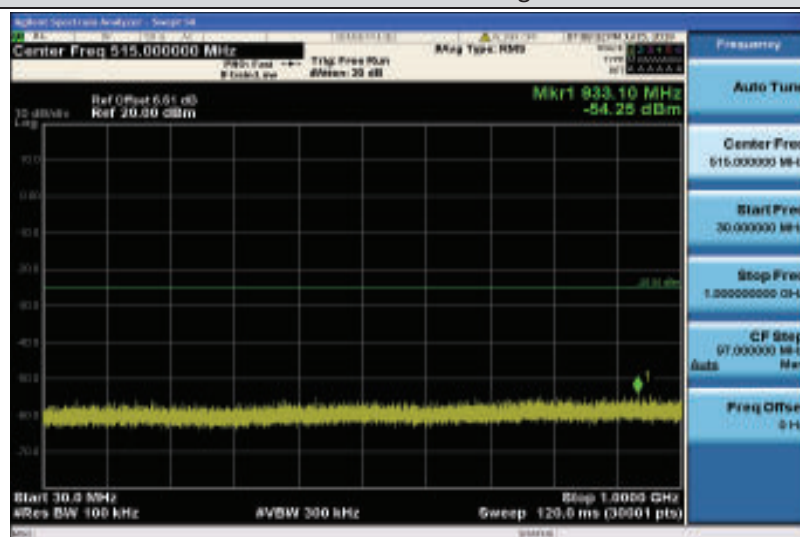
Band38-20MHz-QPSK-38000-1RB#0-Range1:30~1000MHz
