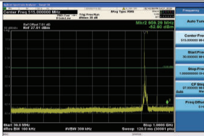
Band26-10MHz-16QAM-26840-1RB#0-30~1000MHz
