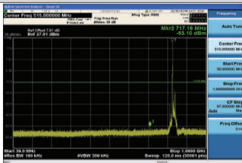
Band26-15MHz-QPSK-26915-1RB#0-30~1000MHz
