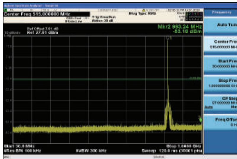
Band26-5MHz-QPSK-26815-1RB#0-30~1000MHz
