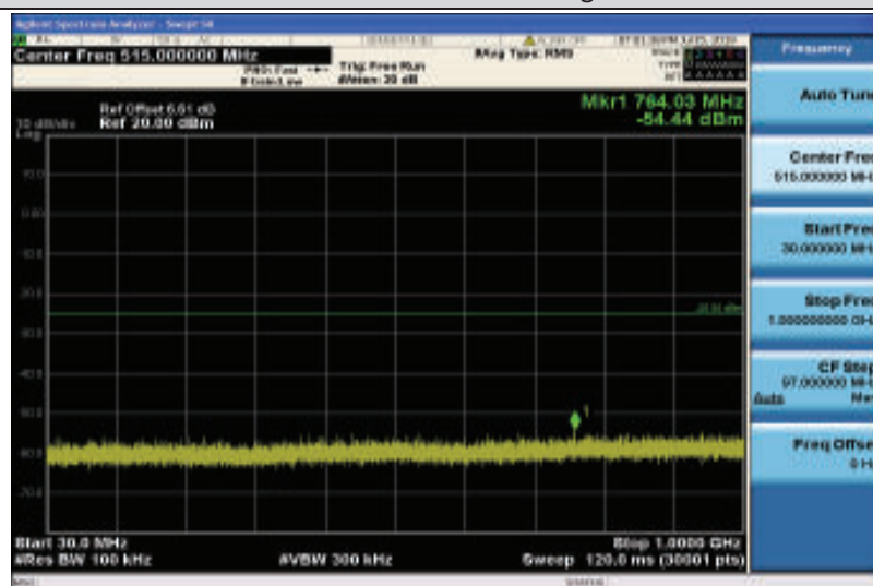
Band38-15MHz-16QAM-38000-1RB#0-Range1:30~1000MHz
