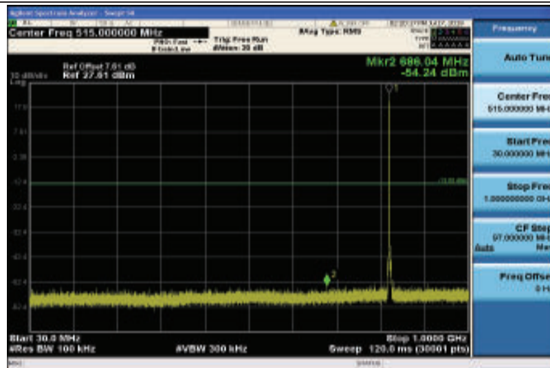
Band26-1.4MHz-16QAM-26797-1RB#0-30~1000MHz
