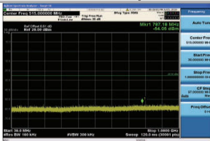
Band38-5MHz-16QAM-38000-1RB#0-Range1:30~1000MHz
