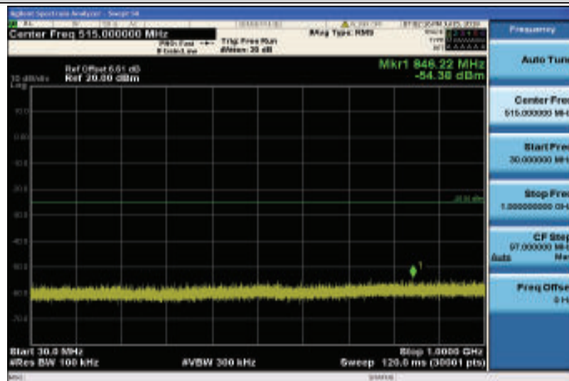
Band38-15MHz-QPSK-38175-1RB#0-Range1:30~1000MHz
