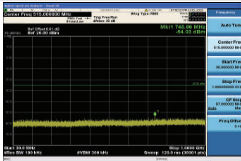
Band38-15MHz-16QAM-37825-1RB#0-Range1:30~1000MHz
