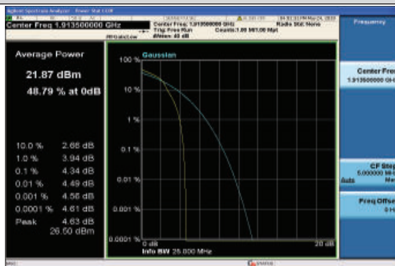
Band25-3MHz-16QAM-26675-1RB#0
