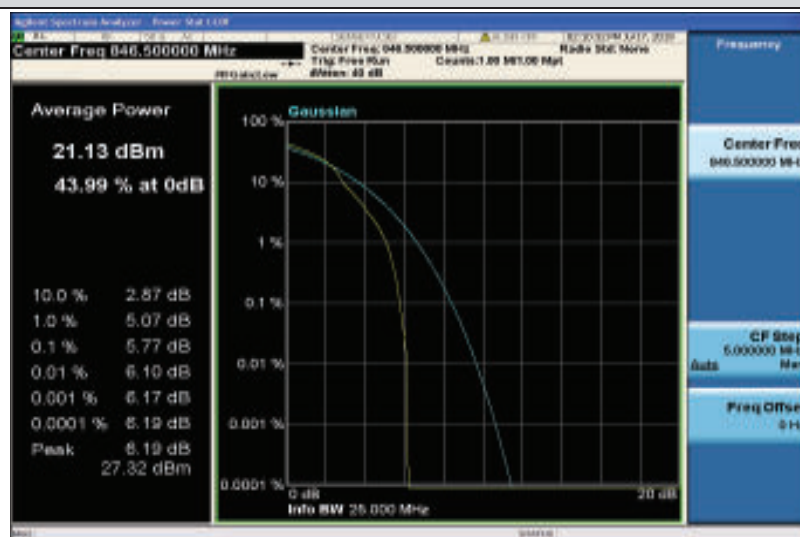
Band26-5MHz-16QAM-27015-1RB#0
