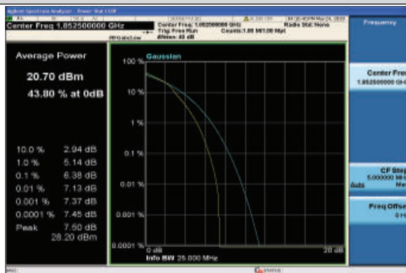
Band25-5MHz-16QAM-26065-25RB#0
