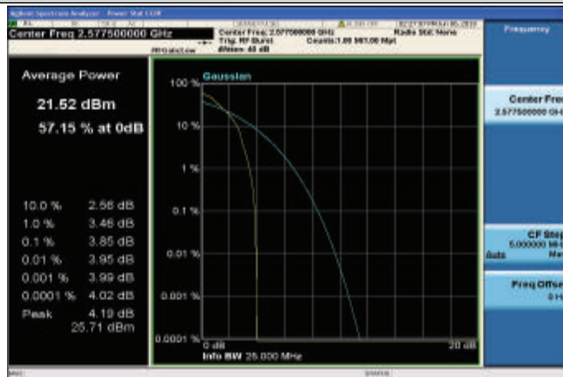
Band38-15MHz-QPSK-37825-1RB#0
