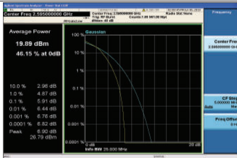
Band38-10MHz-16QAM-38000-50RB#0
