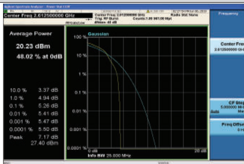
Band38-15MHz-16QAM-38175-1RB#0
