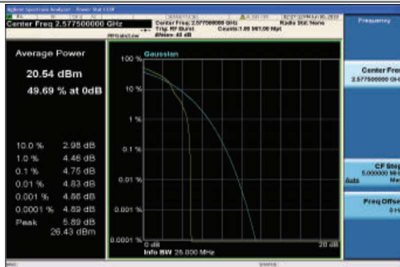
Band38-15MHz-16QAM-37825-1RB#0
