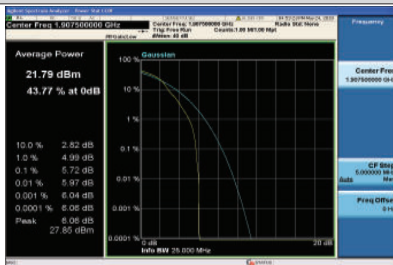
Band25-15MHz-16QAM-26615-1RB#0
