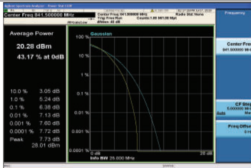
Band26-15MHz-16QAM-26965-75RB#0
