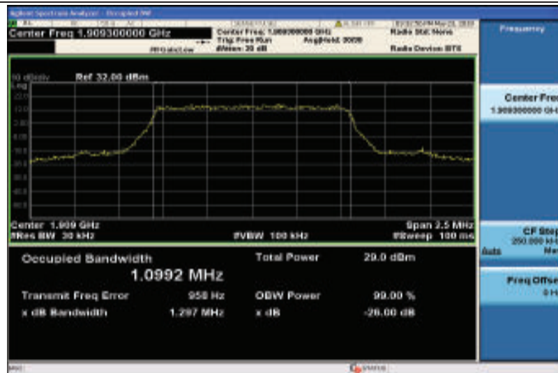
Band2-1.4MHz-QPSK-19193-6RB#0-1.0992
