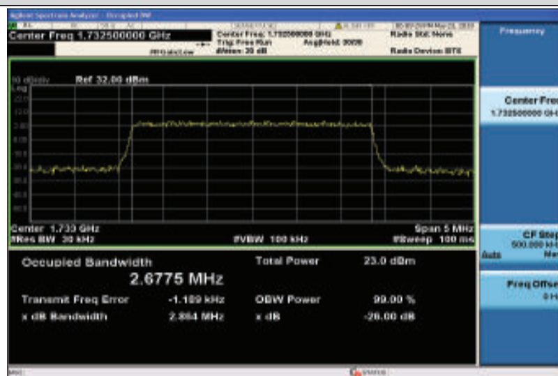
Band4-3MHz-QPSK-20175-15RB#0-2.6775
