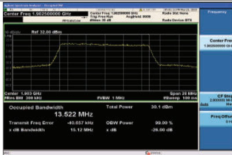
Band2-15MHz-QPSK-19125-75RB#0-13.522
