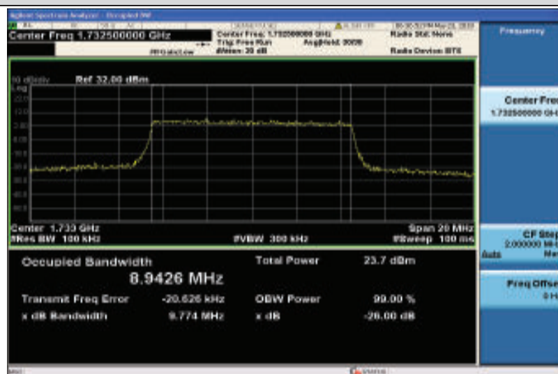
Band4-10MHz-QPSK-20175-50RB#0-8.9426
