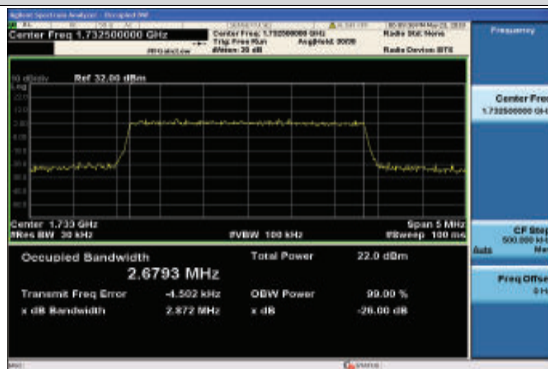
Band4-3MHz-16QAM-20175-15RB#0-2.6793
