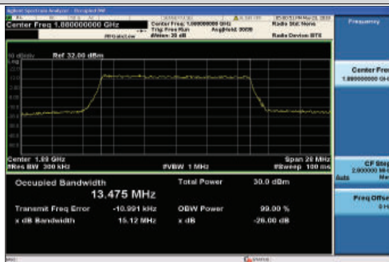
Band2-15MHz-QPSK-18900-75RB#0-13.475
