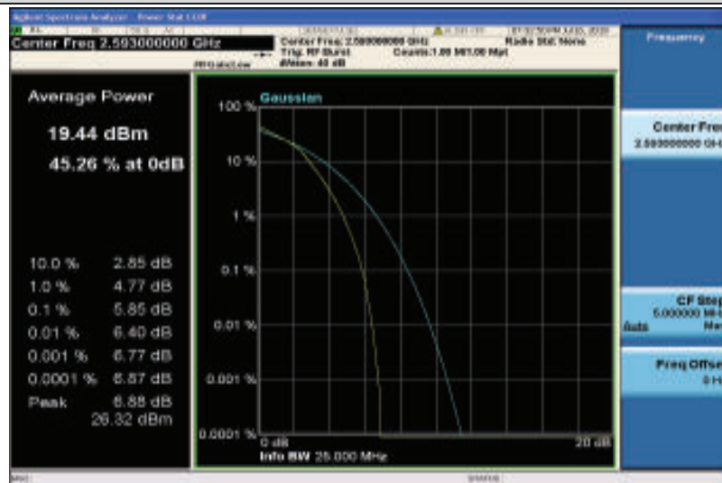
Band41-10MHz-16QAM-40620-50RB#0
