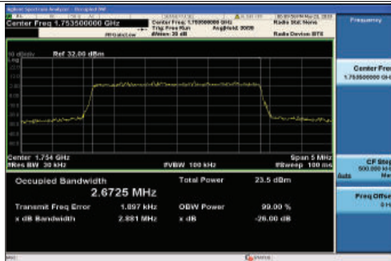
Band4-3MHz-16QAM-20385-15RB#0-2.6725
