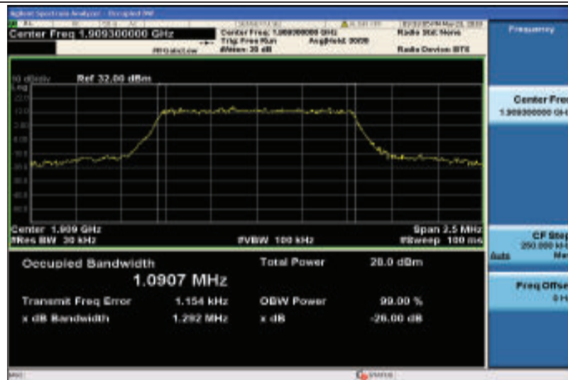
Band2-1.4MHz-16QAM-19193-6RB#0-1.0907
