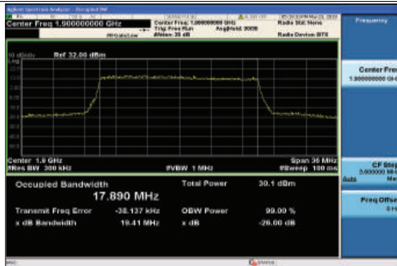
Band2-20MHz-QPSK-19100-100RB#0-17.890
