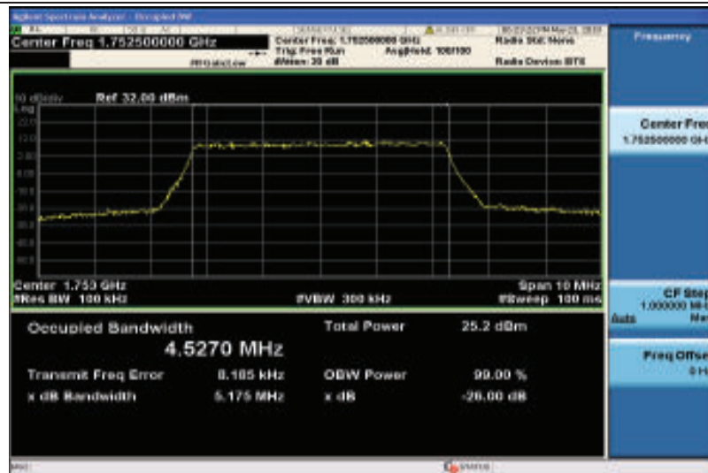
Band4-5MHz-QPSK-20375-25RB#0-4.5270
