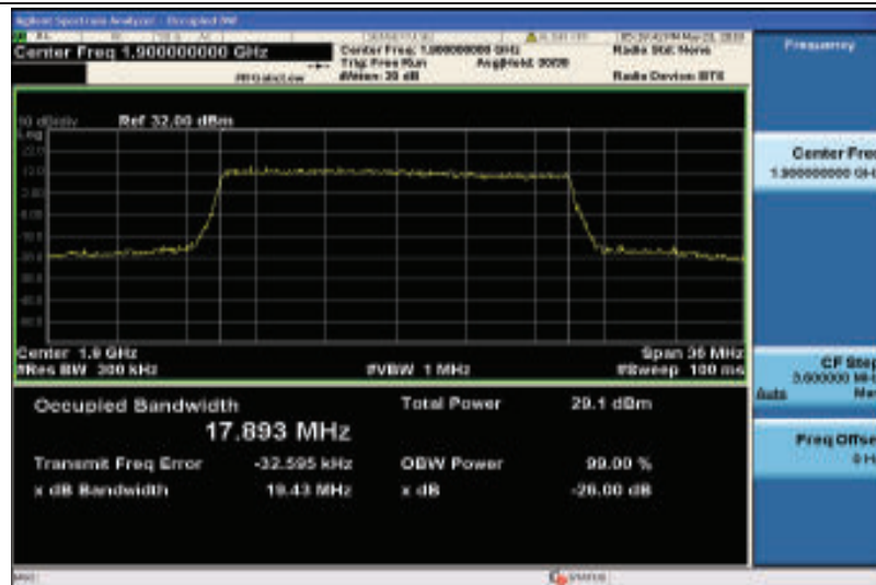
Band2-20MHz-16QAM-19100-100RB#0-17.893
