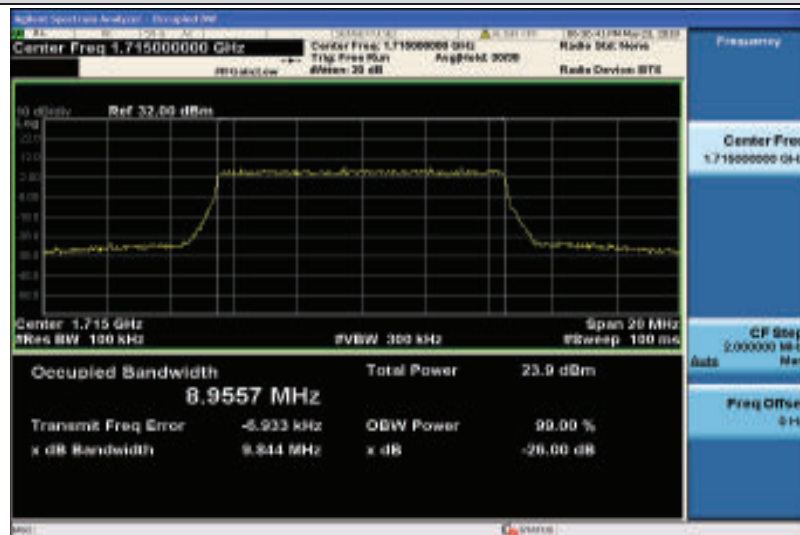
Band4-10MHz-16QAM-20000-50RB#0-8.9557
