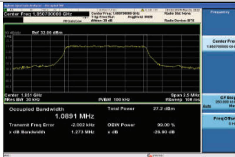
Band2-1.4MHz-16QAM-18607-6RB#0-1.0891
