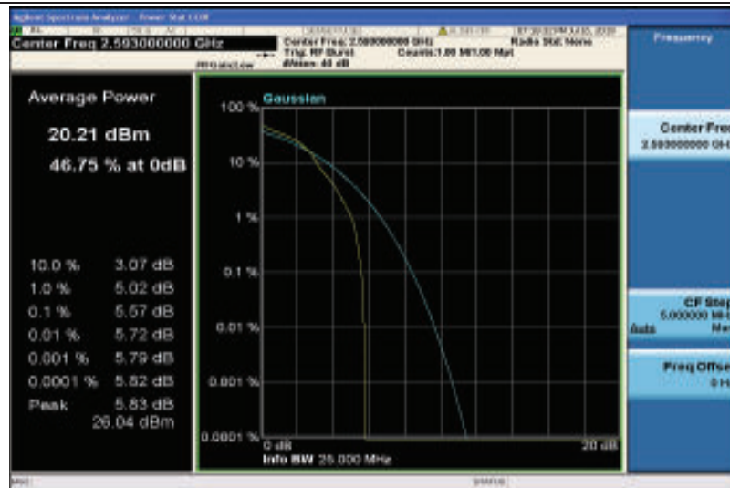
Band41-5MHz-16QAM-40620-1RB#0
