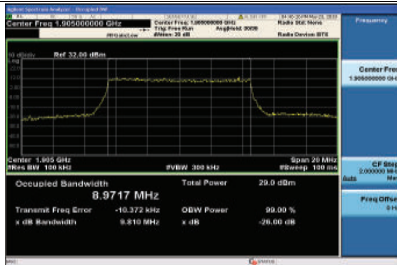
Band2-10MHz-16QAM-19150-50RB#0-8.9717
