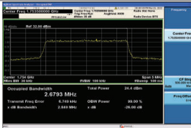
Band4-3MHz-QPSK-20385-15RB#0-2.6793
