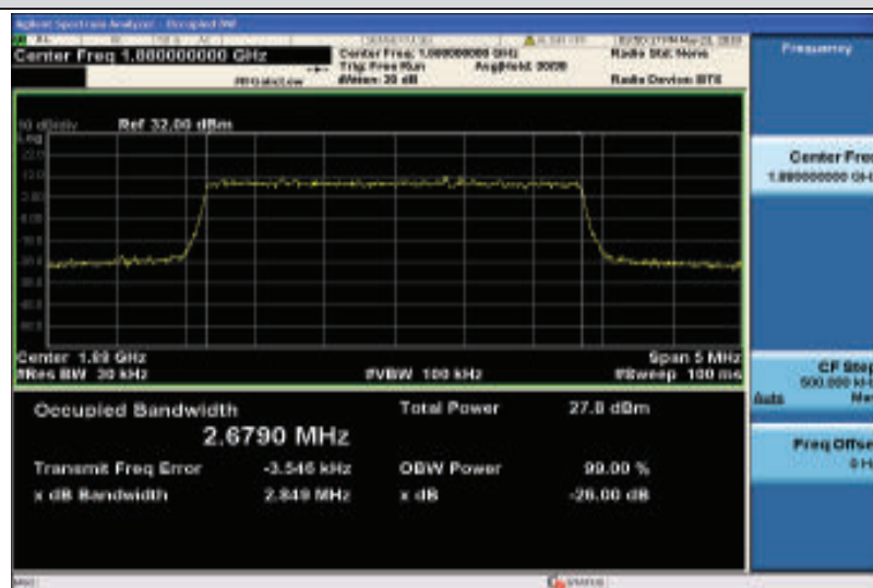
Band2-3MHz-16QAM-18900-15RB#0-2.6790
