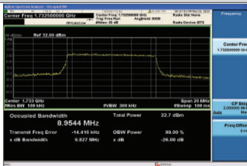
Band4-10MHz-16QAM-20175-50RB#0-8.9544
