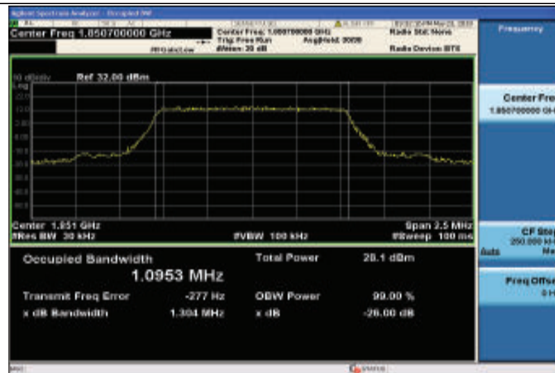
Band2-1.4MHz-QPSK-18607-6RB#0-1.0953
