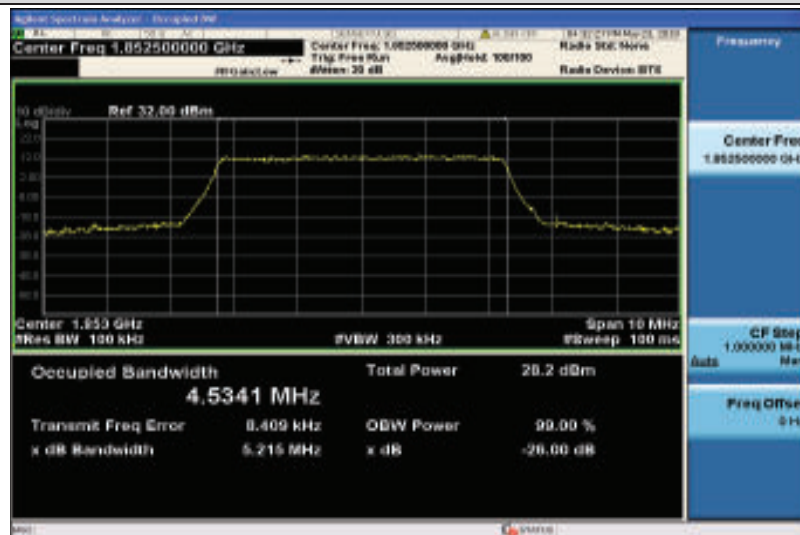
Band2-5MHz-16QAM-18625-25RB#0-4.5341
