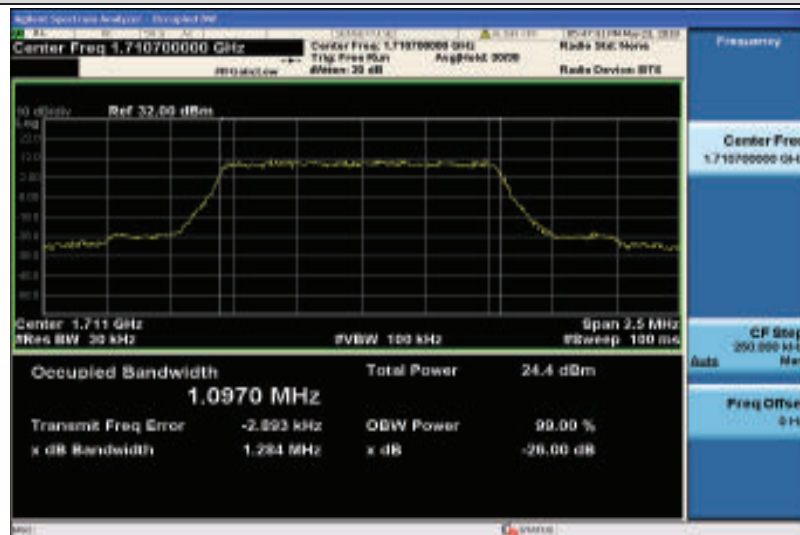
Band4-1.4MHz-QPSK-19957-6RB#0-1.0970
