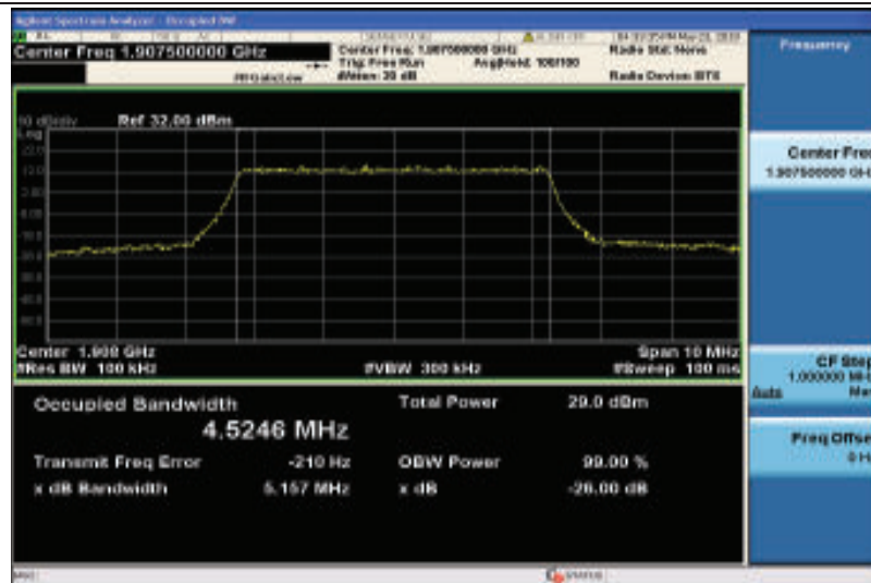
Band2-5MHz-16QAM-19175-25RB#0-4.5246
