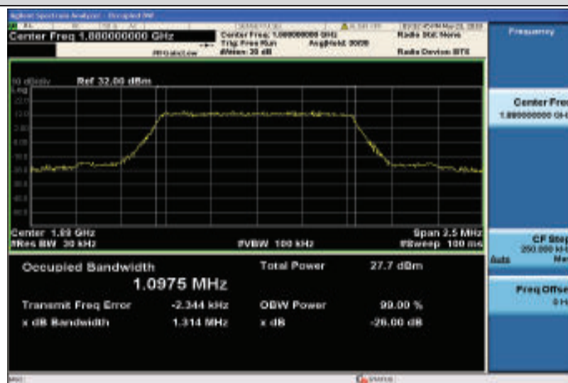
Band2-1.4MHz-16QAM-18900-6RB#0-1.0975
