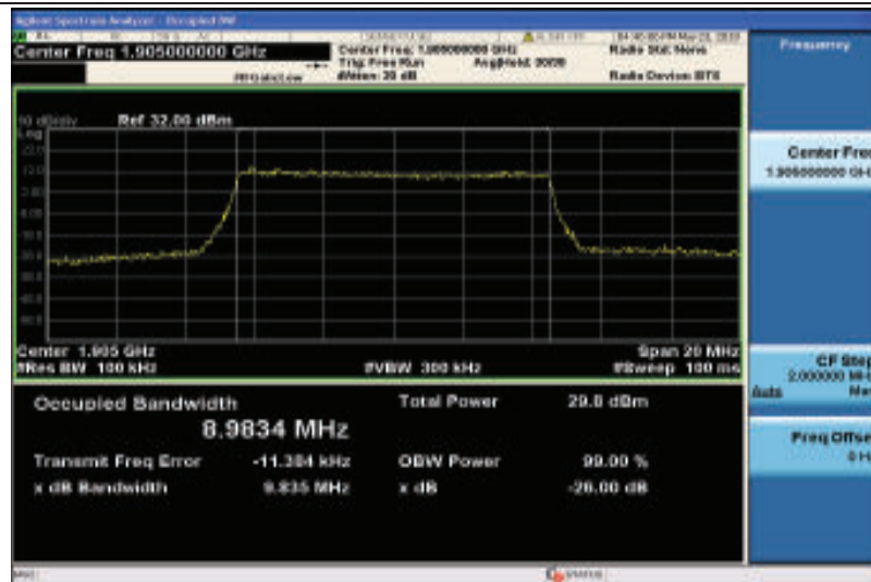
Band2-10MHz-QPSK-19150-50RB#0-8.9834
