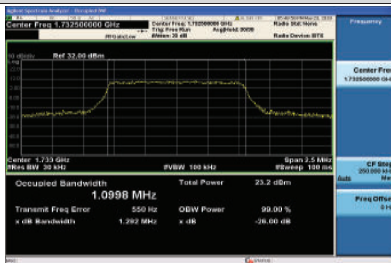
Band4-1.4MHz-QPSK-20175-6RB#0-1.0998
