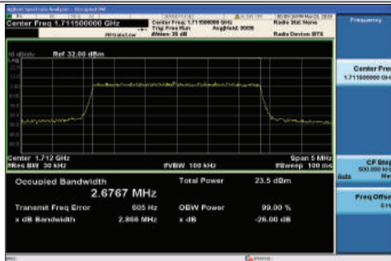
Band4-3MHz-16QAM-19965-15RB#0-2.6767
