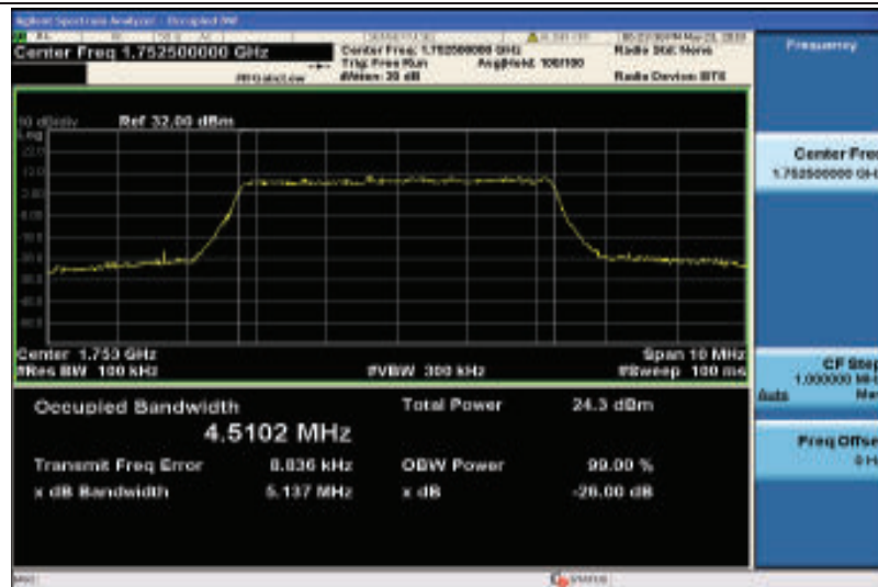
Band4-5MHz-16QAM-20375-25RB#0-4.5102
