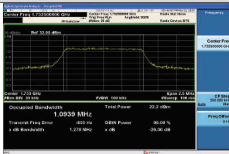
Band4-1.4MHz-16QAM-20175-6RB#0-1.0939
