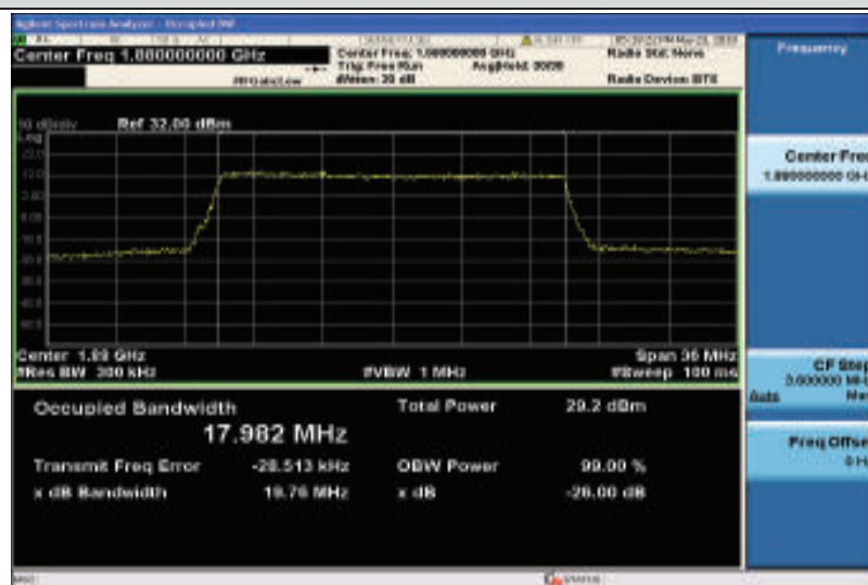
Band2-20MHz-16QAM-18900-100RB#0-17.982
