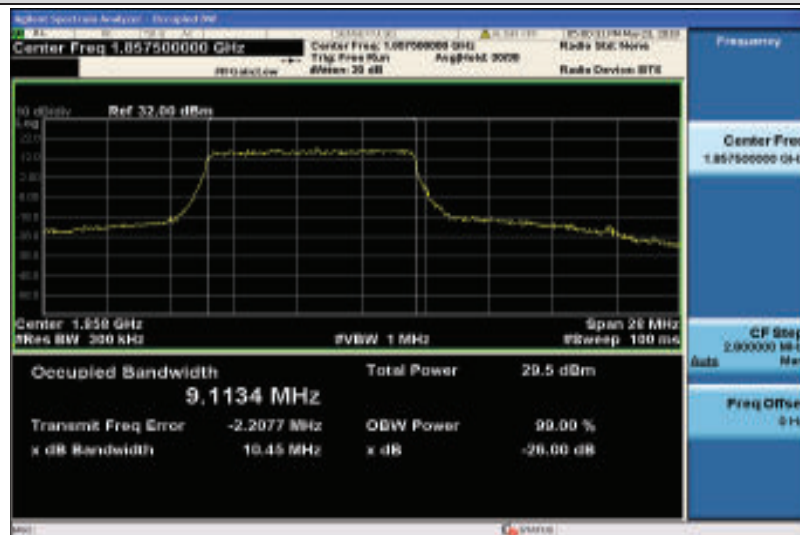
Band2-15MHz-QPSK-18675-75RB#0-9.1134
