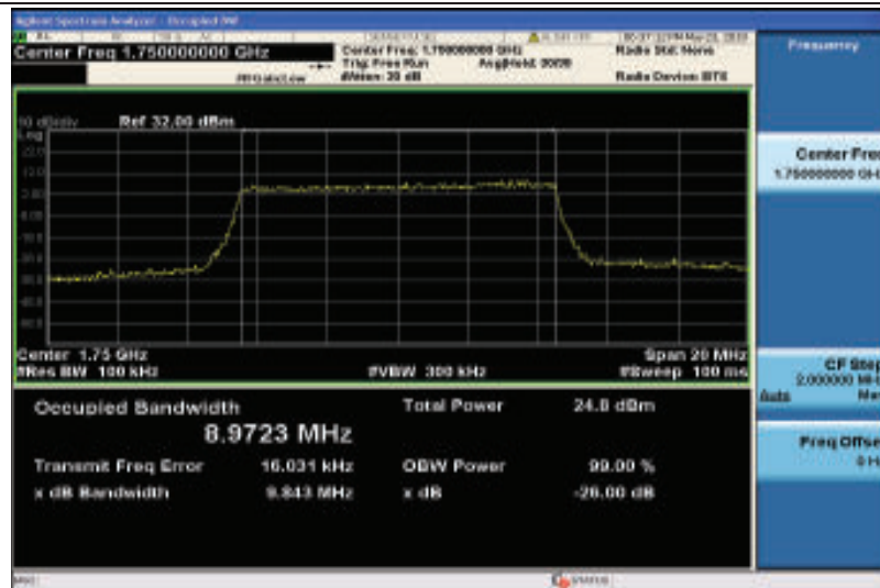
Band4-10MHz-QPSK-20350-50RB#0-8.9723
