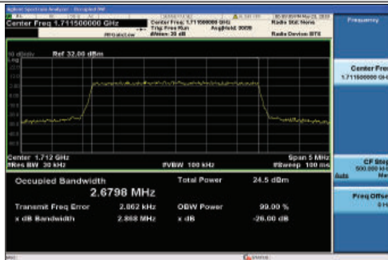
Band4-3MHz-QPSK-19965-15RB#0-2.6798
