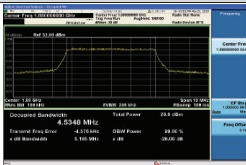
Band2-5MHz-16QAM-18900-25RB#0-4.5348
