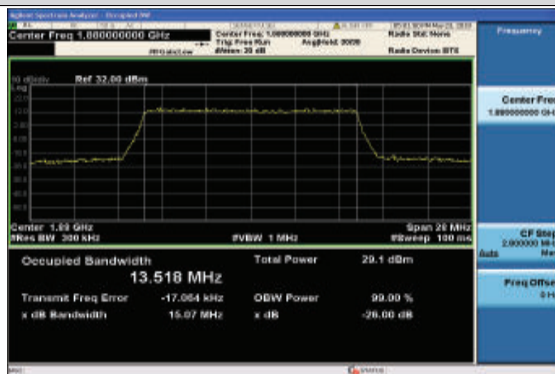
Band2-15MHz-16QAM-18900-75RB#0-13.518
