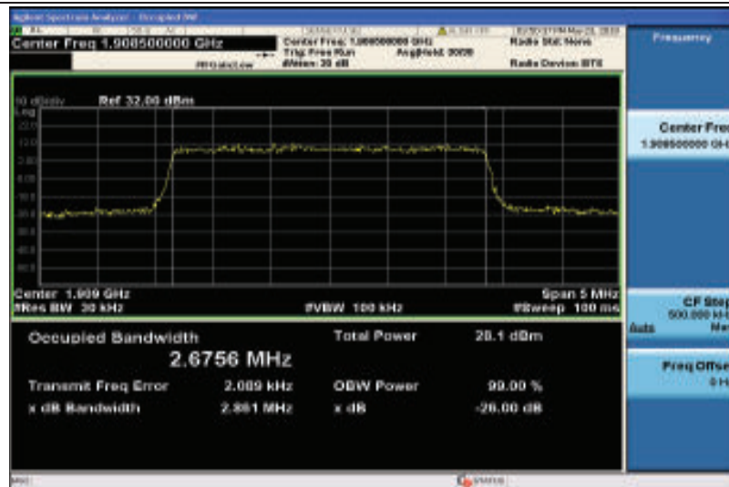
Band2-3MHz-16QAM-19185-15RB#0-2.6756
