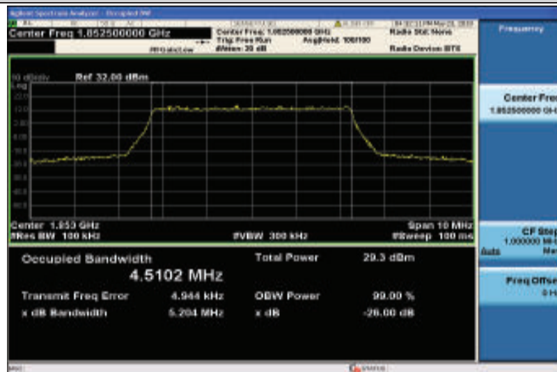
Band2-5MHz-QPSK-18625-25RB#0-4.5102
