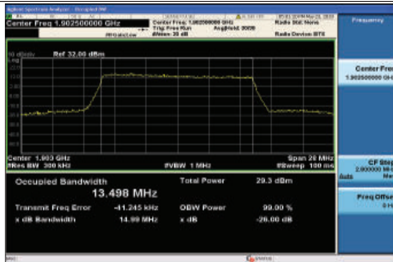
Band2-15MHz-16QAM-19125-75RB#0-13.498
