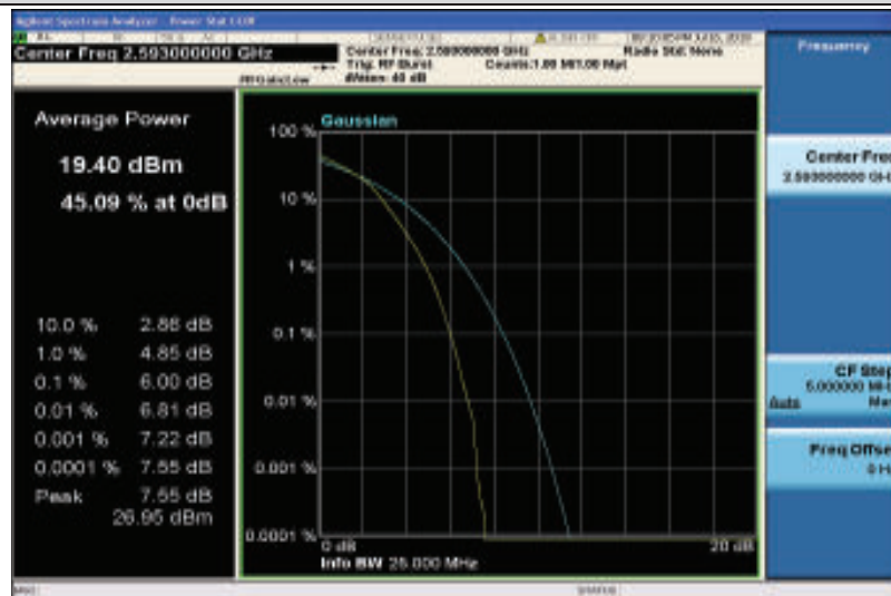
Band41-20MHz-16QAM-40620-100RB#0
