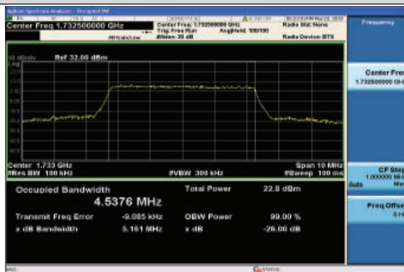
Band4-5MHz-16QAM-20175-25RB#0-4.5376
