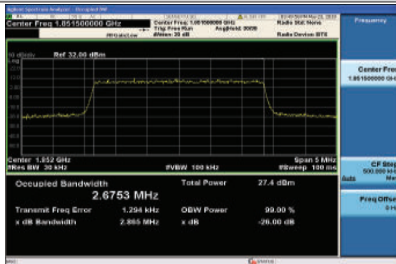
Band2-3MHz-16QAM-18615-15RB#0-2.6753
