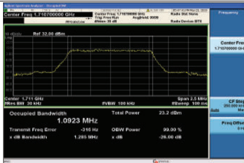
Band4-1.4MHz-16QAM-19957-6RB#0-1.0923
