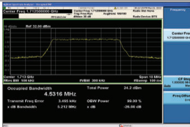
Band4-5MHz-16QAM-19975-25RB#0-4.5316
