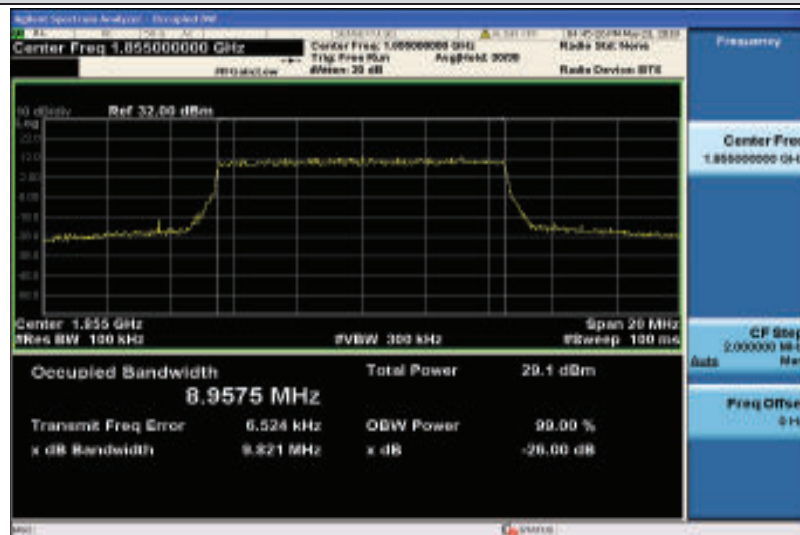
Band2-10MHz-QPSK-18650-50RB#0-8.9575
