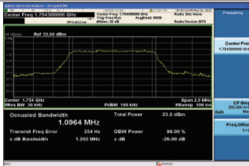
Band4-1.4MHz-16QAM-20393-6RB#0-1.0964
