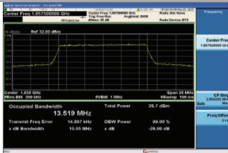
Band2-15MHz-16QAM-18675-75RB#0-13.519
