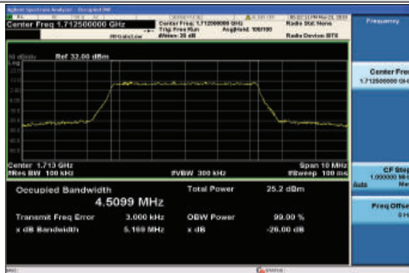
Band4-5MHz-QPSK-19975-25RB#0-4.5099
