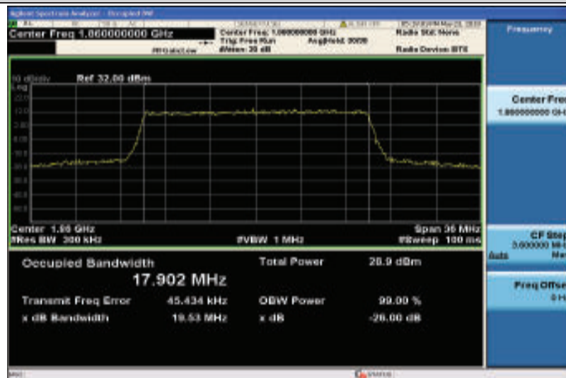
Band2-20MHz-16QAM-18700-100RB#0-17.902
