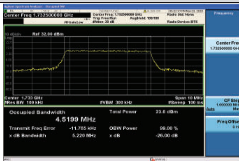
Band4-5MHz-QPSK-20175-25RB#0-4.5199
