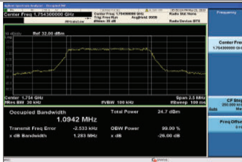
Band4-1.4MHz-QPSK-20393-6RB#0-1.0942
