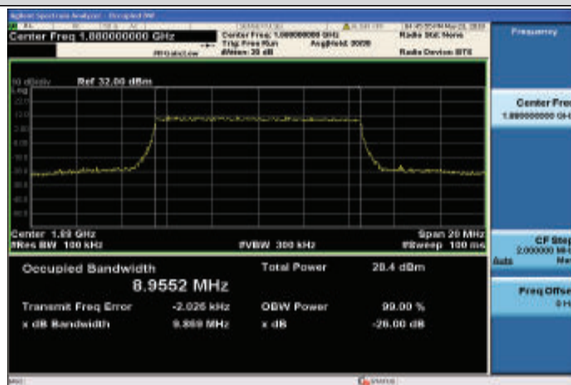
Band2-10MHz-16QAM-18900-50RB#0-8.9552
